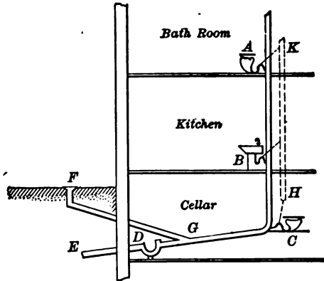
HOUSE-SEWERAGE PIPES.
