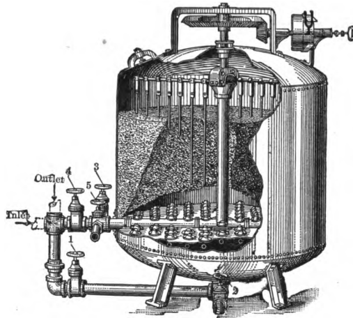
JEWELL MECHANICAL FILTER.
