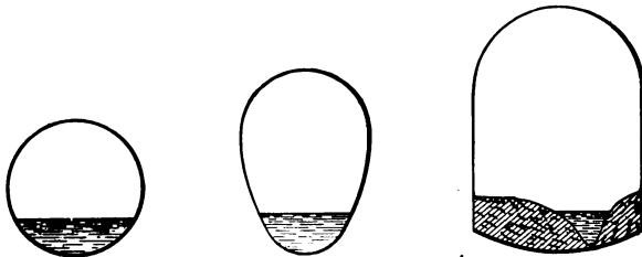
SHAPES OF SEWERS.
