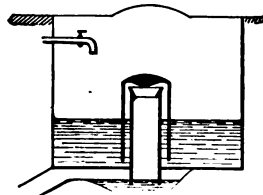
SYPHON FLUSH TANK.
