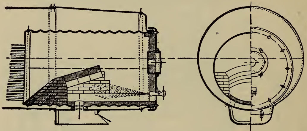
Figure 223m. Oil-Burner in Vanderbilt Type of Firebox.
