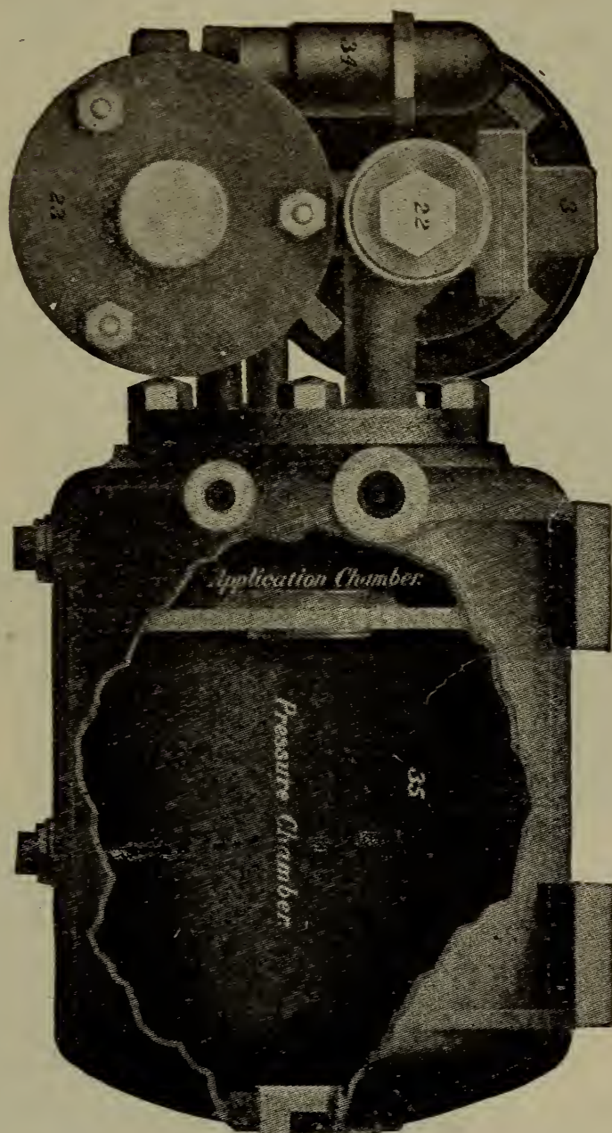
FIG. 297. DISTRIBUTING VALVE AND DOUBLE-CHAMBER RESERVOIR
