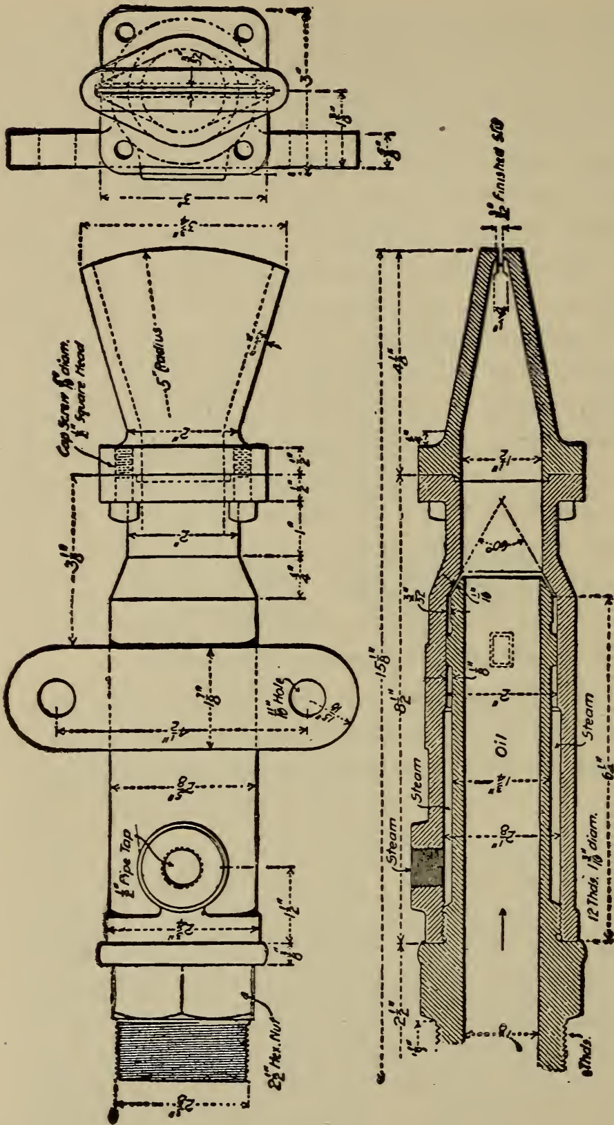
Figure 2231. Details of "Lundholm" Oil-Burner.
