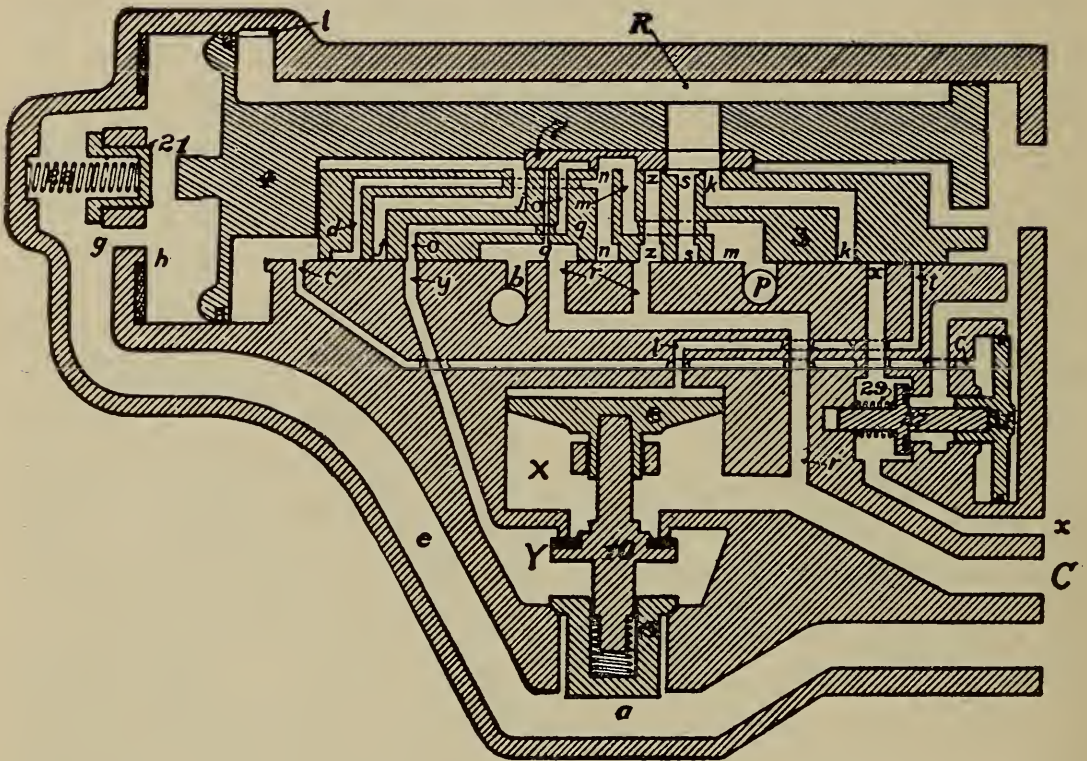
FIG. 354. SERVICE-LAP POSITION
