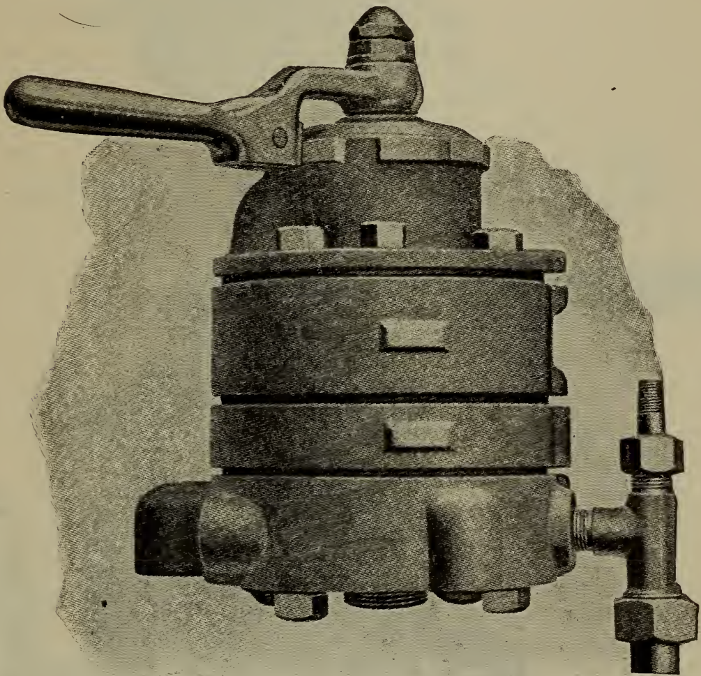
FIG. 310. TYPE H BRAKE VALVE
