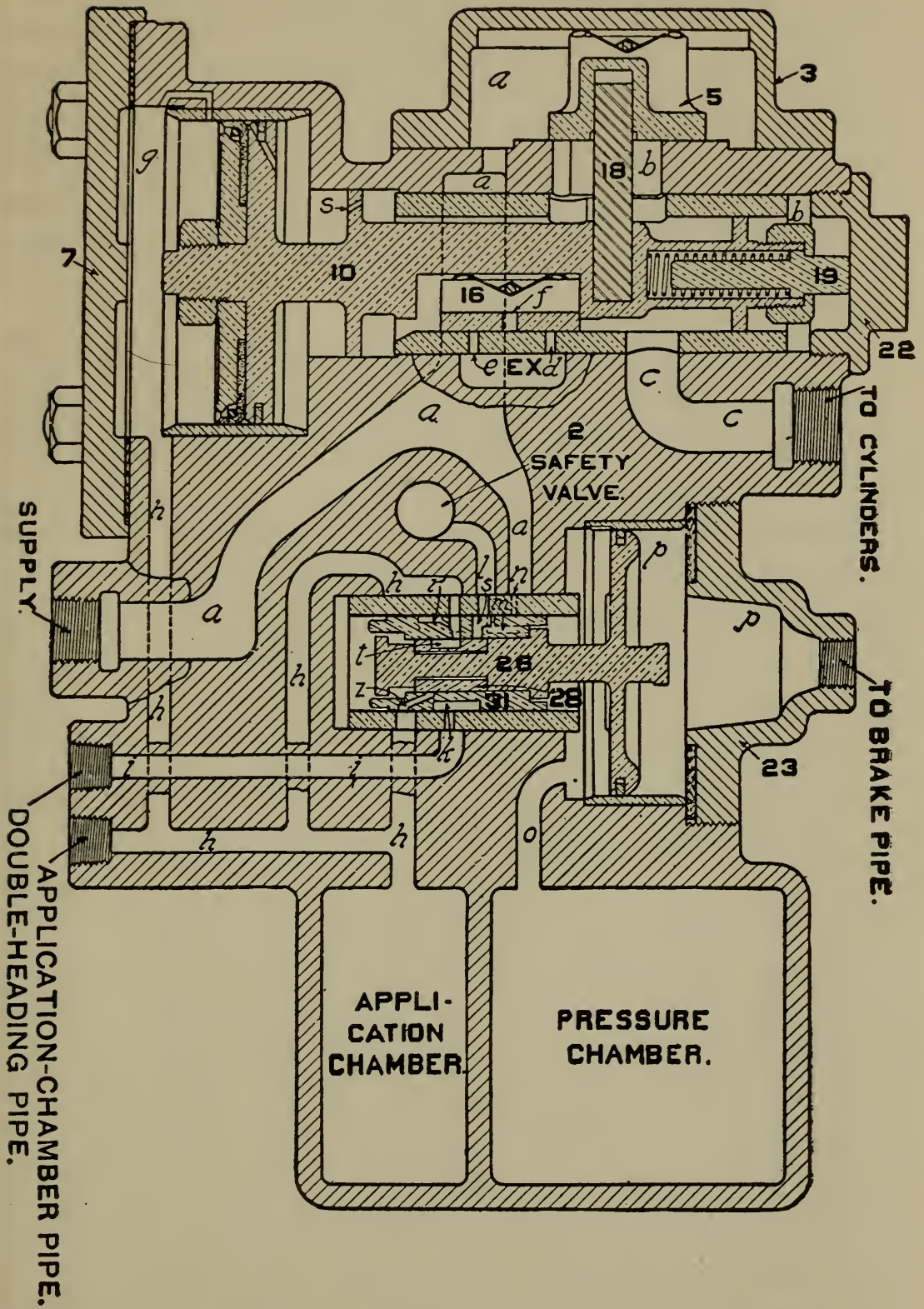
FIG. 303. SERVICE LAP
