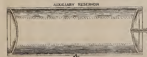
PLATE 32 Diagrammatic Illustration of the Westinghouse Quick-Action Automatic Brake
