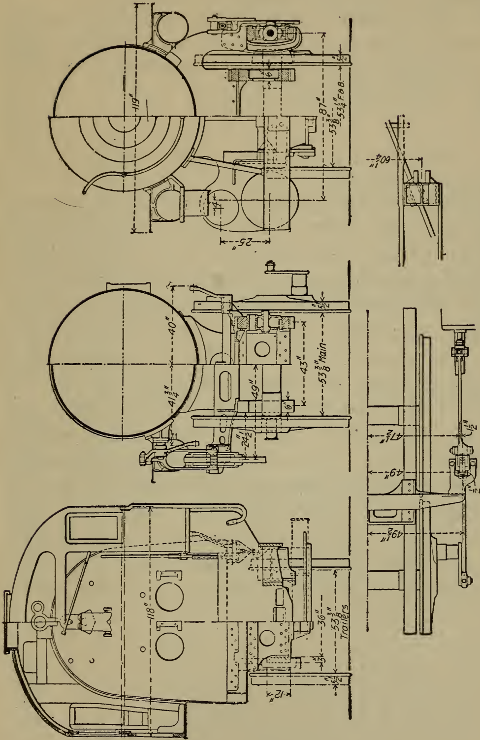
FIG. 342. PRAIRIE TYPE PASSENGER LOCOMOTIVE— PENNSYLVANIA RAILROAD—WALSCHAERT VALVE GEAR
