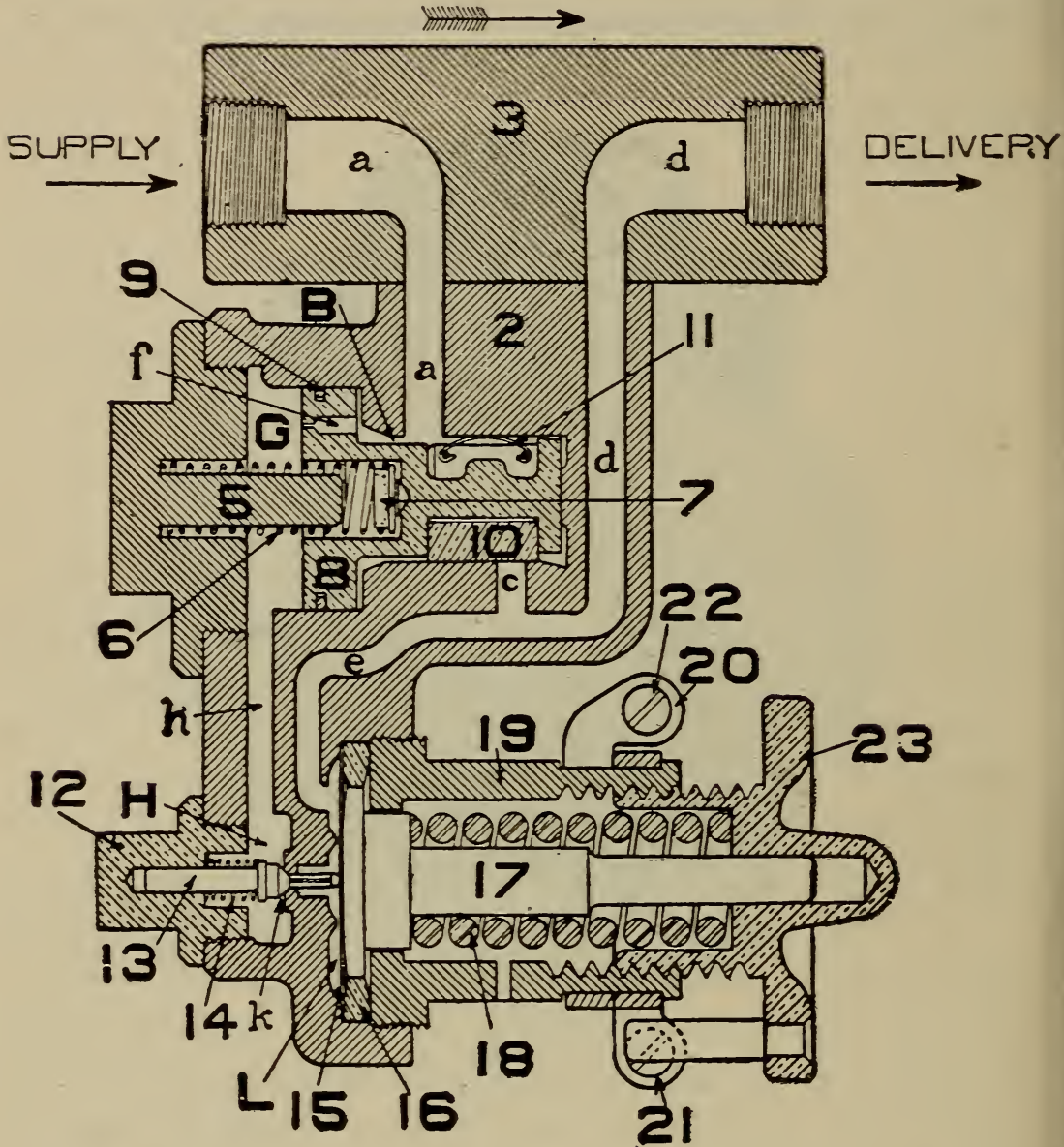
FIG. 318. DIAGRAM OF FEED VALVE, CLOSED
