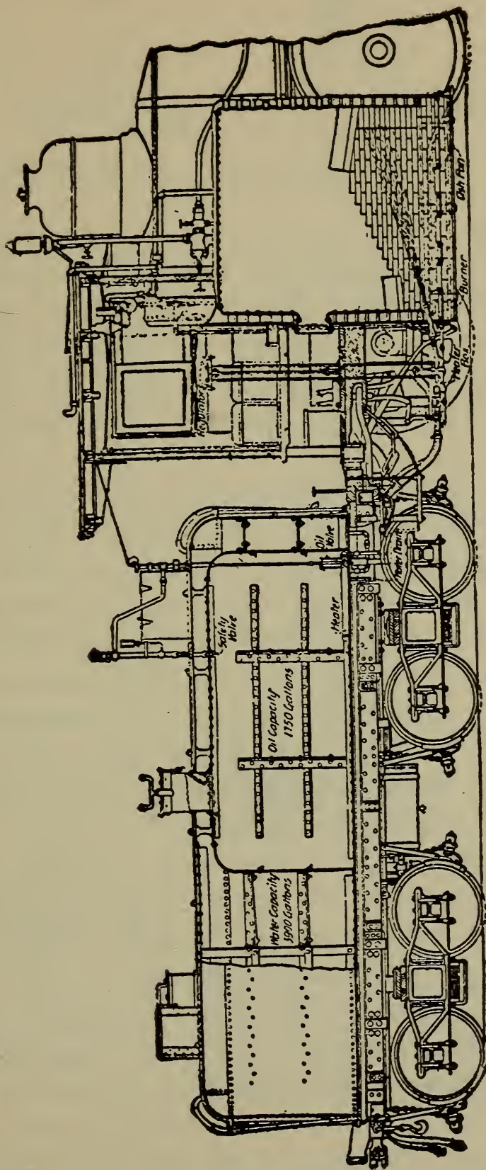
Figure 223b. General Arrangement of Oil-Burning Locomotive—Santa Fe.
