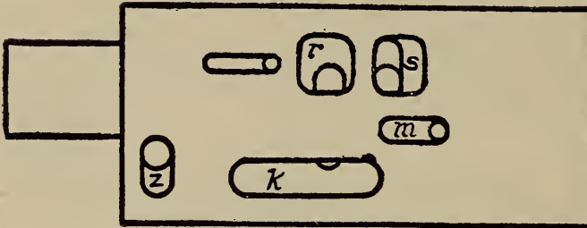
FACE OF SLIDE VALVE.
