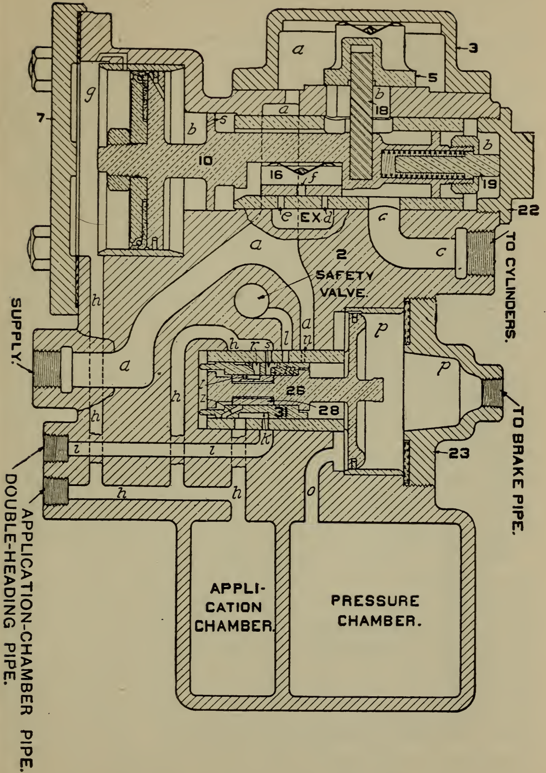
FIG. 301. INDEPENDENT LAP
