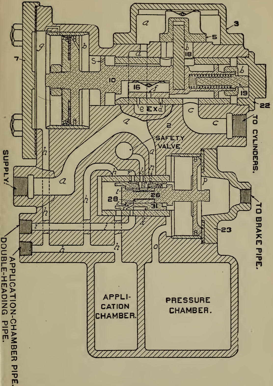
FIG. 305. EMERGENCY LAP
