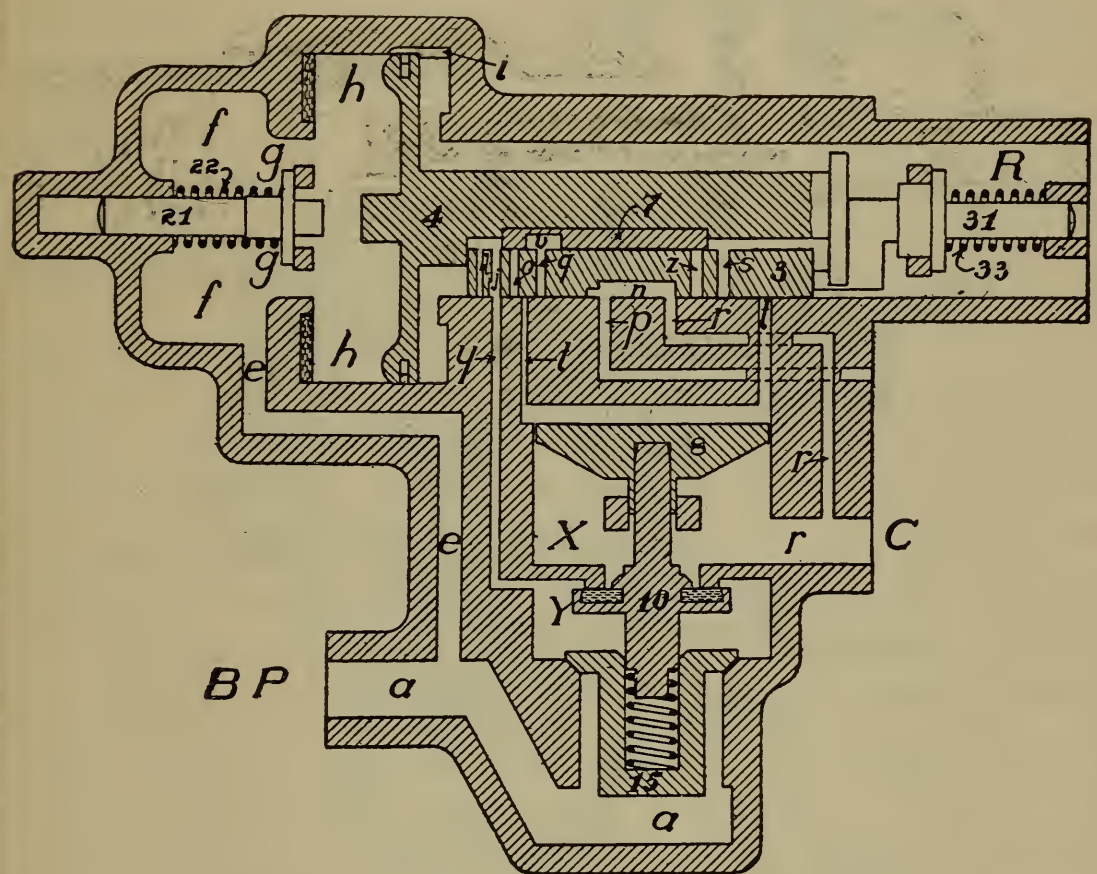
FIG. 326. FULL-RELEASE AND CHARGING POSITION
