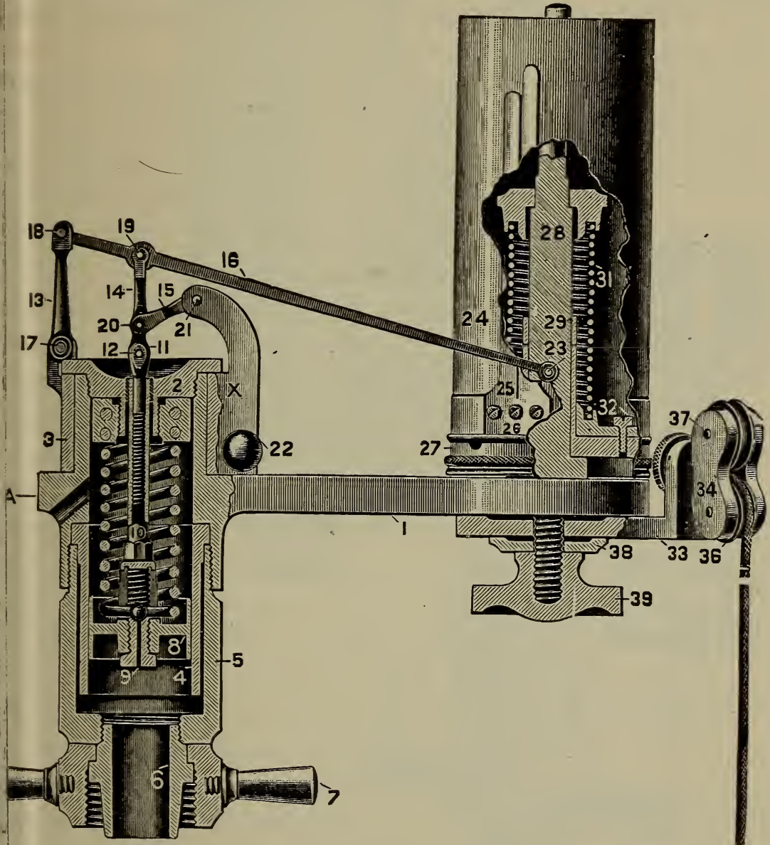
SECTIONAL VIEW CROSBY INDICATOR
