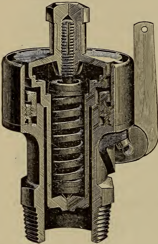
FIGURE 194 KUNKLE POP VALVE FOR PORTABLE AND STATIONARY BOILERS
