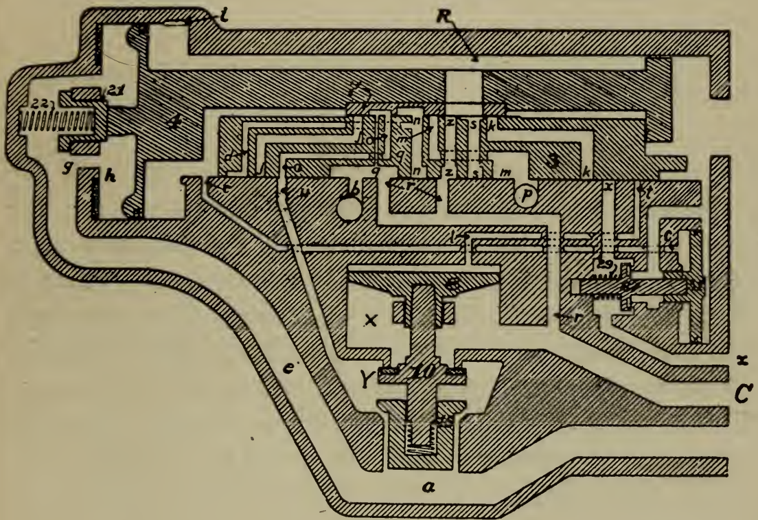
FIG. 352 QUICK-SERVICE POSITION
