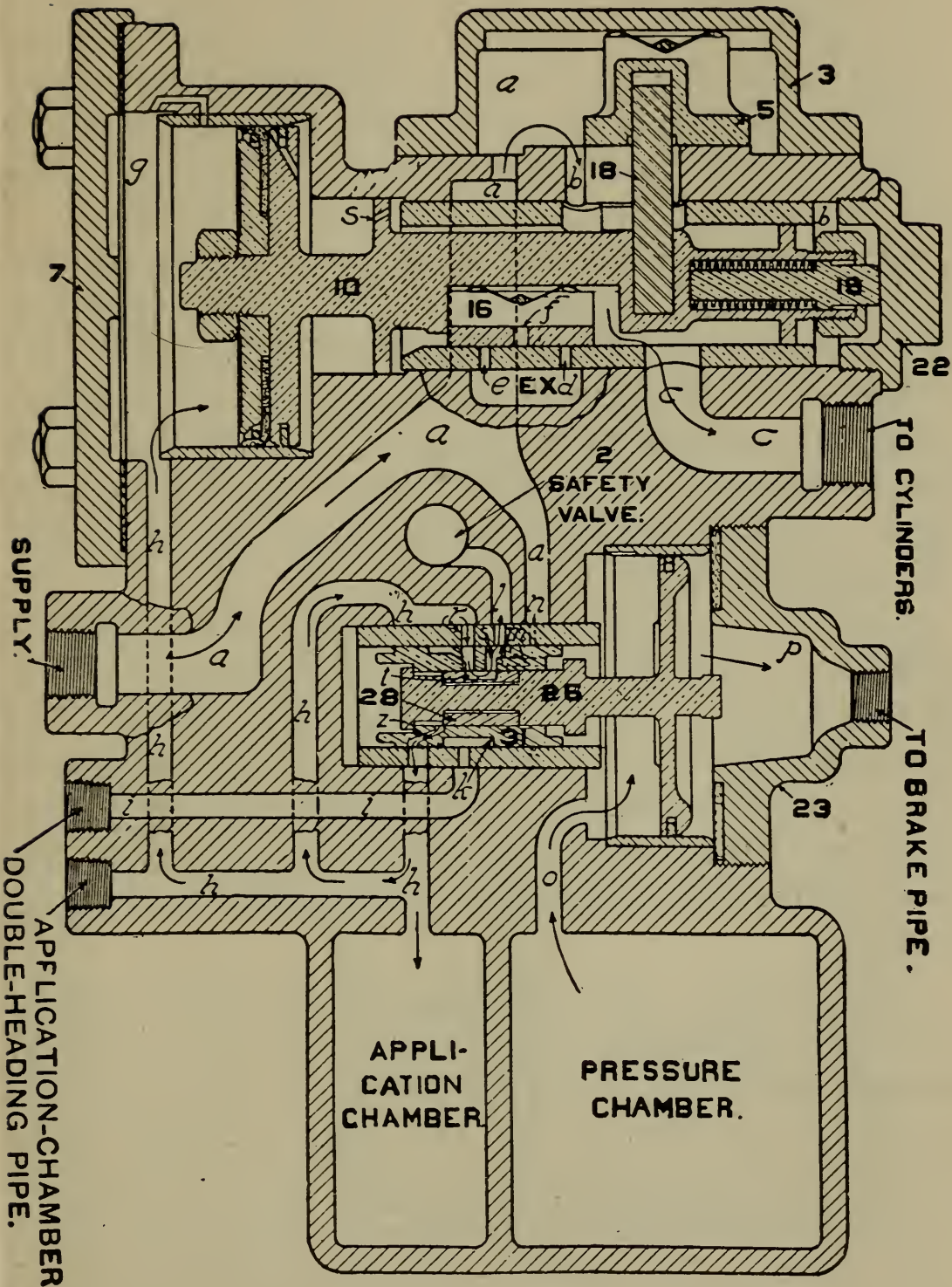
FIG. 302. AUTOMATIC SERVICE
