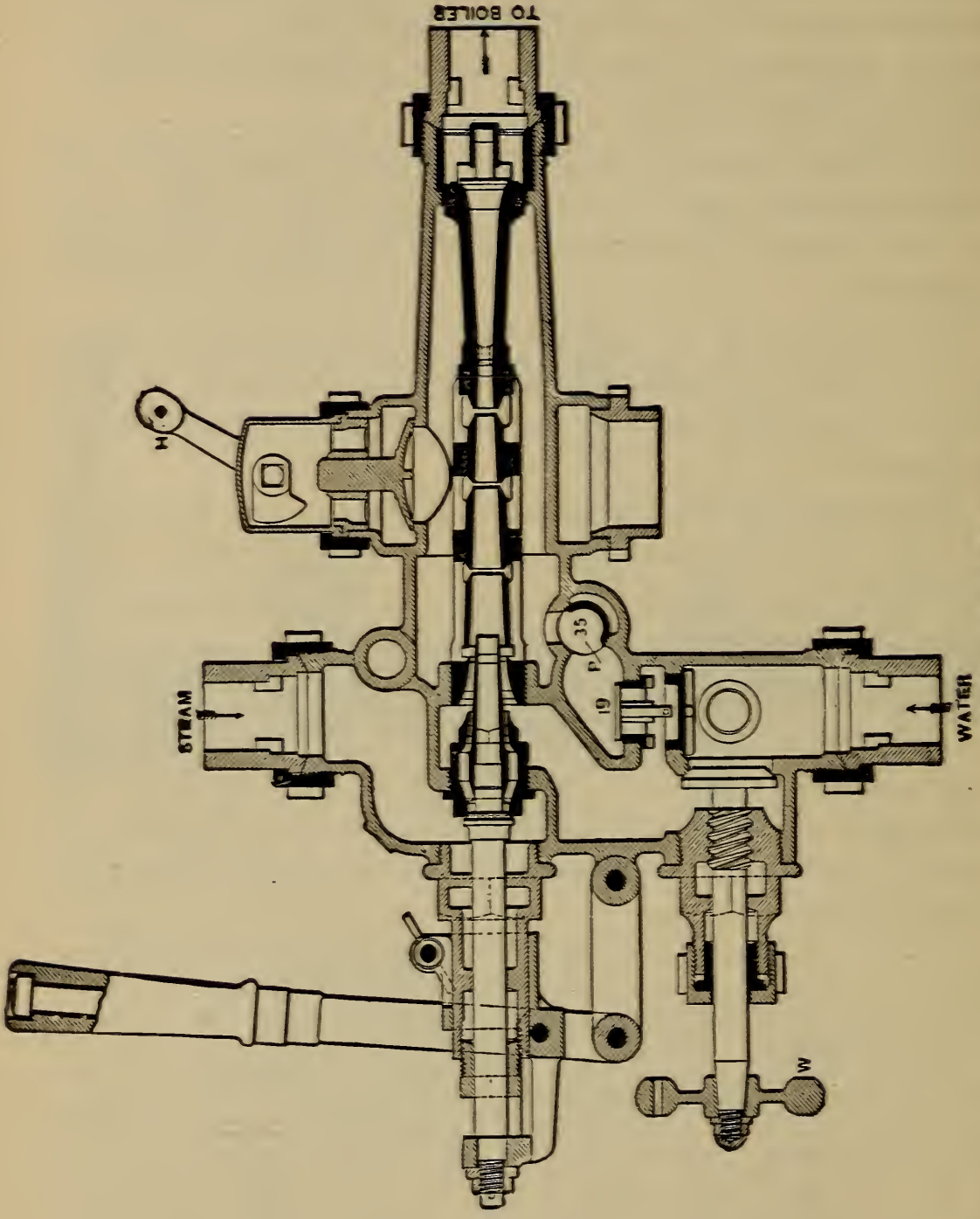
FIGURE 170 THE SIMPLEX INJECTOR
