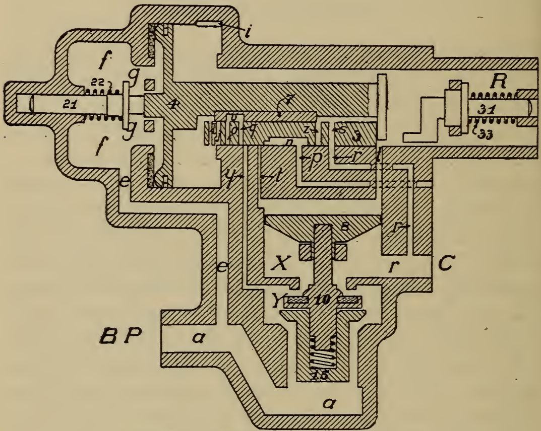
FIG. 331. EMERGENCY POSITION
