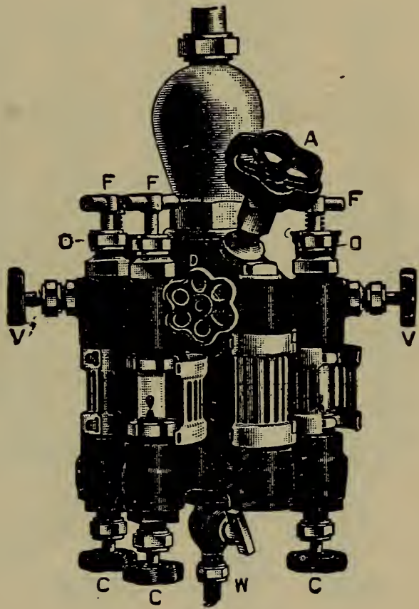
FIGURE 198 NEW NATHAN LUBRICATOR, FRONT VIEW
