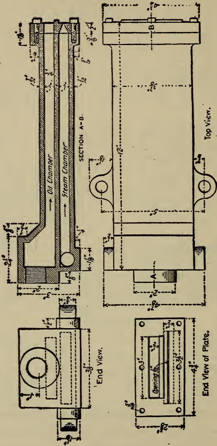
Figure 223f. Details of 'Booth-Wade' Oil-Burner. First Type Used in United States.
