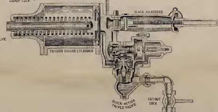
PLATE 32 Diagrammatic Illustration of the Westinghouse Quick-Action Automatic Brake
