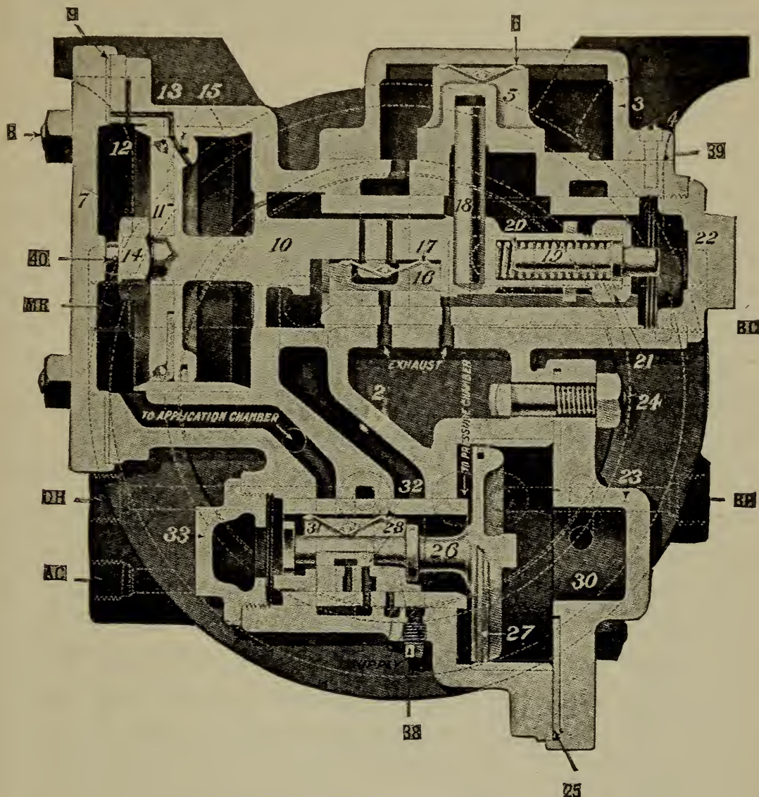
FIG. 308. DISTRIBUTING VALVE
