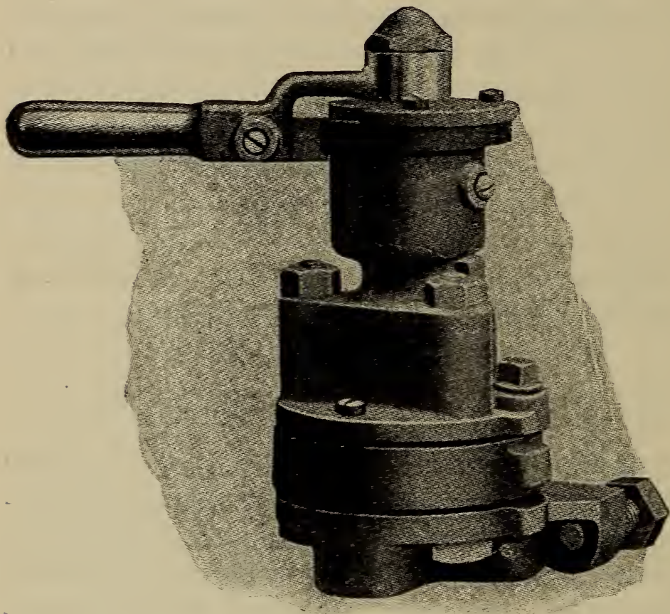
FIG. 314. THE INDEPENDENT BRAKE VALVE
