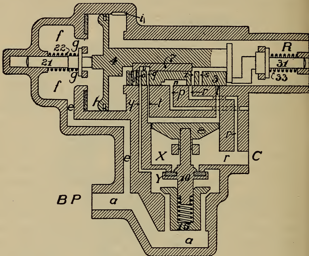
FIG. 327. QUICK SERVICE POSITION
