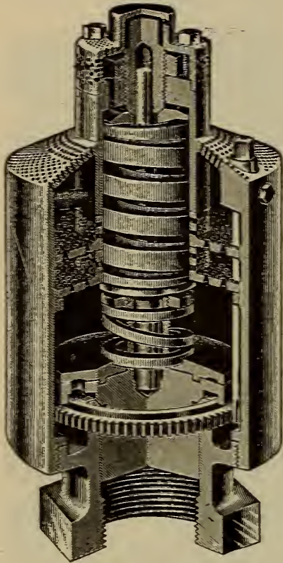
FIGURE 190 CRANE POP VALVE, SECTIONAL VIEW
