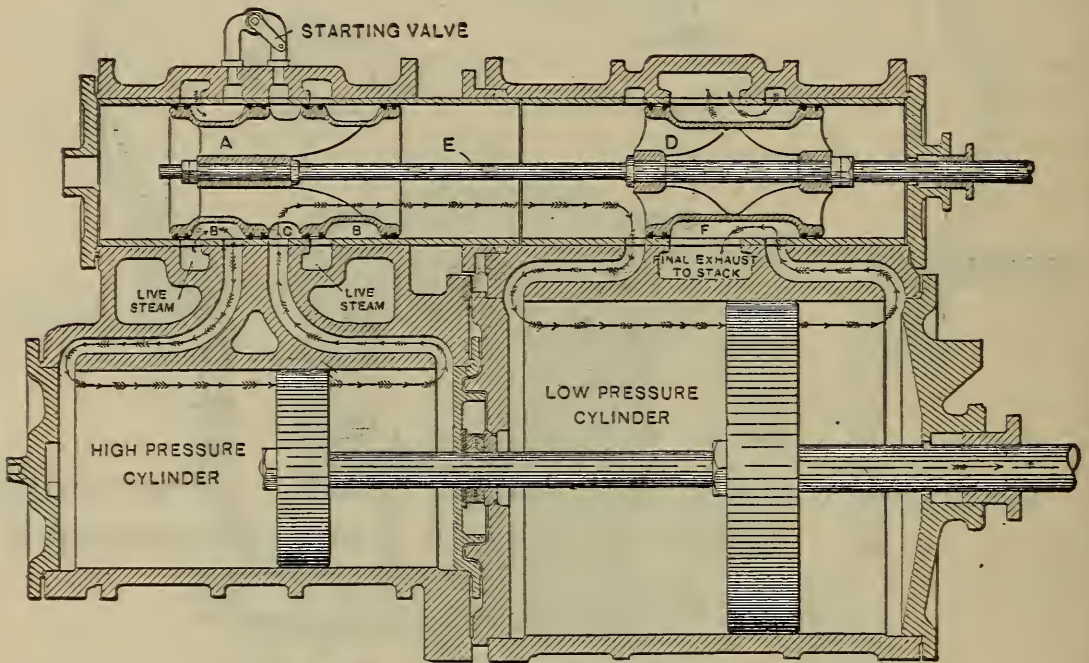
STEAM DISTRIBUTION IN TANDEM COMPOUND CYLINDERS
