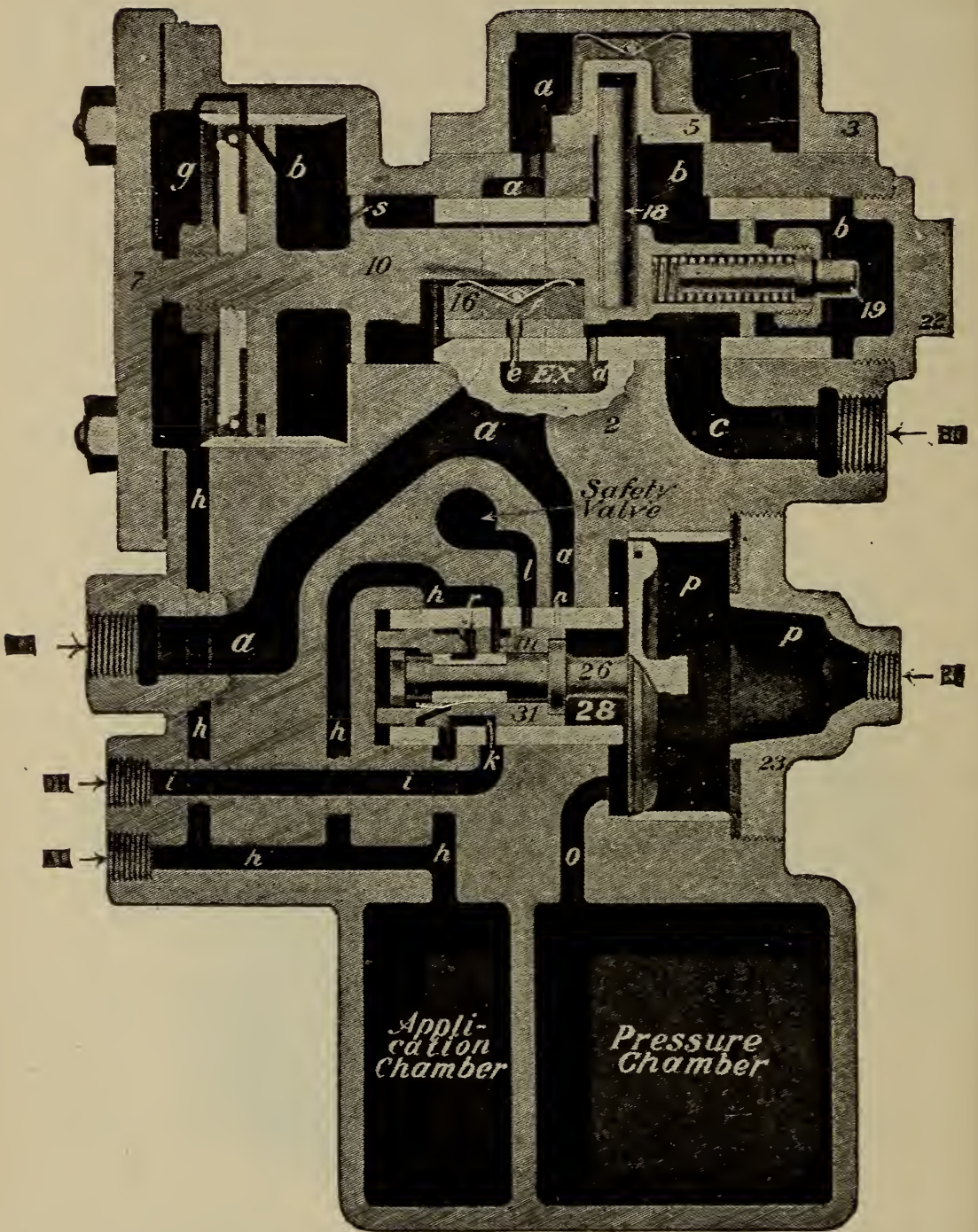
FIG. 298. THE DISTRIBUTING VALVE, DIAGRAMMATIC CONNECTIONS:
