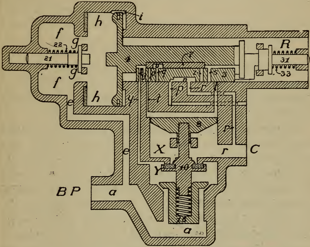
FIG. 330. RETARDED-RELEASE POSITION
