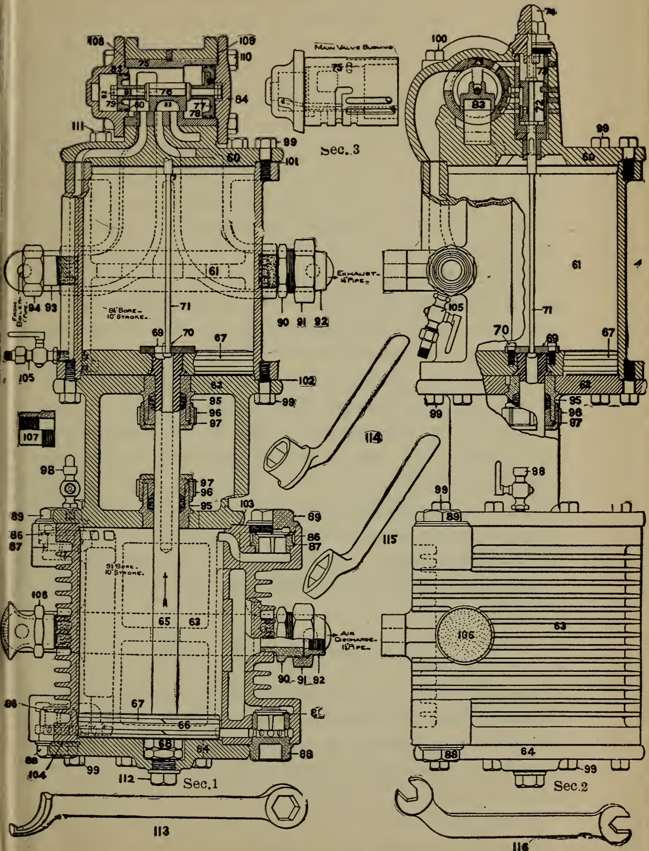
FIGURE 225 NINE AND ONE-HALF INCH PUMP — See page 520.
