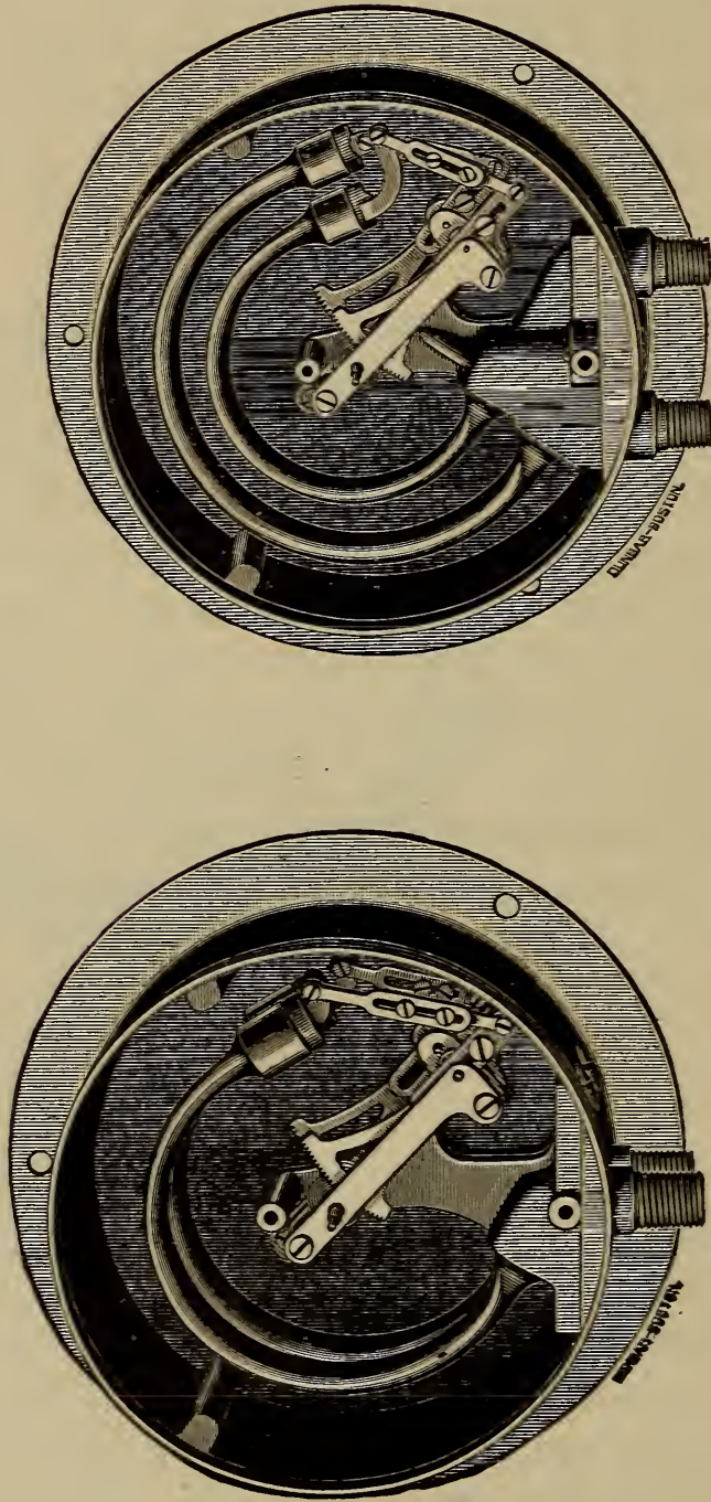
FIGURE 180 CROSBY DUPLEX GAUGE, SECTIONAL VIEW
