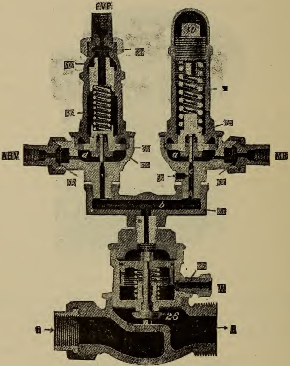
FIG. 321. PUMP GOVERNOR
