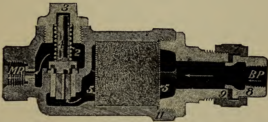
FIG. 322. COMBINED AIR STRAINER AND CHECK VALVE
