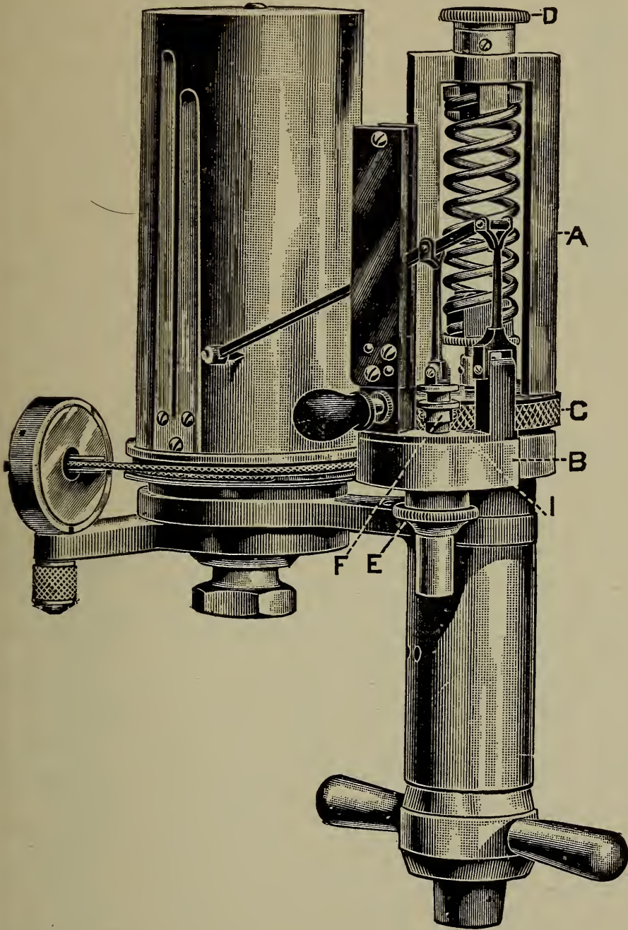
IMPROVED TABOR INDICATOR WITH OUTSIDE CONNECTED SPRING ASHCROFT MFG. CO., N. Y.
