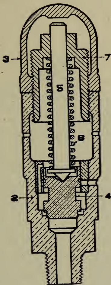
FIG. 309. SAFETY VALVE
