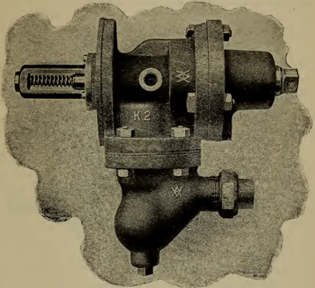
FIG. 323. THE TYPE "K" FREIGHT TRIPLE VALVE
