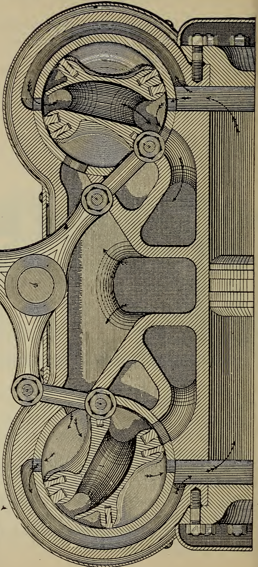
YOUNG VALVES AND GEAR.
