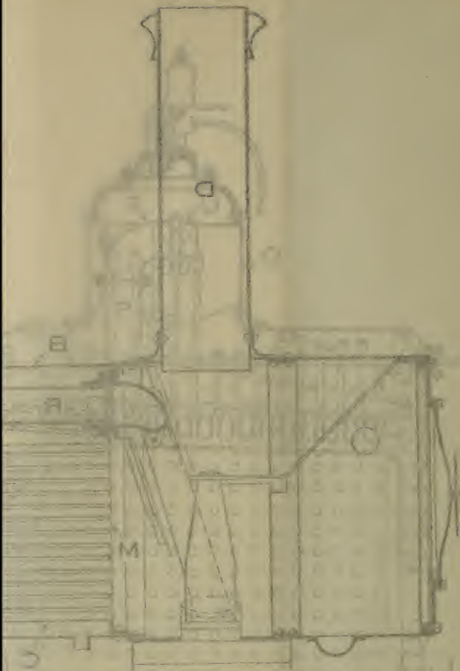
Fig. 6 - Vertical Section
