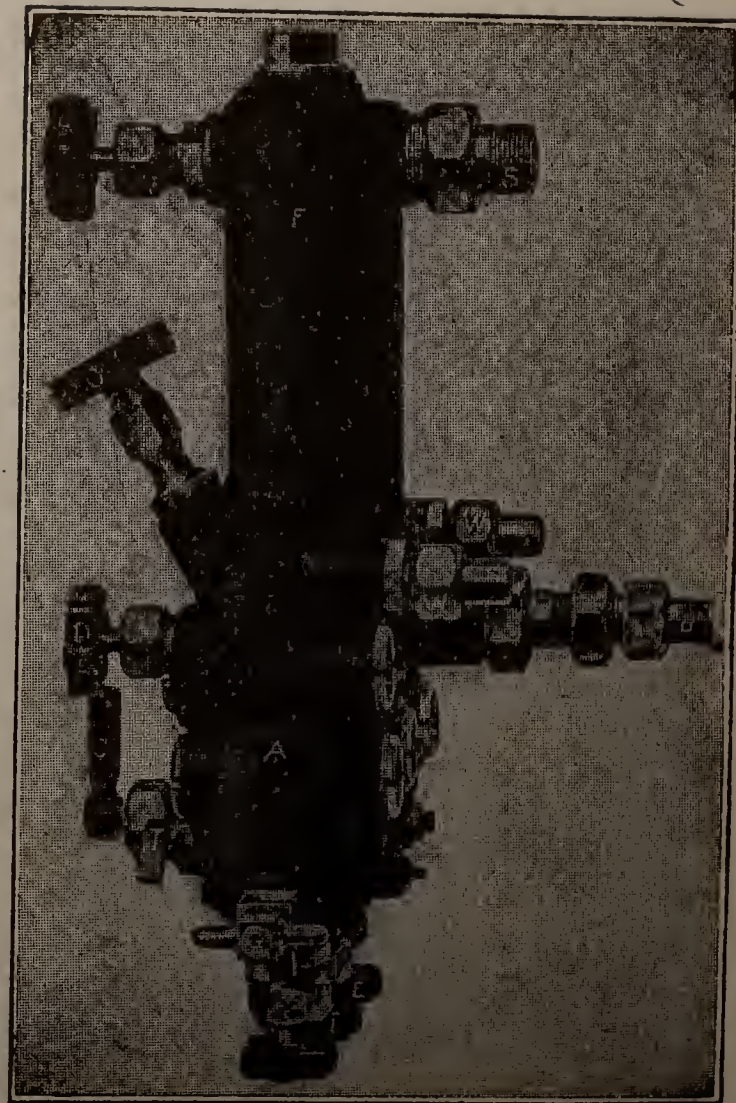
Fig. 203a. Detroit No. 22 Triple Feed Locomotive Lubricator with Automatic Steam Chest Plugs.
