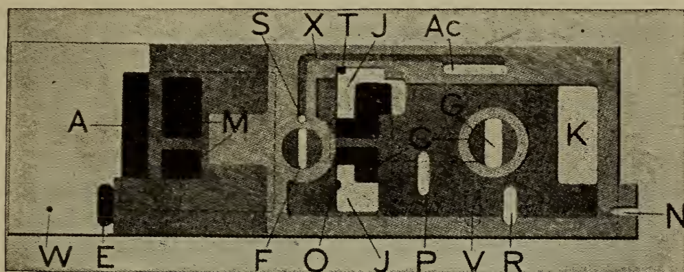
Fig. 272. Release Position.
