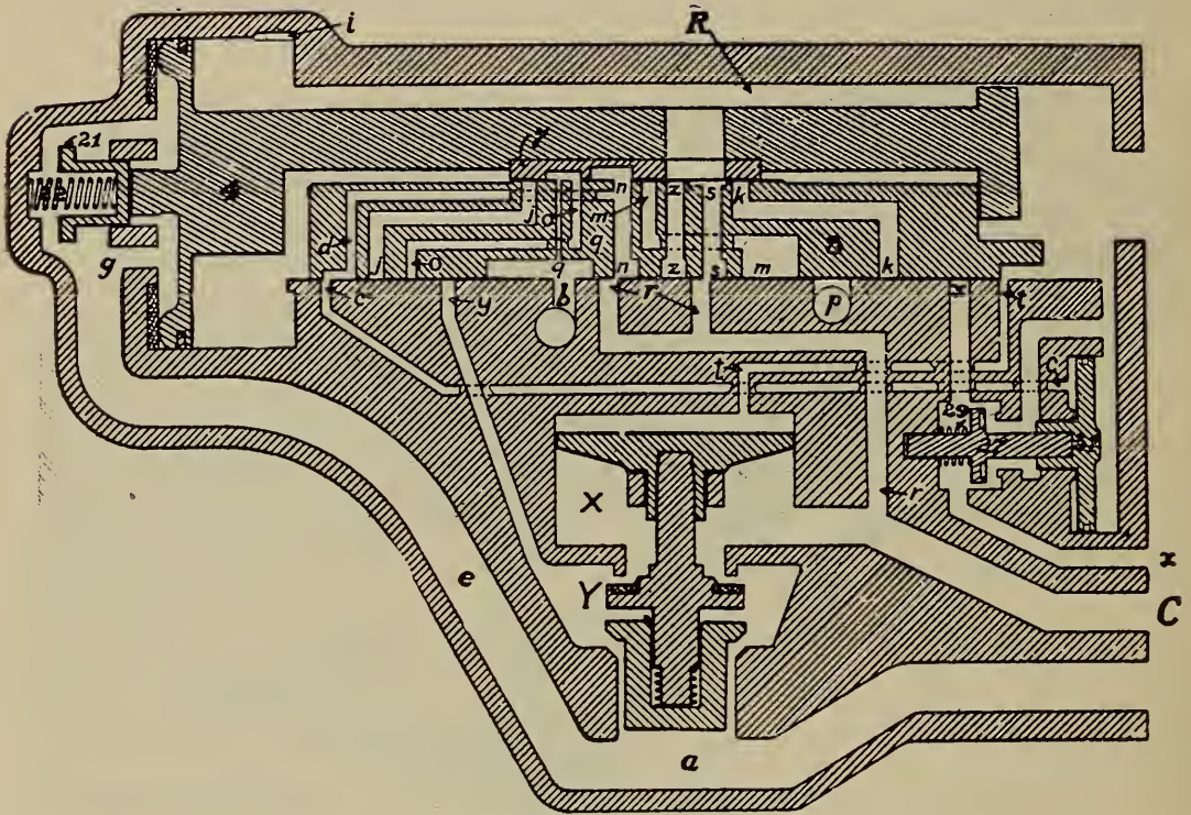
FIG. 356. EMERGENCY POSITION
