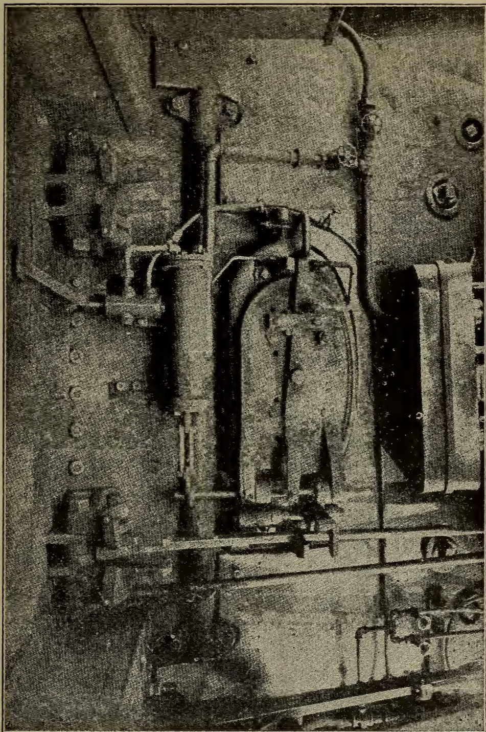
BREWER PNEUMATIC DOOR OPENER, FULL VIEW
