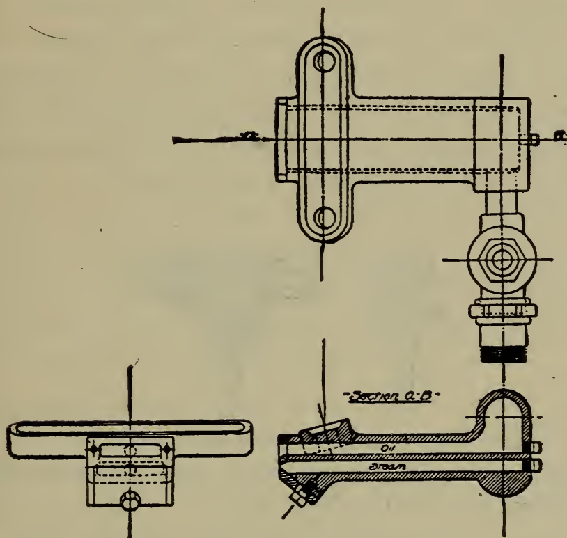
Figure 233g. Baldwin Oil-Burner.
