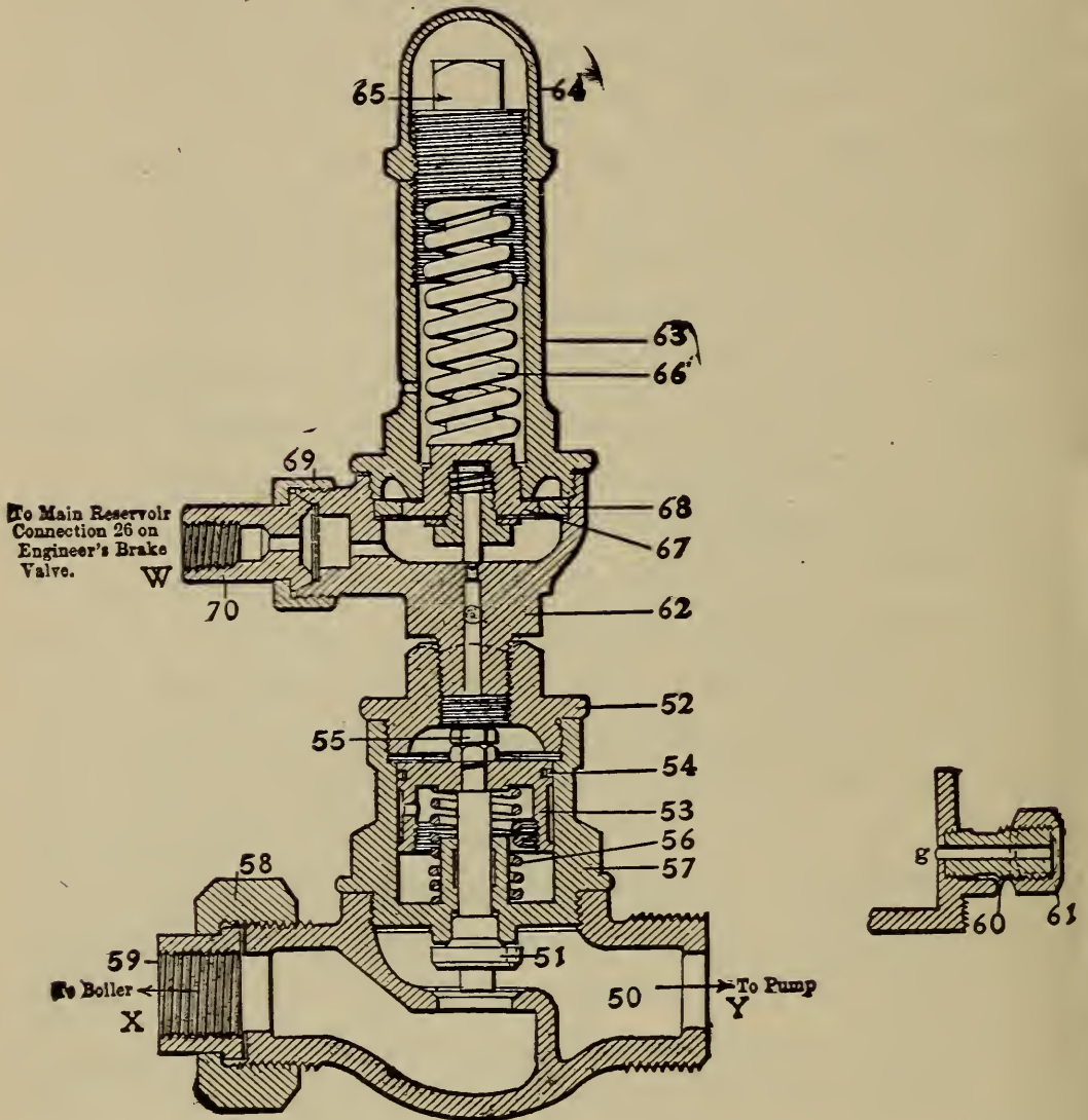
FIGURE 226 PUMP GOVERNOR
