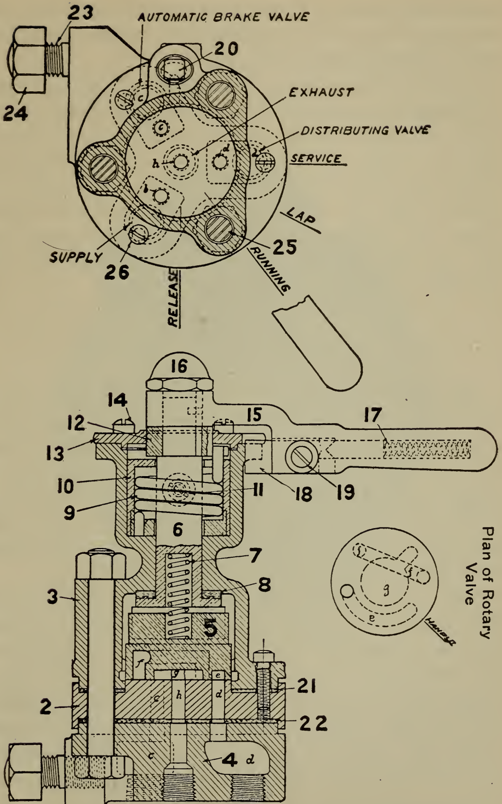
FIG. 316. INTERIOR VIEWS OF THE INDEPENDENT BRAKE VALVE
