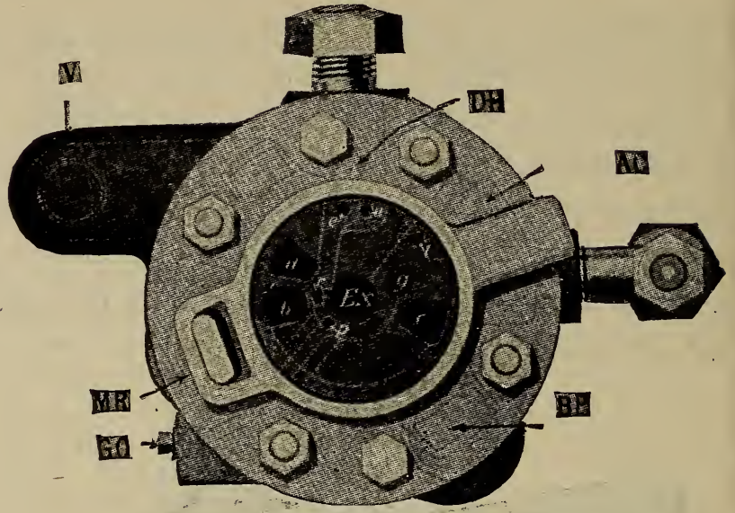
ROTARY-VALVE SEAT.
