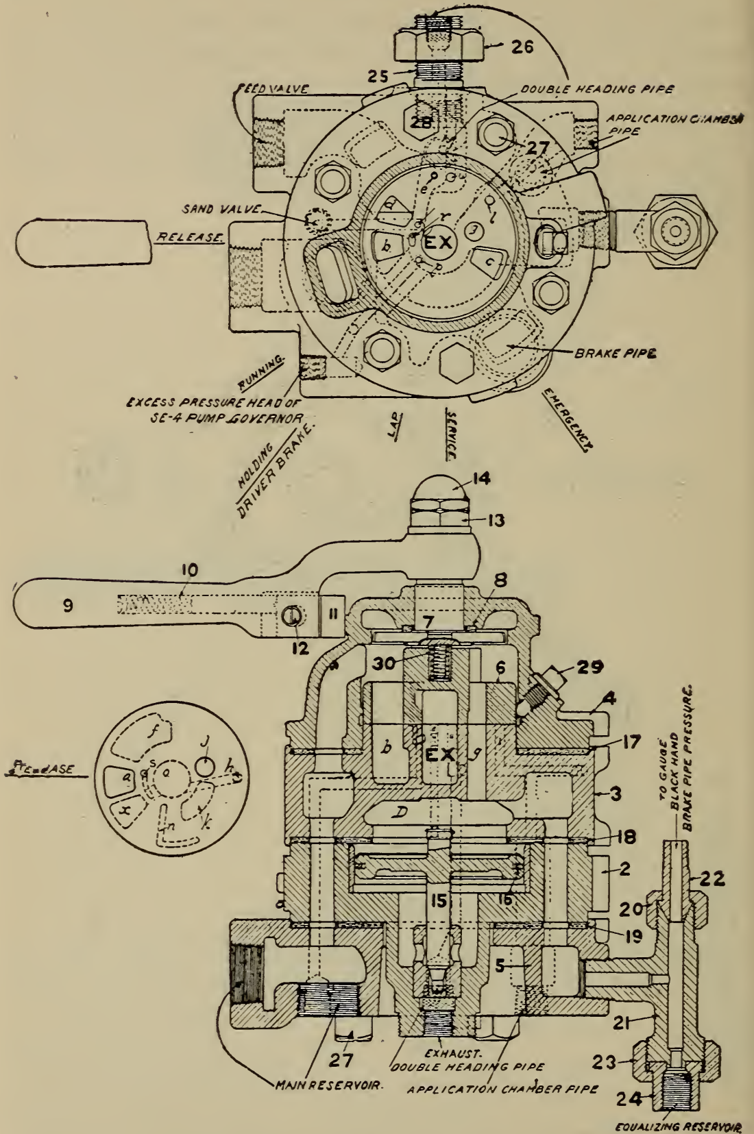
FIG. 313. AUTOMATIC BRAKE VALVE
