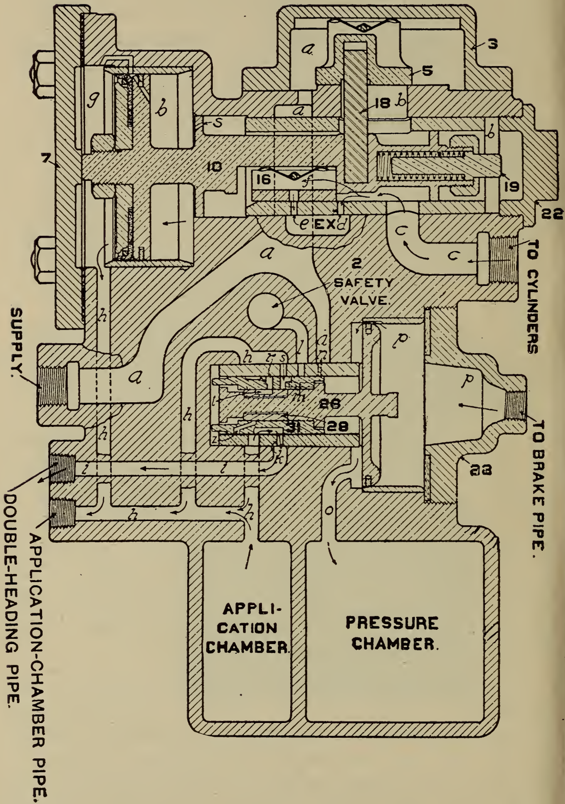
FIG. 299. RELEASE, AUTOMATIC OR INDEPENDENT
