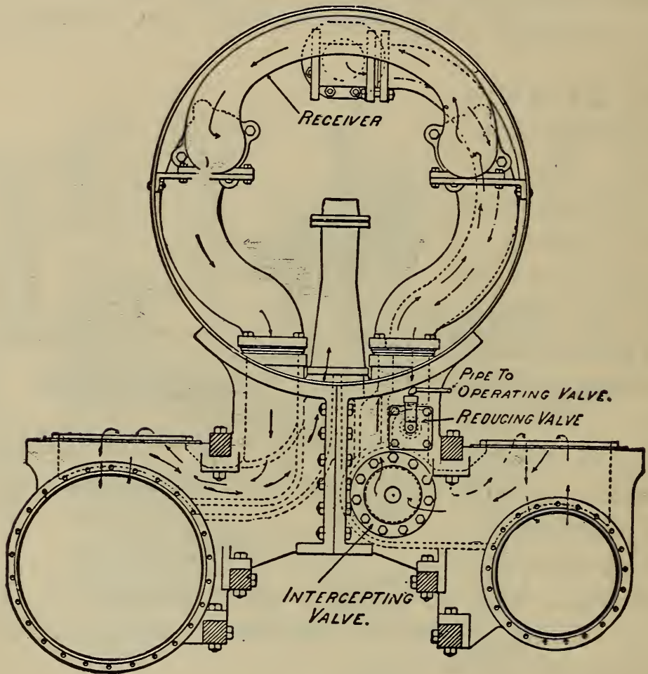
TWO-CYLINDER COMPOUND. CROSS-SECTION
