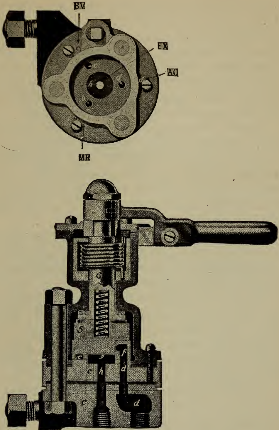
FIG. 315. INTERIOR VIEW OF THE INDEPENDENT BRAKE VALVE
