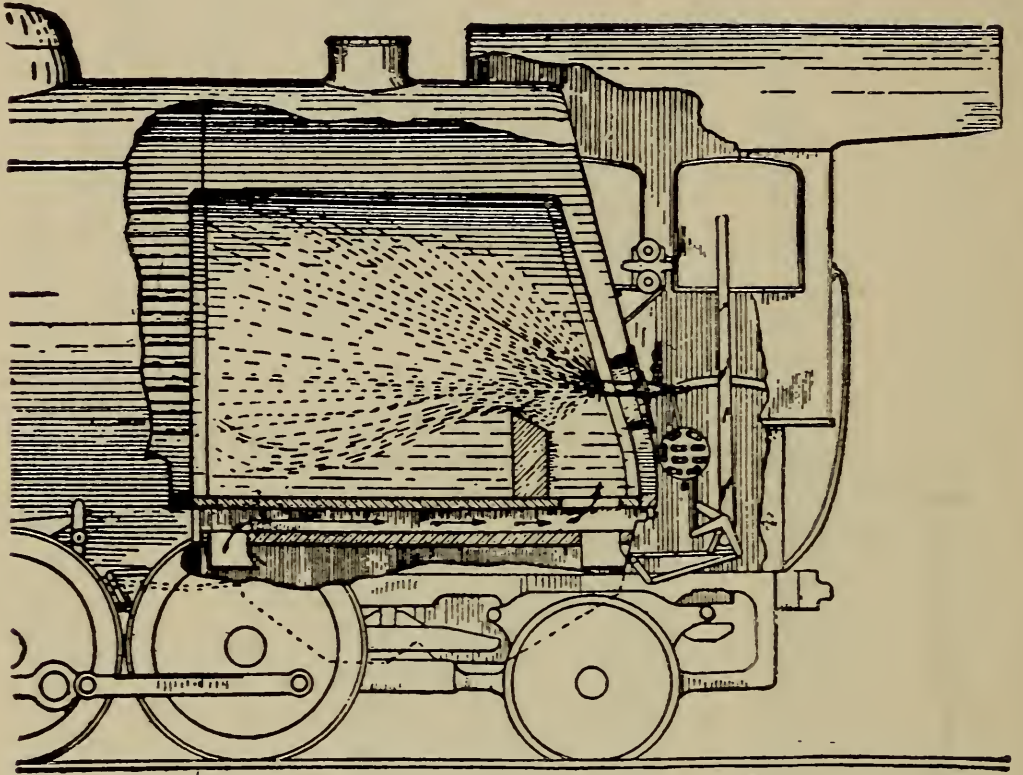
Figure 223k. Lassoë-Lovekin Oil-Burner. Dispenses with Brick Arch. Oil Supplied Under Pressure.
