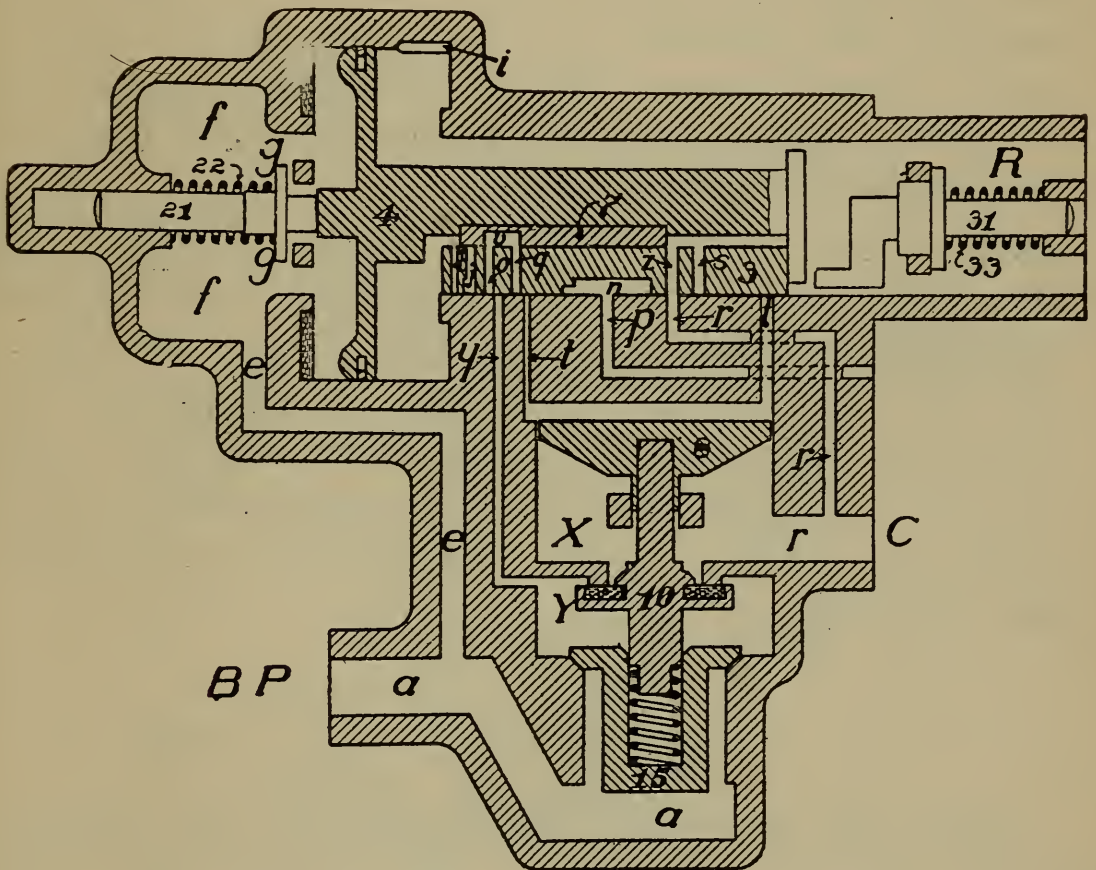
FIG. 328. FULL SERVICE POSITION
