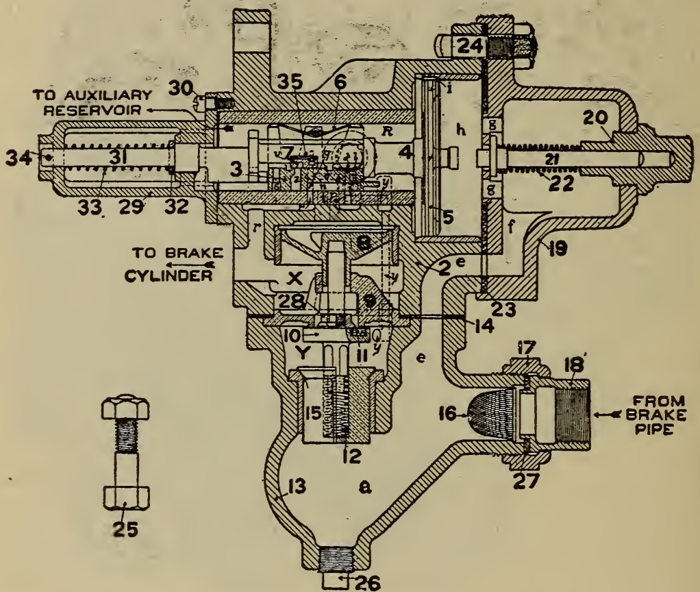
FIG. 324. THE K-2 TRIPLE VALVE
