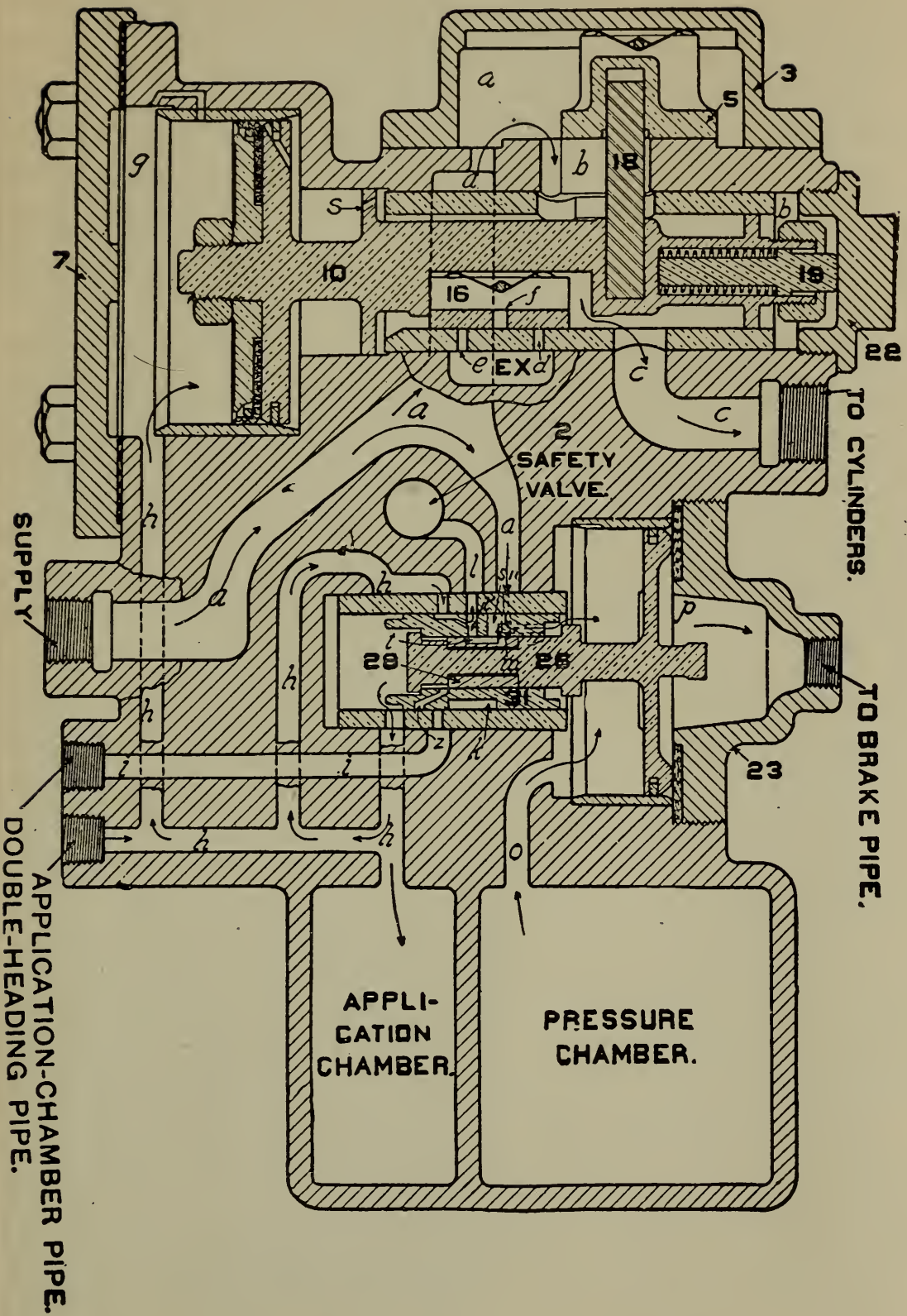
FIG. 304. EMERGENCY
