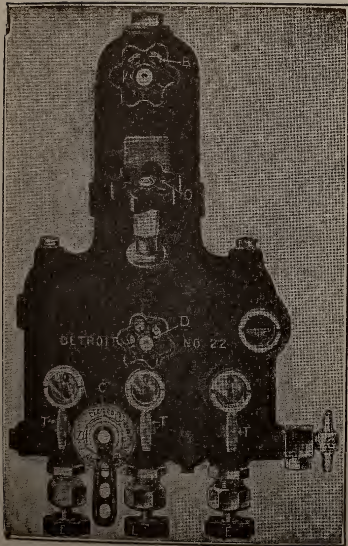
Fig. 203a. Detroit No. 22 Triple Feed Locomotive Lubricator with Automatic Steam Chest Plugs.
