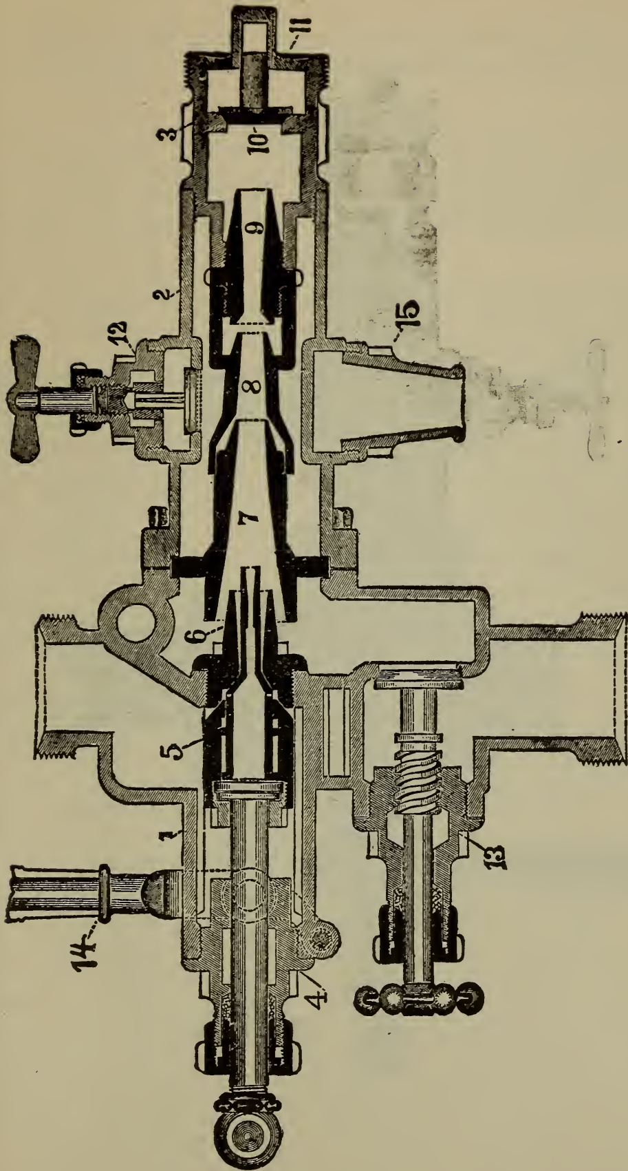
OHIO LOCOMOTIVE INJECTOR. Sectional View.
