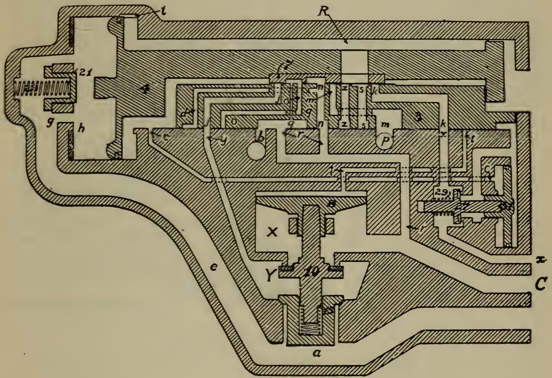
FIG. 355. GRADUATED-RELEASE-LAP POSITION
