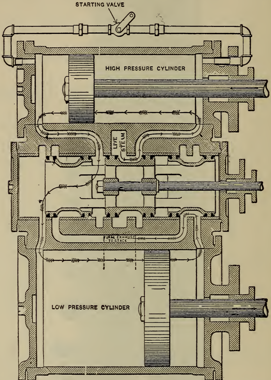
STEAM DISTRIBUTION IN BALANCED COMPOUND CYLINDERS.
