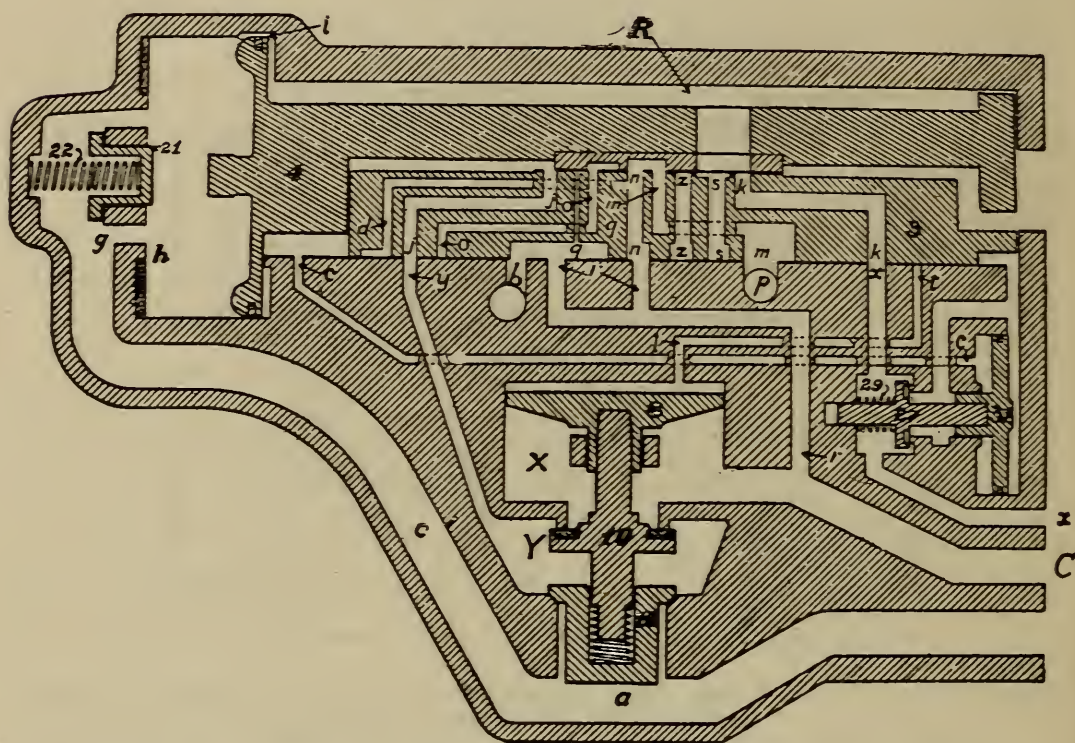
FIG. 351. FULL RELEASE AND CHARGING POSITION
