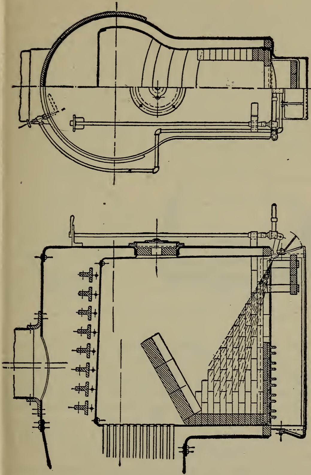
Figure 223 I. Burner and Firebox Arrangement on Baldwin Locomotive.
