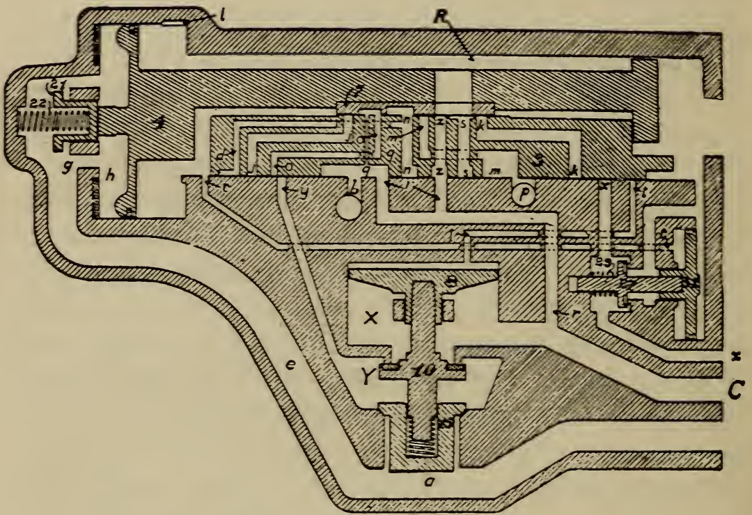
FIG. 353. FULL-SERVICE POSITION
