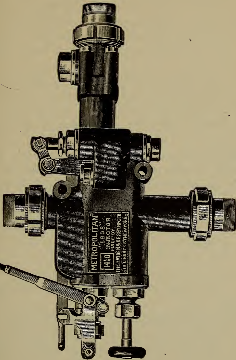
FIGURE 163 METROPOLITAN "1898" LOCOMOTIVE INJECTOR
