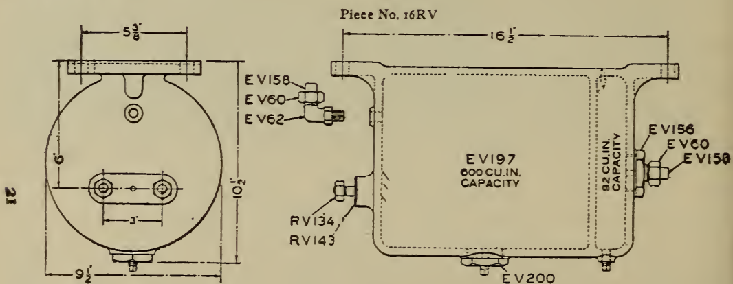
Fig. 279. Divided Reservoir.
