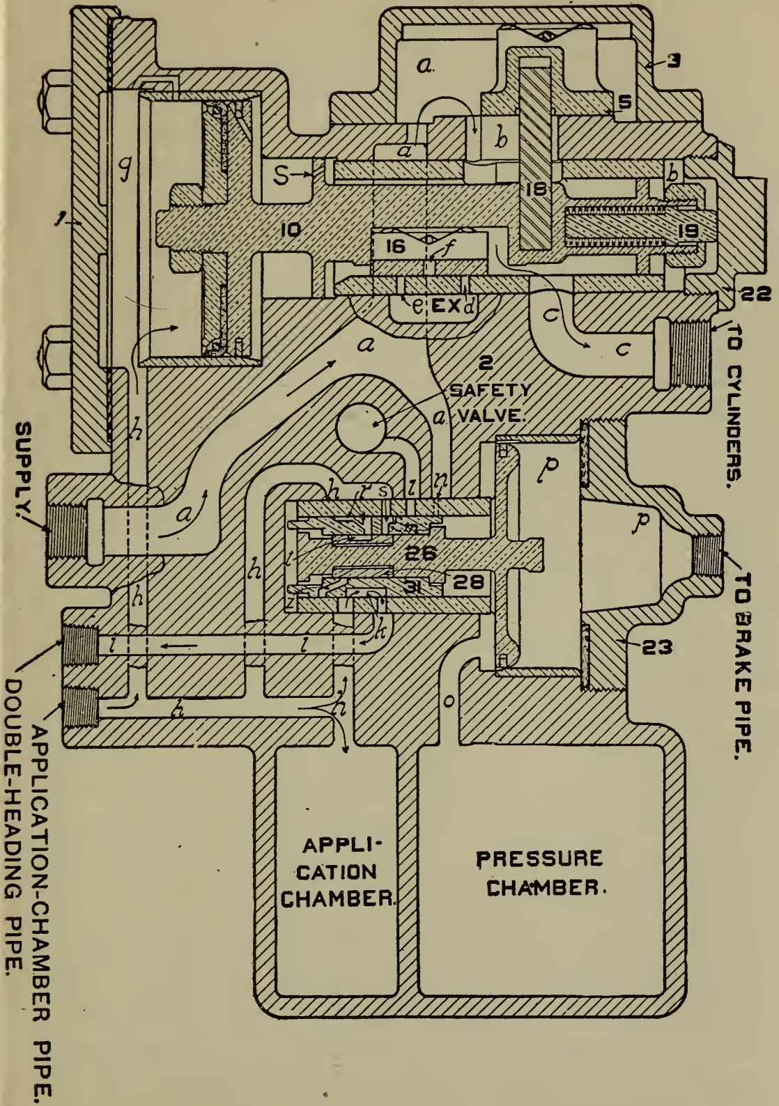
FIG. 300. INDEPENDENT APPLICATION
