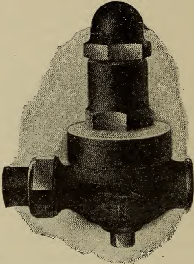
Fig. 289. Straight Air Reducing Valve.
