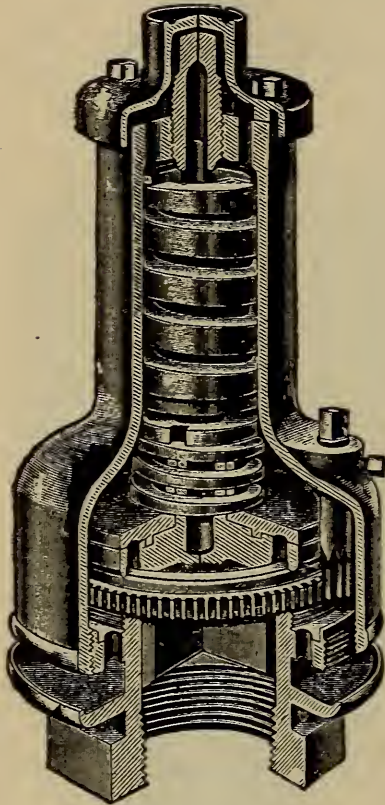
FIGURE 192 CRANE MUFFLED POP VALVE SECTIONAL VIEW
