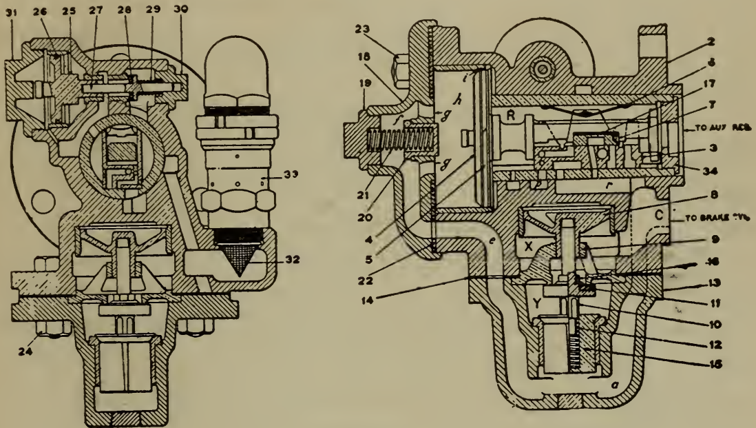
FIG. 349. THE TYPE L TRIPLE VALVE
