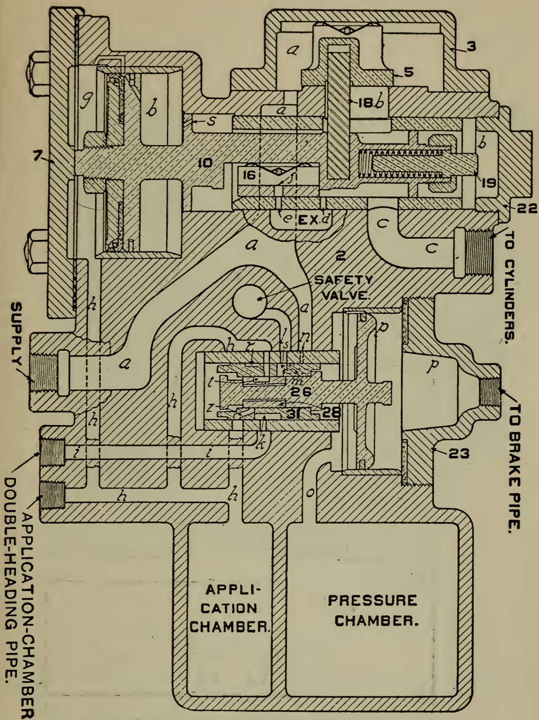
FIG. 306. RELEASE POSITION
