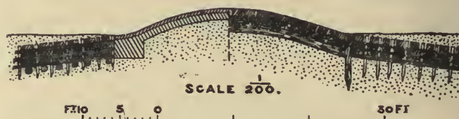
FIG. 10.—Sections of Groynes at Blankenberghe.
