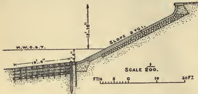
FIG. 8.—Sea Embankment at Ostend.
