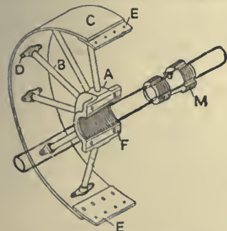
FIG. 1.—Built-up Pulley.
