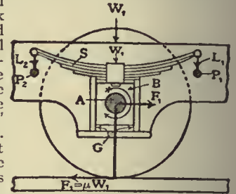
FIG. 16.—Wheel and Connexion to Frame.
