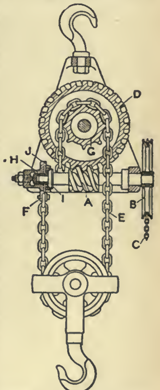
FIG. 8.—Worm-gear Pulley Block with Automatic Brake.
