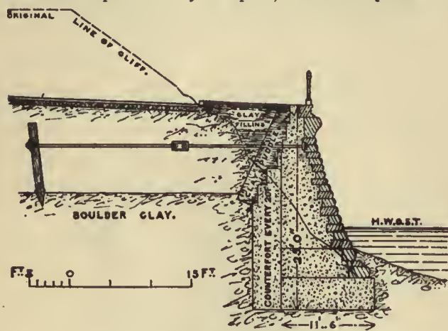
FIG. 7.—Sea-wall at Bridlington.
