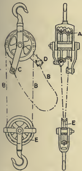
FIG. 6.—Weston Differential Pulley Block.
