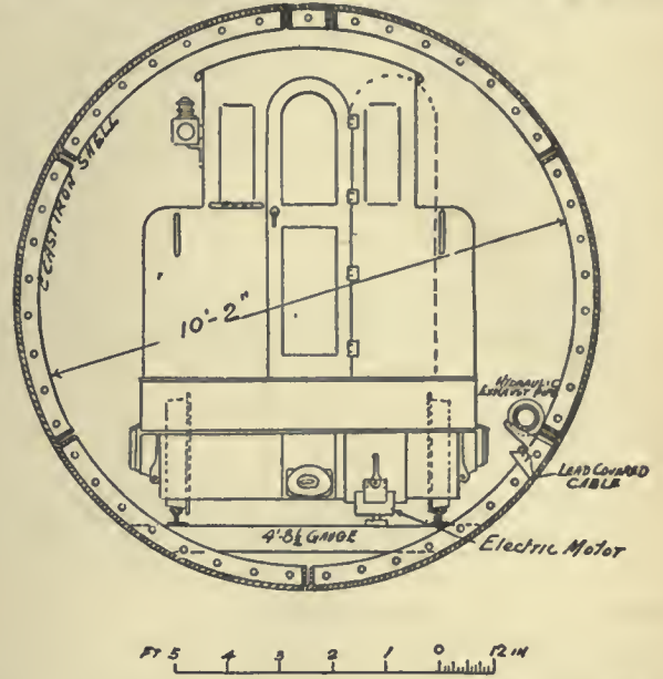
FIG. 33.—Section of Tunnel and Electric Locomotive, City & South London railway.
