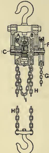
FIG. 7.—Moore and Head Pulley Block.
