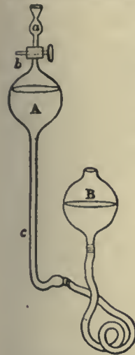
FIG. 3. Geissler's Air-Pump.
