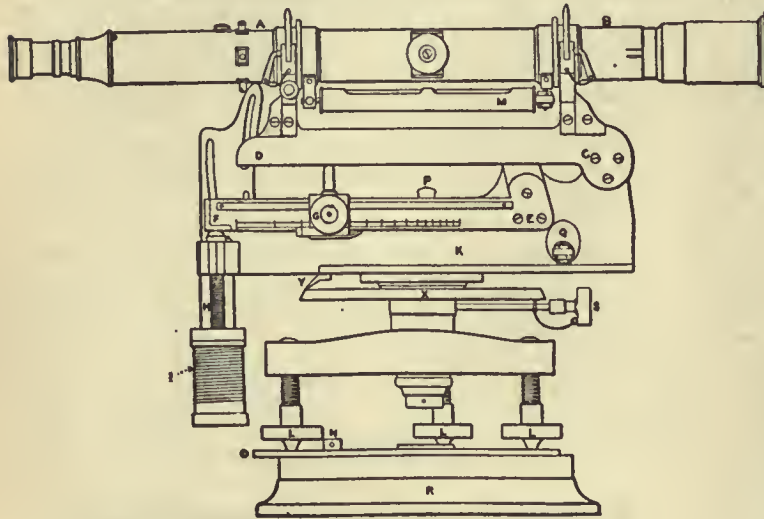
FIG. 6.—Depression Range-Finder.
