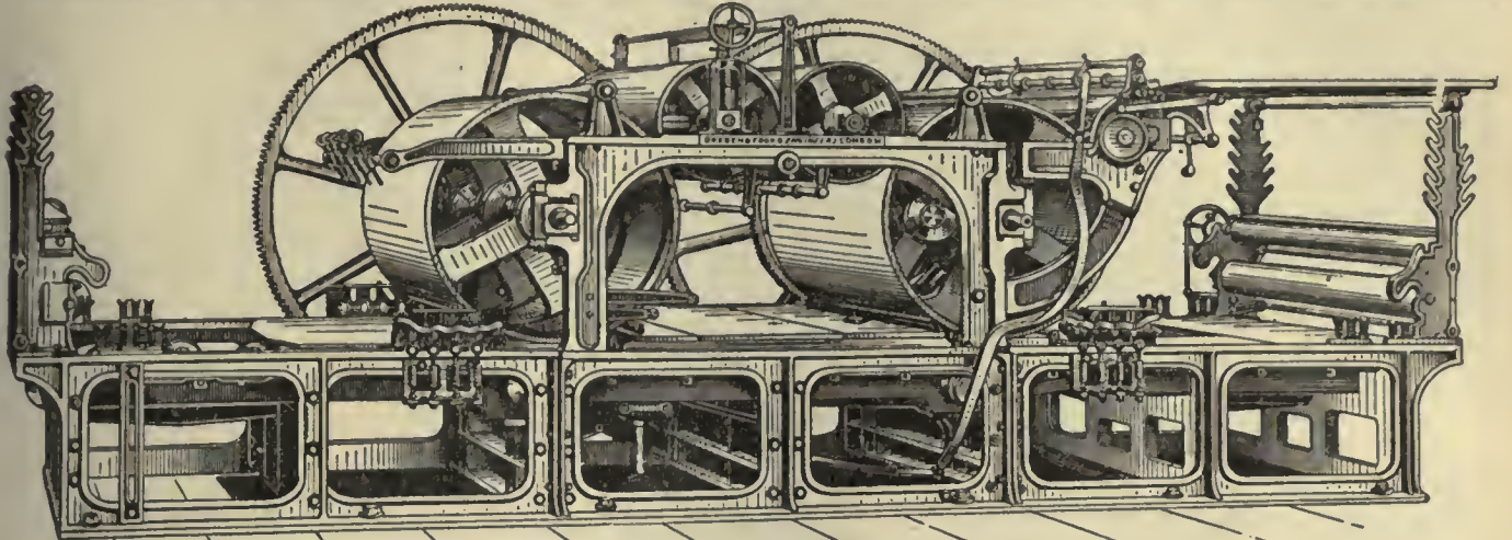
FIG. 6.—Dryden & Foord's Perfecting (two-cylinders) Machine.
