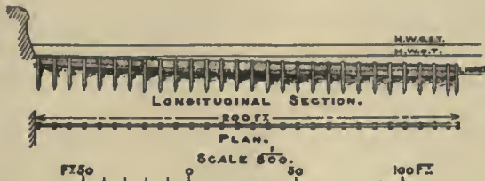
FIG. 11.—Groyne at Bridlington.
