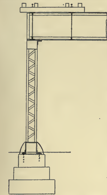
FIG. 32.—Double-Column Elevated Structure (half-section).
