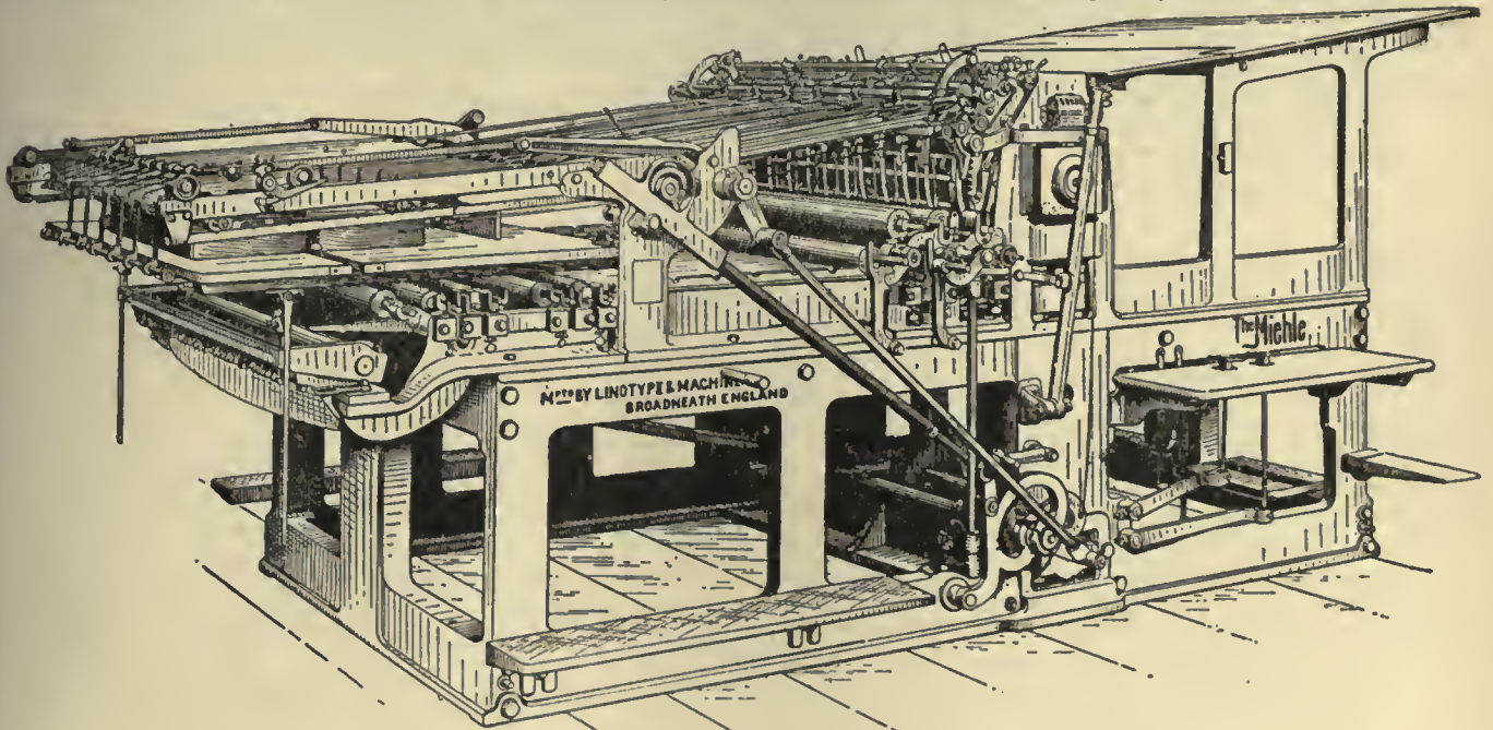
FIG. 7.—The Miehle Two-revolution Cylinder Machine.
