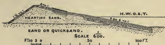
FIG. 2.—Dutch Reclamation Embankment.
