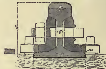
FIG. 12.—French Rail, 90 1/2 lb to the yard, showing rail joint and seat in the sleeper.
