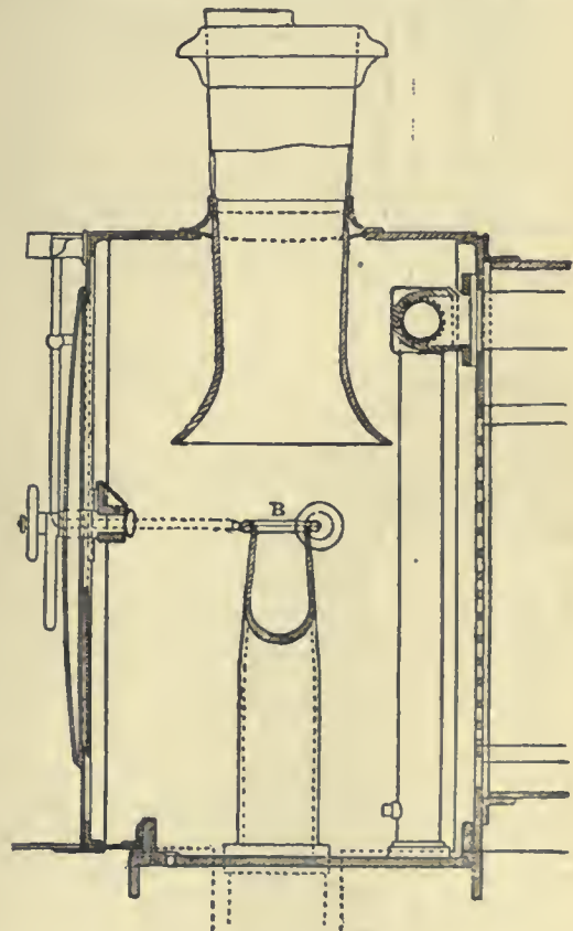
FIG. 18.—Smoke-box, L. & N.W.R. four-coupled 6 ft. 6 in. passenger engine, scale \frac{1}{4} in.
