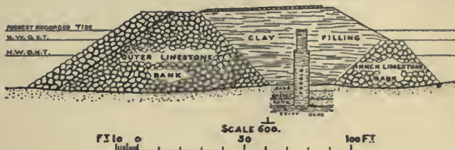
FIG. 3.—Reclamation Bank for the Hodbarrow Iron Mines.
