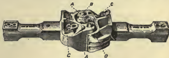
FIG. 28.—Automatic Coupling for Freight Cars (U.S.A.).
