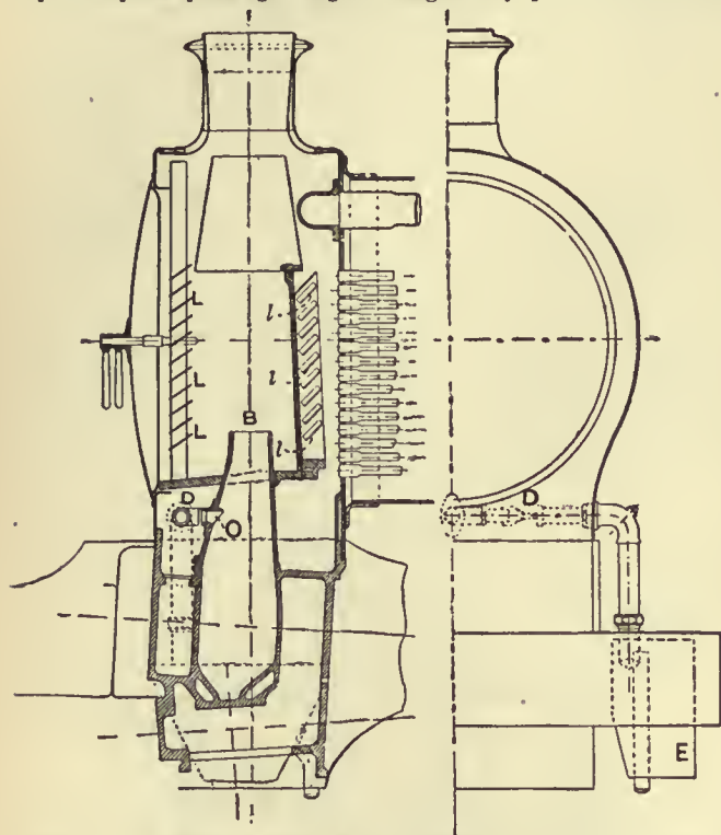
FIG. 19.—Smoke-box and Spark Arrester, G.E.R. four-coupled express engine, scale \frac{3}{4} .
