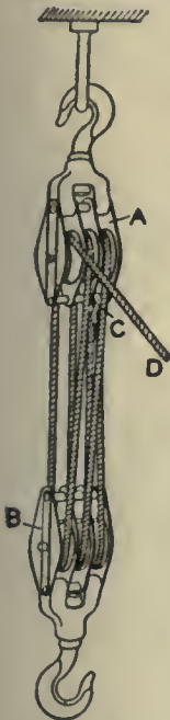
FIG. 5.—Sheave Pulley Block.
