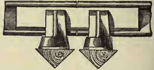
FIG. 7.—The original Fish-Joint of W. Bridges Adams.
