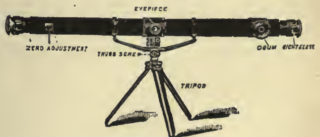
Instrument ready for use. FIG. 4.—Marindin Range-Finder.
