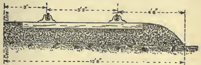
FIG. 8.—Half of English Double Track.
