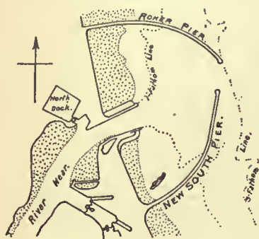
SCALE 50,000. FIG. 6.—Sunderland Harbour.
