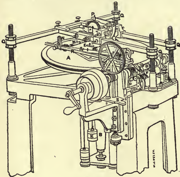
Dividing Engine.
