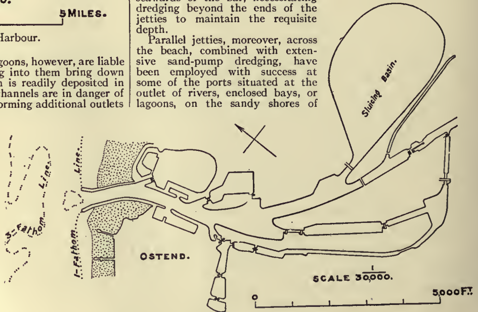
FIG. 2.—Ostend Harbour and Jetty Channel.
