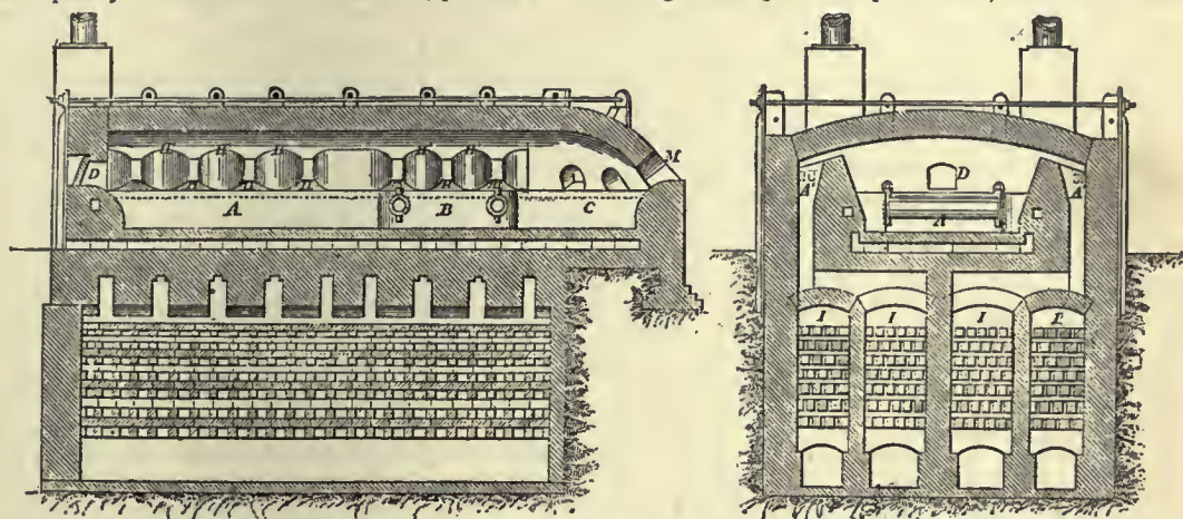
FIG. 15.—Siemens's Continuous Tank Furnace.
