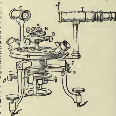
FIG. 3.—Horizontal-Circle Goniometer.
