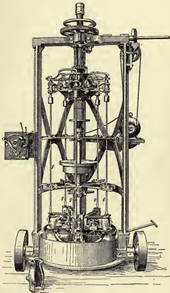
FIG. 19.—Owens's Glass-blowing Machine. g, g, g, Blowing-irons.
