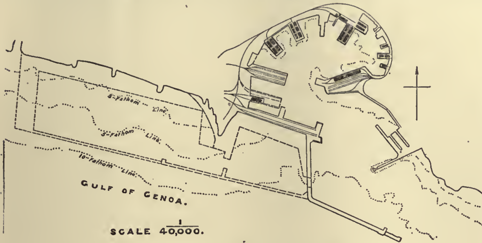
FIG. 3.—Genoa Harbour and Extensions.
