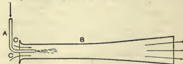
FIG. 9.—Steam-jet Blower.
