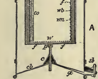
FIG. 19.—Diagram of the Raynor Extractor.
