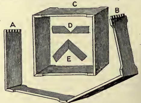
FIG. 10.—"1-lb section" wooden box for holding Comb-honey. (Redrawn from the A B C of Bee-Culture , published by the A. I. Root Co., Medina, Ohio, U. S. A.)
