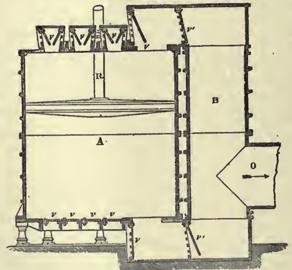
FIG. 3.—Section of Cylinder of Early Blowing Engine (1851).
