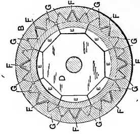
FIG. 9.—Cross-section.
