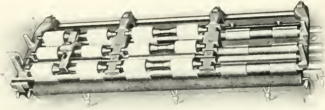
TOP AND BOTTOM ROLLS, CAP BAR AND TRUMPET ROD High-Draft Arrangement
