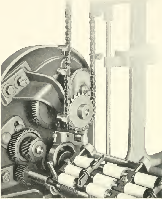
ATTACHMENT FOR SLUB YARN AND HIMALAYA YARN
