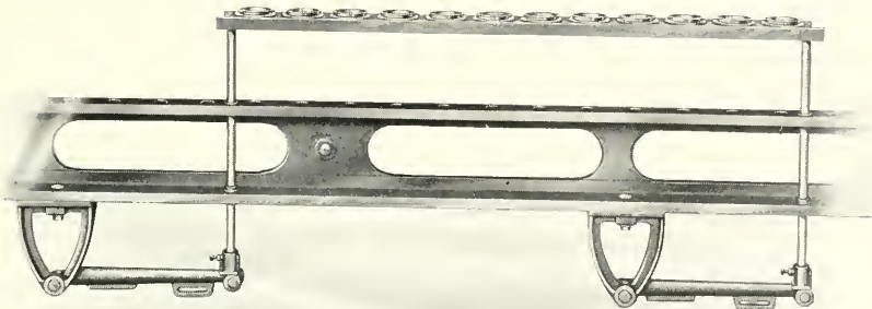
RING RAIL Showing Supports and Rocker Arms
