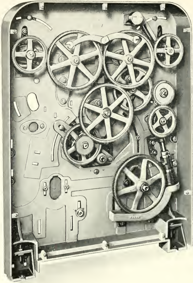
GEARING Showing Builder-Motion Drive
