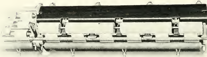
SECTION OF ROLLS SHOWING TOP CLEARERS High-Draft Arrangement
