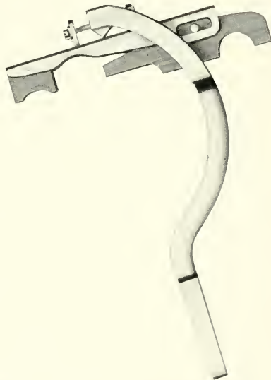
COMBINED OILLESS WOOD BEARING SADDLE AND STIRRUP
