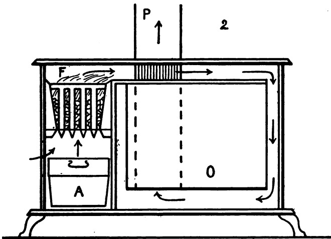
Diagram of a section of range, showing direction of hot-air currents when damper is open, as in No. 1; when closed, as in No. 2.
