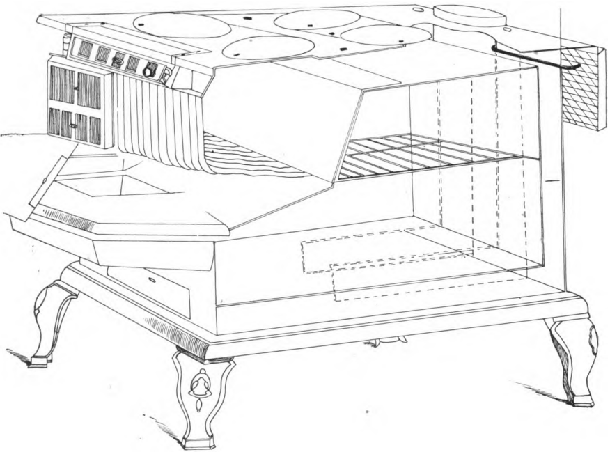
Inner Construction of Range.
