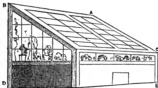
Fig. 1.—SMALL GREENHOUSE WITHOUT HEATING APPARATUS. (A B, hinged cross-beam; C, movable sash; D E, uprights.)
