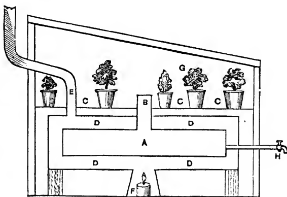
Fig. 2.—SMALL GREENHOUSE WITH HEATING APPARATUS.
