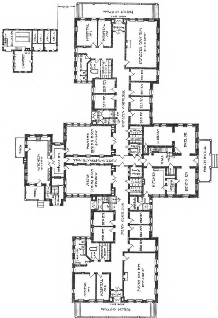
FIRST FLOOR PLAN, ADAMS COUNTY POOR ASYLUM, DECATUR, INDIANA
