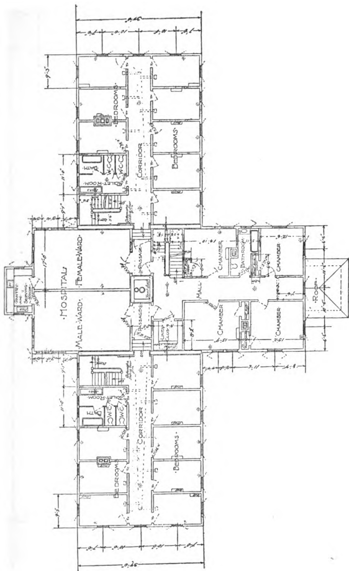
ALMSHOUSE, NEWTON, MASSACHUSETTS. SECOND FLOOR PLAN
