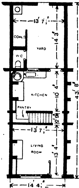
Fig. 117.—Ground Plan of 14-ft. 4\frac{1}{2} -in. House.
