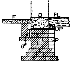
Fig. 38.—Damp-proof Course when Floor is Level with Ground.
