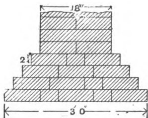
Fig. 28.—Footings for 18-in. Wall.
