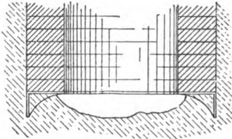
Fig. 34.—Brick Pillar on Cutting Ring.
