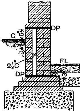
Fig. 39.—Damp-proof Course when Floor is below Ground Level.
