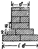
Fig. 26.—Footings for 9-in. Wall.
