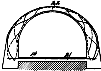
Fig. 190.—Luten patent.
