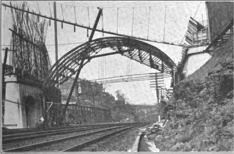
Courtesy of Mr. N. S. Sprague, Superintendent, Dep't. of Public Works, Pittsburgh. FIG. 206.—Steel centers—Atherton Avenue bridge, Pittsburgh.
