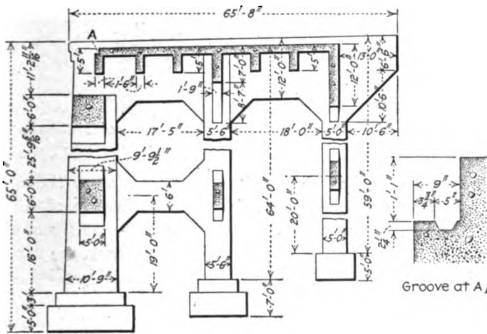
FIG. 309.—Details of abutments of the Judith River viaduct in Montana, C. M. & St. P. Ry.
