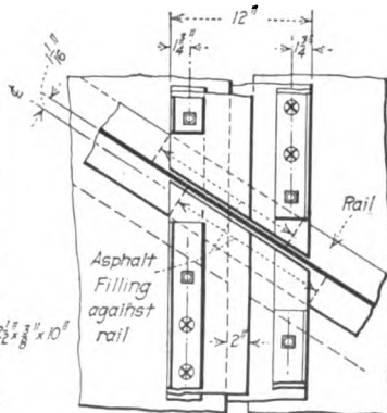
Plan of Expansion Joint in Roadway
