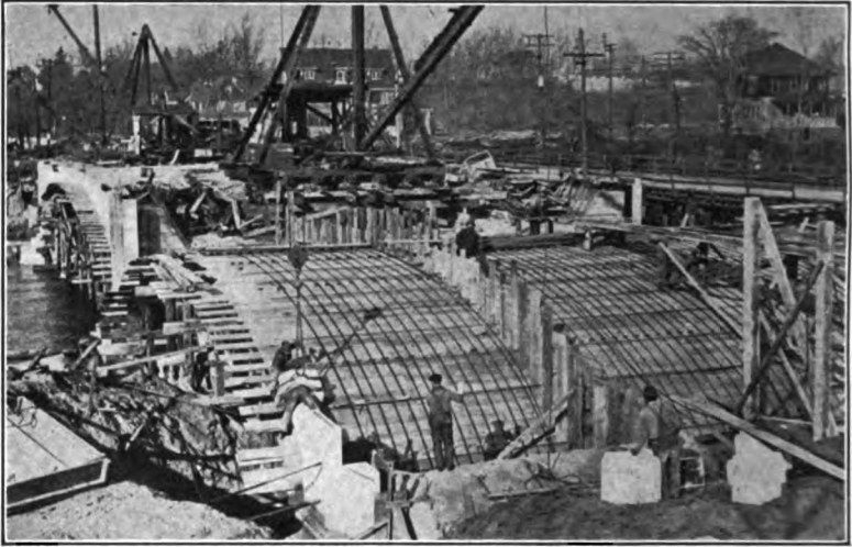
Courtesy of Mr. Charles W. Cole, City Engineer, Mishawaka, Ind. FIG. 87. —Construction view of North Michigan Street bridge, South Bend, Indiana.
