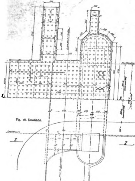
15. Plan of foundation. 16. Top plan.
