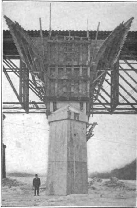
Courtesy of Mr. E. Chamberlain, Ass't. Eng'r., P. & R. Ry. FIG. 420.—Yardley bridge. End view of umbrella forms.
