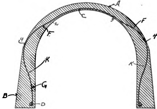
Fig. 189.—Luten patent.
