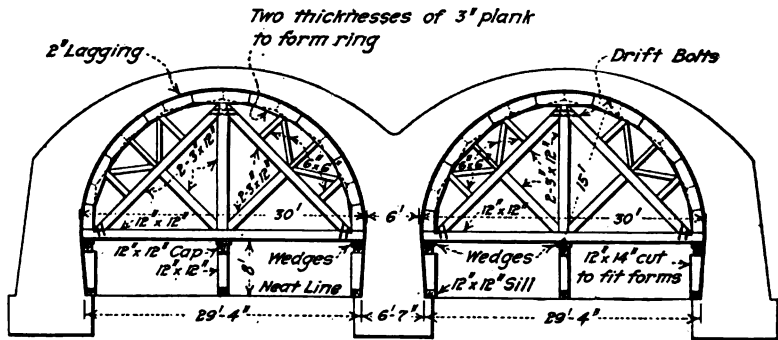
FIG. 333.—Details of centering, Canoe Creek culvert, near Cloe, Pa., B. R. & P. Ry.
