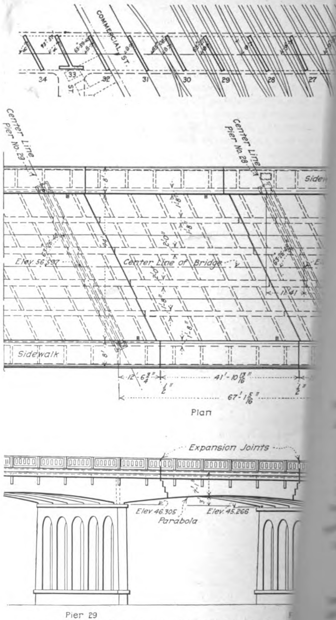
FIG. 360.—Details of Portland bridge, Cumberland
