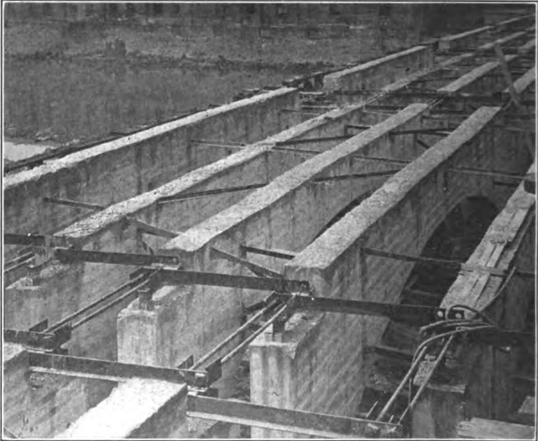
FIG. 137.—Bridge at Central Avenue, Rochester, N. Y. under construction.
