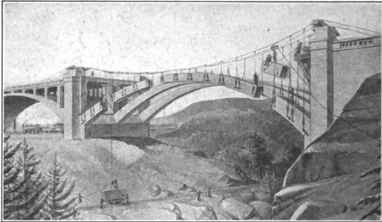
FIG. 109.—Pre-cast voussoir method of arch construction.
