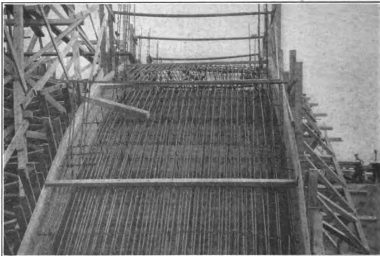
Courtesy of Mr. Daniel B. Luten, Consulting Engineer, Indianapolis. FIG. 96.—Bridge over Saskatchewan River at Saskatoon, Canada. Arch rib ready for concreting.
