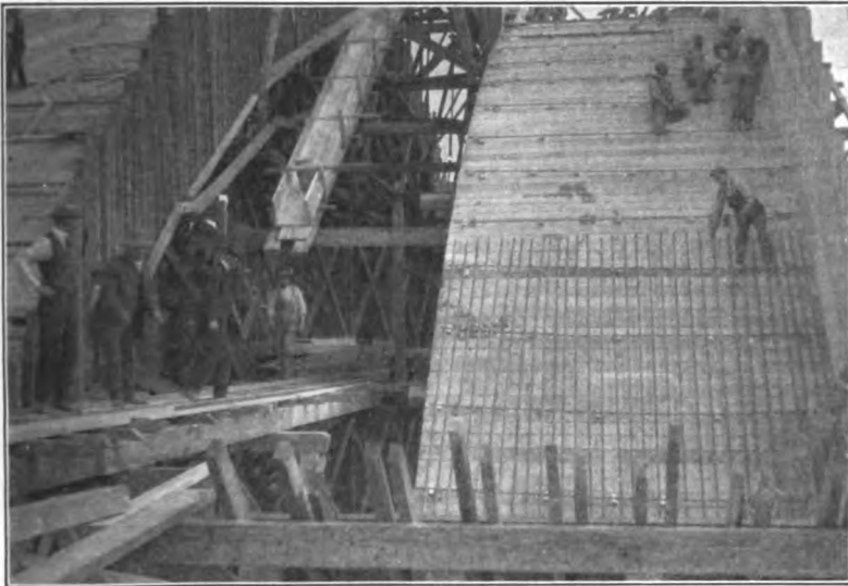
Courtesy of Mr. Daniel B. Luten, Consulting Engineer, Indianapolis. FIG. 94.—Bridge over Saskatchewan River at Saskatoon, Canada. Placing reinforcement in arch ribs.
