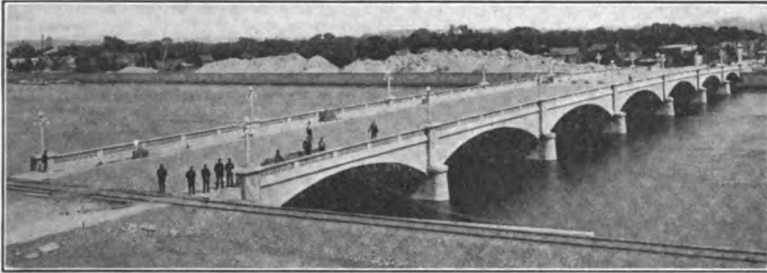
FIG. 366.—Arch bridge with beautiful lines and handsome railing and lamp posts, all of concrete.
