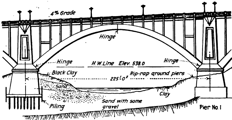
Pier No. 2 FIG. 239.—River span, Main Street viaduct, Fort Worth, Texas.
