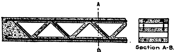
FIG. 486A.—Visintini system.
