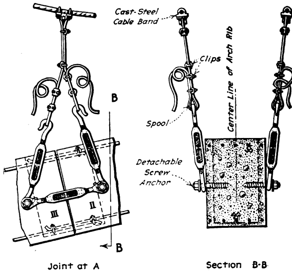
FIG. 133.—Pre-casted voussoir method of arch erection.
