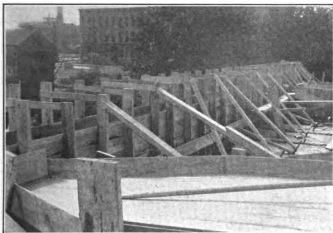
FIG. 152.—Spandrel-wall forms.
