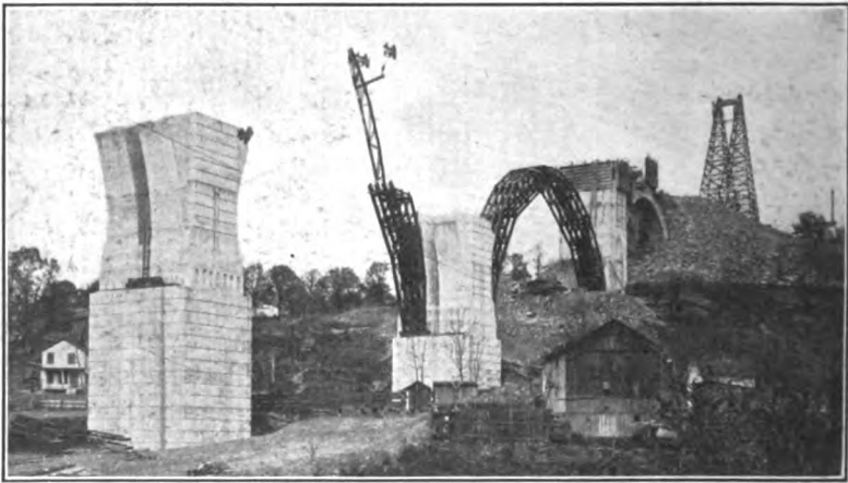
FIG. 440.—Tunkhannock viaduct. Erecting segment of arch centering by means of double cableway. Centers for one rib in adjacent span erected.
