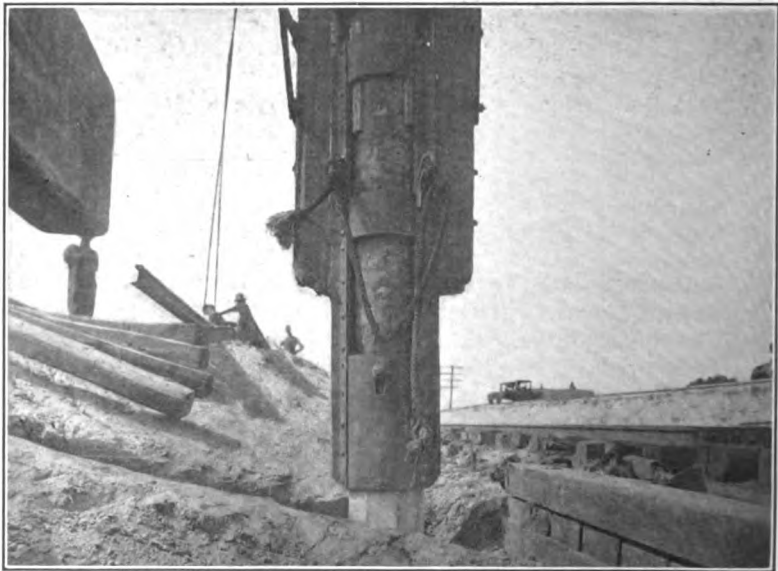
Courtesy of Mr. Maro Johnson, Engineer of Bridges and Buildings, I. C. R. R. FIG. 453.—Pile trestle. Near view of wood cushion in metal guides fastened to driver leads to prevent breaking of pile heads.
