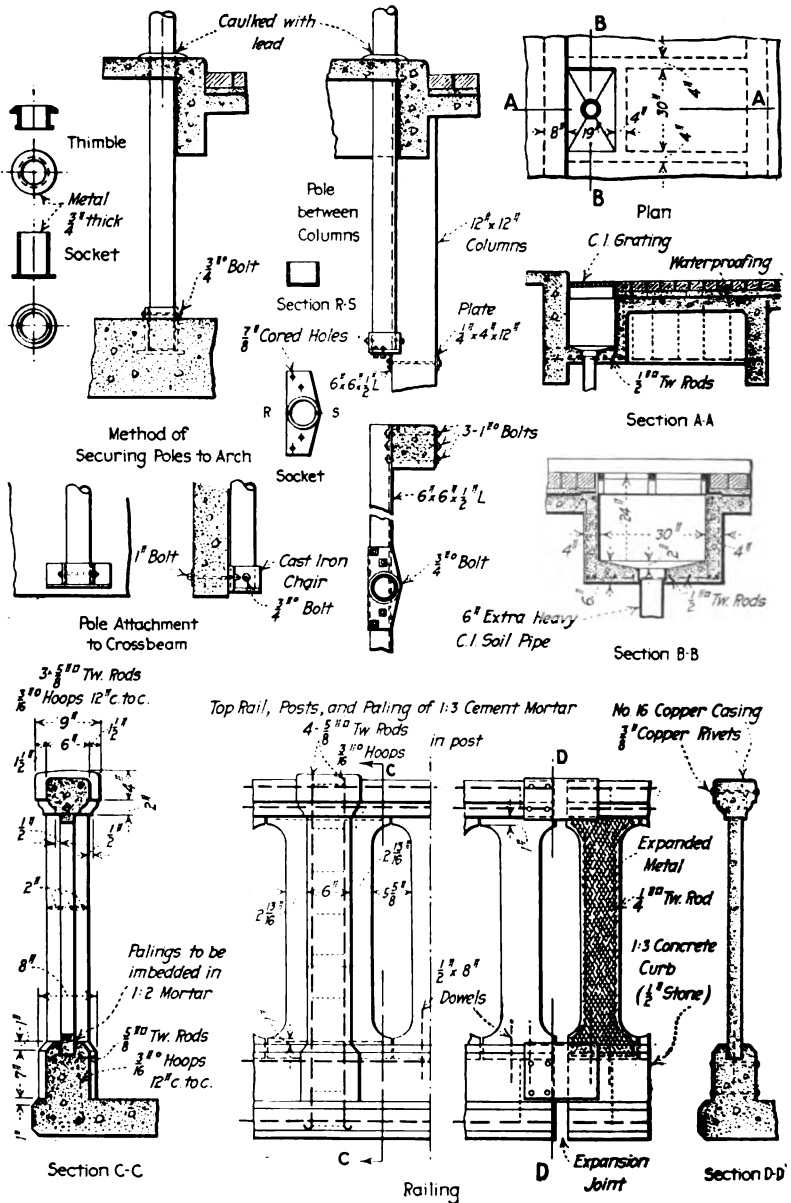
Ludlow Avenue viaduct, Cincinnati, Ohio.
