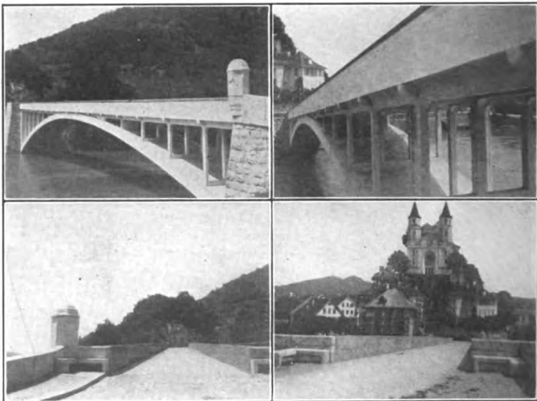
FIG. 550.—Aare River bridge at Aarburg, Switzerland. (Note terminal pedestal seats.)
