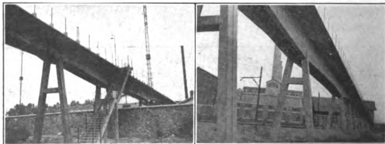
FIG. 532.—Reinforced-concrete trestle, electric plant, Paris.
