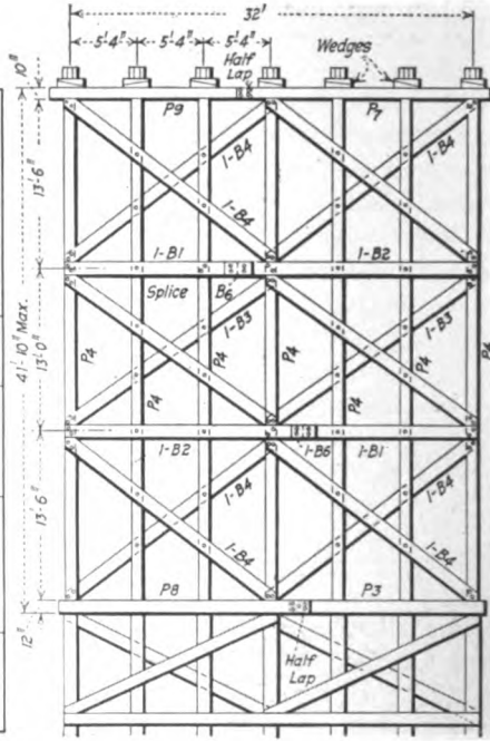
Transverse Elevation of Tower below Trusses
