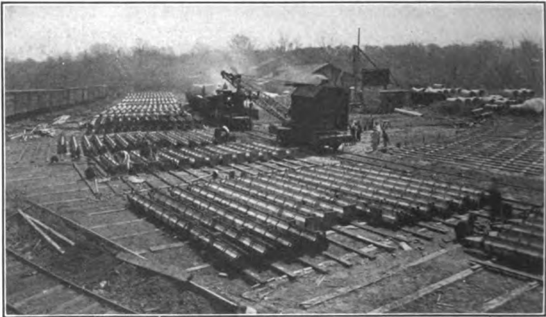
FIG. 450.—Pile trestle. Pouring concrete piles. Various stages of the work are shown.
