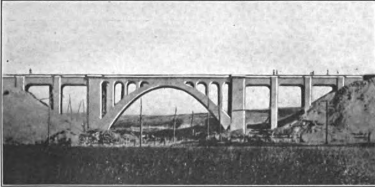
FIG. 376.—Arch awkwardly combined with girder approaches. Lack of harmony, and also lack of symmetry, with no good reason. No apparent attempt to distinguish between two types of structural members.
