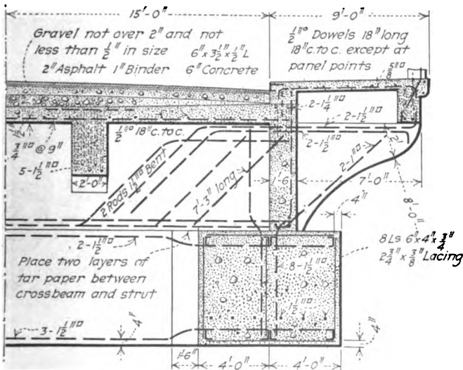
Section near Crown
