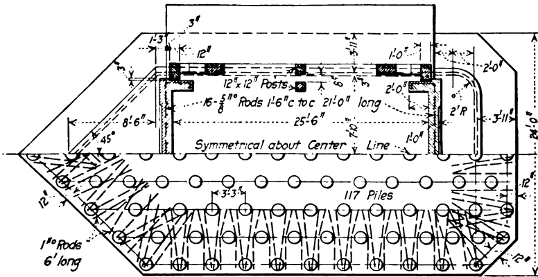
Chippewa River bridge, Eau Claire, Wis.
