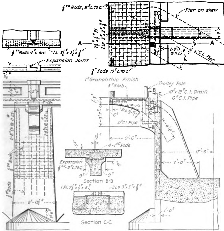
Side Elevation Section A-A FIG. 63.—Counterforted spandrel wall, highway bridge at Ansonia, Conn.
