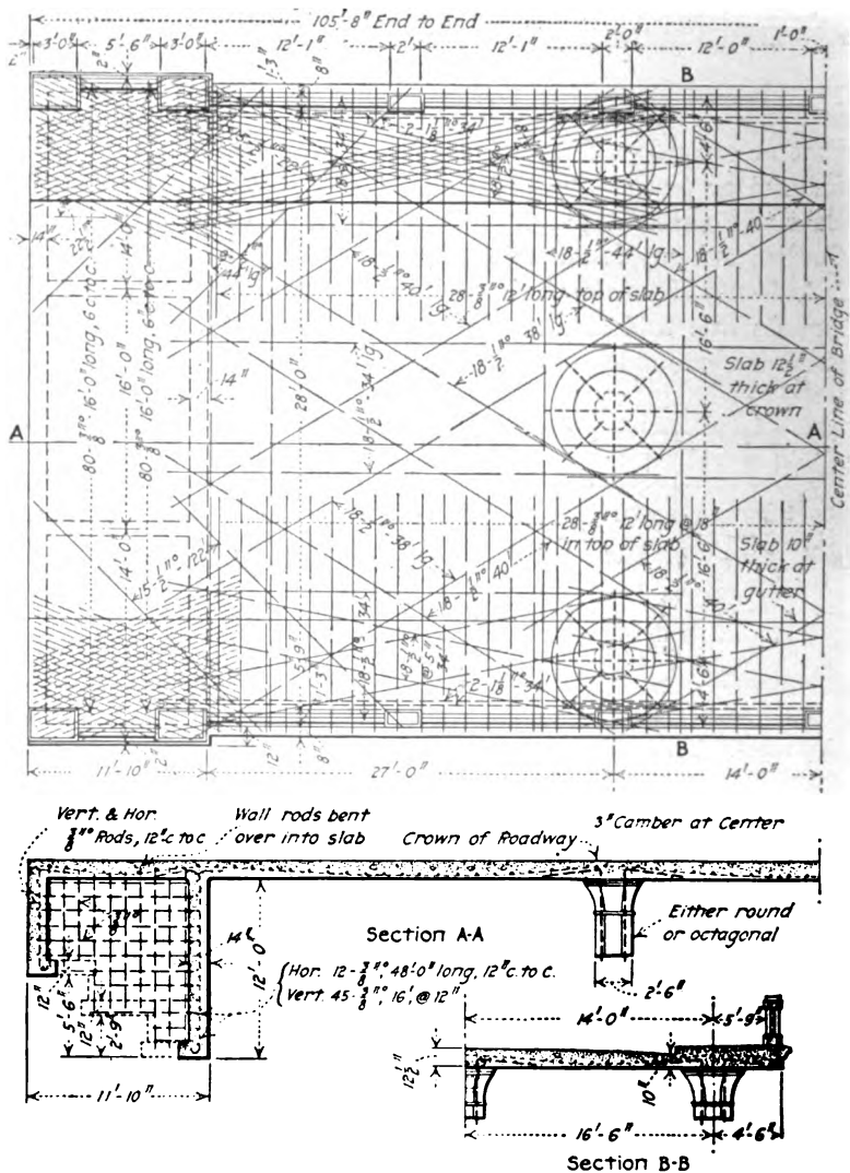
FIG. 266.—Cantilever flat-slab bridge on Mississippi River Boulevard, St. Paul, Minn.
