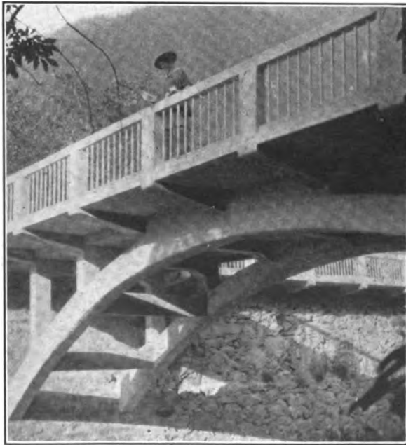
FIG. 539.—Plessur bridge at Chur, Switzerland.
