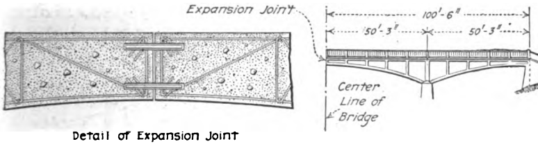
FIG. 298.—Half-elevation and detail of expansion joint of arch-shaped cantilever bridge over Rouge River, Wayne County, Mich.
