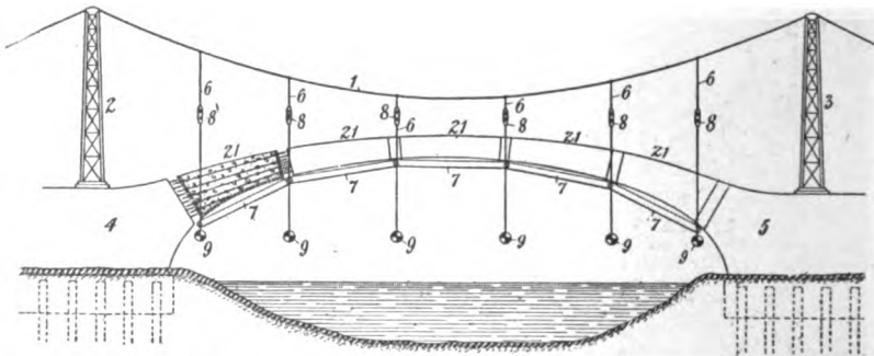
FIG. 197.—Aylett Patent.
