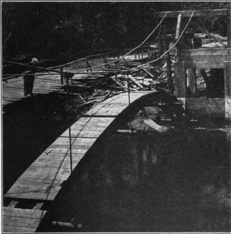
FIG. 108.—Construction view of Chickahominy River bridge near Richmond, Va. Suspended centering in place.
