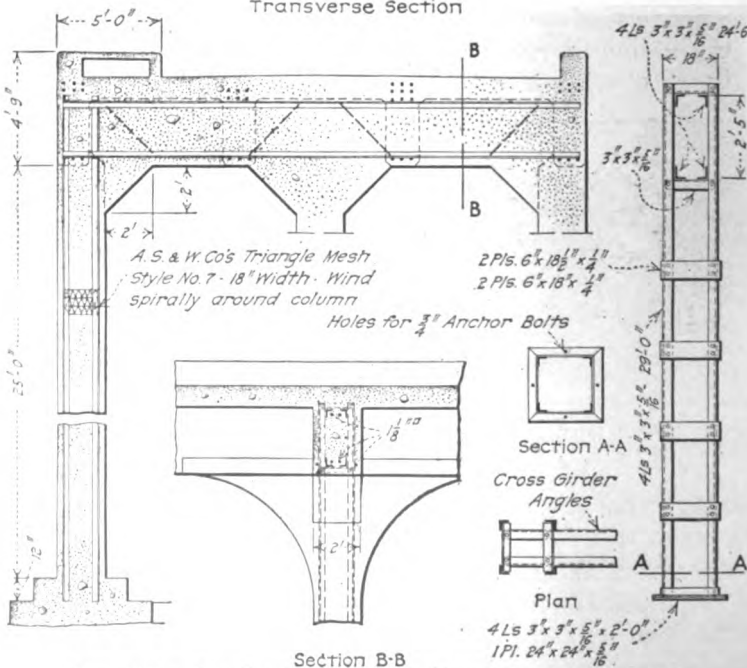
Section B-B FIG. 292.—Details of Mill Creek bridge, Village of Cazenovia, Richland Co., Wis.
