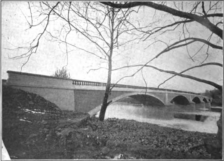
FIG. 385.—Polished arch ring contrasting with roughened spandrel wall. The accentuation of structural members results in a beautiful bridge.
