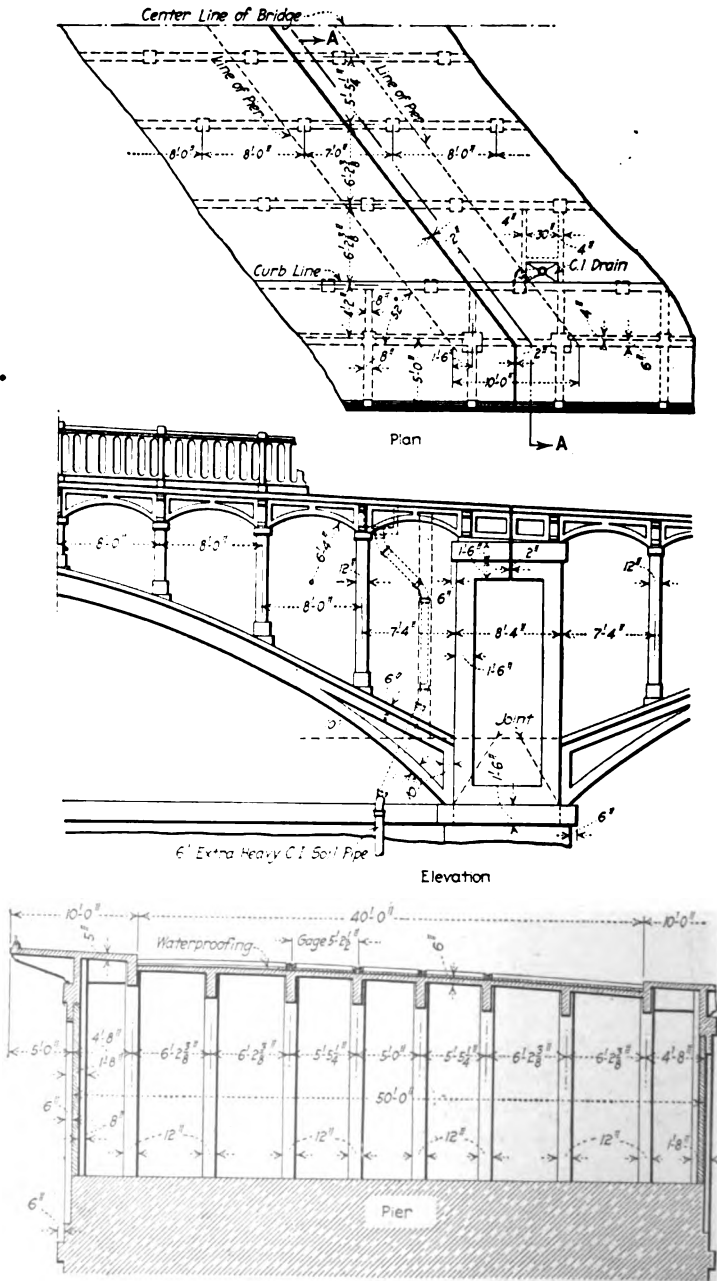
Section A-A Ludlow Avenue viaduct, Cincinnati, Ohio.
