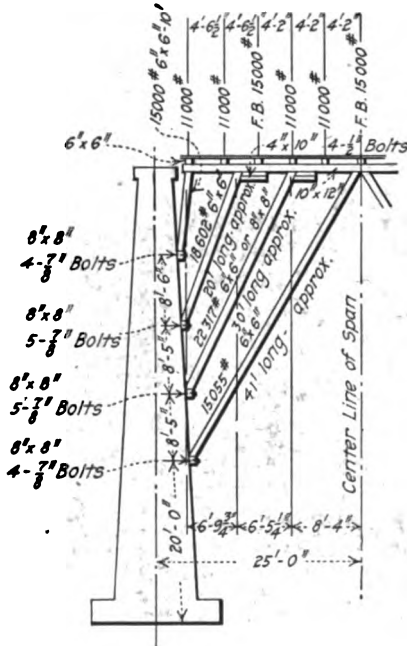
FIG. 476.—Samuel's Avenue viaduct. Detail of river span falsework used on the Fourth Street viaduct (Ft. Worth) of the same type of construction.
