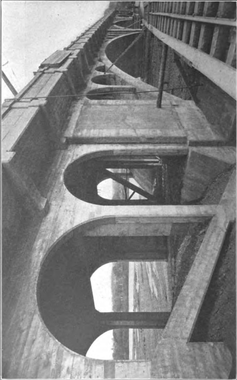
Courtesy of Sandusky Portland Cement Co. Fig. 217. —Chippewa River bridge, Eau Claire, Wis.
