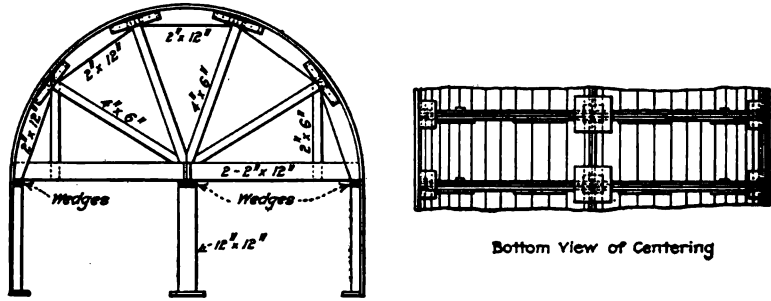
FIG. 332.—Centering for arch culverts.
