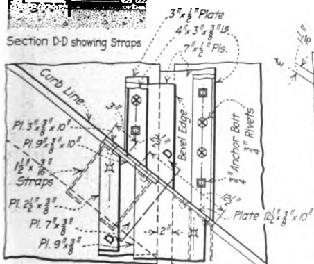
Expansion Joint Detail at Curb Line
