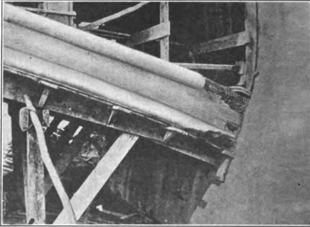
FIG. 575.—Portion of Chateau Thierry bridge. Armouring exposed (before filling).
