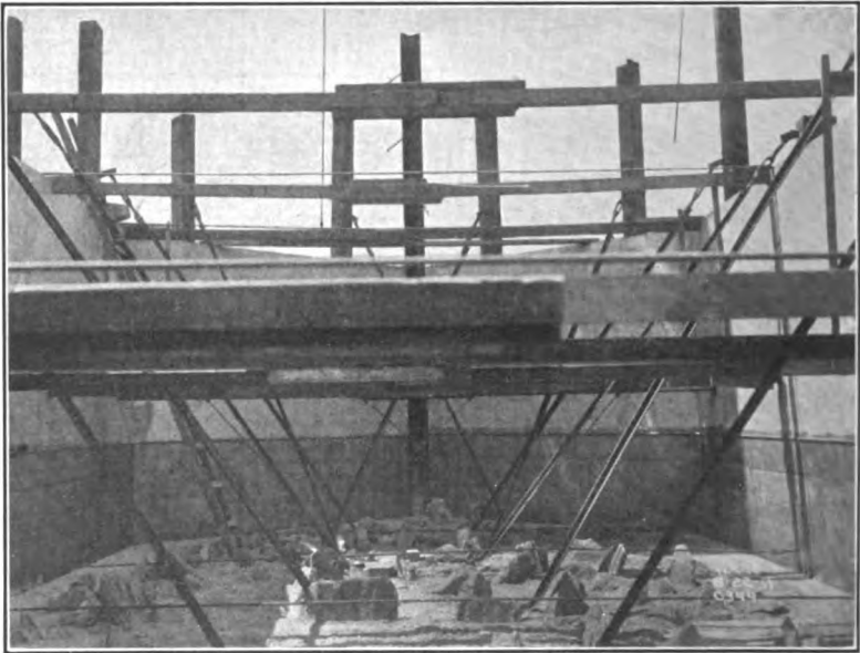
FIG. 417.—Yardley bridge. View inside of pier form showing bracing.
