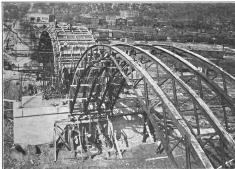
FIG. 126.—Steel centers for North Side Point bridge, Pittsburgh, Pa.
