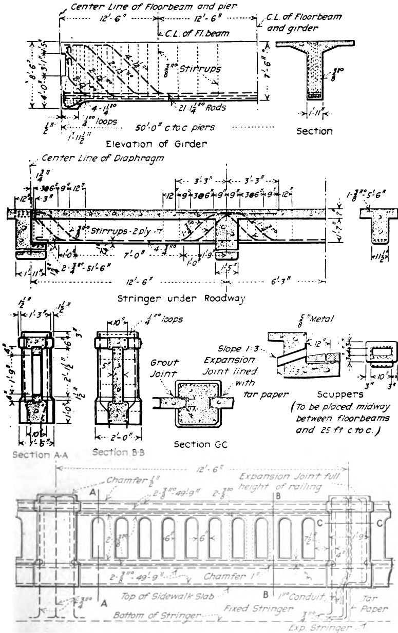
Typical Post Typical Panel of Hand Railing Post carrying Lamp Fig. 278.—Details of floor system and railing, North Samuels Avenue viaduct, Fort Worth, Texas.
