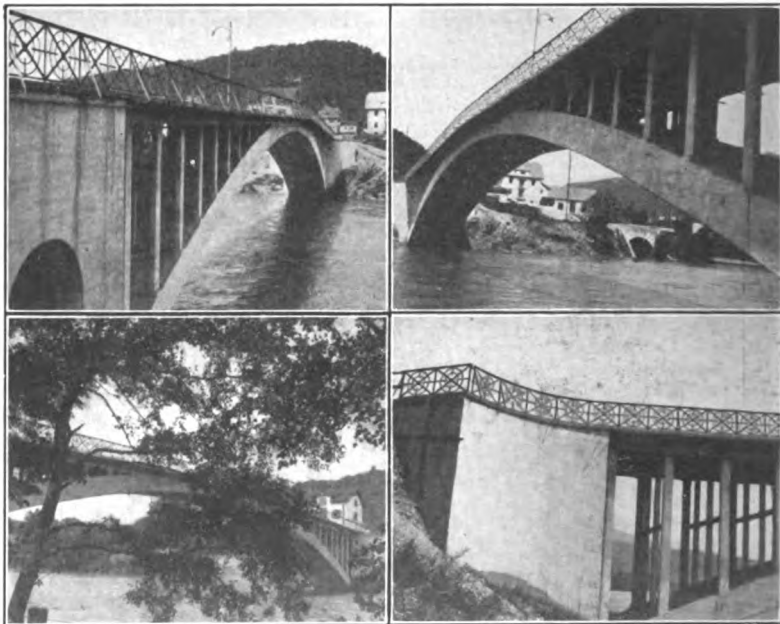
FIG. 546.—Aare River bridge at Olten, Switzerland.
