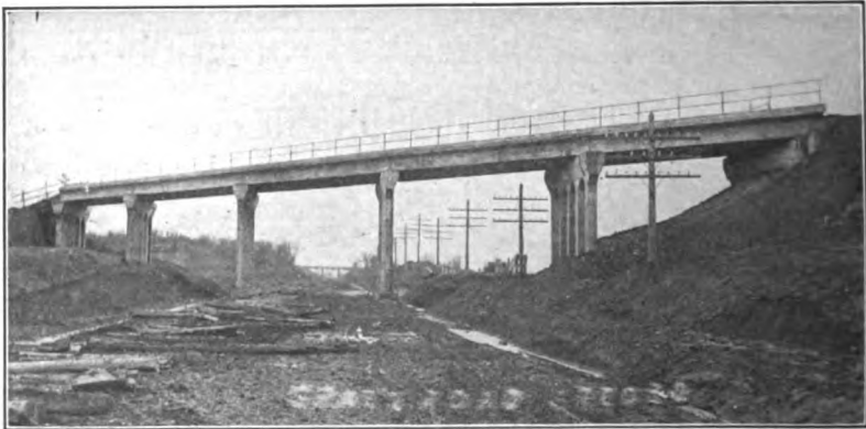
FIG. 375.—Pile trestle in concrete. Supports appear to be inadequate, and the entire effect is one of cheapness accentuated by the gas pipe railing which is not even panelled in harmony with the spans. This structure is a wooden trestle moulded in concrete.
