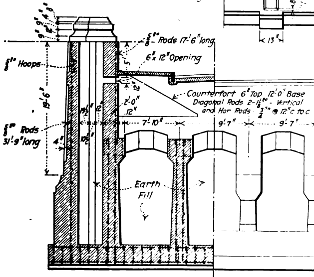
Section at Center Line of Monument
