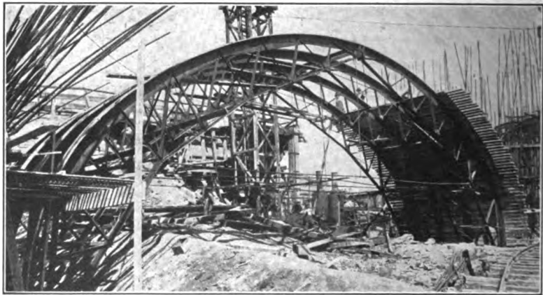
Courtesy of Mr. N. S. Sprague, Superintendent, Dep't. of Public Works, Pittsburgh. Fig. 107.—Steel centering for North Side Point bridge, Pittsburgh, Pa.
