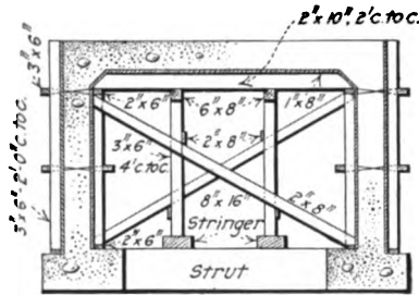
FIG. 326.—Box-culvert forms, C. M. & St. P. Ry.
