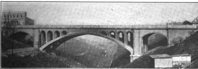
Courtesy of Mr. N. S. Sprague, Superintendent, Board of Public Works, Pittsburgh. FIG. 10F.—Atherton Avenue bridge over P. J. R. R., Pittsburgh, Pa. Note fake joints in ribs, posts, and quoins.
