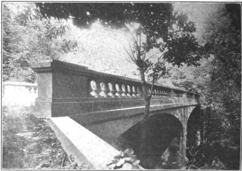
FIG. 402.—A properly-detailed railing. Pier and coping, however, not sufficiently pronounced.
