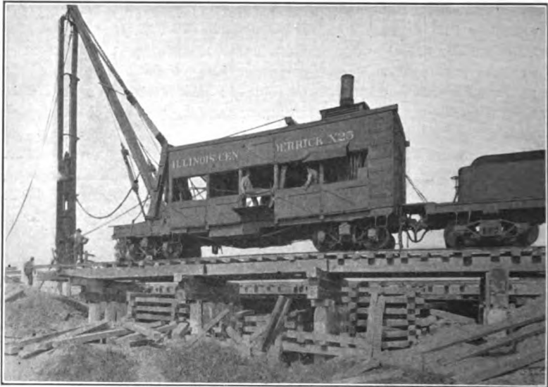
Courtesy of Mr. Maro Johnson, Engineer of Bridges and Buildings, I. C. R. R. FIG. 452.—Pile trestle. Driving concrete piles with steam hammer. Temporary track for driver blocked up on piles just driven.
