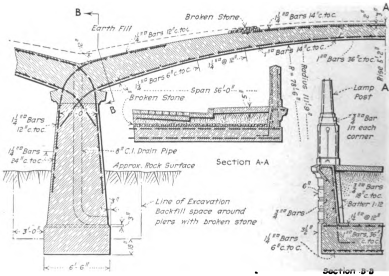
FIG. 61A. —Details of Pine Street bridge, Lima, Ohio.
