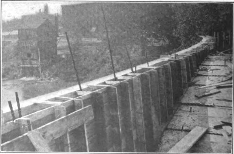
FIG. 151. —Spandrel-wall forms.
