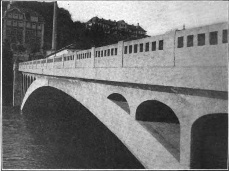
FIG. 511.—Reuss River bridge at Lucern, Switzerland. (Note rough stubble finish.)
