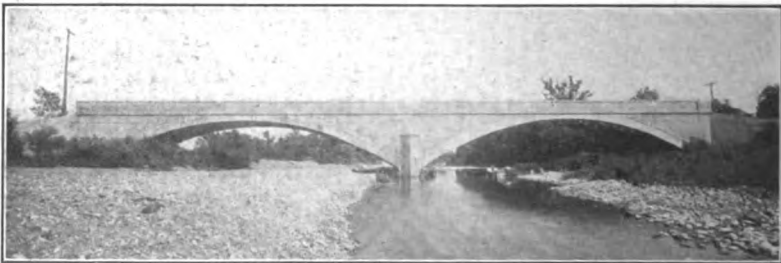
FIG. 379.—Unsatisfactory design with low and inadequate pier; awkward cutwater details; no camber, resulting in an appearance of sag in coping.
