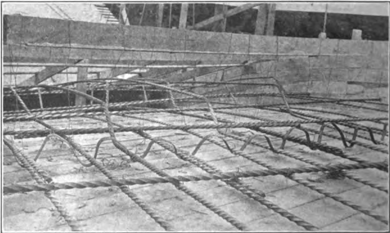
FIG. 93. —Arch reinforcement held in place by being wired to transverse timbers supported above the surface of the finished concrete. Bridge of Lutén Design.
