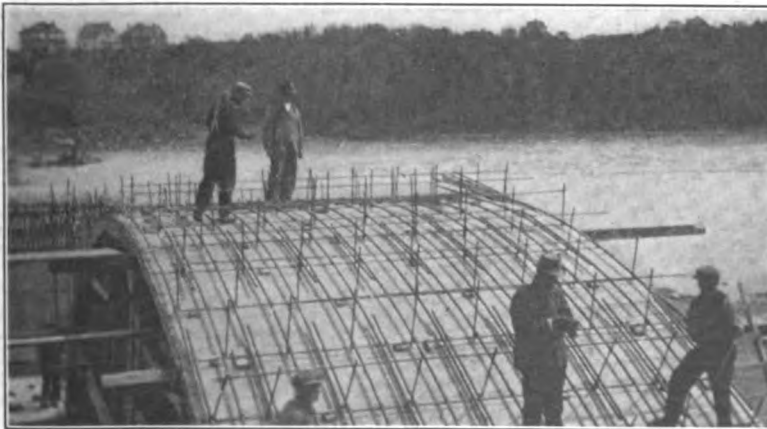
Courtesy of Mr. Daniel B. Luten, Consulting Engineer, Indianapolis. FIG. 95.—Bridge over Saskatchewan River at Saskatoon, Canada. Reinforcement in place on one of the arch ribs.
