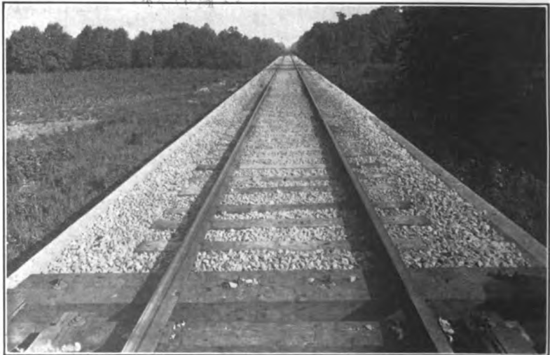
Courtesy of Mr. Maro Johnson, Engineer of Bridges and Buildings, I. C. R. R. FIG. 261.—Roadbed of trestle shown in Fig. 260.
