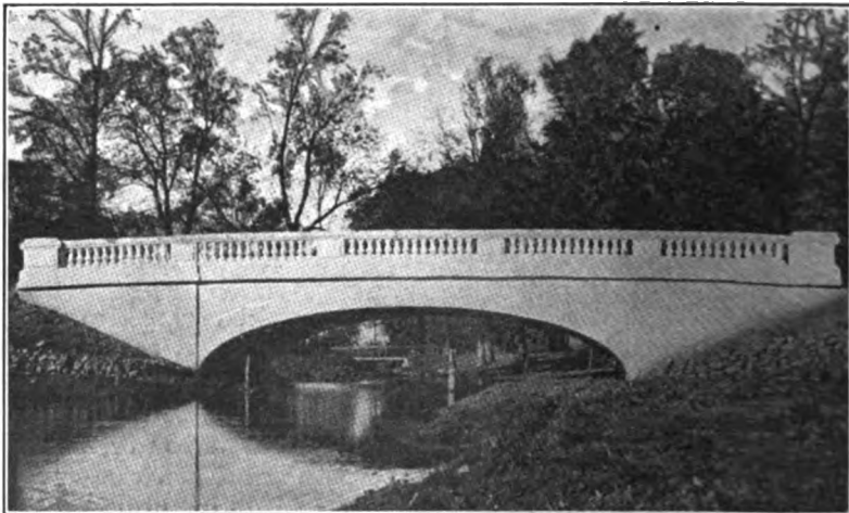
FIG. 405.—A handsome bridge except for two defects. A heavy post and closed dado would have been preferable over each abutment, and the curved camber should have ended with the span.
