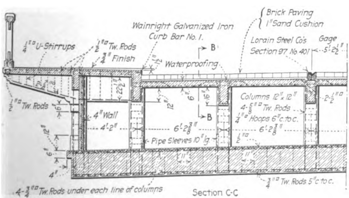
Ludlow Avenue viaduct, Cincinnati, Ohio.
