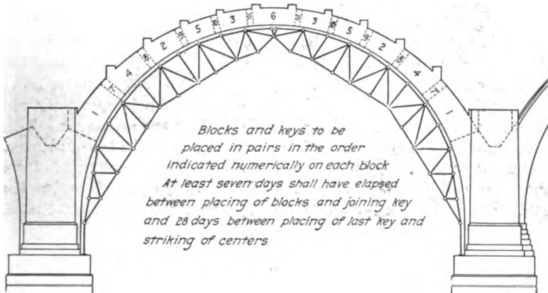
FIG. 443.—Tunkhannock viaduct. Diagram showing schedule of pouring voussoirs and keyways of arches.
