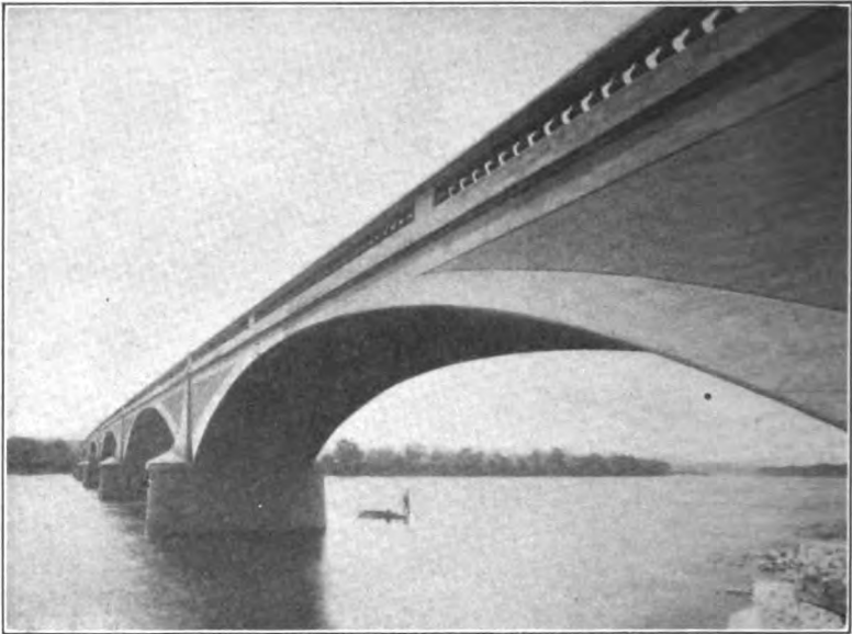
Courtesy of Mr. Daniel B. Luten, Consulting Engineer, Indianapolis. FIG. 60. —Georgetown bridge over Wabash River, Georgetown, Indiana.
