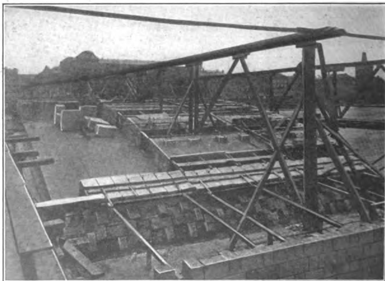
FIG. 516.—View of Rudolfinum bridge at Prague under construction, showing skewback hinge blocks, also subdivided erection (or placing) of arch in progress.
