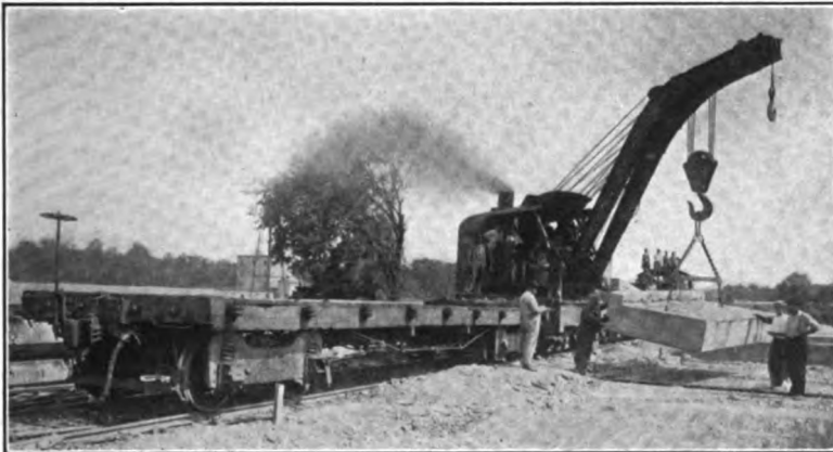
FIG. 457.—Pile trestle. Handling 19-ton concrete slab with locomotive crane.
