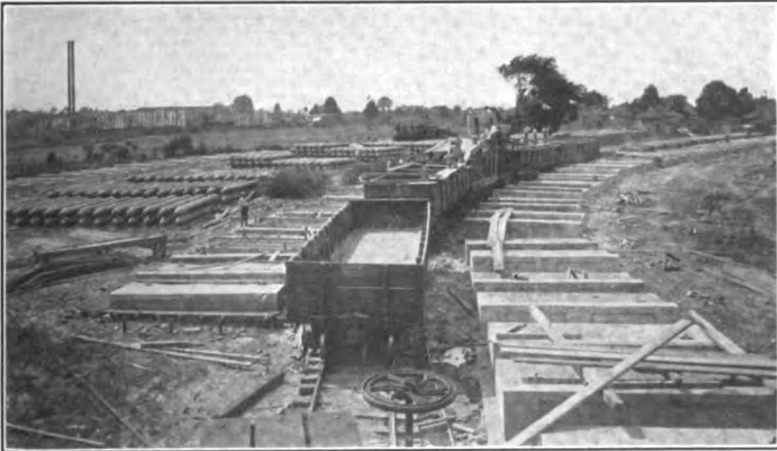
FIG. 451.—Pile trestle. Near view of mixer train concreting slabs. Concrete piles and slabs seasoning alongside the track.
