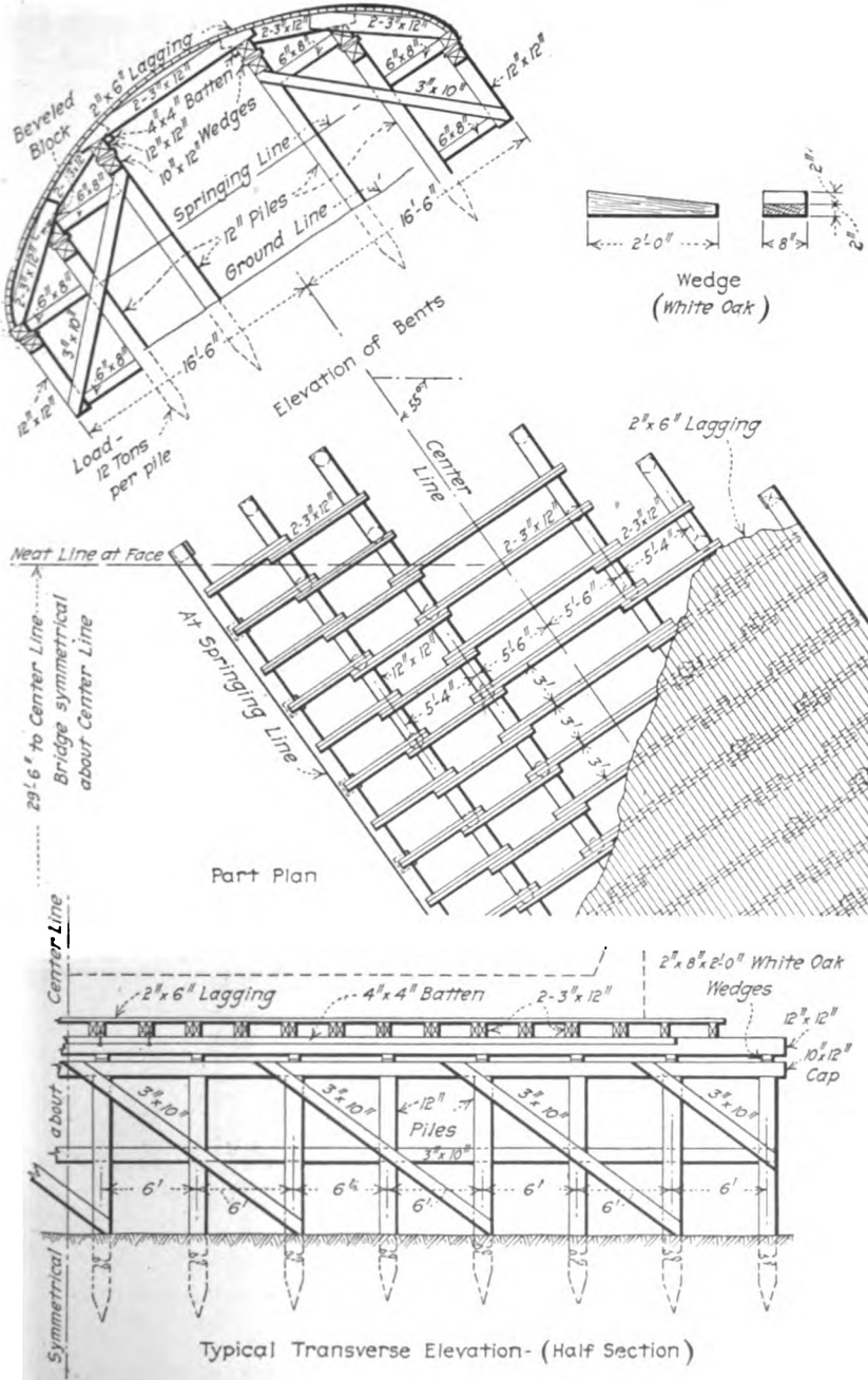
FIG. 116.—Details of arch centers for proposed renewal, C. R. R. Co. of N. J.
