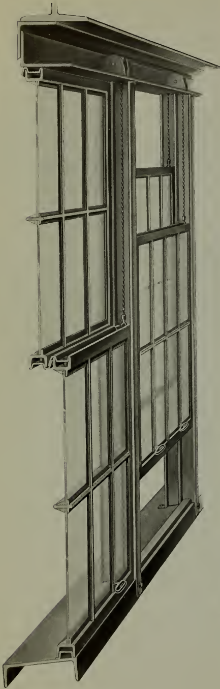
Sectional Perspective of Counterbalanced United Steel Sash.
