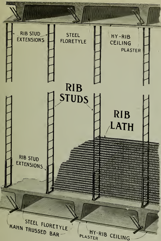
Hollow Walls or Partitions. Rib Lath wired to Rib Studs.
