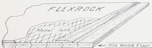
End Installation with Wood Strip.
