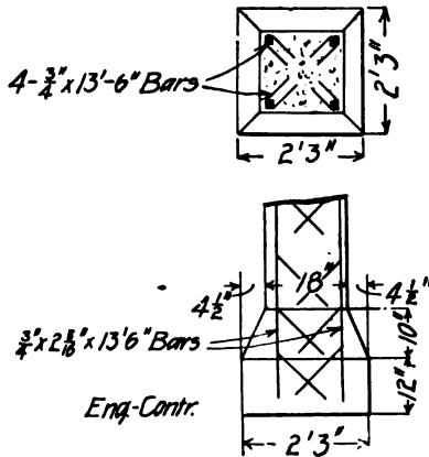
Fig. 276.—Column Construction for 75,000-Gallon Reservoir.
