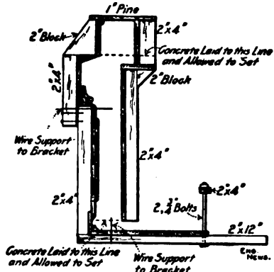
Fig. 297.—Form for Concrete Facade Shown by Fig. 298.
