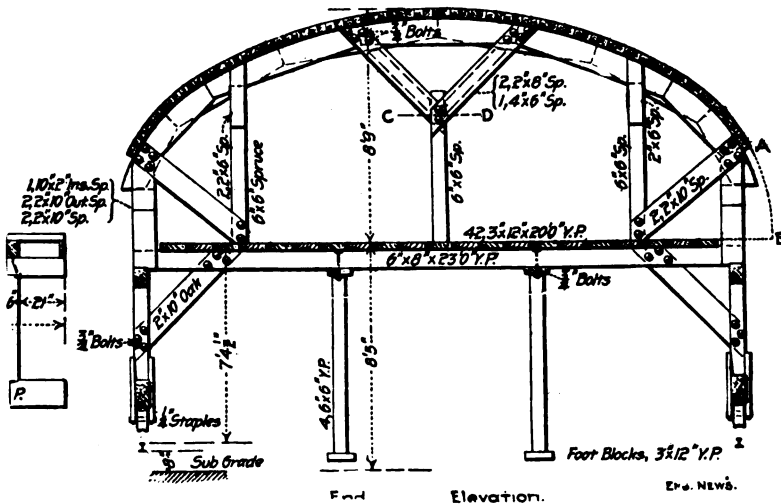
Fig. 145.—Travelling Form for Roof Arch, New York Subway Tunnels. rangement as operated in the Central Park tunnel is shown by Fig. 146. In the Park Ave. tunnel the “bridges” were dispensed with, the skips being hoisted through the open end bays of the derrick car and set directly on the cars on the center traveler.
