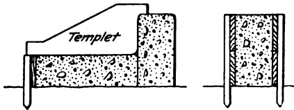
Fig. 124.—Form for Two-Piece Curb Construction.
