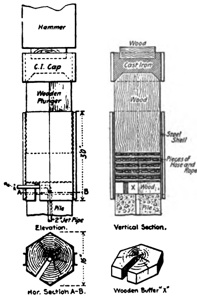
Fig. 62.—Cushion Cap for Driving Glibreth Corrugated Pile.
