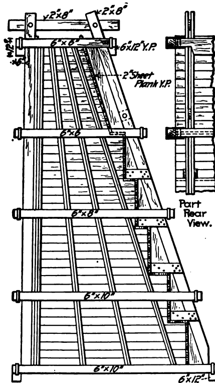
Fig. 110.—End View of Forms for Retaining Wall, New York Central Terminal Work.
