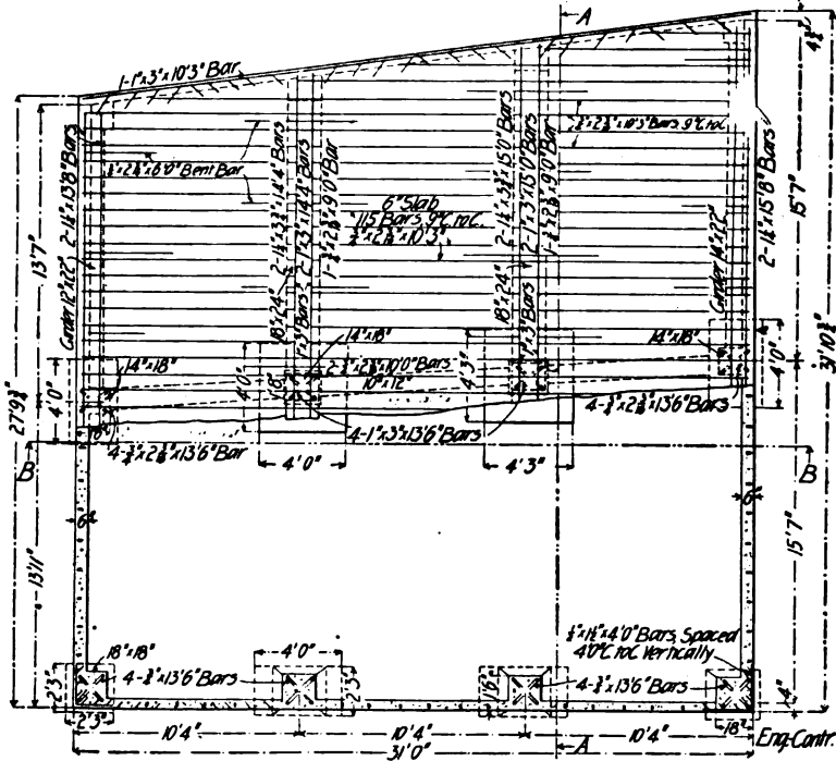
Fig. 273.—Sectional Plan of 75,000-Gallon Reservoir.
