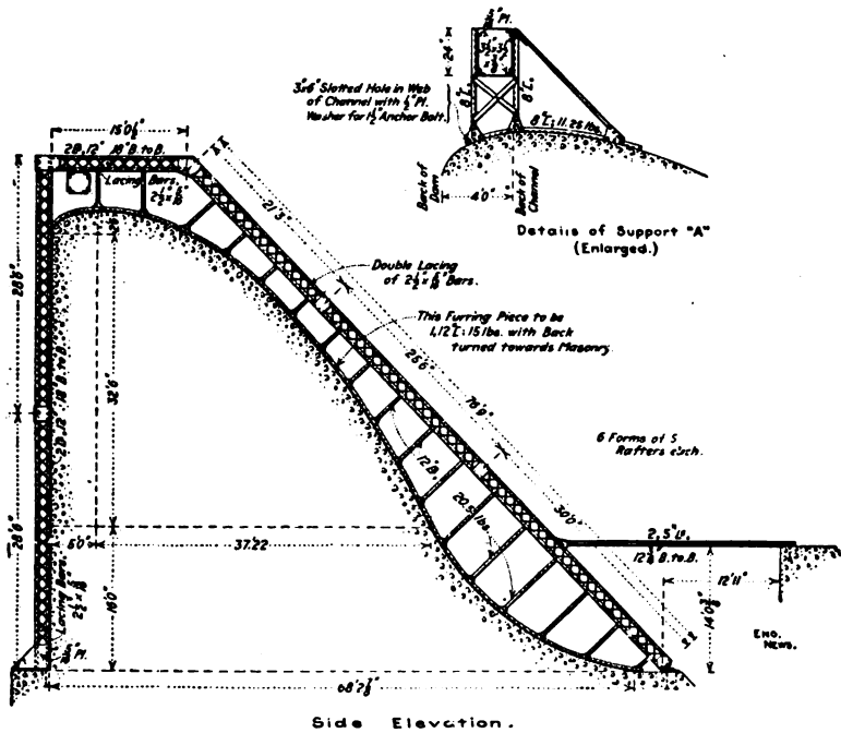
Fig. 90.—Steel Forms for McColl Ferry Dam.
