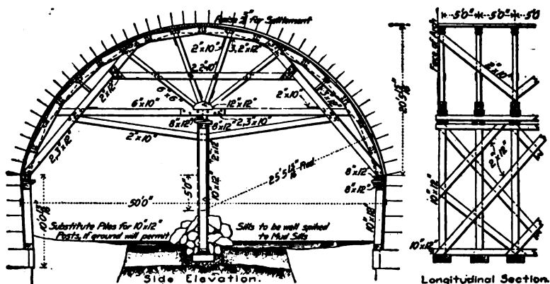
Fig. 148.—Center for 50 ft. Arch Span (Supported).
