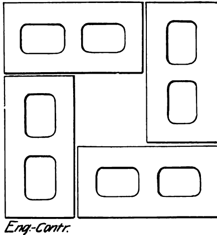
Fig. 246.—Concrete Block Pilaster for a Factory Building.
