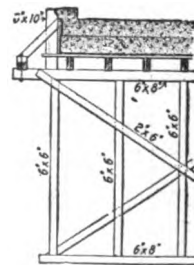
Fig. 301.—Method of Supporting Cornice Forms Shown by Fig. 300.
