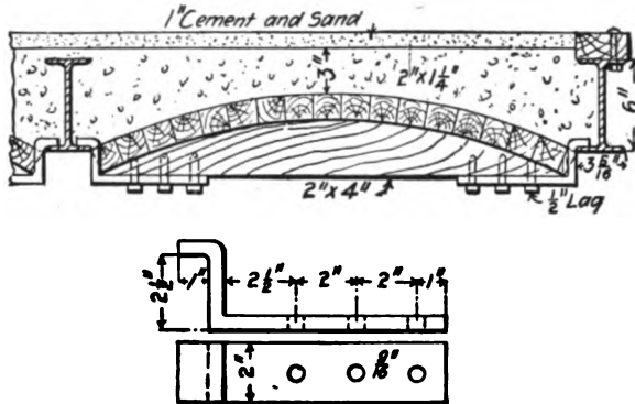
Fig. 192.—Form for Arch Slab Between I-Beams.
