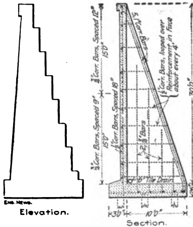
Fig. 98.—Comparison of Plain and Reinforced Sections for Retaining Walls (C. E. Graft).
