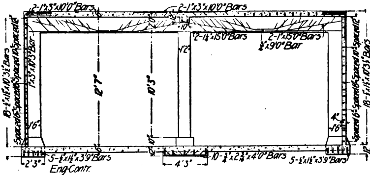
Fig. 275.—Transverse Section of 75,000-Gallon Reservoir.
