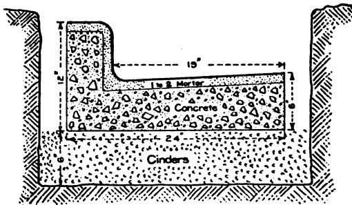
Fig. 125.—Concrete Curb and Gutter at Champaign, Ill.
