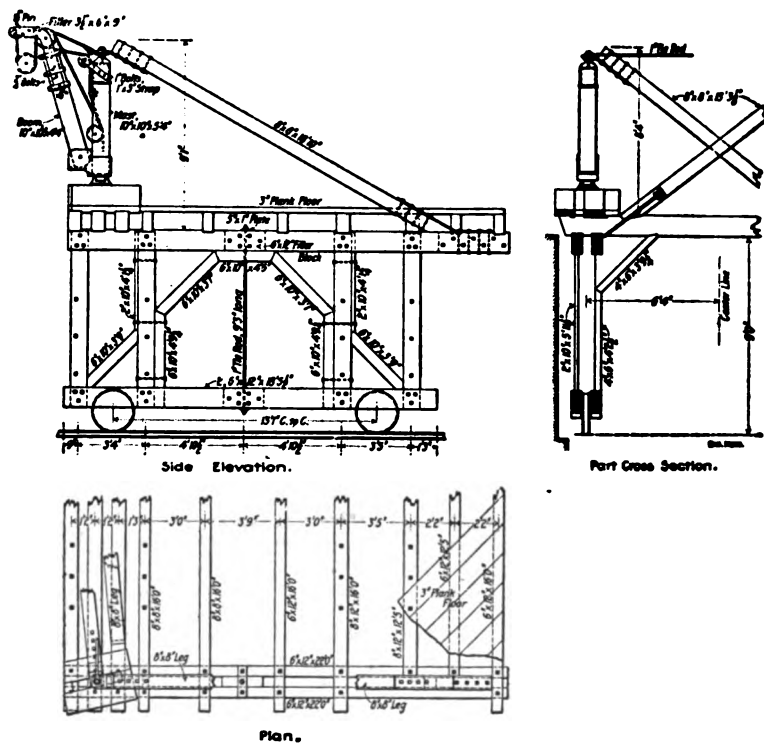
Fig. 127.—Traveling Derrick for Constructing Side and Center Walls, Capitol Hill Tunnel.
