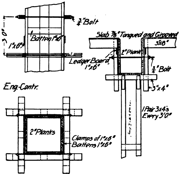
Fig. 238.—Column and Floor Forms for Four-Story Garage.
