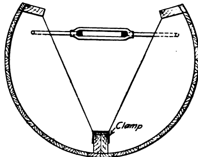
Fig. 249.—Invert Form for Conduit Construction.
