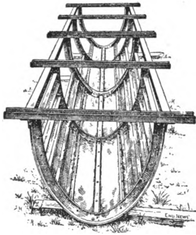
Fig. 263.—Invert Form for Sewer Construction.
