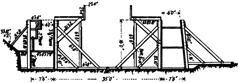
Section G-H.
