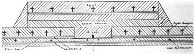
Fig. 270.—Bordenave Pipe for Swansea, England, Water Works.
