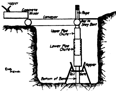
Fig. 14.—Belt Conveyor and Chute for Handling Concrete.
