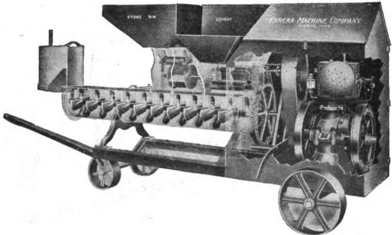
Fig. 22.—Eureka Automatic Feed Continuous Mixer.
