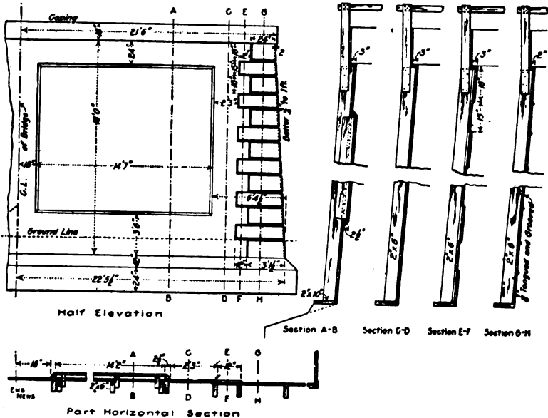
Fig. 299.—Forms for Curved Concrete Abutments.
