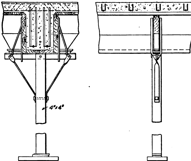
Fig. 193.—Girder and Slab Form for Warehouse at St. Paul, Minn.
