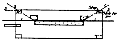
Fig. 209.—Table for Bending Reinforcing Bars.
