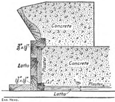
Fig. 300.—Cornice Form.
