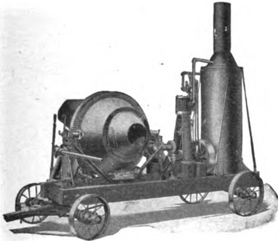
Fig. 21.—Smith Concrete Mixer.
