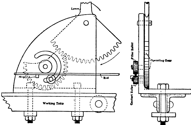
Fig. 212.—Device for Bending Reinforcing Rods.
