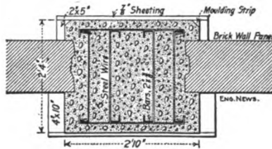
Fig. 223.—Section of Rectangular Wall Column.
