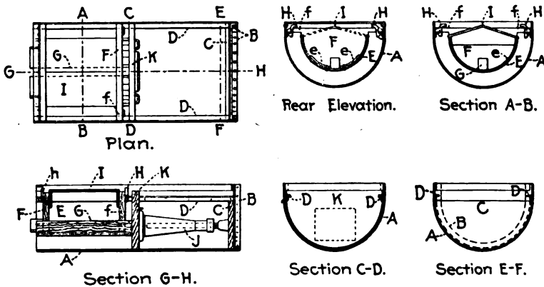
Fig. 260.—Travelling Invert Form for Sewer Construction.
