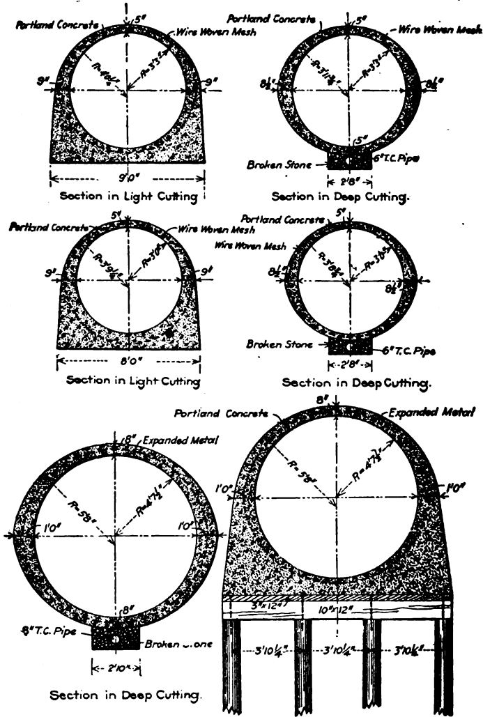
Section through Marsh. Fig. 265.—Cross-Sections of Sewer at Wilmington, Del.
