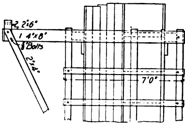
Fig. 182.—Form for Corner Wall Column.
