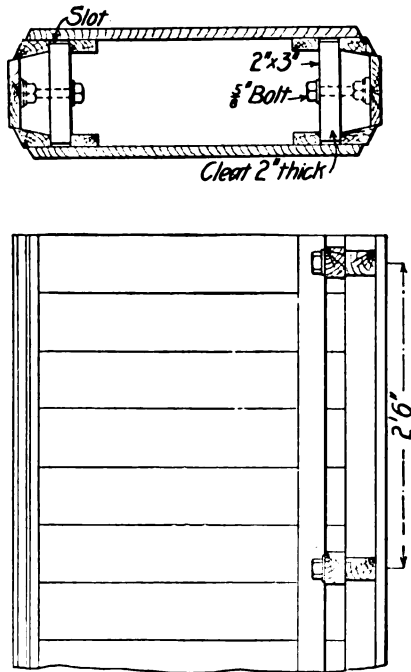
Fig. 183.—Core Form for Hollow Column.
