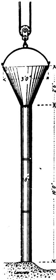
Fig. 33.—Steel Tremie for Depositing Concrete Under Water.
