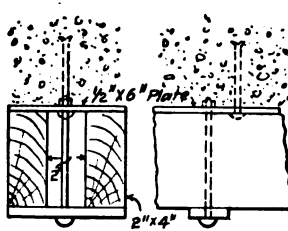
Fig. 283.—Sketch Showing Filler for Joint Between Form Panels.
