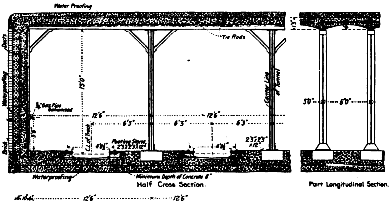
Fig. 143.—Cross-Section of New York Rapid Transit Subway.
