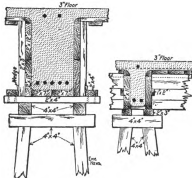
Fig. 196.—Girder and Beam Forms for Factory Building, Beverly, Mass.
