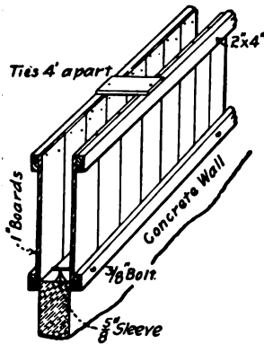
Fig. 203.—Sectional Form for Wall Construction.
