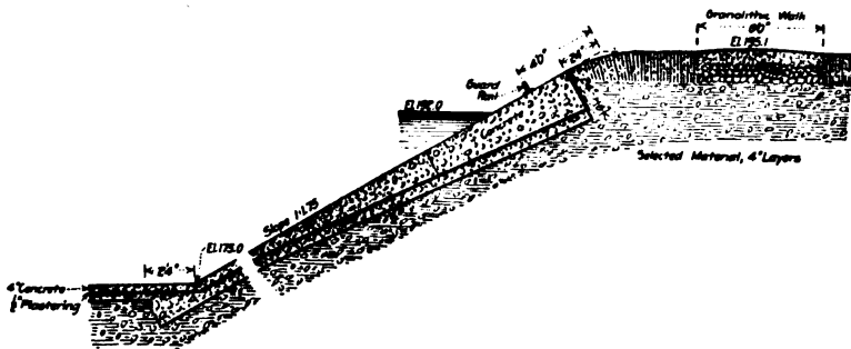
Fig. 285.—Section of Reservoir Lining, Quincy, Mass.
