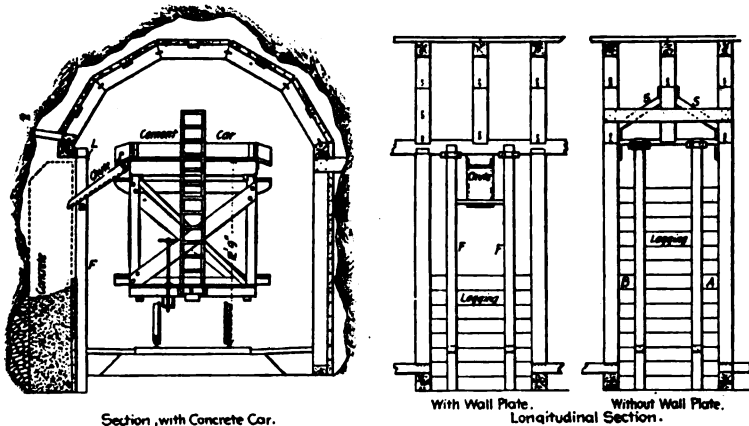
Fig. 130.—Sketches Showing Method of Lining Mullin Tunnel.
