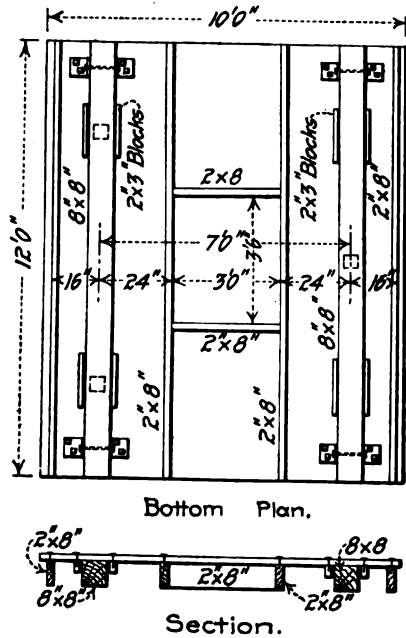
Fig. 57.—Details of Working Platform for Concrete Pier Construction.
