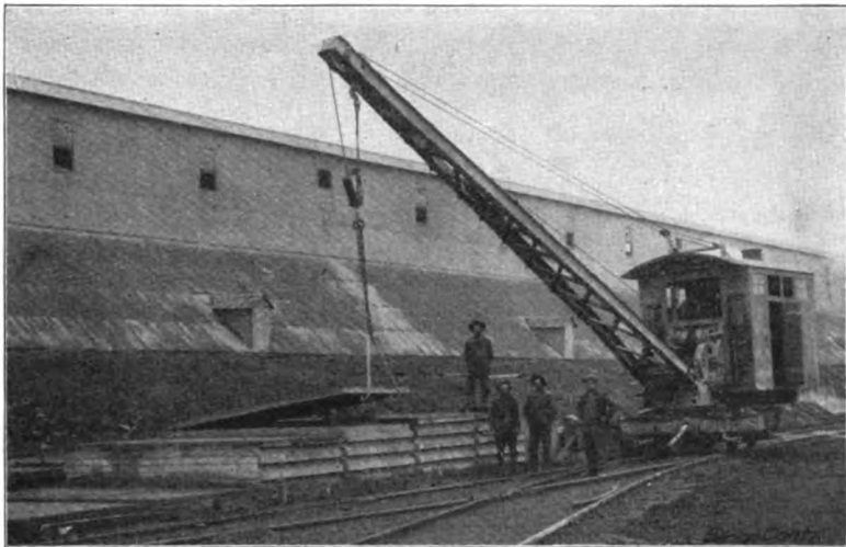
Fig. 245.—View Showing Method of Handling Roof Slabs.
