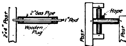
Fig. 166. Fig. 167. Details of Haulage Rope Guides.
