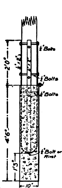
Fig. 305.—Base for Wooden Pole.
