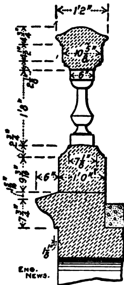
Fig. 302.—Cornice and Balustrade for Arch Bridge.
