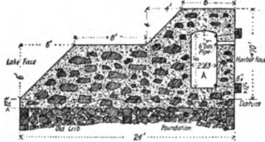
Fig. 77.—Cross Section of Marquette Breakwater.
