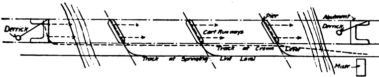
Fig. 152.—Sketch Showing Car and Trestle Plant for Concreting an Arch Bridge.
