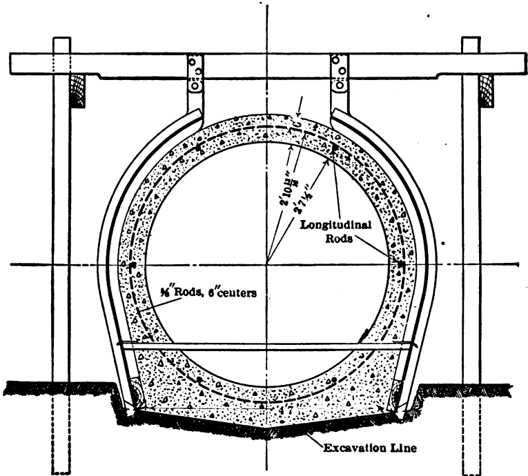
Fig. 251.—Cross-Section of Pinto Creek Irrigation Conduit.
