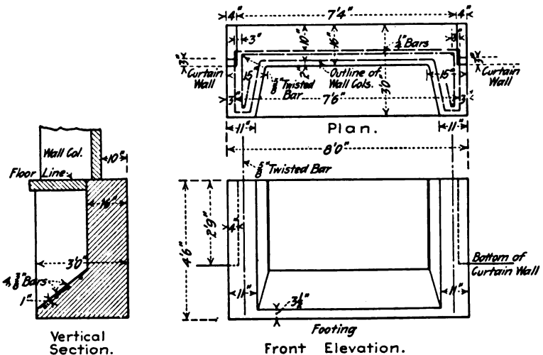
Fig. 229.—Footing for Wall Column Shown by Fig. 228.
