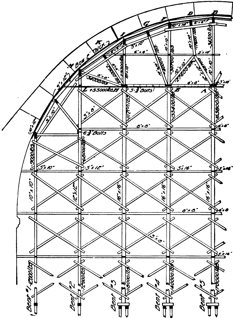
Fig. 158.—Center for Connecticut Ave. Bridge (Elevation).
