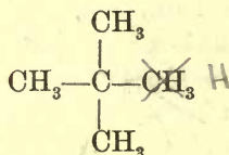
Isobutane.
