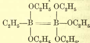
Boron-ethopentethoxide.
