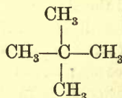
Tetramethylmethane.
