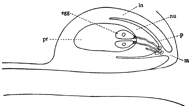
FIG. 326. Diagram of a vertical section of a pine ovule and the scale to which it is attached and of the male and female gametophytes at the time of fertilization: pr represents the prothallus with two archegonia; in represents the integument, nu the nucellus, m the micropyle, and p pollen tubes, two of which have reached the neck cells of the archegonia. Redrawn from Strasburger.
