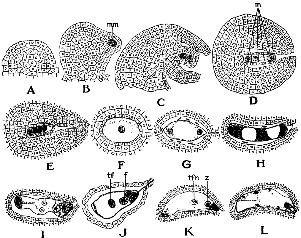
FIG. 166. Stages in the development of an ovule and a young seed of pepper. A-D, formation of four megaspores (m) from a megaspore mother cell (mm) in a young ovule; E, disintegration of three of the megaspores; F-I, development of an 8-nucleate embryo sac from one of the megaspores, a fusion nucleus is formed by the fusion of the two nuclei near the center of the sac, only a little of the surrounding ovule tissue is represented; J, fertilization (f) and triple fusion (tf); K, zygote (z) and triple-fusion nucleus (tfn); L, early stages in the development of the embryo and endosperm of the seed. After H. L. Cochran, Journal of Agricultural Research , with some modification.
