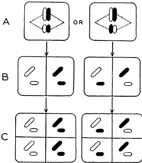
FIG. 210. A diagram of chromosome distribution during the formation of microspores from microsporocytes, or of megaspores from megasporocytes in a plant having two pairs of unlike chromosomes; all breaks disregarded.
