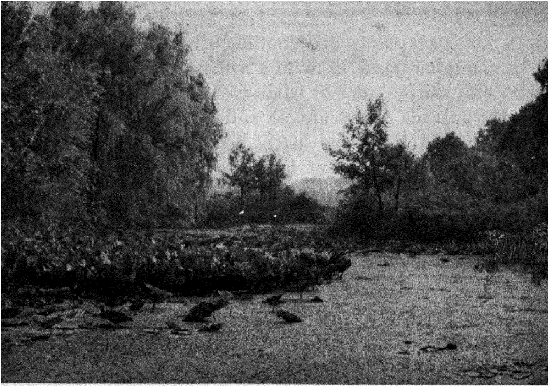
FIG. 268. Plants in various degrees of submergence. Many plants not evident in the picture are wholly submerged. Water milfoils, hornwort, elodeas, pondweeds, and many others may be wholly submerged or with their tips slightly above the surface (foreground). Leaf blades of water lily and pond lily may be floating or raised above the surface. The leaves of cat-tail and bulrush are mostly aerial, and all but the root systems or parts of root systems of dogwood, alder, and willow are above the water. Photo by E. S. Thomas, Ohio State Museum.
