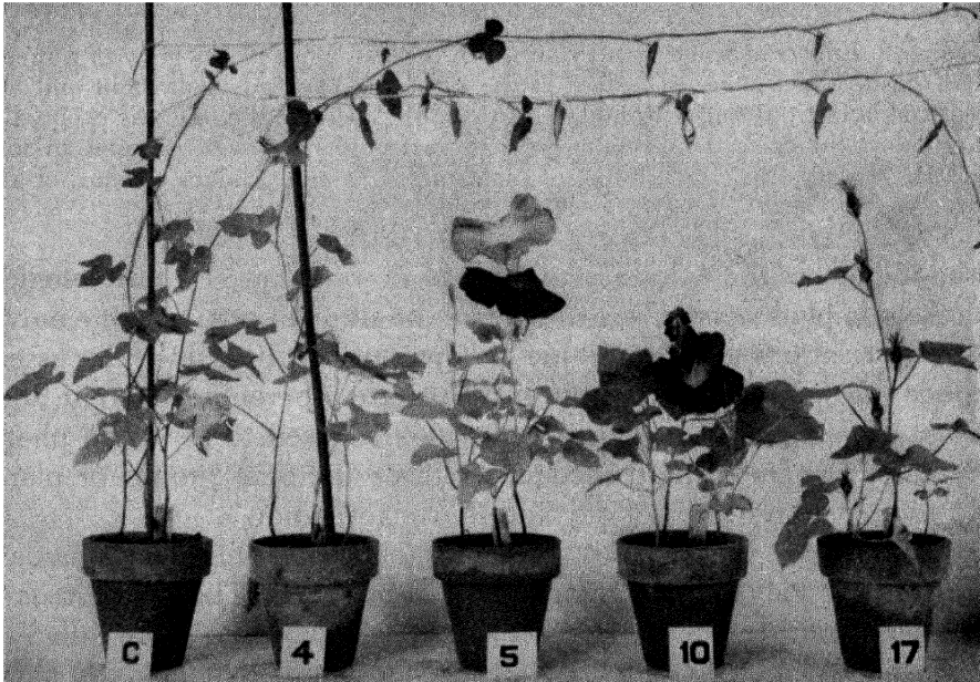
FIG. 143. Effects of length of day on vegetative growth and flower formation in morning glory. C, control plant exposed to long days from time of germination. Figures indicate the number of short-day periods to which the other plants were exposed during the seedling stage. All plants completed their development in long days. Photo by Victor A. Greulich.
