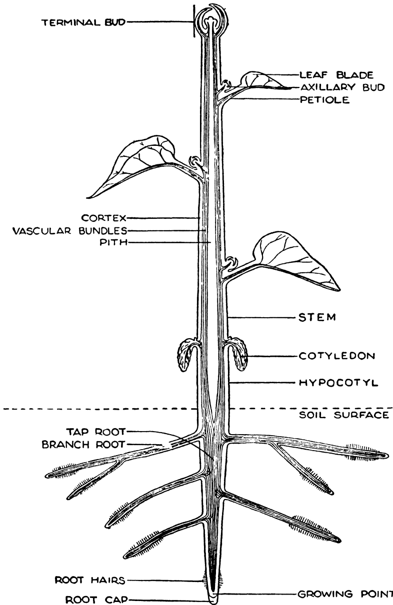
FIG. 10. Diagram of some external and internal structures of a seed plant.
