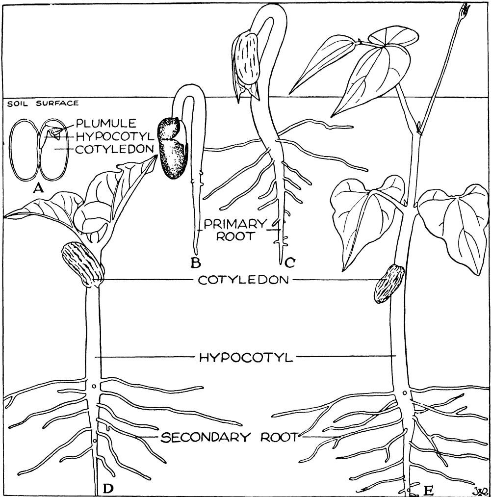
FIG. 8. Early stages in the development of a bean plant.
