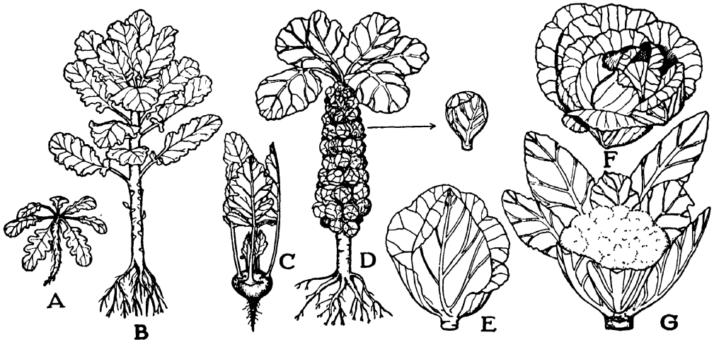
FIG. 196. Domesticated varieties derived from the wild cabbage, Brassica oleracea (A), a native of Europe. B is kale, Brassica oleracea acephala ; C, kohlrabi, B. oleracea caulo-rapa ; D, Brussels sprouts, B. oleracea gemmifera ; E, pointed-head cabbage, B. oleracea capitata ; F, round-head cabbage, B. oleracea capitata ; G, cauliflower, B. oleracea botrytis .
