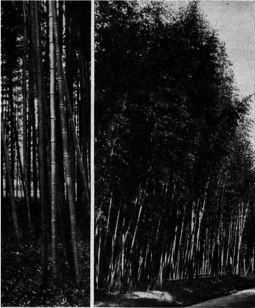
FIG. 99. Interior and exterior view of bamboo forest at Savannah, Georgia. Photo from United States Department of Agriculture.
