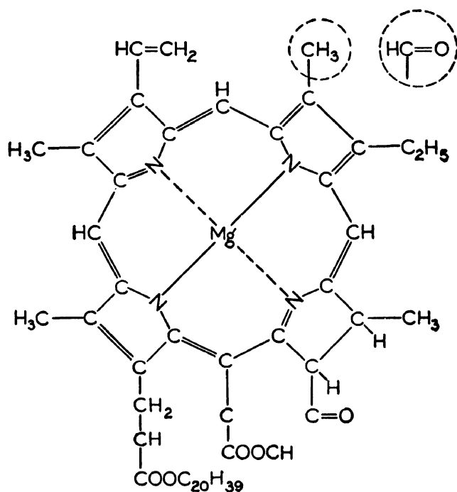
FIG. 56. Diagram representing the arrangement and complexity of the molecule of chlorophyll a. If the group, \text{CHO} , in the detached circle is substituted for the \text{CH}_3 group nearby, the diagram would represent the molecule of chlorophyll b. From B. S. Meyer and D. B. Anderson, 1939.
