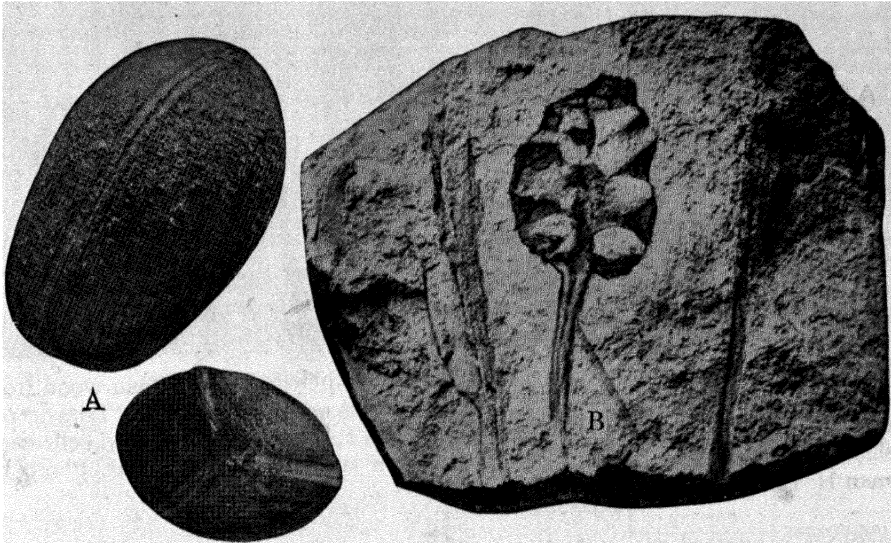
FIG. 355. A, side and end views of cast of seed-fern seed from the Upper Carboniferous; B, cast of redwood ( Metasequoia ) cone of the Upper Cretaceous age of Alaska. After W. Berry and C. C. Martin.
