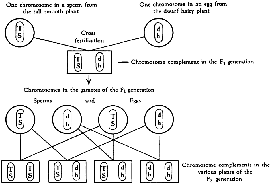
FIG. 213. Hereditary factors in the same chromosome are transmitted together from generation to generation unless a break occurs between them.
