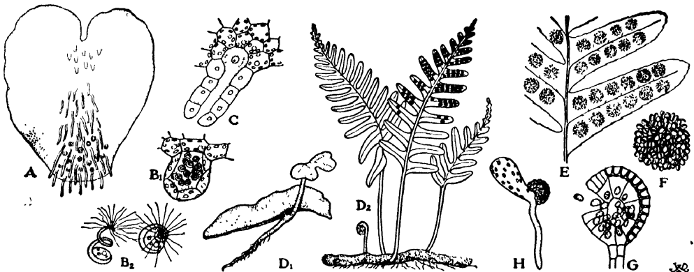
FIG. 311. The life cycle of a fern. The gametophyte (A) bears egg cells and sperms in archegonia and antheridia. When one of the sperms ( B_2 ) from an antheridium ( B_1 ) unites with an egg cell in an archegonium (C) a zygote is formed. From this zygote the sporophyte ( D_1 and D_2 ) develops and bears spores in groups of sporangia (E and F) on the lower side of the leaves. By the bursting of a sporangium (G) the spores are set free. When these spores germinate (H) on moist substrates a new gametophyte, like the one represented by A, develops from each of them.
