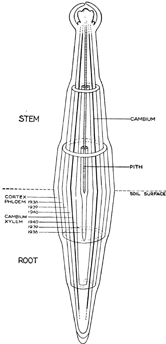
FIG. 96. Diagram of relative positions of xylem and phloem in a 3-year-old stem and root.
