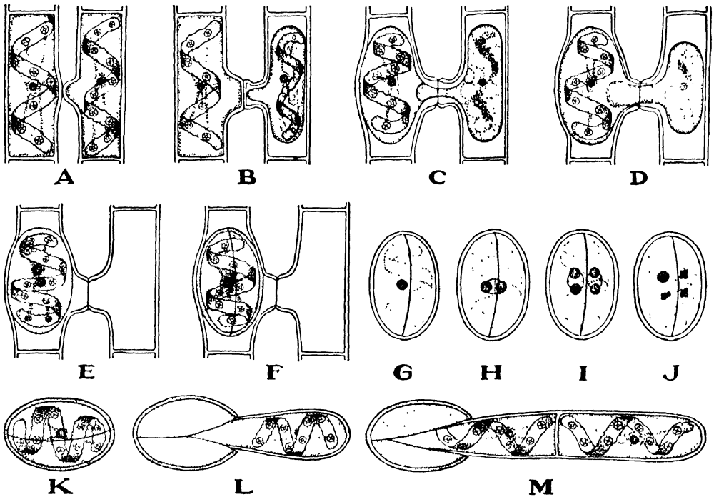
FIG. 283. Reproduction in Spirogyra and inheritance of the chloroplast.
