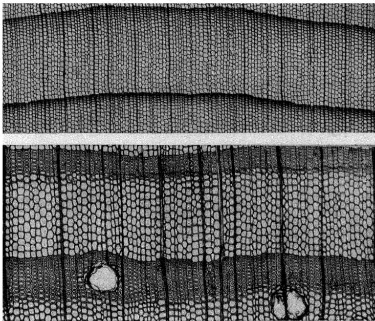
FIG. 109. Non-porous woods of arbor vitae (above) and of long leaf yellow pine (below). The large openings in the latter are cross sections of resin ducts. Photos from Forest Products Laboratory.
