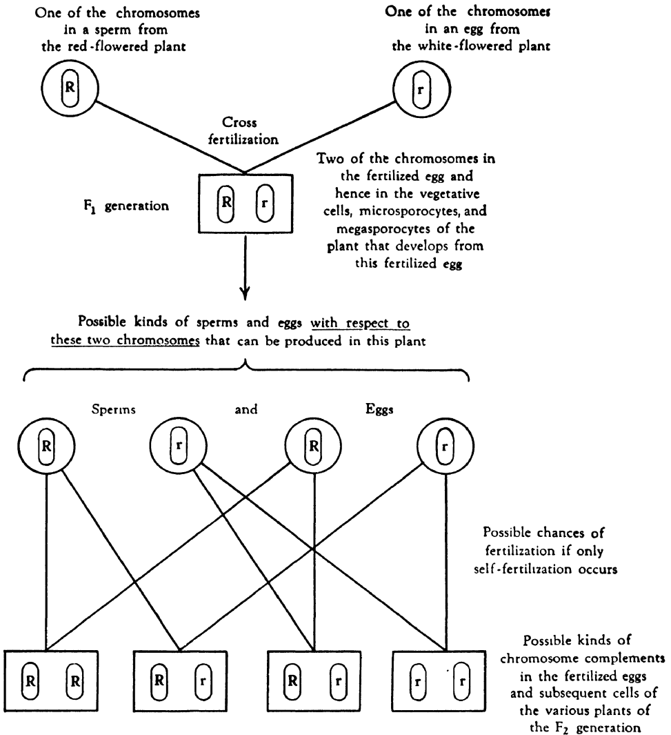
FIG. 212. A diagrammatic representation of the relation of chromosomes and factors of flower color in snapdragon.
