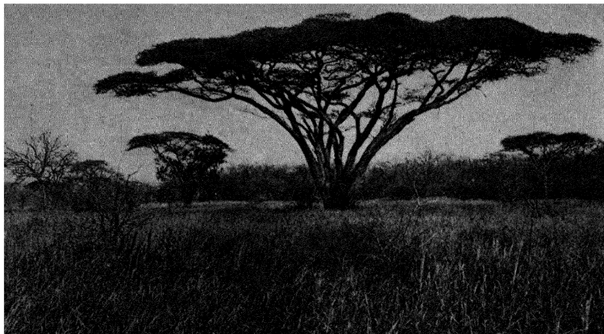
FIG. 344. An acacia savanna in Kenya Colony, Africa. In the background is an area of "thornbush." Photo by Walter Busse.
