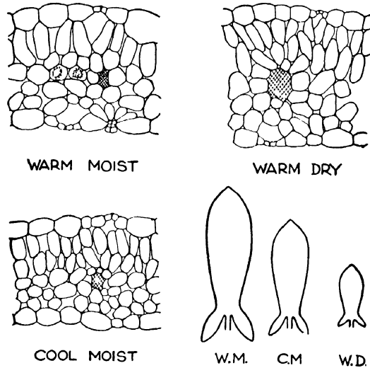
FIG. 41. Effects of temperature and drought on leaf size and structure of the sour dock. In the warm dry culture the plants wilted daily. The temperature of the substrate in the "cool moist" culture was on the average 10 degrees below that of the "warm moist" culture.
