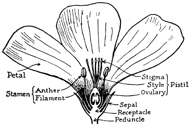
FIG. 151. Vertical section through a complete flower (Flax). Courtesy of World Book Co.
