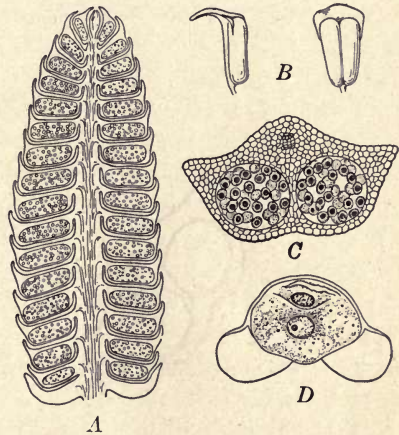
FIG. 97. — Staminate cone of pine: A, longitudinal section of cone, showing the stamens (microsporophylls) bearing pollen sacs (microsporangia) upon the under side; B, views of stamen from the side and from below, the latter showing the two pollen sacs; C, cross-section of a stamen, showing the two pollen sacs containing pollen grains (microspores); D, a winged pollen grain, showing within the early cells of the male gametophyte.
