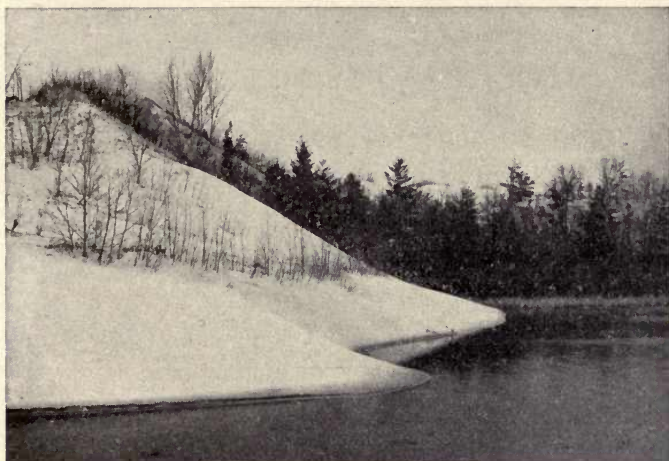
FIG. 235. — Dunes of Lake Michigan encroaching upon the land, in this case diverting Calumet River.
