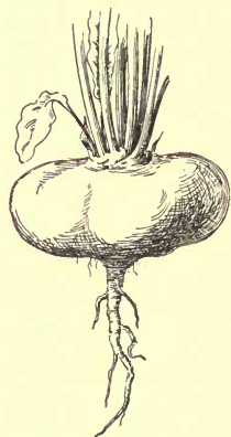
FIG. 49 — Turnip.—After BAILEY.
