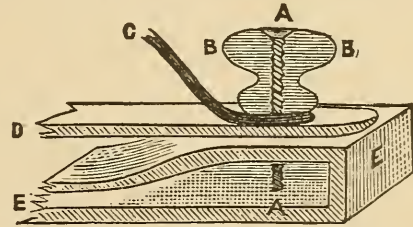
Fig. 4.—A Screw. B B Button. C Wire spring. D Spring-board. E E Stand.
