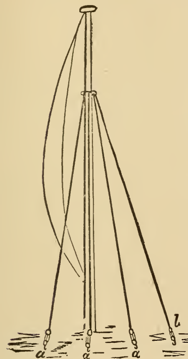
FIG 4 a a a, Shrouds. b, Stay.
