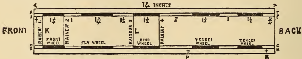
Fig. 1.—Plan of foundation, quarter of size.
