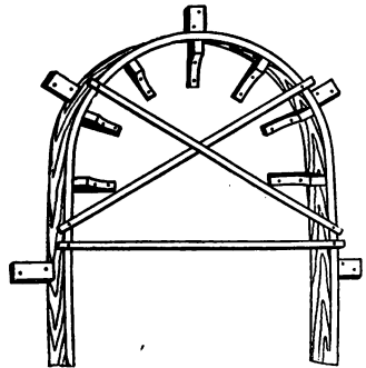
BENDING THE PLANK FOR THE HUNTING CABIN
