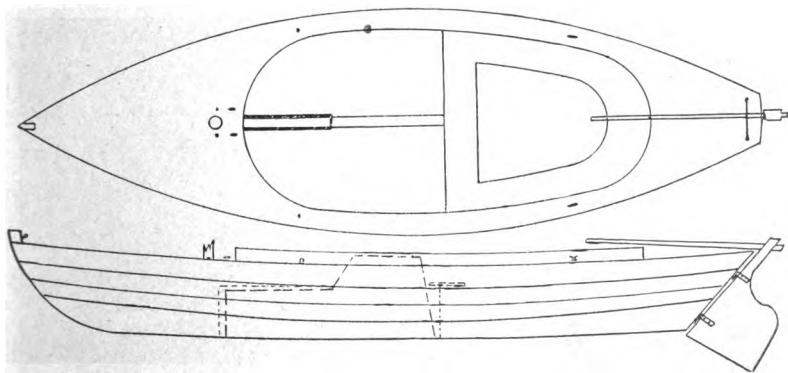
THE 17-FT. OVER ALL CLUB SAILING DORY, "BEE"
