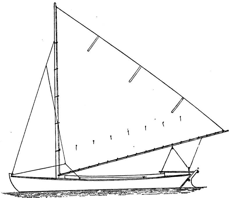
SAIL PLAN
