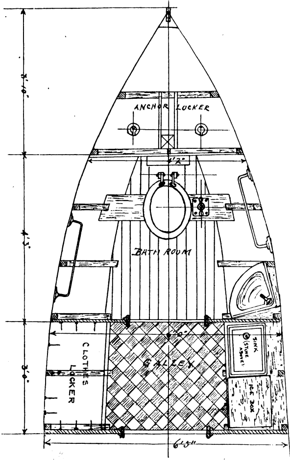
GALLEY AND TOILET ROOM PLAN OF THE "GO-SUM"
