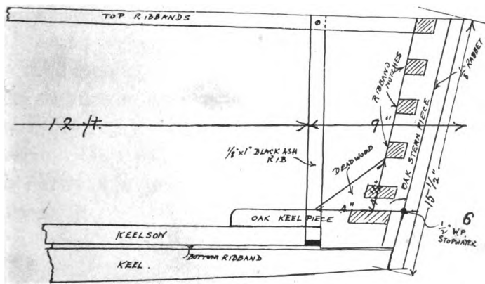
DETAILS OF STERN CONSTRUCTION, DECKED SAILING CANOE "WATERBAT IV"
