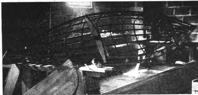
DECK FRAMING OF THE "WATERAT IV" Note center mould to left.
