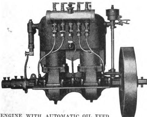
TWO CYLINDER ENGINE WITH AUTOMATIC OIL FEED
