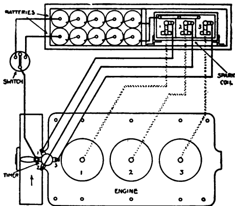
ELECTRICAL CONNECTIONS FOR JUMP-SPARK IGNITION, 3-CYLINDER ENGINE
