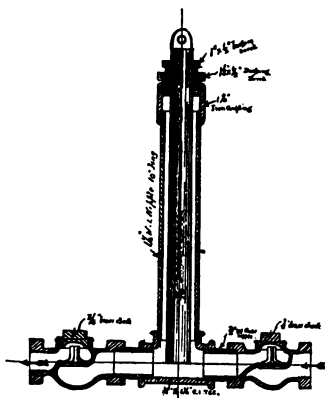
▲ HOME-MADE FORCE PUMP FROM PIPE-FITTINGS
