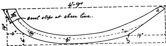
Fig. 3.—Stem piece, with measurements for making pattern
