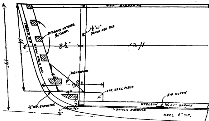
DETAILS OF STEM CONSTRUCTION, DECKED SAILING CANOE "WATERBAT IV"
