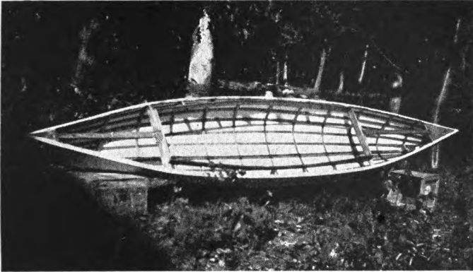
"WATERAT IV" WITH HER CANVAS ON Showing deck timbers.
