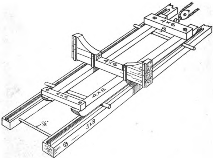
A SIMPLE MARINE RAILWAY
