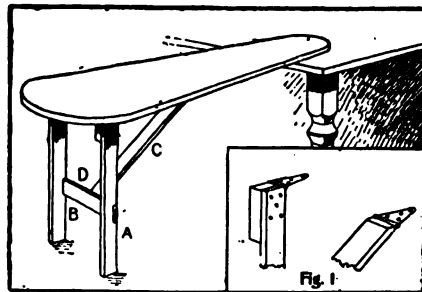
Ironing-Board Stand
