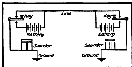
Diagram of One-Wire Line
