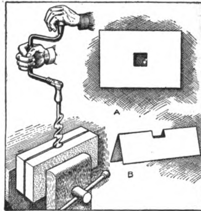
Boring a Square Hole
