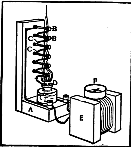
Thermo Battery
