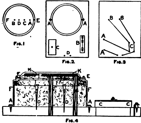
Details of Electric Stove
