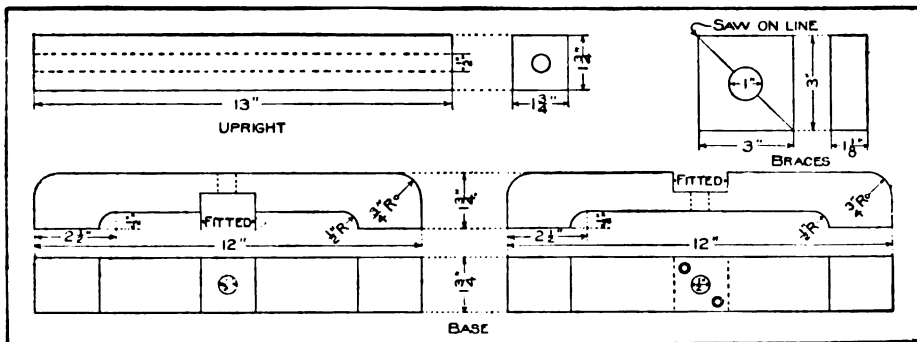
Details of Construction of Library Lamp Stand
