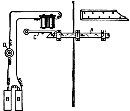
Simple Electric Lock
