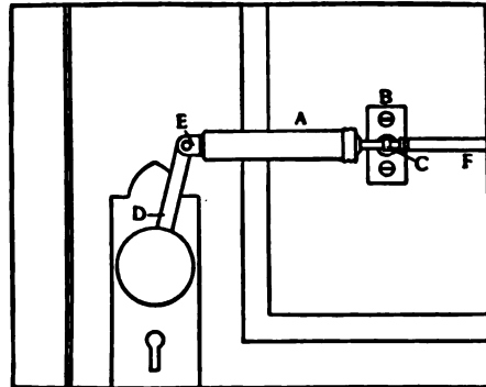
Pneumatic Door-Opener
