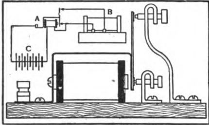
Interrupter for Induction Coil
