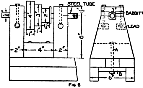
Fig. 6 Headstock Details
