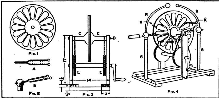
Details of a Homemade Static Machine
