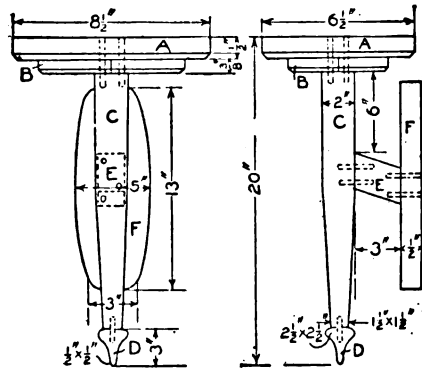
Details of the Wall Bracket
