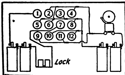
Wiring Diagram
