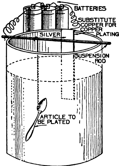
Electroplating Apparatus
