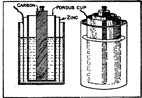
Cross Section and Completed Cell
