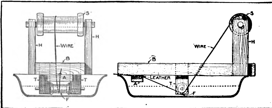
Home-Made Apparatus for Paraffining Wire
