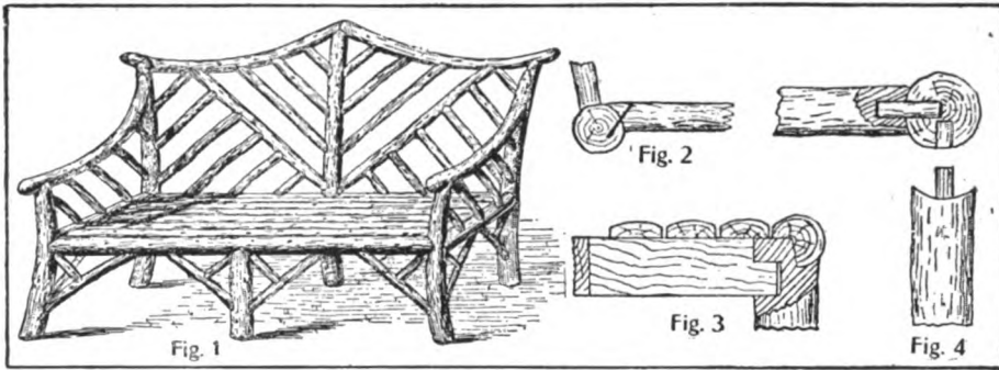
Rustic Seat and Details of Construction
