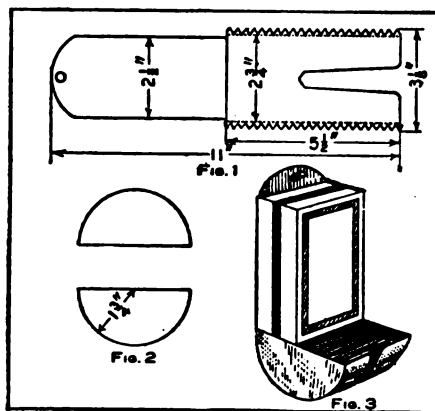
Details of the Match Safe
