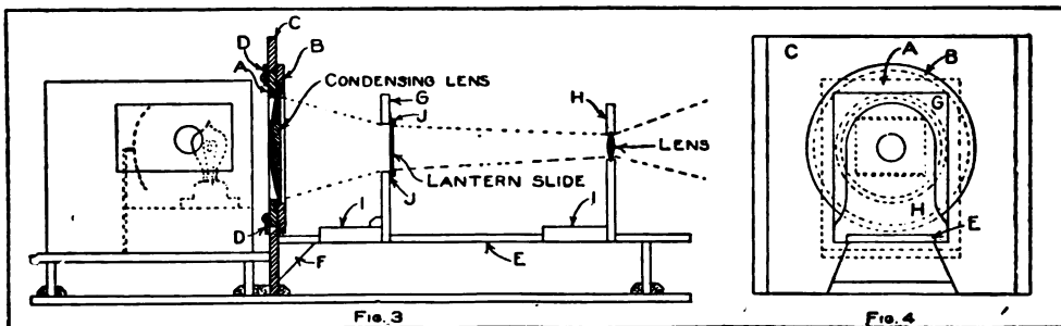
Magic Lantern Details
