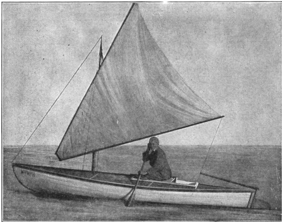
Completed Sailing Canoe
