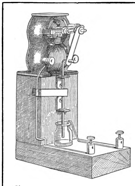
Motor-Driven Make-and-Break
