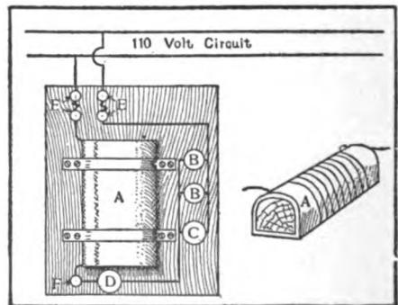
Electric Furnace
