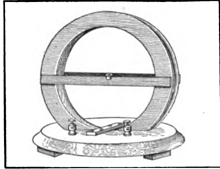
Tangent Galvanometer
