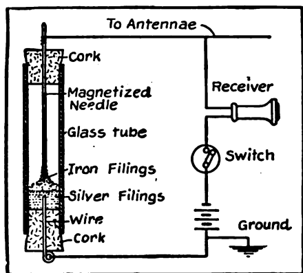
Detail of Coherer
