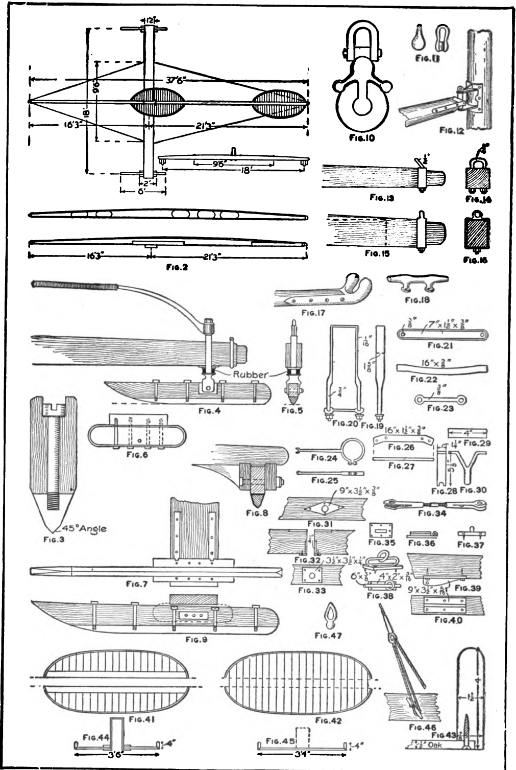
Details of the Ice-Yacht Parts
