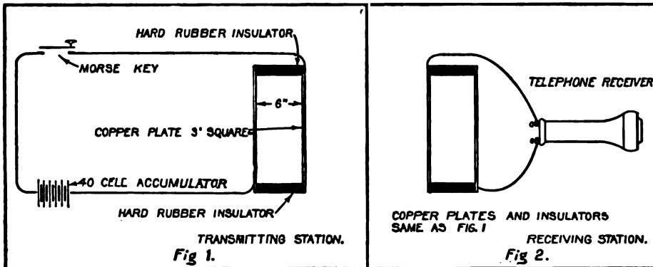
Simple Wireless System
