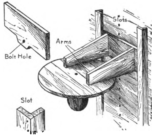
Adjustable Platform
