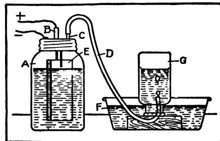
Hydrogen Generator
