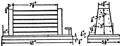
Detail of Toaster
