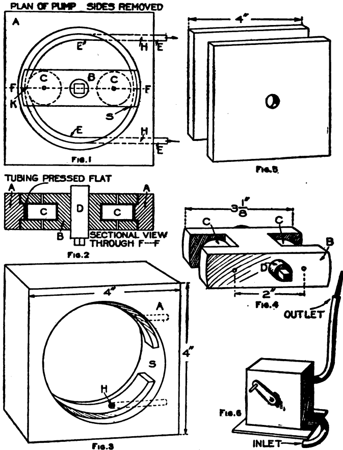
Details of Rotary Pump
