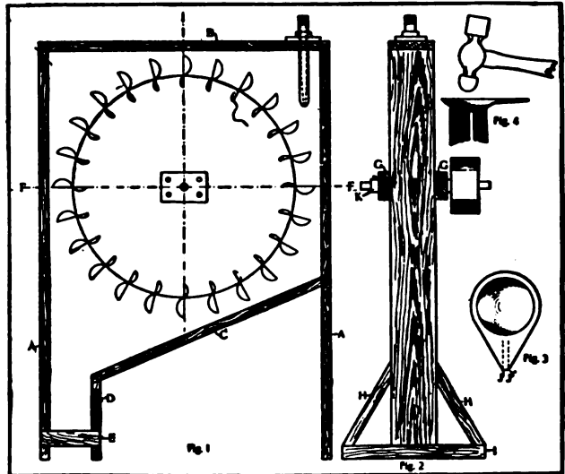
Detail of Homemade Waterwheel
