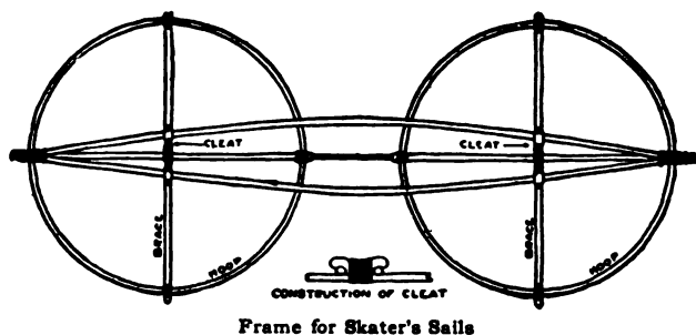
Frame for Skater's Sails
