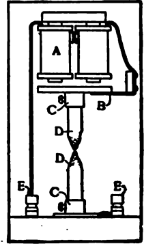
Arc Light
