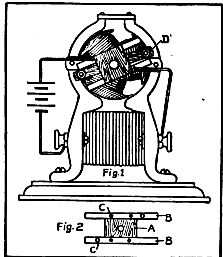
Direct-Connected Reverse
