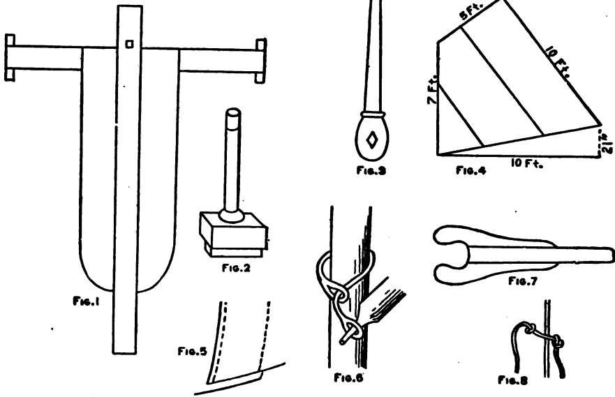
Details of Ice Boat Construction
