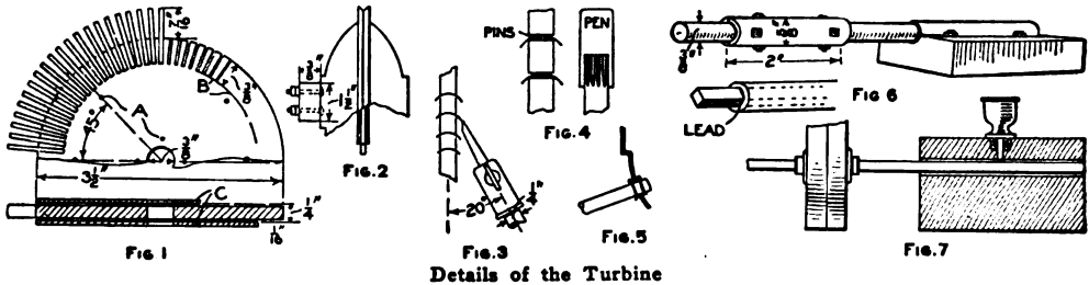
Details of the Turbine
