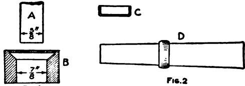
Tools for Forming the Ring
