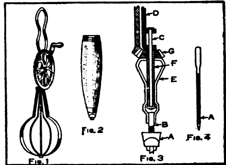
Details of Hand Drill Construction
