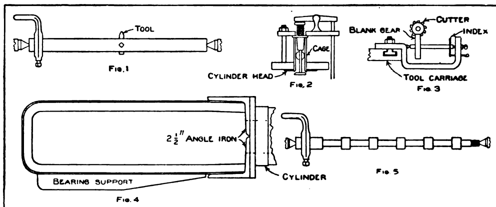
Steps in Making the Home-Made Gasoline Engine
