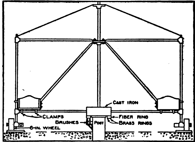
Details of the Swing
