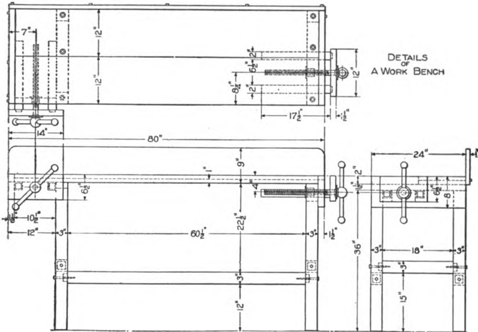
Detail of the Bench
