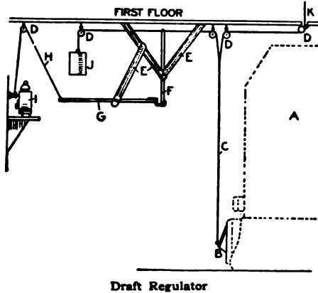
Draft Regulator
