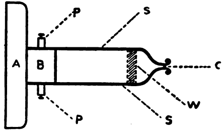
Simple Fire Alarm
