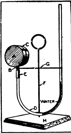
Air Thermometer
