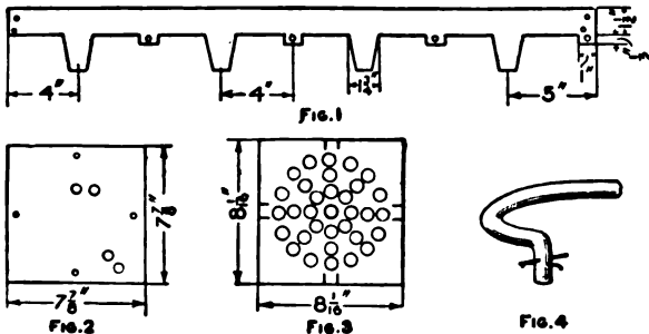
Pattern for Parts of the Electric Stove
