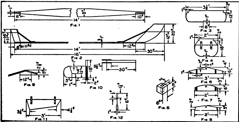
Details of a Home-Made Sailing Canoe
