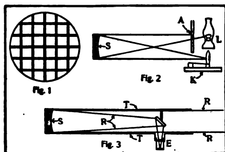
Detail of Telescope Construction
