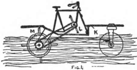
Fig. 1 Water Bicycle Complete
