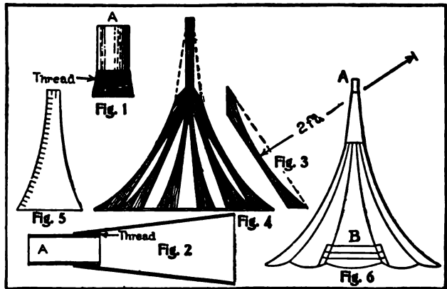
Detail of Phonograph Horn
