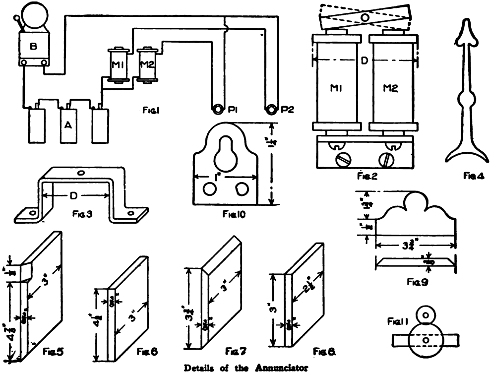
Details of the Annunciator
