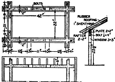
Concrete Forms
