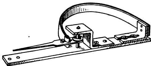
FIG. 13 Assembled Thermostat
