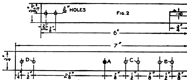
Couple and Mounting Strip
