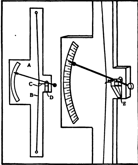
The Hygrometer
