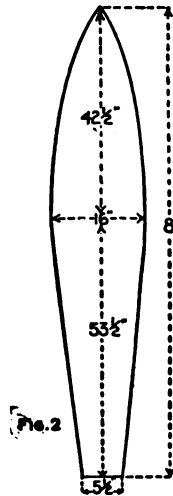
Fig. 2 Pattern and Parts to Make Balloon
