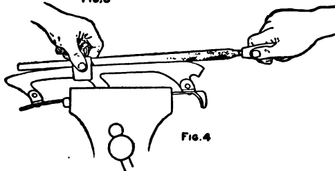
Filing a Curved Surface
