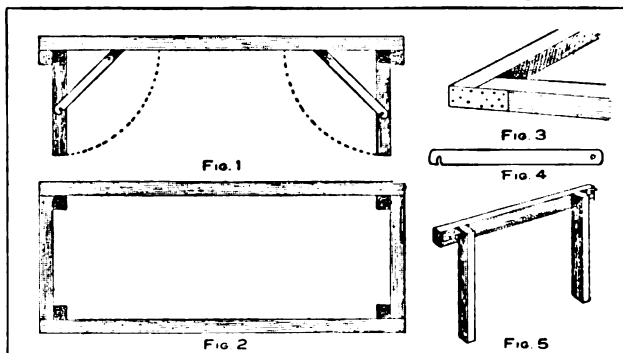
Details of Canvas Cot Construction
