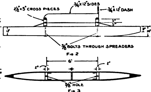
Details of the Pontoons
