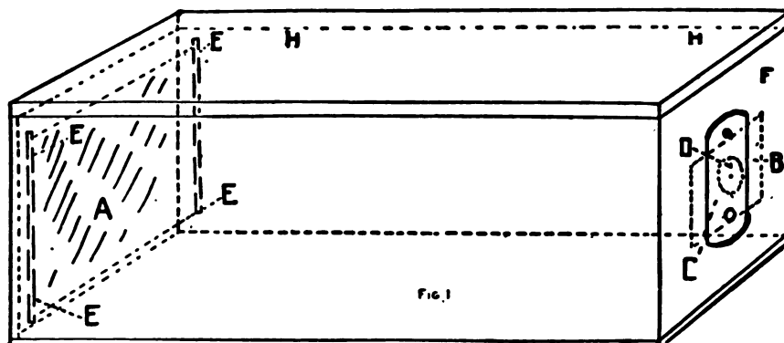
Construction of Camera Box
