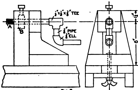
Fig. 7 Details of Tailstock
