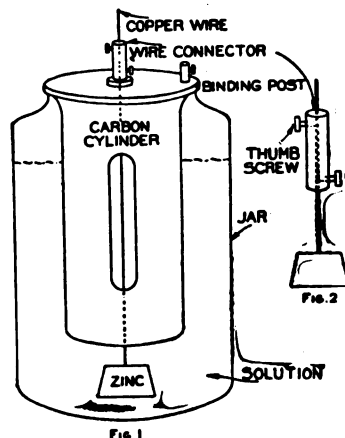
Fig. 1 Details of Homemade Battery
