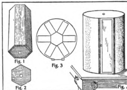
Phonograph Wax Record Case
