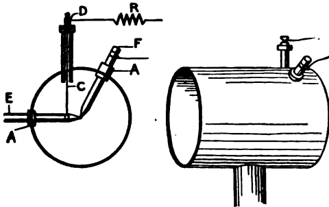
Arc in a Large Tin Can
