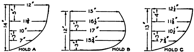
Fig. 1 Canoe and Molds Details
