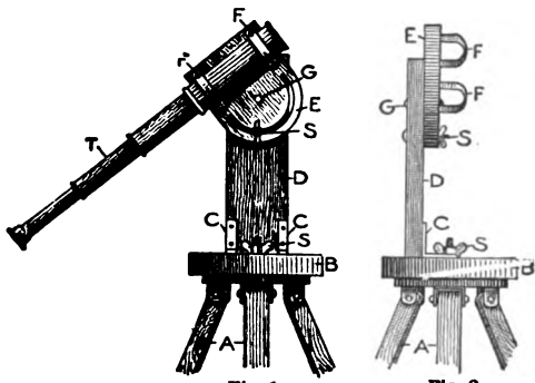
Fig. 1 Made of a Camera Tripod
