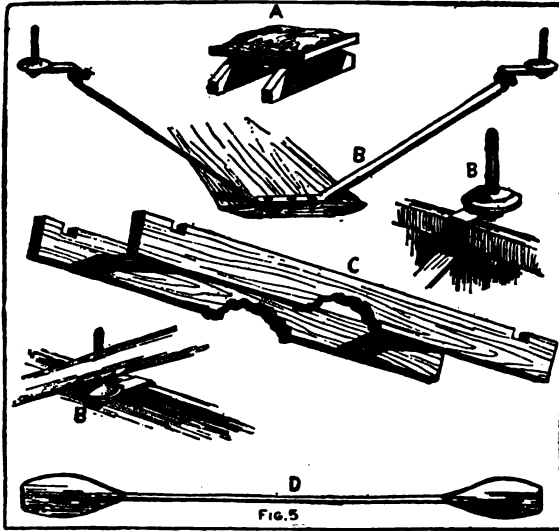
Fig. 5 Important Features of Construction
