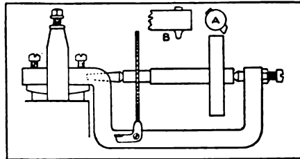
Gear-Cutting Attachment for Lathes
