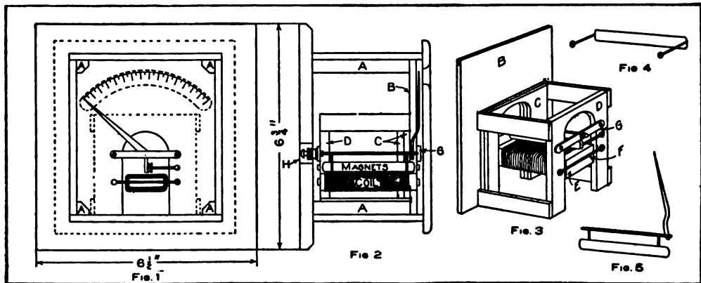
Details of an Ammeter
