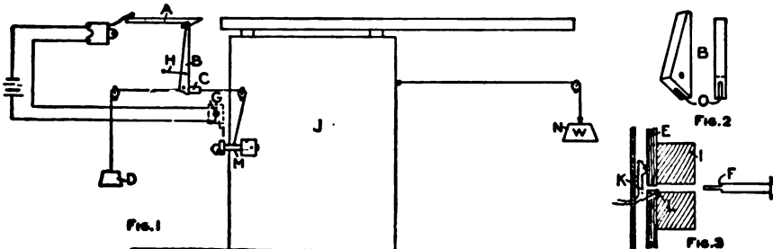
Electric Lock for Sliding Door
