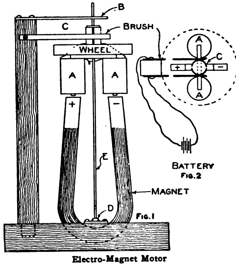
Electro-Magnet Motor
