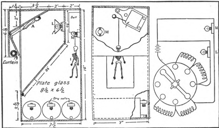
Construction of the "Pepper's Ghost" Illusion
