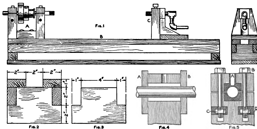
Assembled Lathe Bed and Bearing Details
