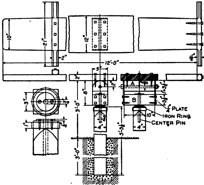
Details of Teeter Board
