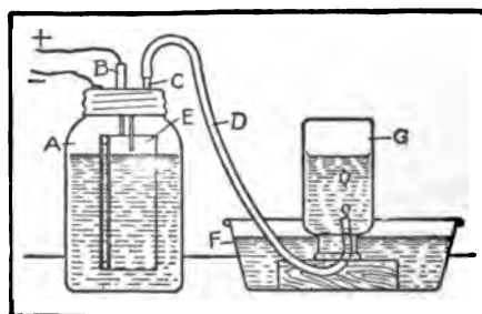
Hydrogen Generator
