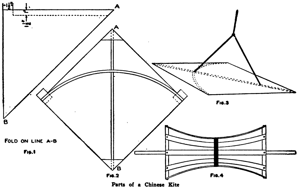
Parts of a Chinese Kite
