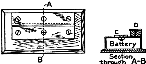
Lamp Tester
