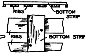
Construction of the Various Parts
