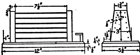
Detail of Toaster
