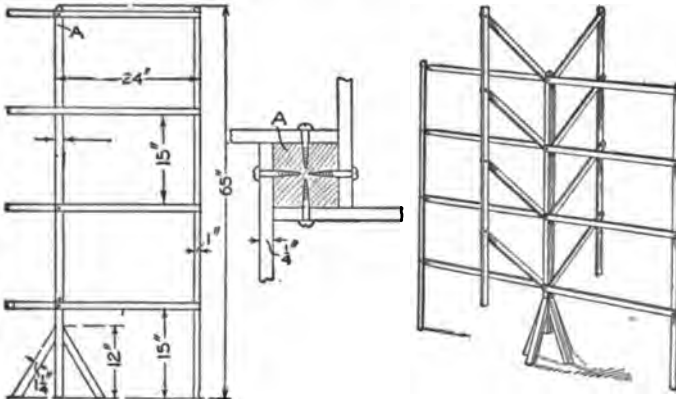
Folding Clothes Rack
