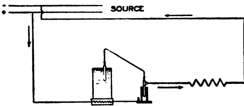
Wiring Diagram Showing How the Connections to a Source of Current Supply are Made
