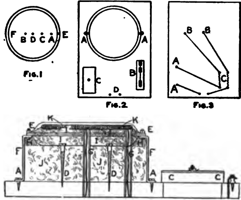
Fig. 4 Details of Electric Stove
