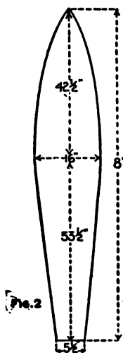
Pattern and Parts to Make Balloon
