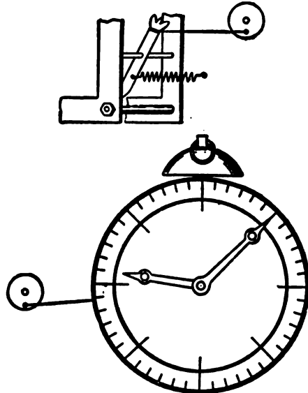
Revolution Recorder
