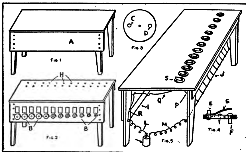
How the Electric Piano is Constructed
