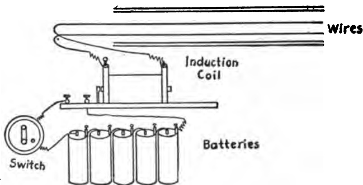
Electric Apparatus for Driving Away Cats
