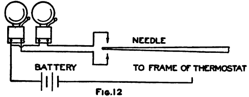
Wiring Diagram for One and Two Bells
