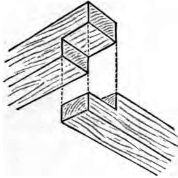
FIG. 21.—Fitting.
