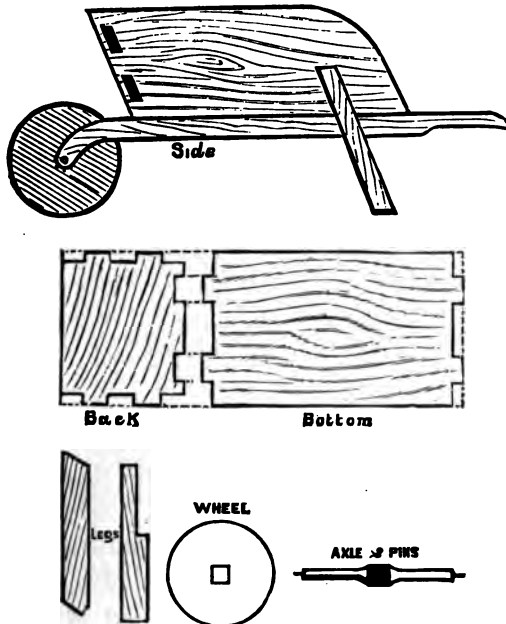
FIG. 69.—Wheelbarrow.
