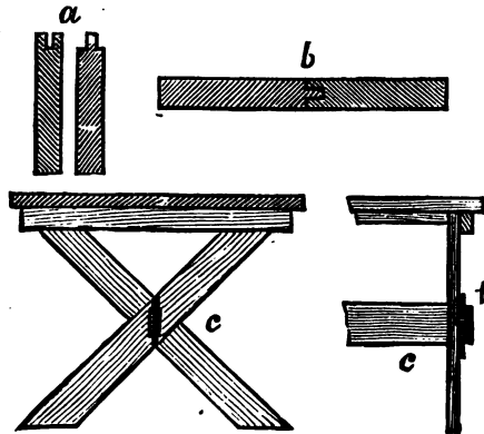
FIG. 51.—Summer-house Table.
