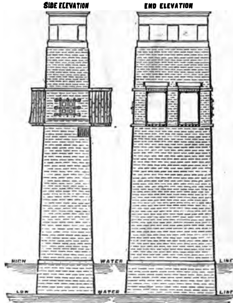
FIG. 98 a.—Land Tower.
