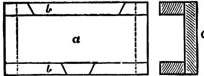
FIG. 89.—Plan of Mitre-box. a. Flat board; b. sides with cuts at angle of 45^\circ ; c. end plan of mitre-box.
