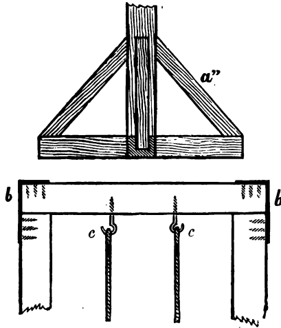
FIG. 47.—The Swing.
