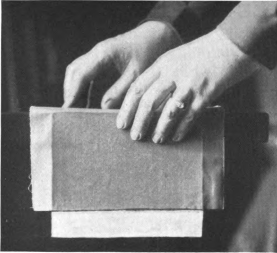
PLATE XXXV. An illustration of the method of covering the outside of the case when no block of wood is available.
