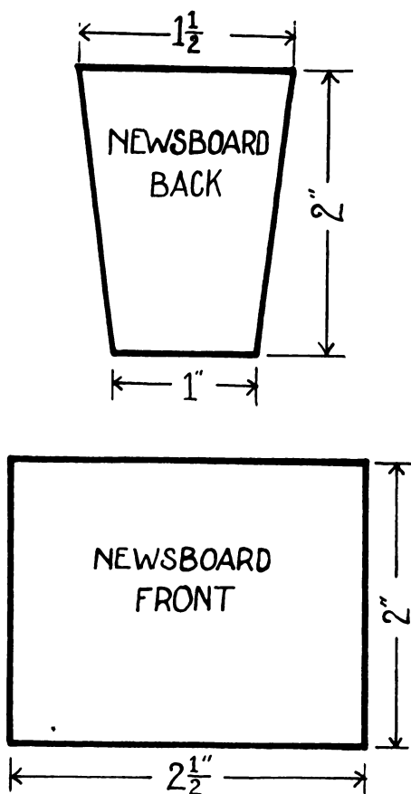
PLATE XX. The foundation pieces for an easel mount.
