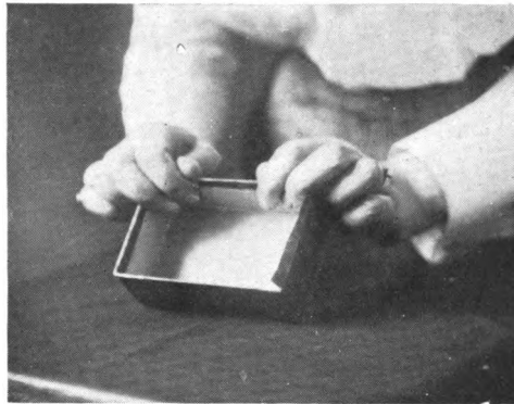
PLATE XXIX. Showing method of pasting the laps to the inside of the box.
