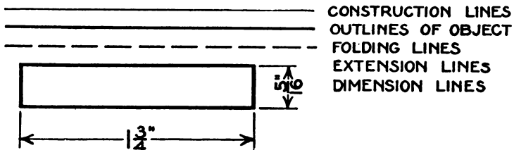
PLATE II. Line Conventions.
