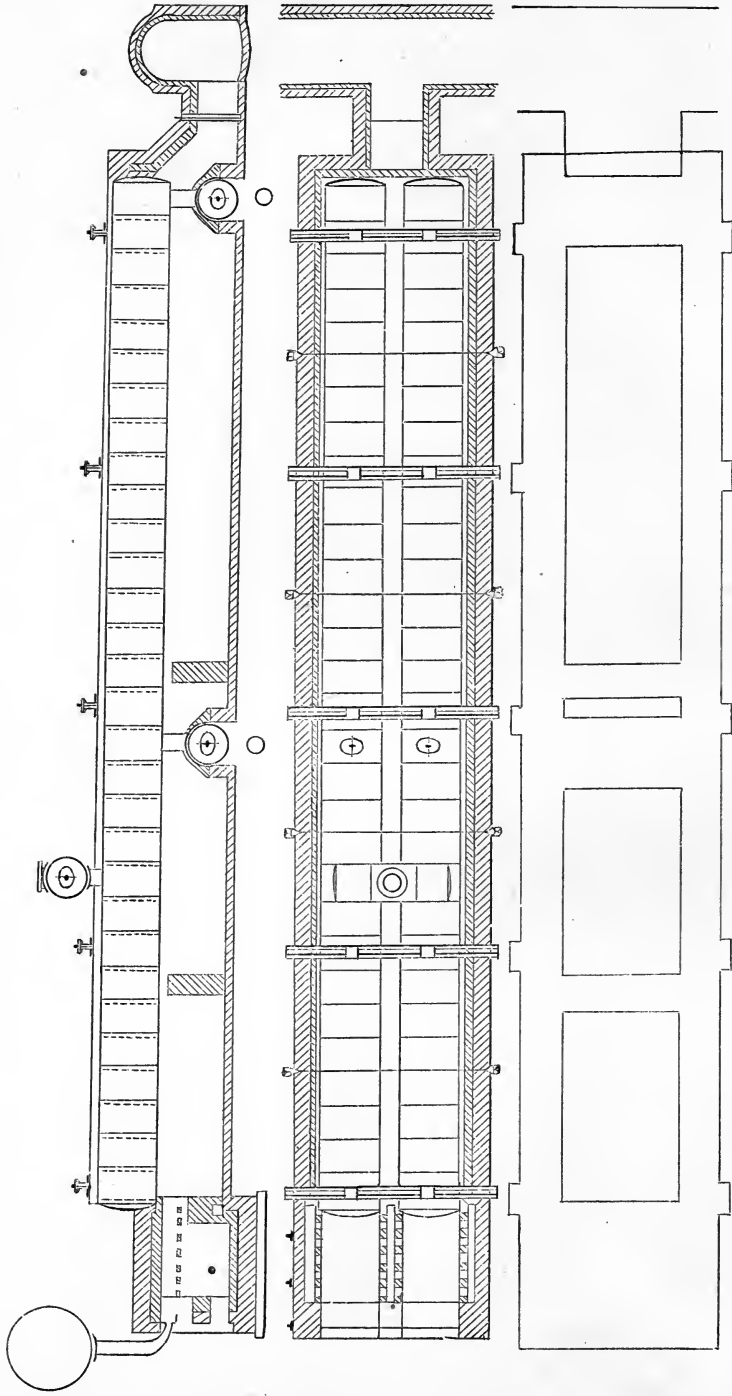
BOILERS OF THE MEIER IRON CO., NEAR ST. LOUIS, MO.
