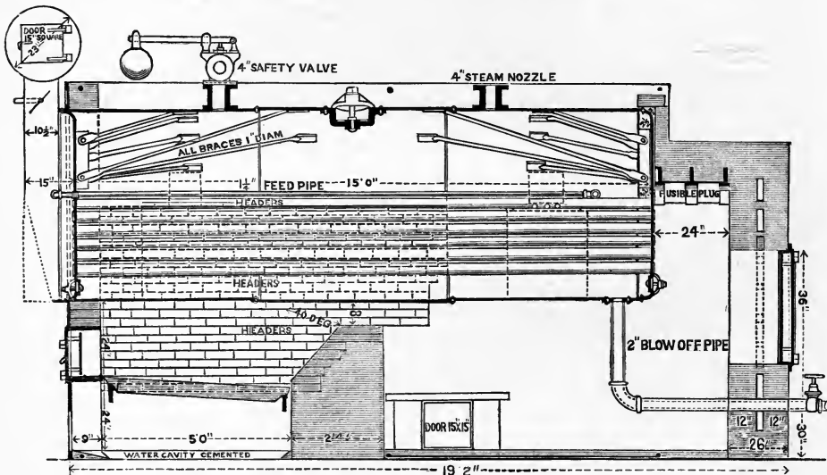
SECTIONAL ELEVATION.
