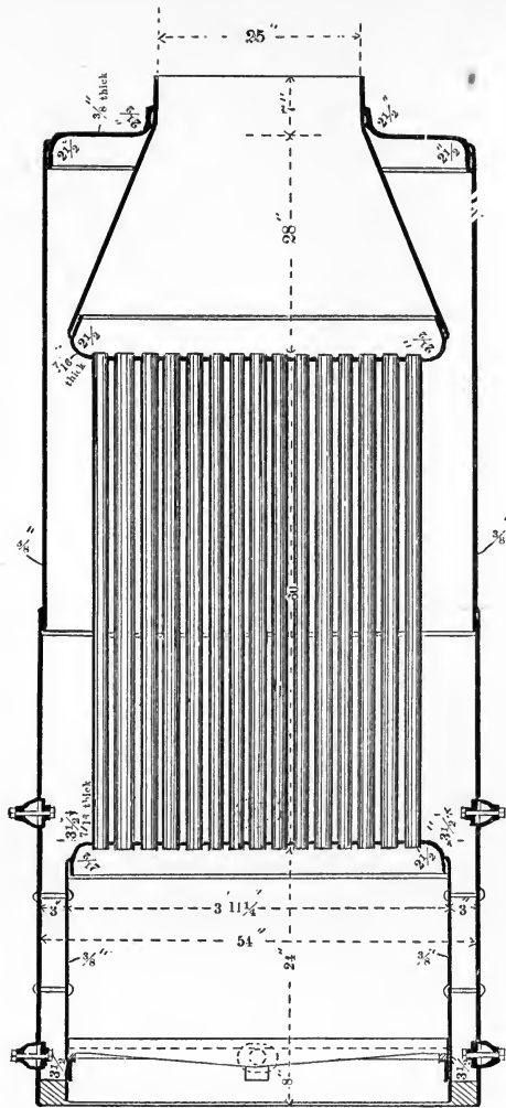
SECTIONAL ELEVATION.
