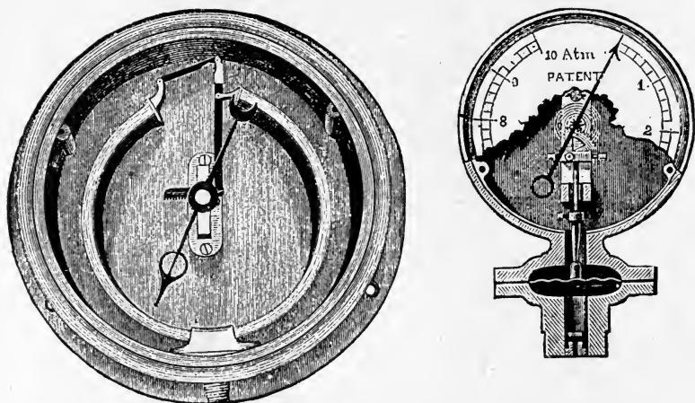
STEAM GAUGES.
