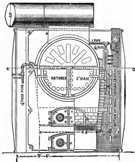
TRANSVERSE VIEWS.
