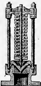
ORDINARY SAFETY VALVES.
