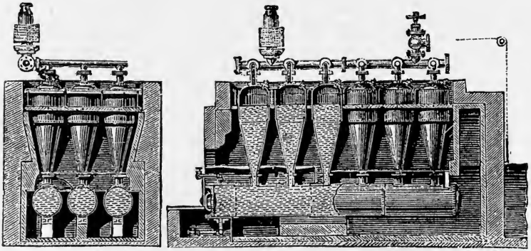
SHEPHERD'S BOILER.
