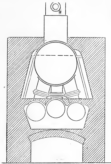
TRANSVERSE SECTION.
