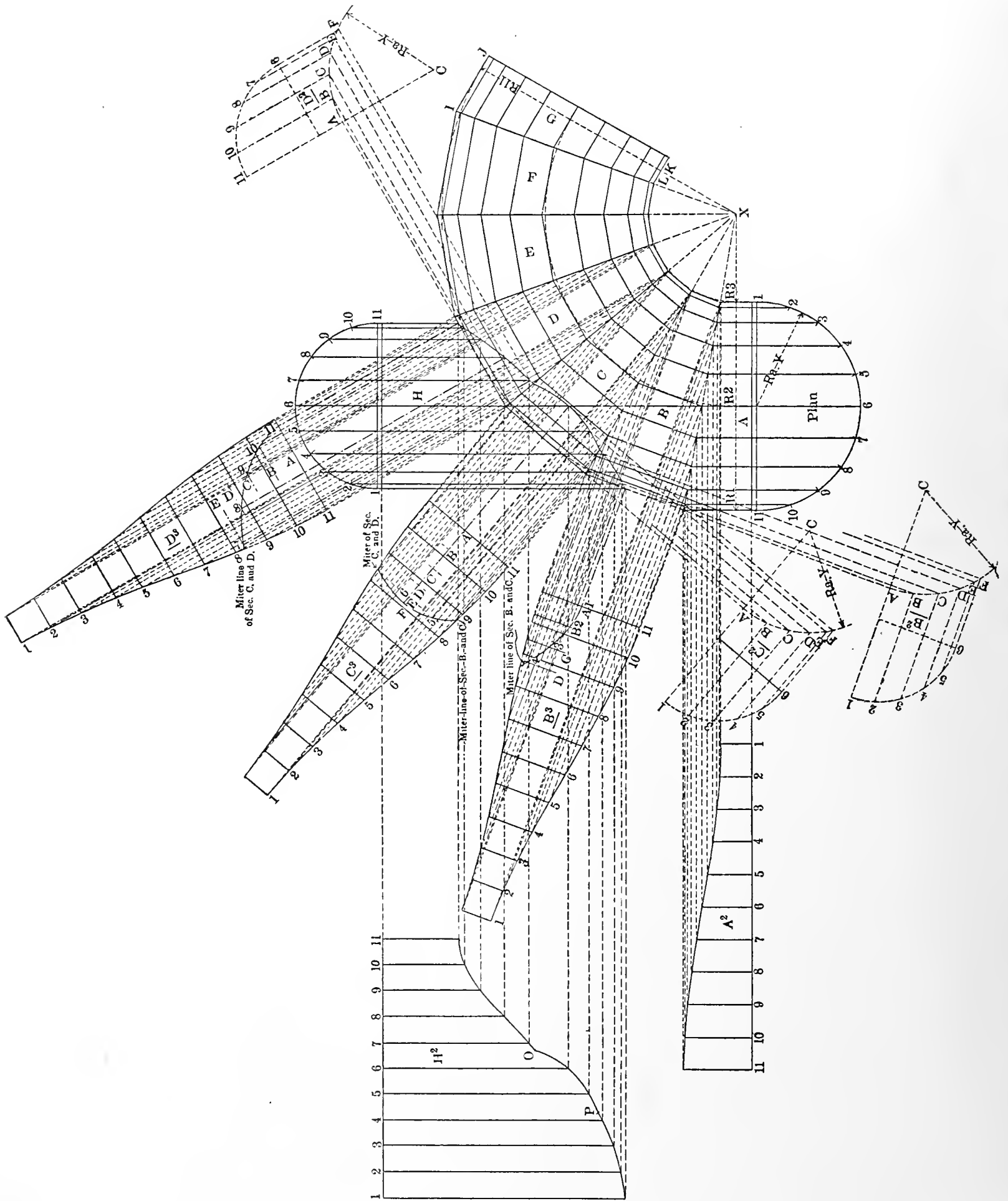
SIDE ELEVATION AND PATTERNS FOR A CYLINDER INTERSECTING AN ELBOW.
