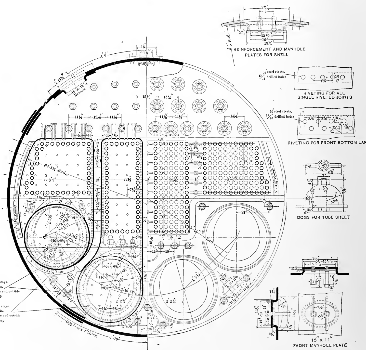
HALF CROSS-SECTIONS AND DETAILS OF TUBES, MANHOLES AND HANDHOLES OF A MODERN, FOUR-FURNACE, SINGLE-ENDED SCOTCH BOILER, 16 FEET 6 INCHES DIAMETER BY 10 FEET 4 INCHES LONG.
