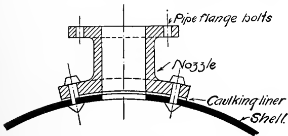
FIG. 5.—STEAM NOZZLE.
