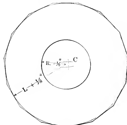
FIG. 3 Dome Ring Before Being Flanged
