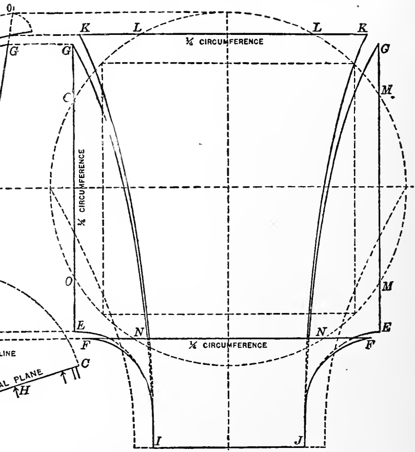
FIG. 2.—FRONT VIEW OF COWL, SHOWING THE WORKING POINTS IN THE PATTERN SHEET.
