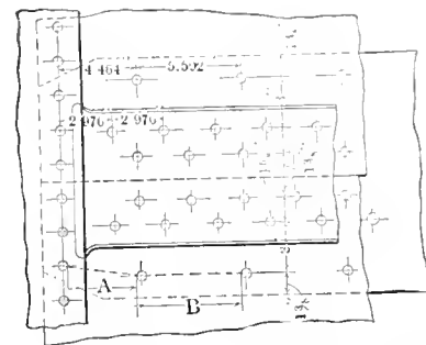
FIG. 49.—DETAIL OF SEAM SHOWN IN FIG. 52.
