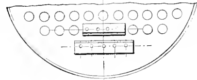
FIG. 50.—DETAIL OF BRACING ON LOWER PART OF BACK HEAD.
