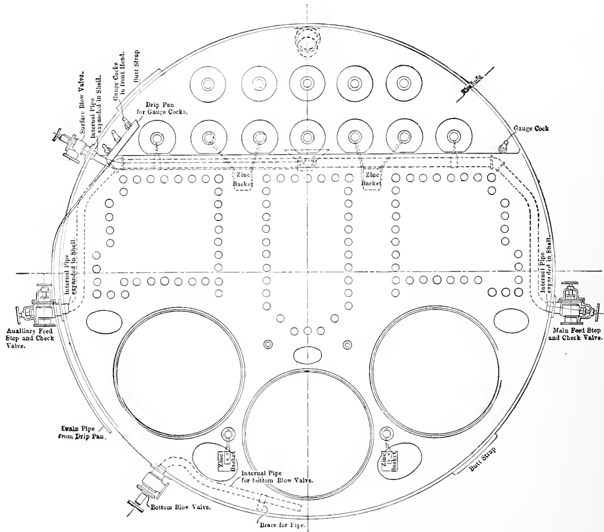
FIG. I.—END ELEVATION.
