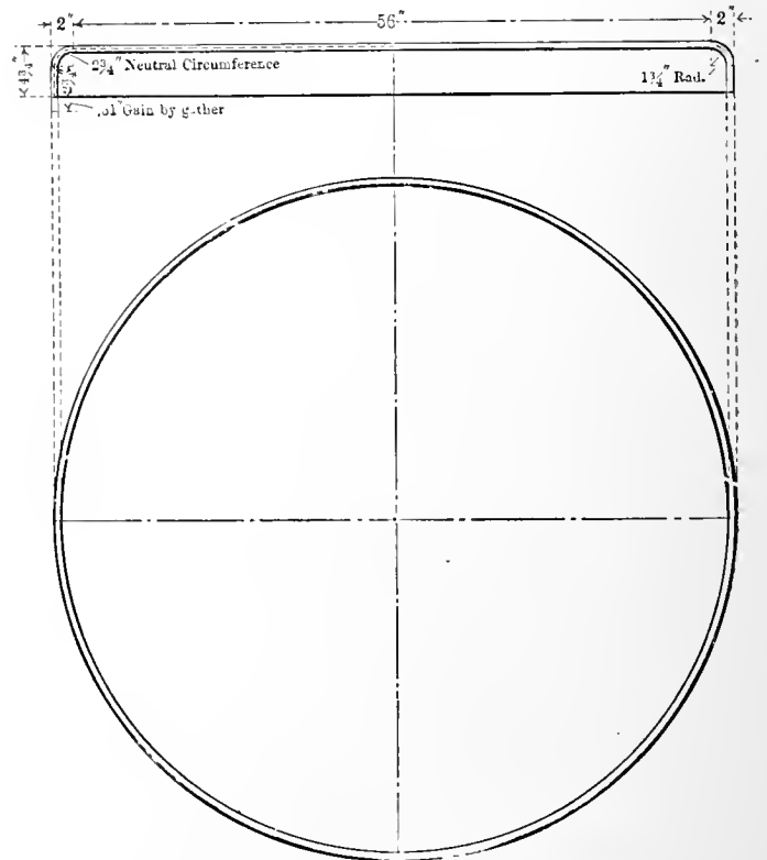
FIG. 13.—PLAN AND ELEVATION OF HEAD.
