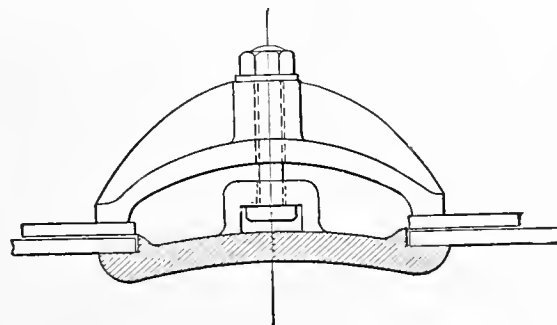
FIG. 44.—MANHOLE REINFORCED WITH STEEL LINER PLATE.
