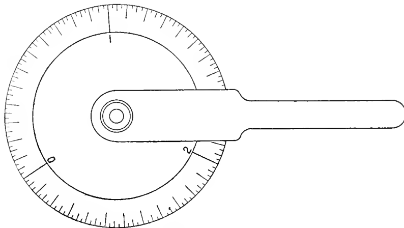
FIG. 2.—MEASURING WHEEL.
