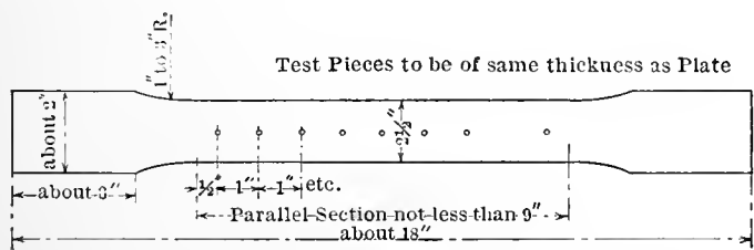
FIG. 14.—STANDARD TEST PIECE FOR BOILER PLATE.
