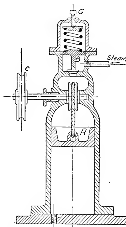
FIG. 16.—SECTIONAL VIEW OF DAMPER REGULATOR.
