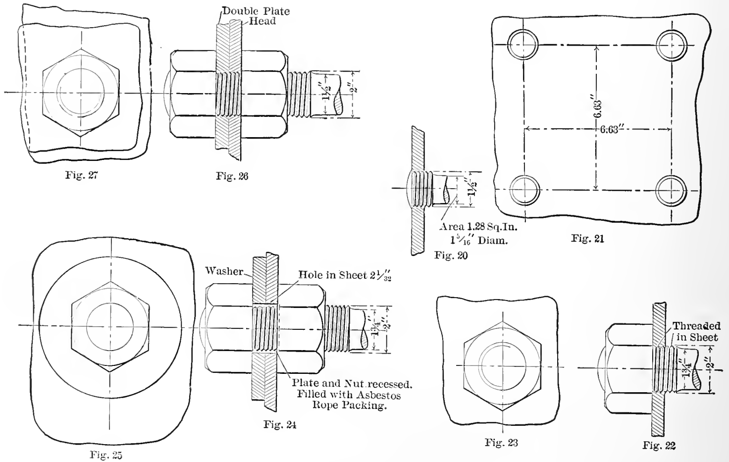
METHODS OF FASTENING DIRECT STAYS.
