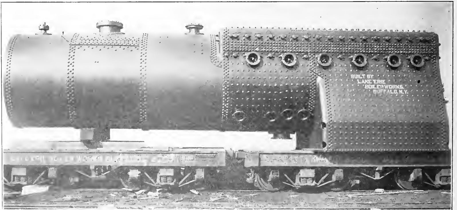
A LARGE STATIONARY BOILER OF THE BELPAIRE LOCOMOTIVE TYPE, BUILT TO SUPPLY STEAM AT HIGH PRESSURE FOR HIGH-DUTY PUMPING ENGINES: TOTAL WEIGHT OF BOILER 75 TONS. LENGTH, 33 FEET 7 INCHES; DIAMETER, 90 INCHES; TWO FURNACES EACH 10 FEET 6 INCHES LONG BY 4 FEET 6 INCHES WIDE; 201 3-INCH TUBES; HEATING SURFACE, 3,032 SQUARE FEET; GRATE AREA, 68\frac{3}{4} SQUARE FEET; RATIO, 44:1.
