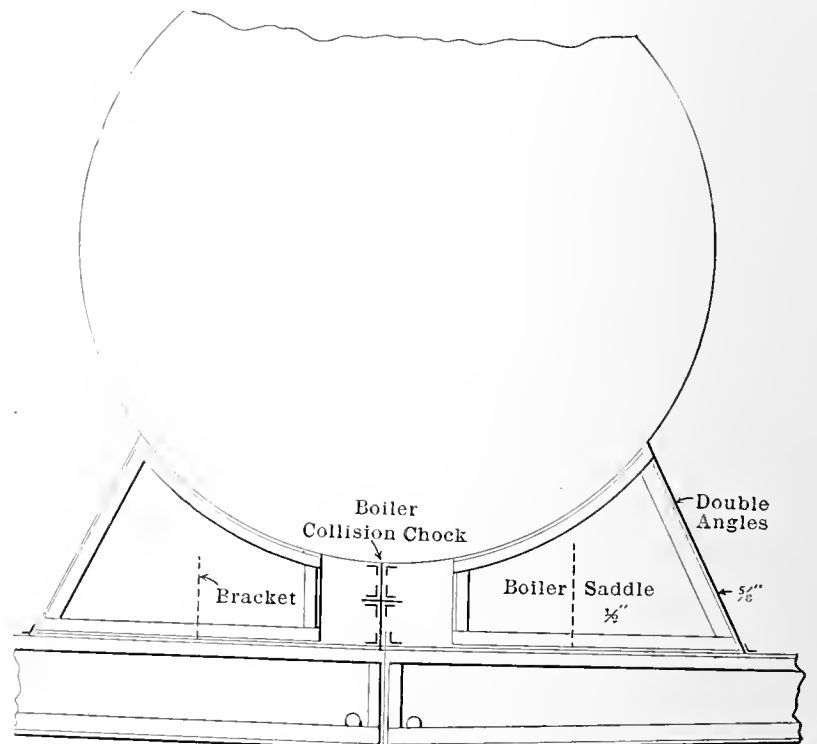
ORDINARY TYPE OF SADDLE FOR SCOTCH BOILER.
