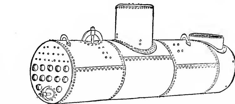
THE SIX INCH FLUE BOILER. FIG. 20.
