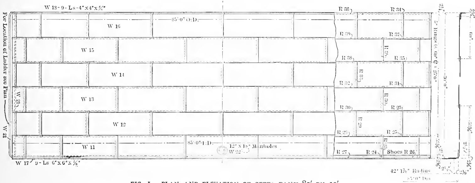
FIG. I.—PLAN AND ELEVATION OF STEEL TANK 85' BY 30'.
