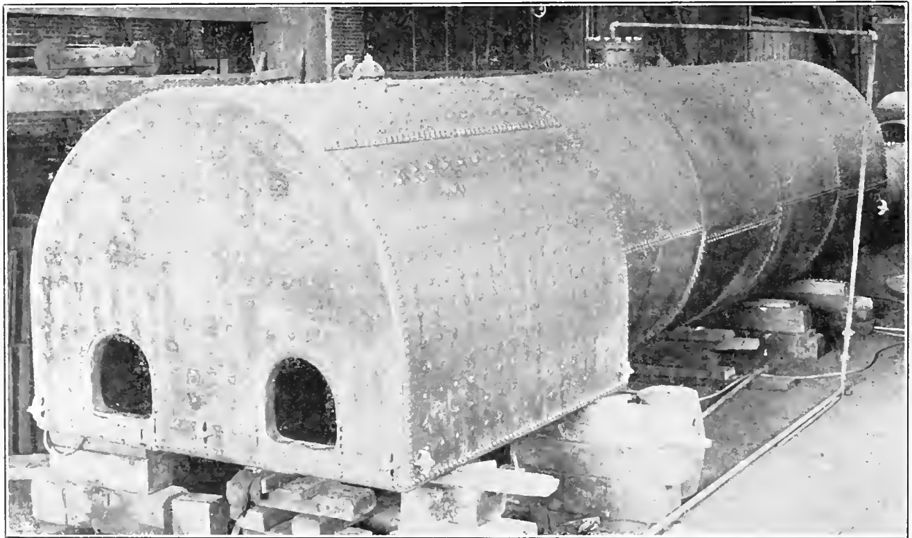
A LOBSTER BACK RETURN FLUE MARINE BOILER, 8 FEET 9 INCHES DIAMETER BY 33 FEET LONG, CONSTRUCTED WITH TWO FURNACES AND THREE COMBUSTION CHAMBERS: TWO FLUES, 24 INCHES DIAMETER; TWO FLUES, 13 INCHES DIAMETER, AND 68 TUBES, 3 INCHES DIAMETER BY 16 FEET LONG; STEAM PRESSURE, 55 POUNDS PER SQUARE INCH
