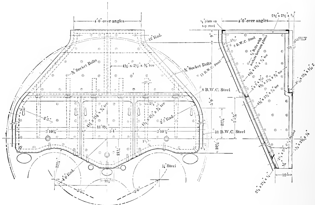
ARRANGEMENT OF UPTAKES.
