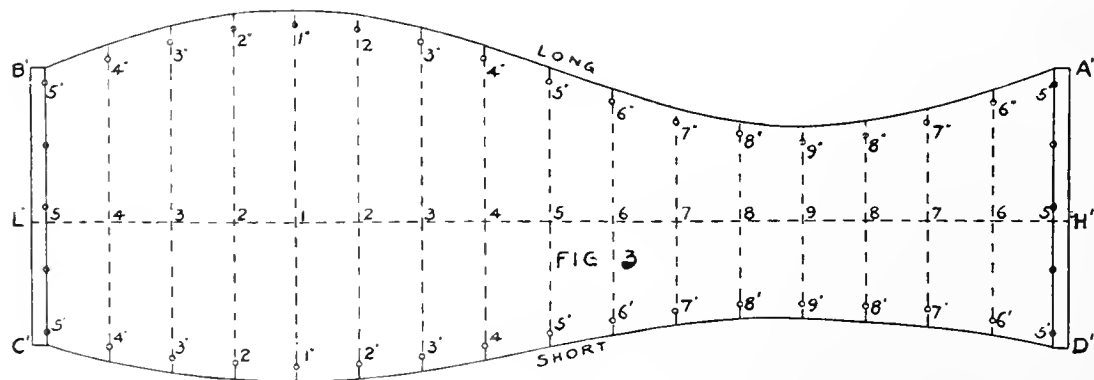
LAYOUT OF FOUR-PIECE 90-DEGREE ELBOW.
