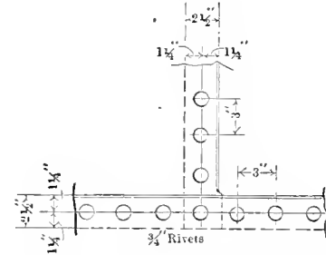
FIG. 6.—DETAIL OF RIVETING OF TOP RINGS.
