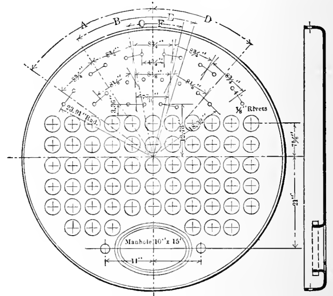
FIG. 47.—LAYOUT OF FLUES AND BRACES.
