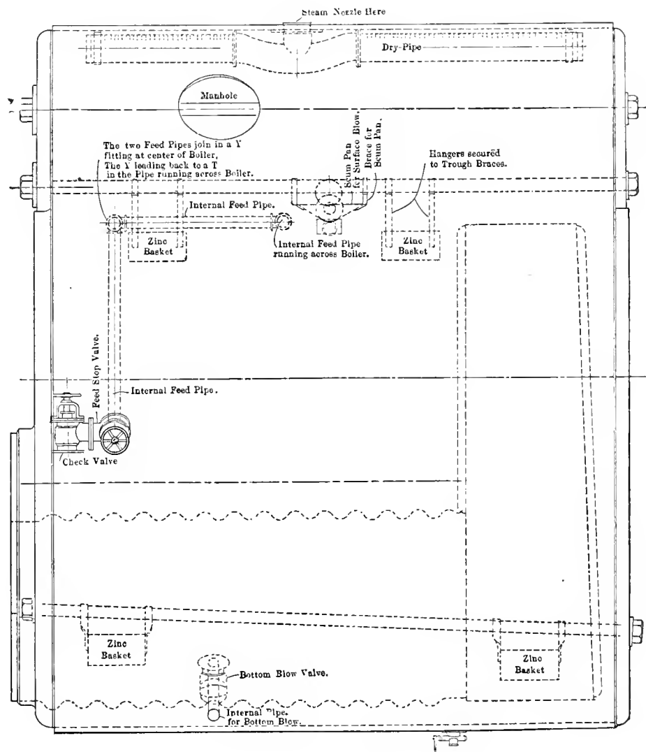
FIG. 2.—SIDE ELEVATION.
