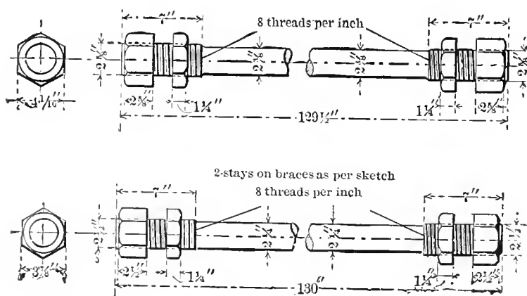
FIG. 12.—STAYS OR BRACES AS PER SKETCH.
