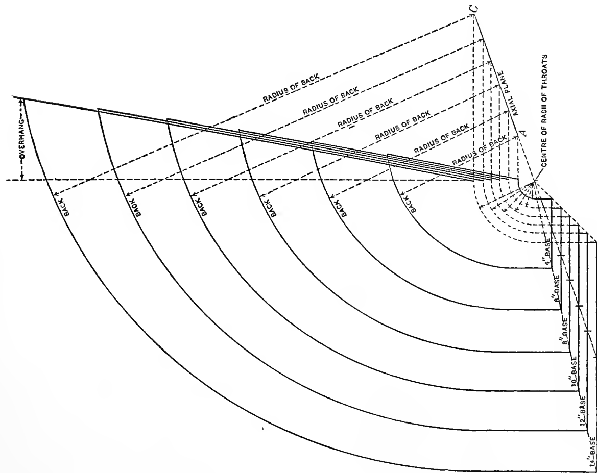
FIG. 3.—GROUP OF SIX COWLS.
