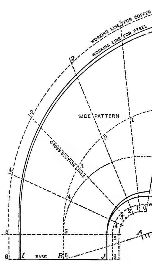
FIG. 1.—SIDE VIEW OF COWL, SHOWING METHOD OF OBTAINING THE SIDE PATTERNS.
