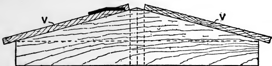
Fig. 24.—Beehive Roof Wings.
