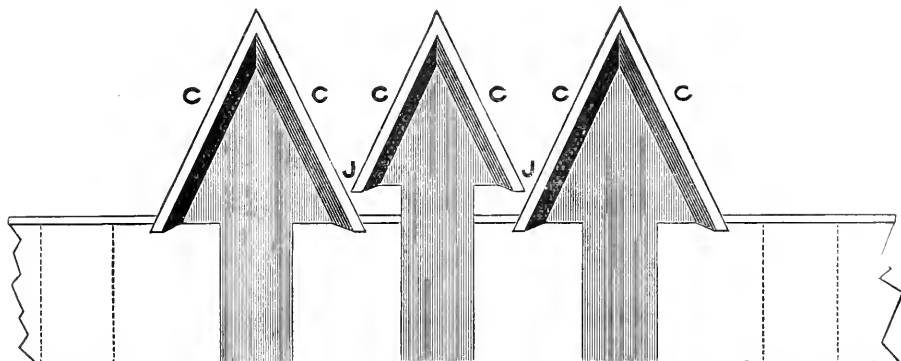
C, RAISED CUTTING EDGES. J, BROKEN JOINT SHOWING HOW ONE CUTTER CLEARS BEHIND THE NEXT.
