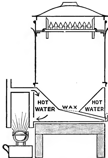
No. 2—The Practical Uncapper, with circulating heater for disposing of the cappings at same time.
