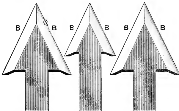
BACKS OF CUTTERS SHOWING B, THE BEVELLED EDGES, AND EXACT RELATIVE SITUATIONS.
