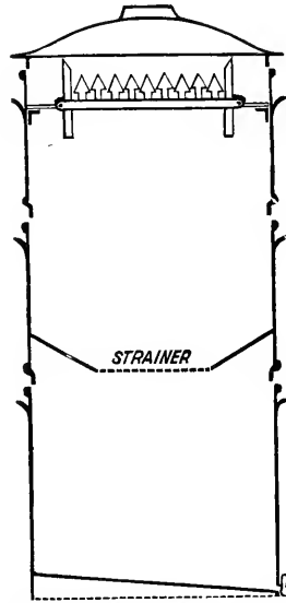
CROSS-SECTION OF NO. 1 UNCAPPER.
