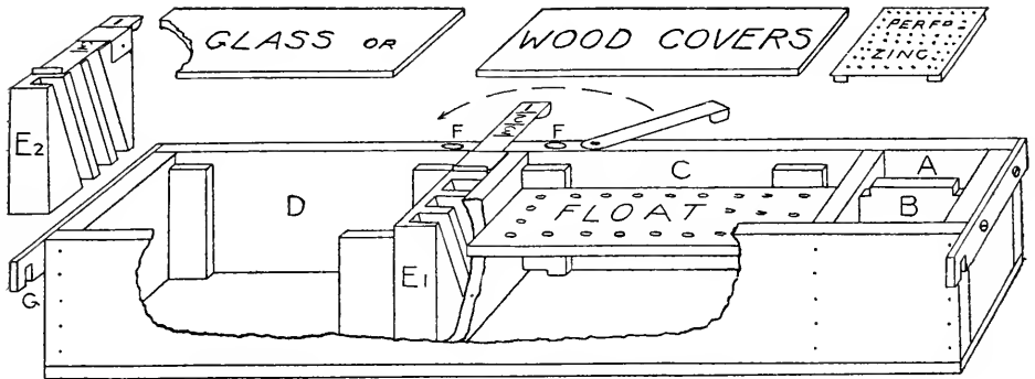
IMPROVED FLOORBOARD FEEDER.
