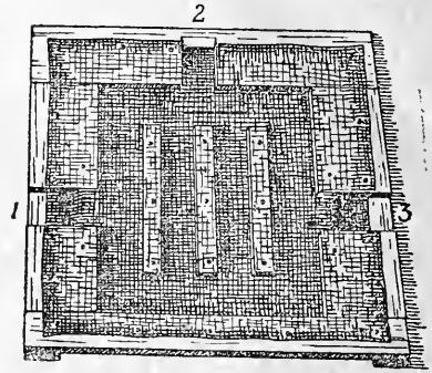
Fig. 6.—Floor for three nuclei in upper story.
