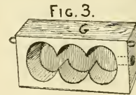
TOP VIEW OF COVER.—G, food feeder.
