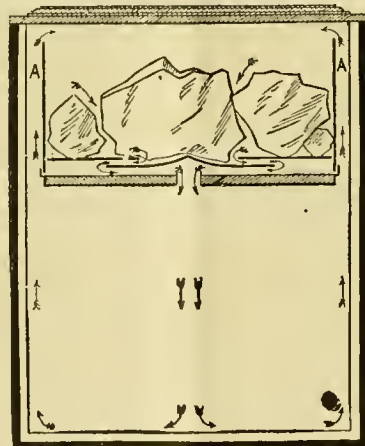
Refrigerator—Showing Air-Currents.
