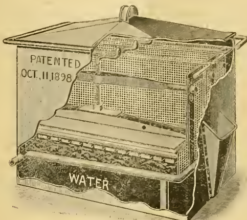
A Three-Basket Wax-Extractor.
