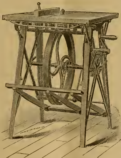
Combined Scroll and Circular Saw.
