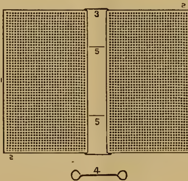
1, 1. Two lids of equal size, made of light galvanized wire-netting. 2, 2. The outside bound by tin. 3, 3. A wire to hold the lids together, and likewise serve as a hinge between the two. The two stems (3) are about an inch apart and connected. Where inside cloth of the wire is used, different hinges must be used, such as 4, to be placed at 5.
