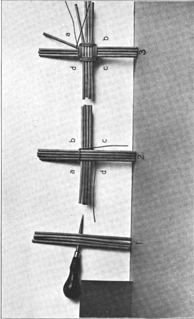
FIGURE III. FOUR-SPOKED BASE
