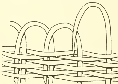
Detail of Edge of Basket
