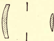
FIG. 101a.—Airy and Mittenzuey Ocular.
