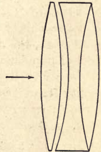
FIG. 18.—Peter Dolland's Triple Objective.
