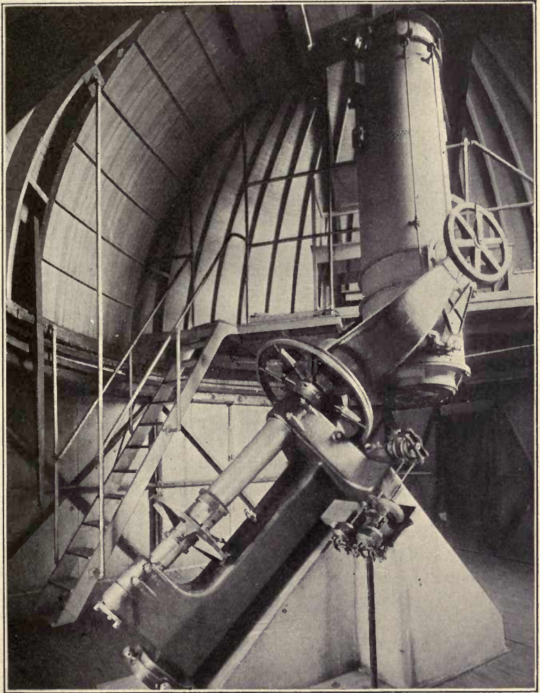
FIG. 139.—Gerrish Drive on 24 inch Reflector.
