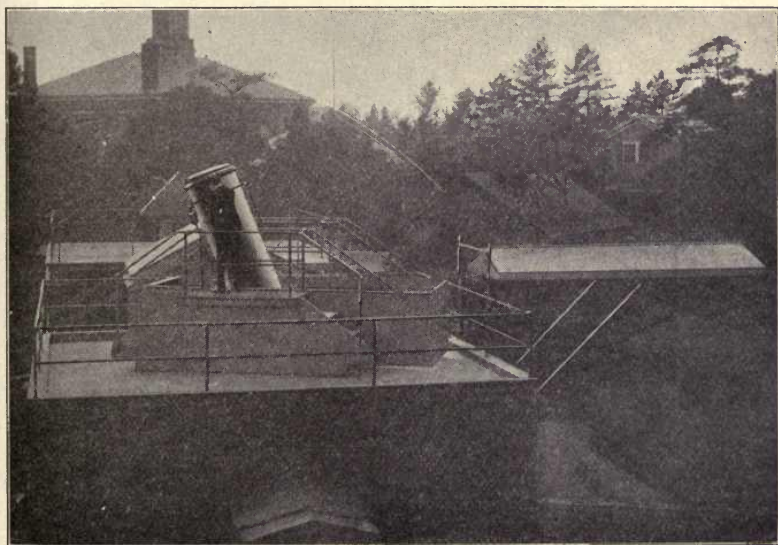
Fig. 178.—Turret Housing of the 24-inch HARVARD Hewitt Reflector.
