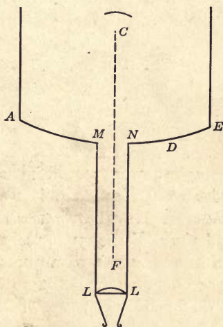
FIG. 12.—Gregory's Diagram of his Telescope.
