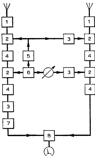
Fig. 35. Spectral harmonic interferometer for determining the presence of coherent harmonics
