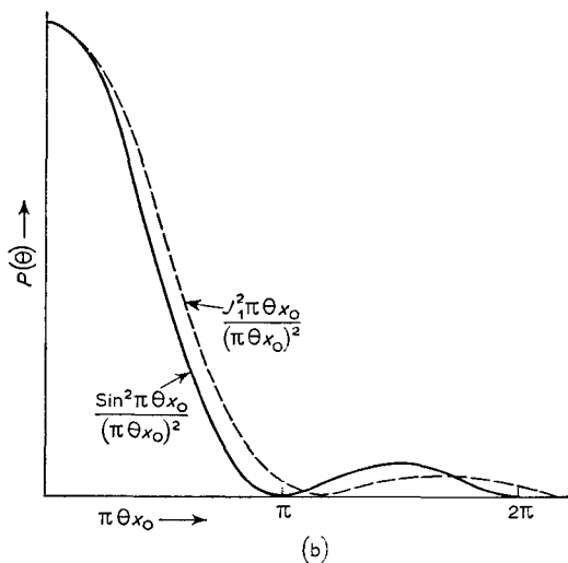
Fig. 21. Directivity patterns of a rectangular telescope aperture (full line) and a circular aperture (dotted) (a) amplitude (b) intensity
