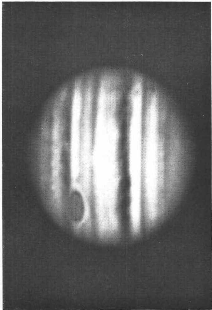
Plate 7. The planet Jupiter showing the giant Red Spot (By courtesy of the Mount Wilson and Palomar Observatories)
