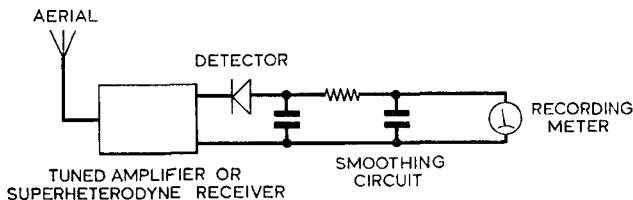
Fig. 2. A simple radio astronomy receiver
