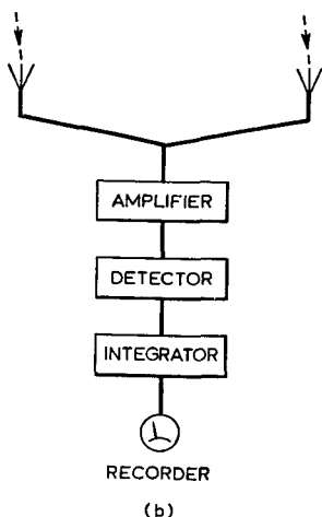
Fig. 4. The Michelson stellar interferometer (a) optical technique (b) radio analogue
