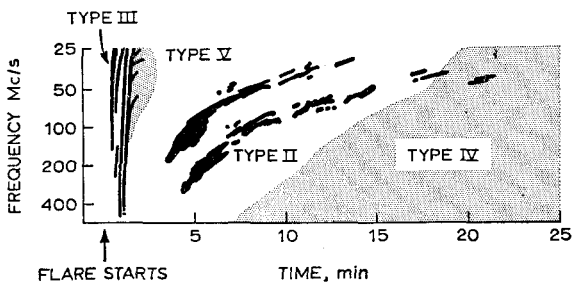
Fig. 12. Idealized dynamic solar spectrum following an outburst (After J. P. Wild)
