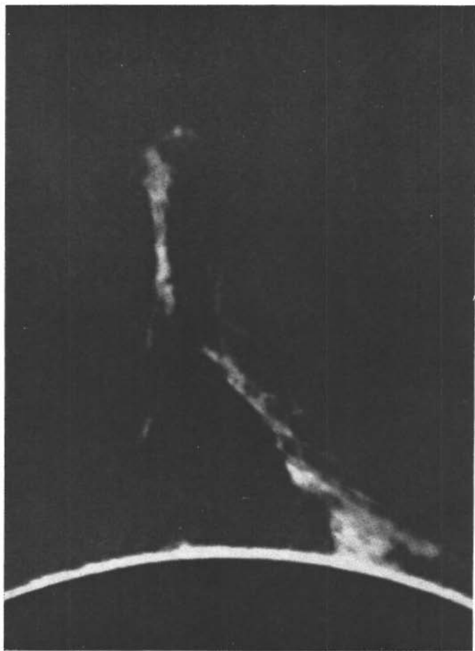
Plate 6. A solar outburst (By courtesy of the Mount Wilson and Palomar Observatories)
