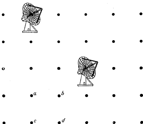
Fig. 23. Aperture synthesis. The combination of readings from different spacings synthesizes the survey that would be obtained with an aerial covering the whole area. Not all possible pairs of readings need be taken— ab is the same as cd and ac the same as bd
