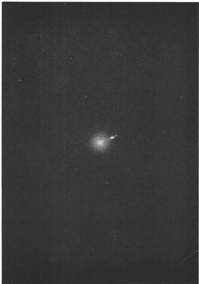
Plate 11. The galaxy associated with the radio source Virgo A. The blue jet pointing outwards from the centre emits polarized light consistent with synchrotron radiation. The radio source envelops the whole nebula. (Lick Observatory Photograph)
