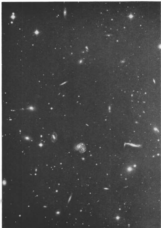
Plate 2. A cluster of extra-galactic nebulae in Hercules (By courtesy of the Mount Wilson and Palomar Observatories)
