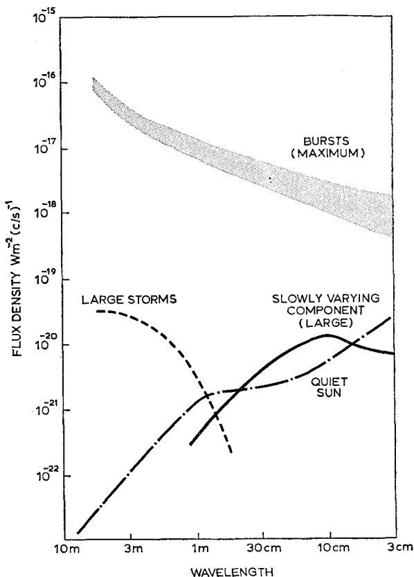
Fig. 11. The spectra of the active Sun (After J. P. Wild)
