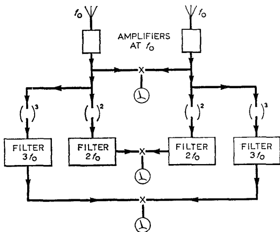
Fig. 34. No increase of resolving power is obtained with this harmonic interferometer
