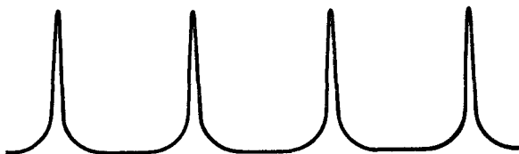
Fig. 14. The waveform from a single electron orbiting at a high speed in a magnetic field. The peaks become sharper if the speed of the electron approaches closer to that of light. In most astronomical contexts only a single pulse may be received from each electron
