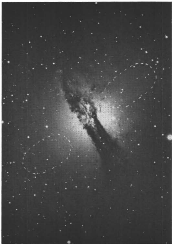
Plate 10. The galaxy NGC 5128 in Centaurus showing the two central components of the radio source (Superimposed on Mount Wilson and Palomar Observatories photograph)
