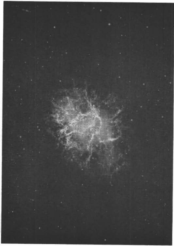
Plate 8. The Crab Nebula in Taurus, remnants of the Supernova of 1054 (By courtesy of the Mount Wilson and Palomar Observatories)
