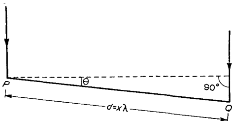
Fig. 27. Ray paths applicable to dispersion
