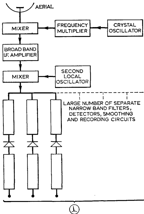
Fig. 7. Simple multi-channel hydrogen line spectrometer receiver
