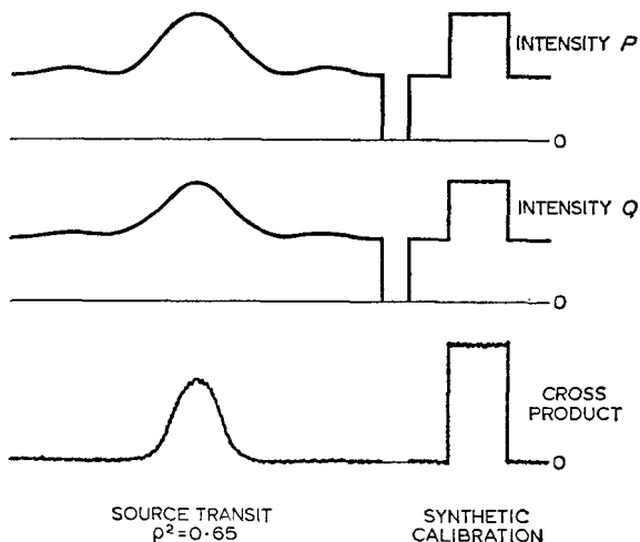
Fig. 32. The output of the intensity interferometer. The upper two traces show the outputs of the separate channels and the lower trace shows the cross product. The bump from the source on the left shows a correlation coefficient of 65 per cent by comparison with the unity correlation of the synthetic signal appearing as a rectangle on the right
