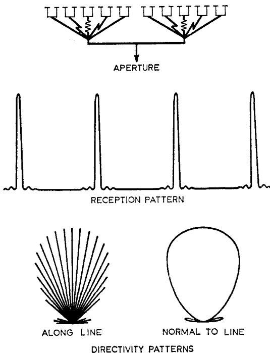
Fig. 36. Christiansen's radio analogue of the diffraction grating. The zig-zag lines in the upper diagram represent equal lengths of feeders
