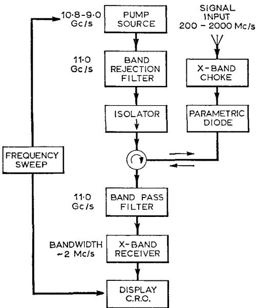
Fig. 9. An Australian solar spectrometer with large dynamic range (200 to 2000 Mc/s). A moving film is passed in front of the cathode-ray oscilloscope (c.r.o.) in order to obtain a permanent record of the variations at different frequencies as a function of time, as in Fig. 12
