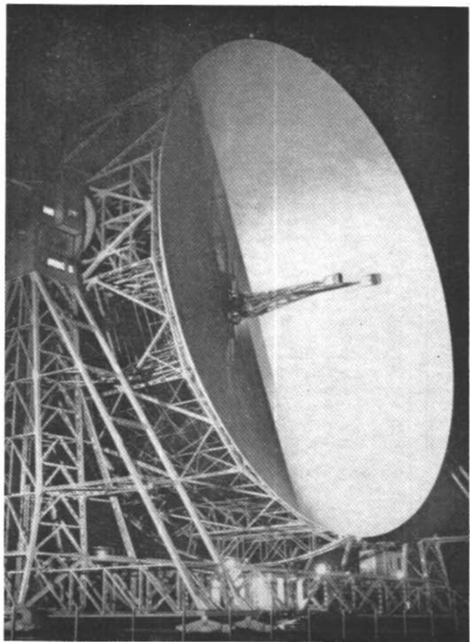
Plate 3. The 250 ft Jodrell Bank radio telescope
