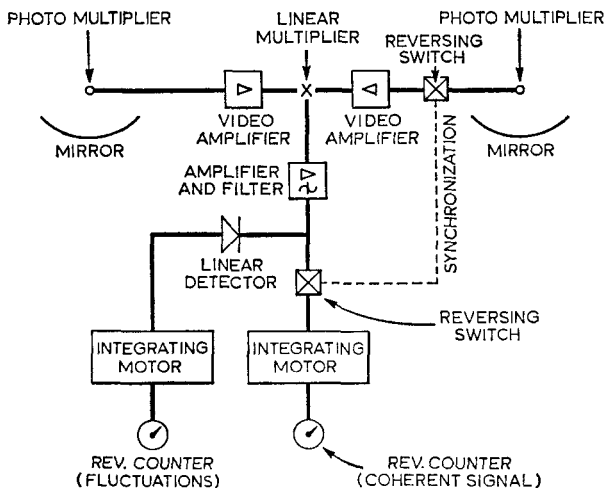
Fig. 33. Optical version of the intensity interferometer
