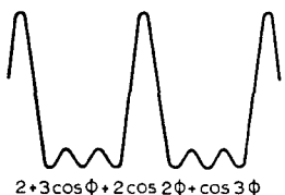
Fig. 38. Four aerials multiplied in three different ways (a), (b), (c), compared to the conventional addition and detection (d)
