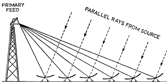
Fig. 41. An echelon telescope
