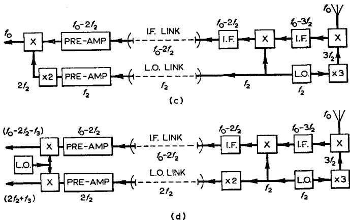
Fig. 28. Coherent radio links. The more complex arrangements in (c) and (d) show only remote station and link circuits. These circuits are less troubled by feedback instability and (d) shows how the L.O. link may be boosted prior to mixing by using a further oscillator. In this case the original frequency, f_0 , may be obtained by amplifying and mixing the two outputs. It is usually preferable not to reconstitute f_0 but to inject an oscillator into both limbs in order to amplify coherently at a lower frequency
