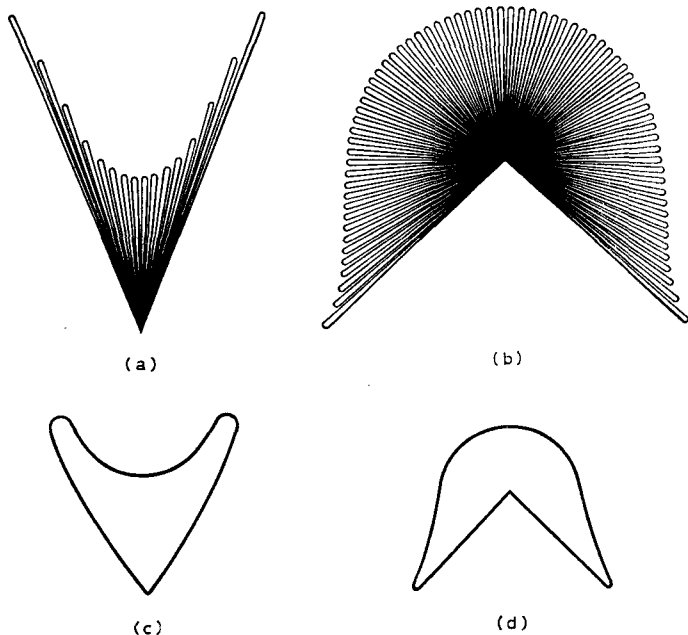
Fig. 43. (a) and (b) Polar diagrams corresponding to Fig. 42. The patterns (c) and (d) show the effect of a finite bandwidth and ionospheric inhomogeneity
