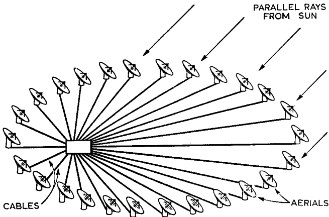
Fig. 37. The ring radio telescope
