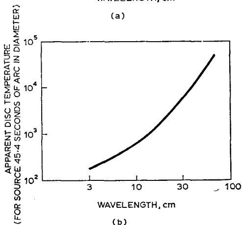
Fig. 13. The decimeter spectrum of Jupiter
