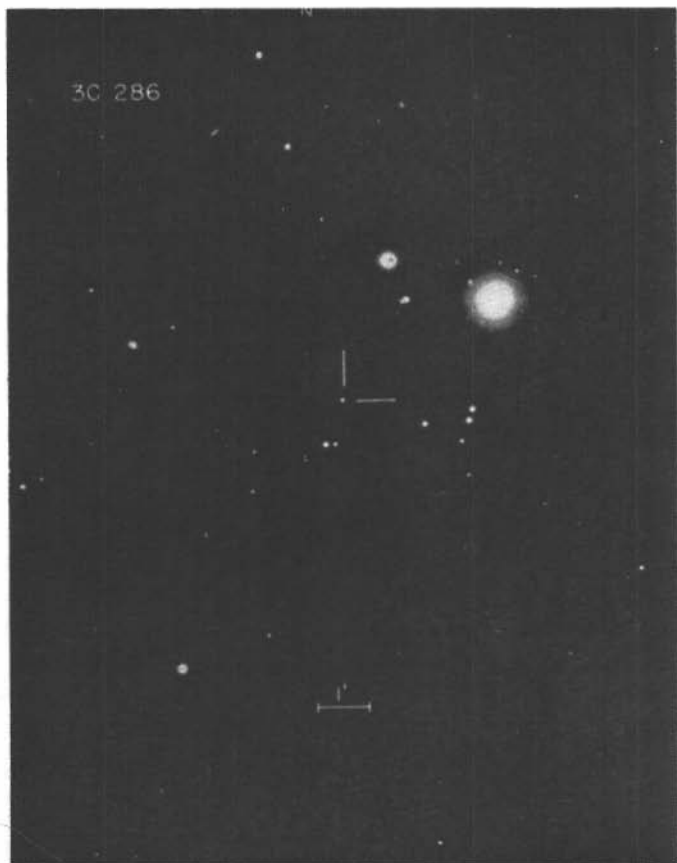
Plate 12. The 'Quasar' 3C 286 marked by the two white dashes (By courtesy of Alan Sandage, Mount Wilson and Palomar Observatories)
