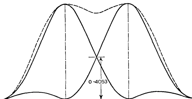
Fig. 22. The Rayleigh criterion of resolution. Individual patterns, full lines; combined pattern, dotted
