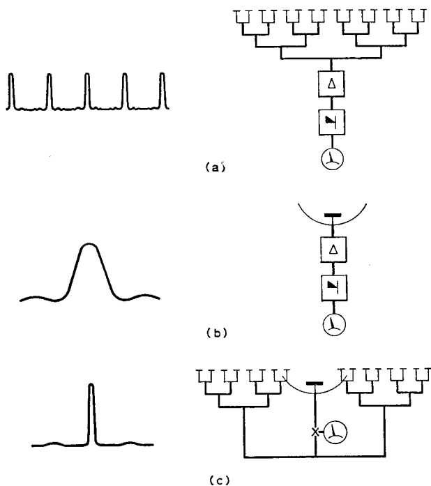
Fig. 39. The use of the principle of multiplication to produce a knife edge beam (c) from the directivity patterns of a grating (a) and a filled aperture (b)
