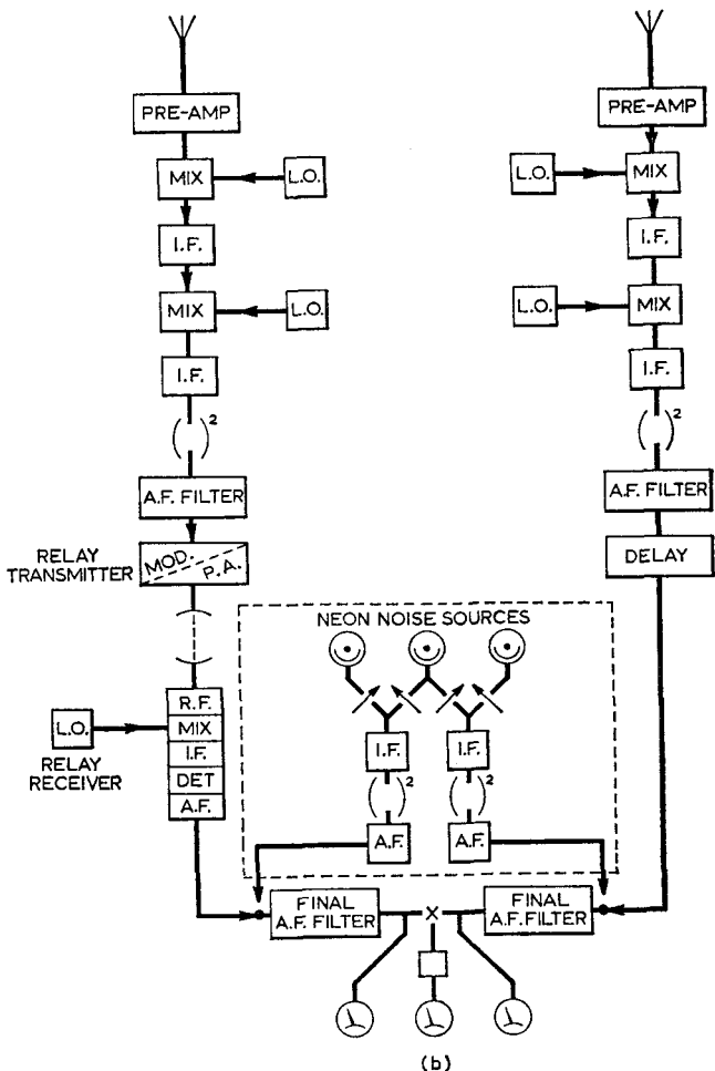
Fig. 31. The intensity interferometer
