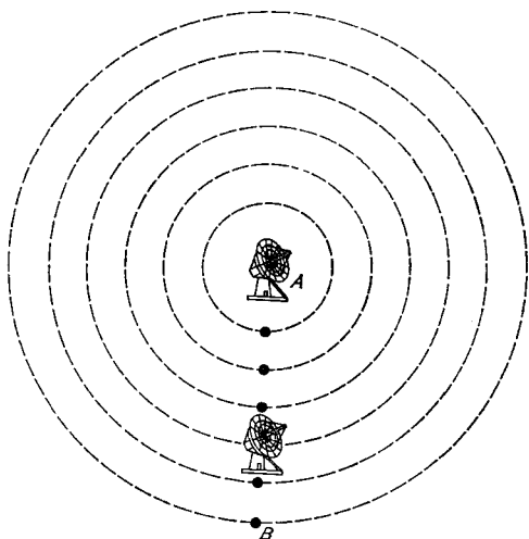
Fig. 24. Supersynthesis is a sophistication of aperture synthesis. The rotation of the Earth is used to sweep out the whole area if the measurements are made along the line AB
