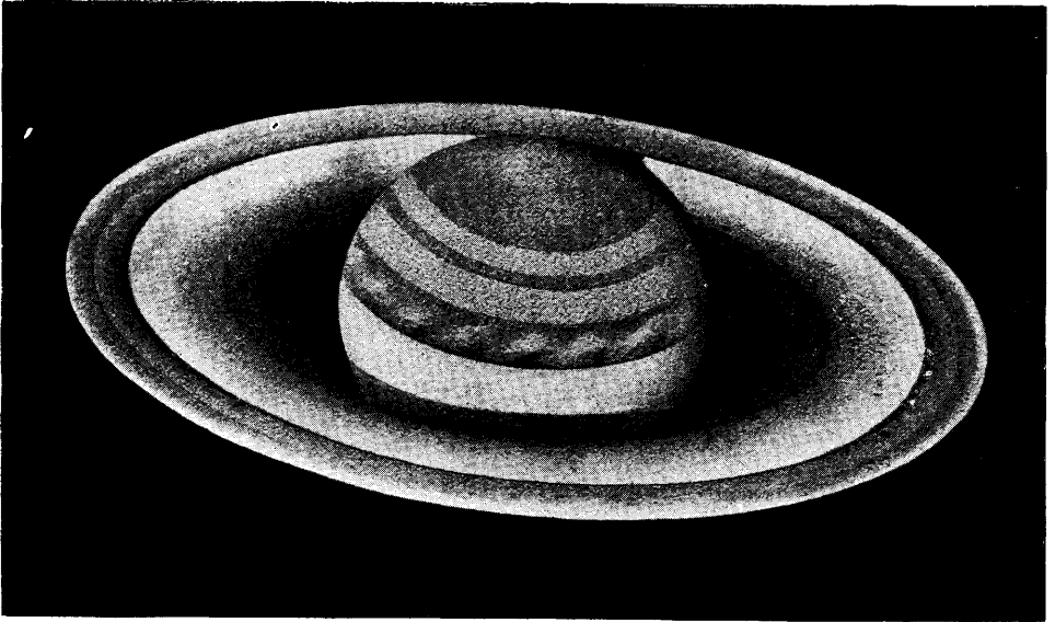
FIG. 187.—SATURN, FEBRUARY II, 1884 From a Drawing by Henry Pratt
