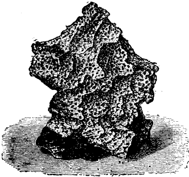
FIG. 137.—METEORITE FOUND IN CHILI IN 1860
