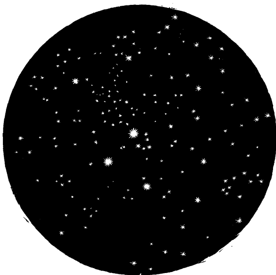
FIG. 279.—A CLUSTER OF STARS IN PERSEUS
