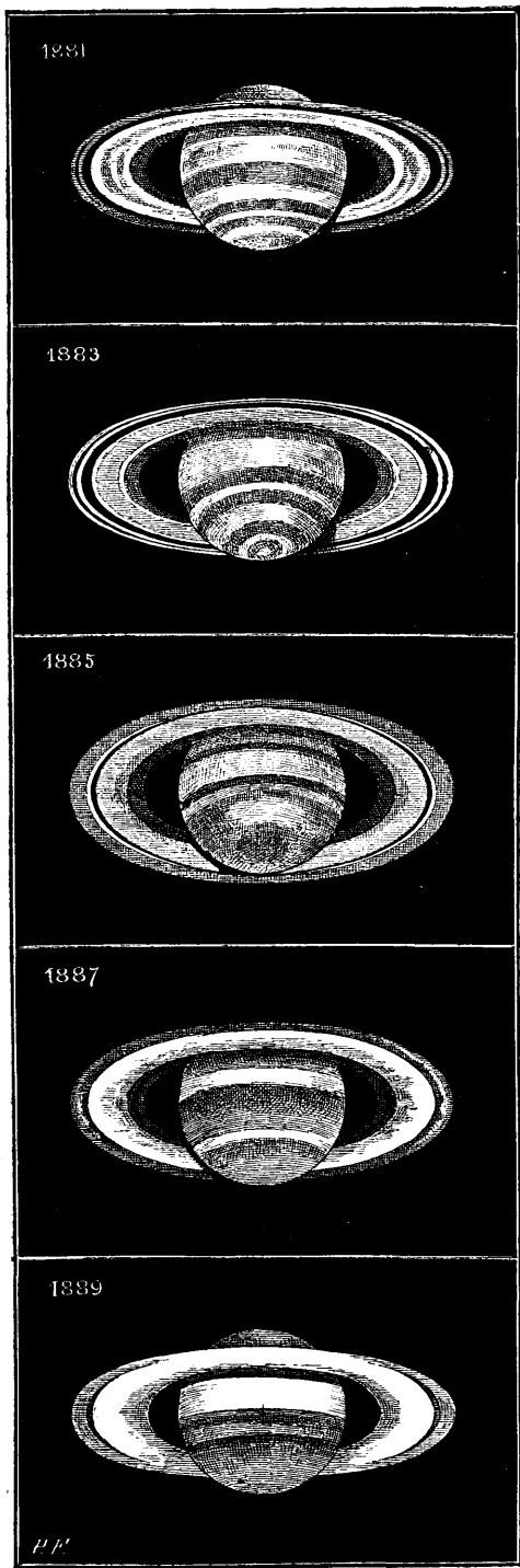
FIG. 189.—CHANGES IN APPEARANCE OF SATURN'S RINGS
