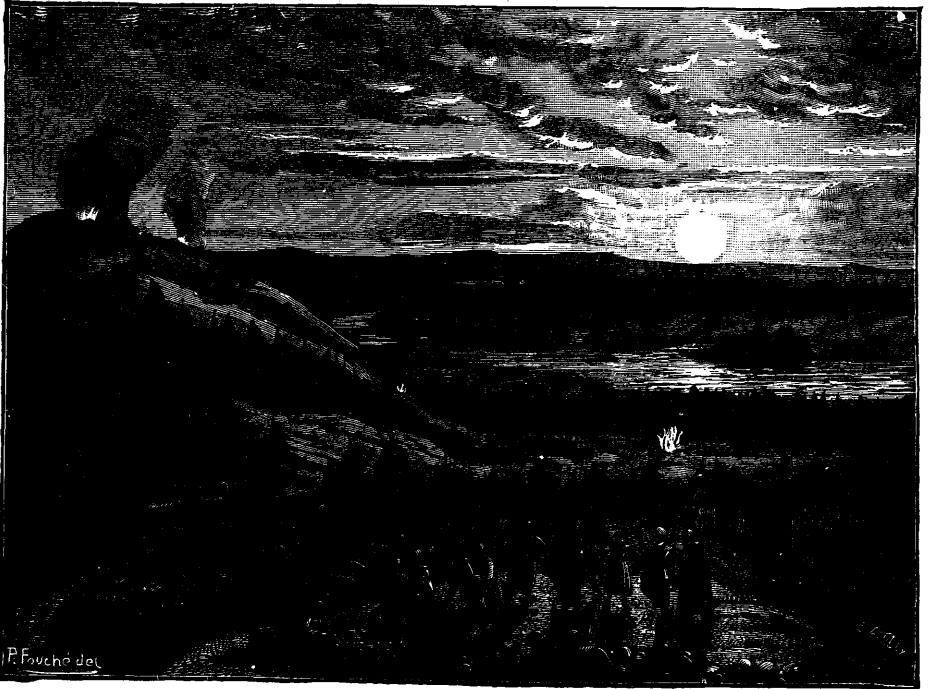
FIG. 11.—THE SUN SHINING OVER AVASAXA (RUSSIA) AT MIDNIGHT, ON JUNE 21
