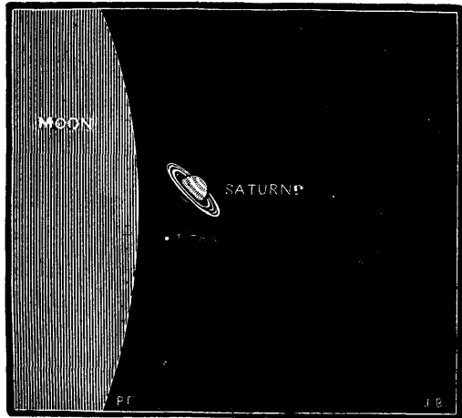
FIG. 56.—OCCULTATION OF SATURN BY THE MOON, APRIL 9, 1883, as seen in an inverting telescope
