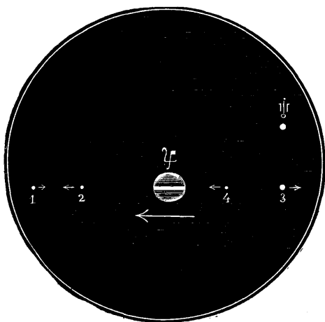
FIG. 195.—URANUS AND THE SATELLITES OF JUPITER, JUNE 5, 1872
