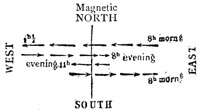
FIG. 128.—MOVEMENTS OF THE MAGNETIC NEEDLE
