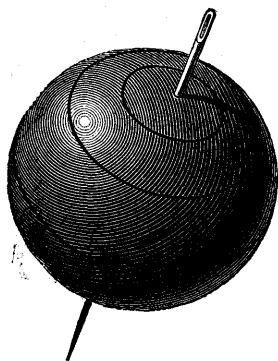
FIG. 3.—THE TERRESTRIAL GLOBE TURNING UPON ITS AXIS
