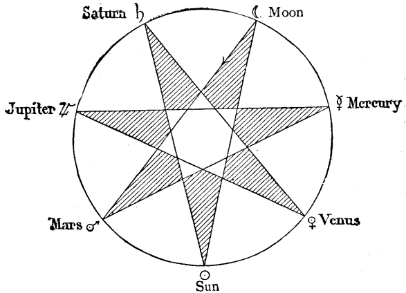
FIG. 39.—ASTRONOMICAL ORIGIN OF THE NAMES OF THE DAYS OF THE WEEK
