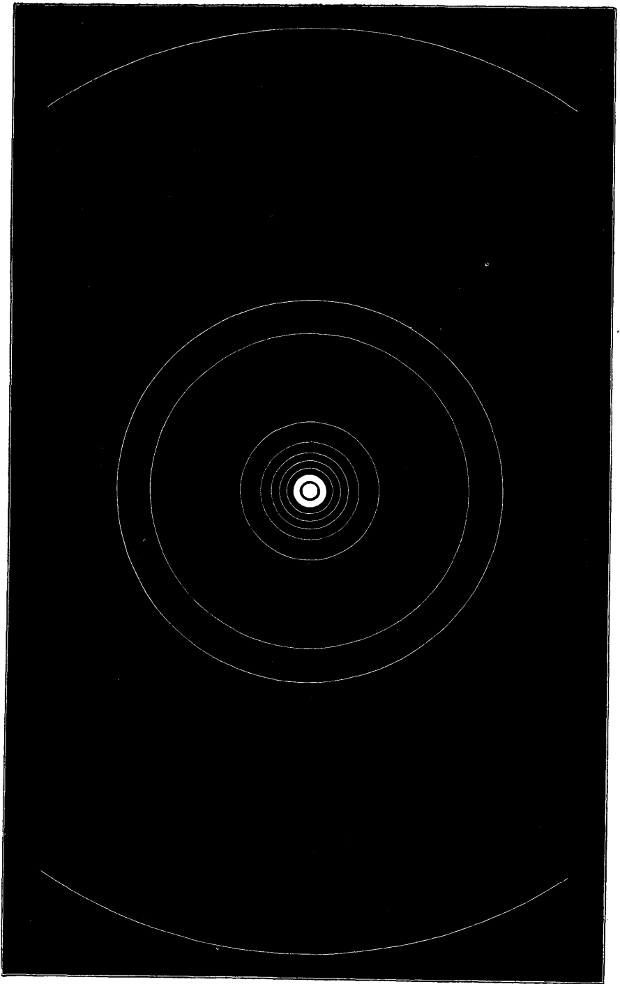
FIG. 194.—THE SYSTEM OF SATURN
