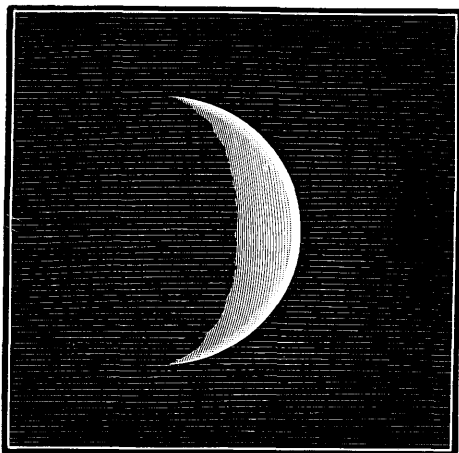
FIG. 159.—VENUS AT HER GREATEST BRILLIANCY
