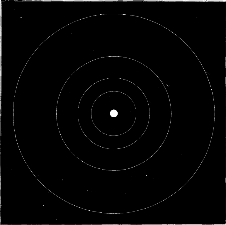
FIG. 181.—THE SYSTEM OF JUPITER (The Orbits of the Fifth, Sixth and Seventh Satellites are not given)
