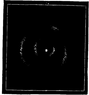
FIG. 27.—NEBULA : REMAINS OF DETACHED RINGS
