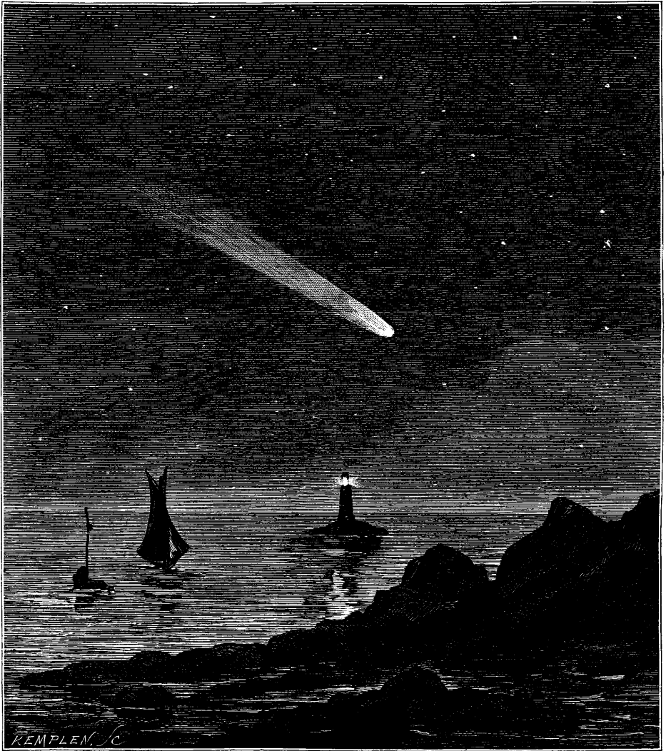
FIG. 203.—A COMET SEEN OVER THE SEA
