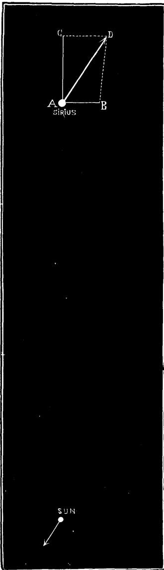
FIG. 274.—MOVEMENT OF SIRIUS IN SPACE
