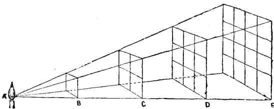
FIG. 84. — DECREASE OF INTENSITY IN PROPORTION TO THE SQUARE OF THE DISTANCE
