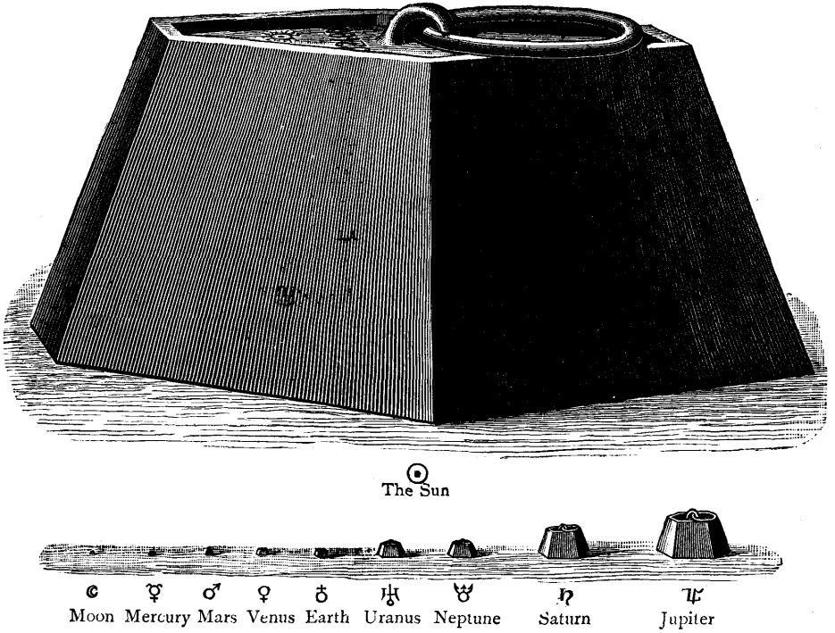
FIG. 97.—WEIGHTS REPRESENTING THE MASSES OF THE CELESTIAL BODIES
