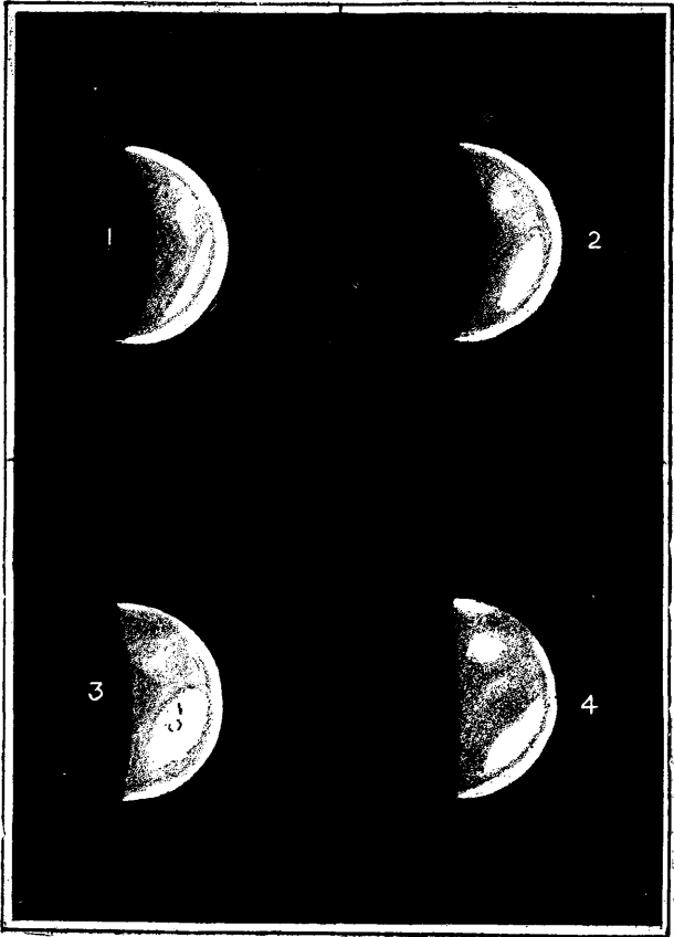
FIG. 154.—MERCURY AS A MORNING STAR, NOVEMBER 1882 (From Drawings by W. F. Denning. 1. November 5, 1 h 50 m . 2. November 6, 18 h 55 m . 3. November 8, 19 h 30 m . 4. November 9, 19 h 39 m . With 10-inch Reflector, Power 252
