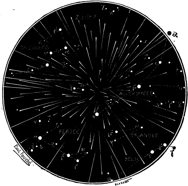
FIG. 230.—POINT OF EMANATION OF THE SHOOTING STARS OF NOVEMBER 27
