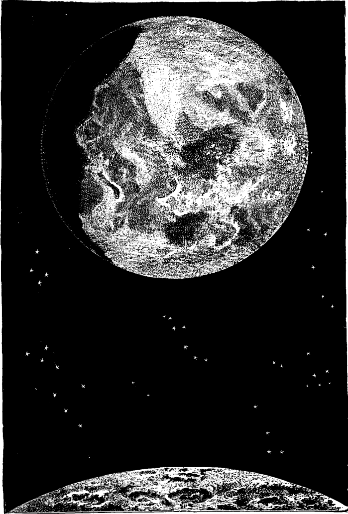
FIG. 1.—THE EARTH, AS SEEN FROM THE MOON
