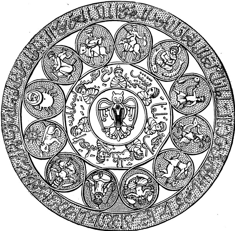
FIG. 251.—ANCIENT ARABIAN ZODIAC
