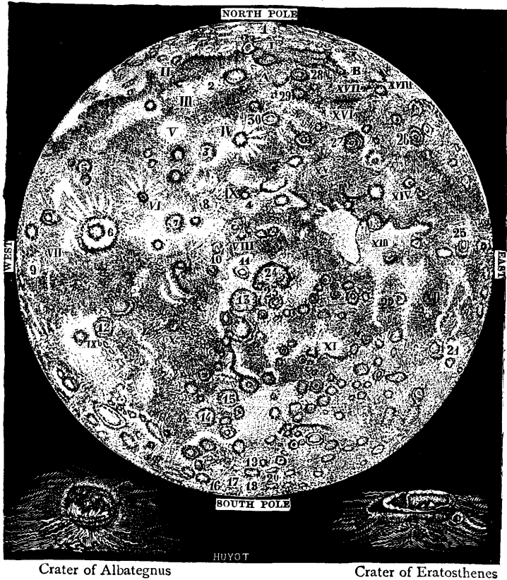
FIG. 47.—THE FULL MOON, AS SEEN THROUGH A TELESCOPE
