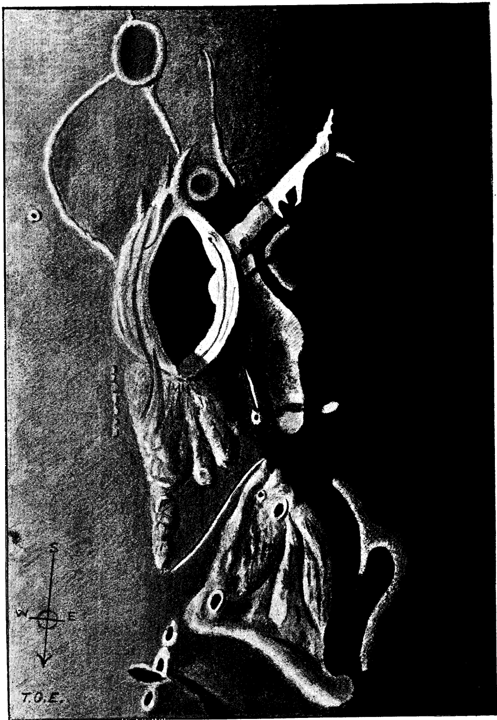
FIG. 49.—ARISTARCHUS AND THE WEST WALL OF HERODOTUS, MARCH 8, 1884 (Drawn by T. G. Elger. Powers 350-400, on 8½-inch Calver Reflector)
