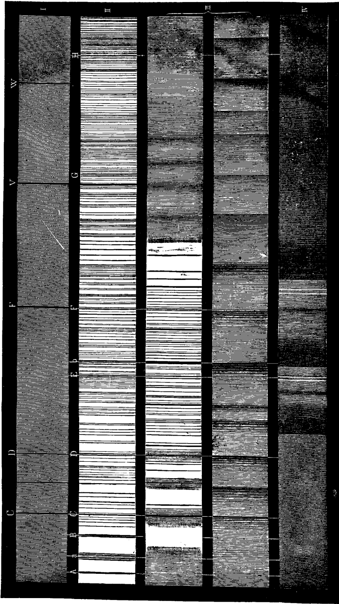
FIG. 263.—PRINCIPAL TYPES OF STELLAR SPECTRA
