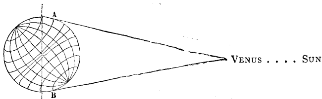
FIG. 92.—INCLINATION OF THE EARTH AT THE TIMES OF THE PASSAGE OF VENUS BEFORE THE SUN
