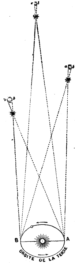
FIG. 23.—SMALL APPARENT ELLIPSES DESCRIBED BY THE STARS AS A RESULT OF THE ANNUAL MOVEMENT OF THE EARTH
