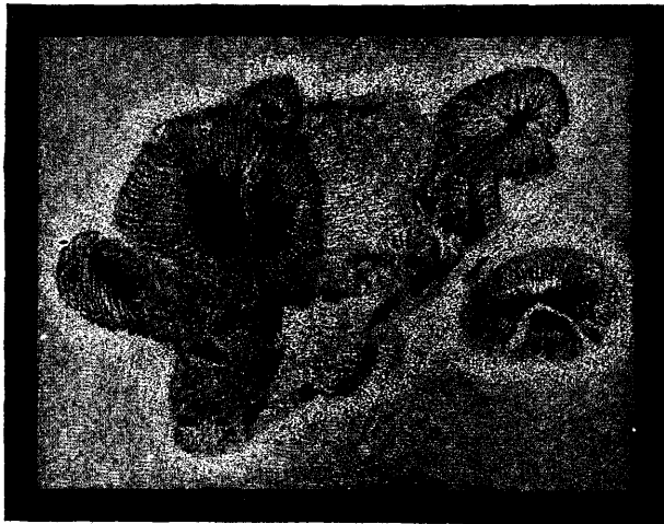
FIG. 101.—TYPICAL SUN-SPOTS
