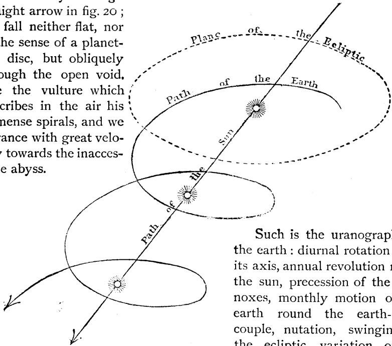
FIG. 20.—SPIRAL COURSE OF THE EARTH IN SPACE
