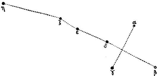
FIG. 270.—THE GREAT BEAR 50,000 YEARS AGO
