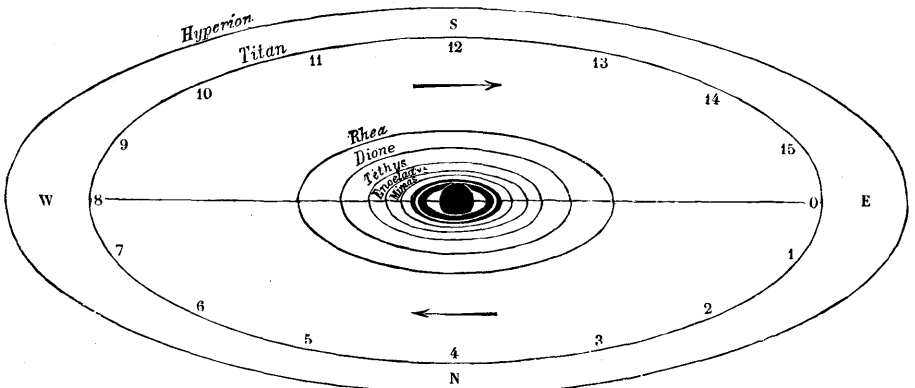
FIG. 193.—MINIMUM INCLINATION OF THE SYSTEM OF SATURN AS SEEN FROM THE EARTH (Phœbe and Themis not given)
