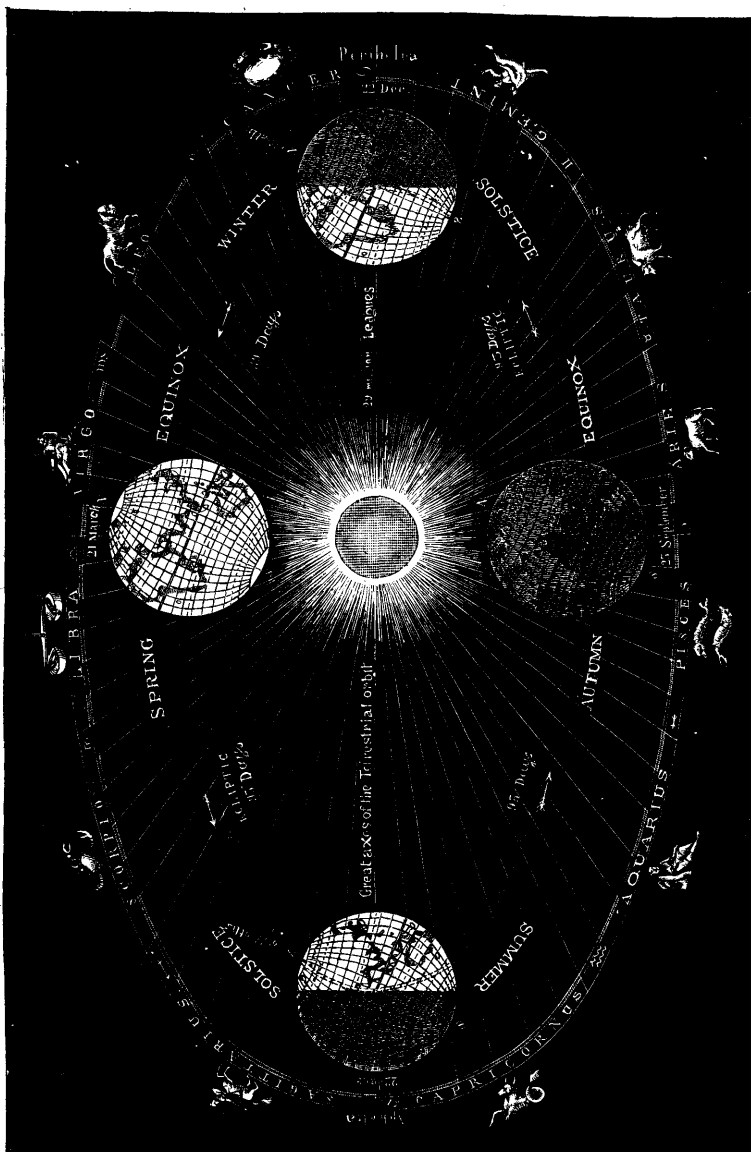
FIG. 9.—DIAGRAM OF THE ROTATION OF THE EARTH ROUND THE SUN
