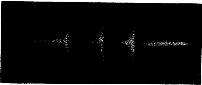
FIG. 228.—SPECTRUM OF COMET III. OF 1874
