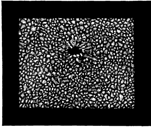
FIG. 100.—SURFACE OF THE SUN, HIGHLY MAGNIFIED
