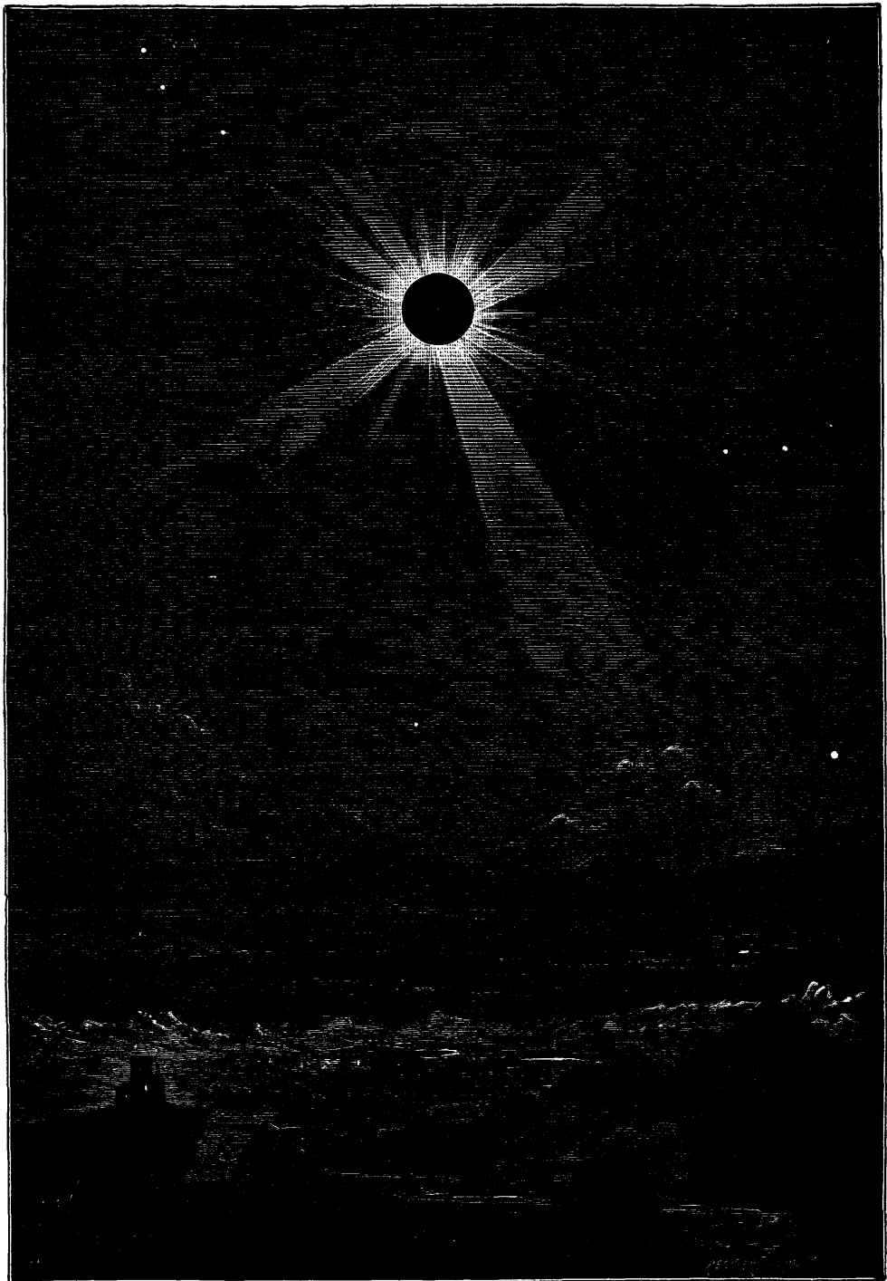
FIG. 75.—TOTAL ECLIPSE OF THE SUN, JULY 29, 1878, AS OBSERVED FROM THE ROCKY MOUNTAINS (UNITED STATES)
