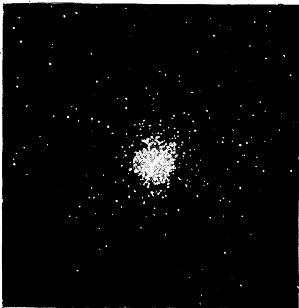
FIG. 281.—STAR CLUSTER IN HERCULES (13 MESSIER) (From a Photograph by MM. Henry)
