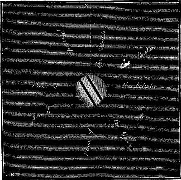
FIG. 197.—BANDS OBSERVED ON URANUS, AND PROBABLE INCLINATION OF ITS EQUATOR
