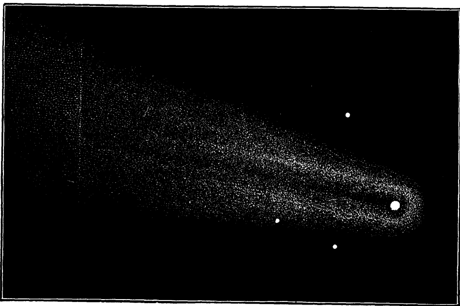
FIG. 227.—COMET III. OF 1874, ON JULY 6
