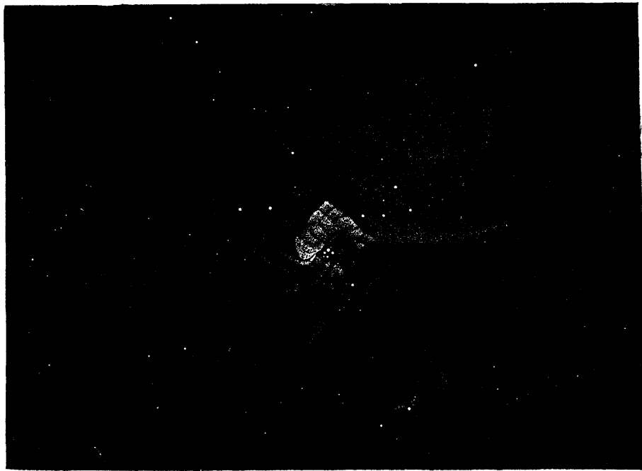
FIG. 283.—NEBULA IN ORION
