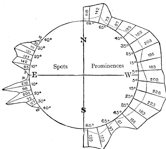
FIG. 123.—RELATIVE DISTRIBUTION OF SOLAR SPOTS AND PROMINENCES
