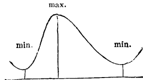
FIG. 127.—UNDECENNIAL SPOT CURVE
