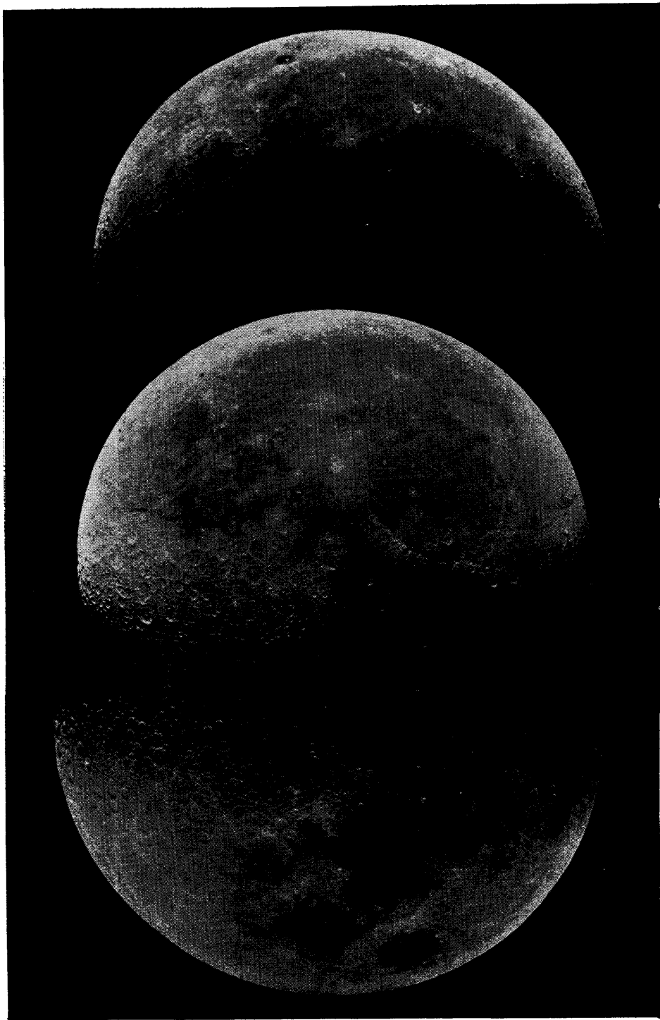
1 2 3 FIG. 44.—PHOTOGRAPHS OF THE MOON TAKEN WITH THE GREAT REFRACTOR OF THE LICK OBSERVATORY, CALIFORNIA
