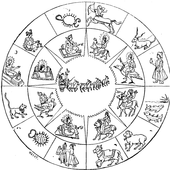
FIG. 252.—ANCIENT HINDOO ZODIAC
