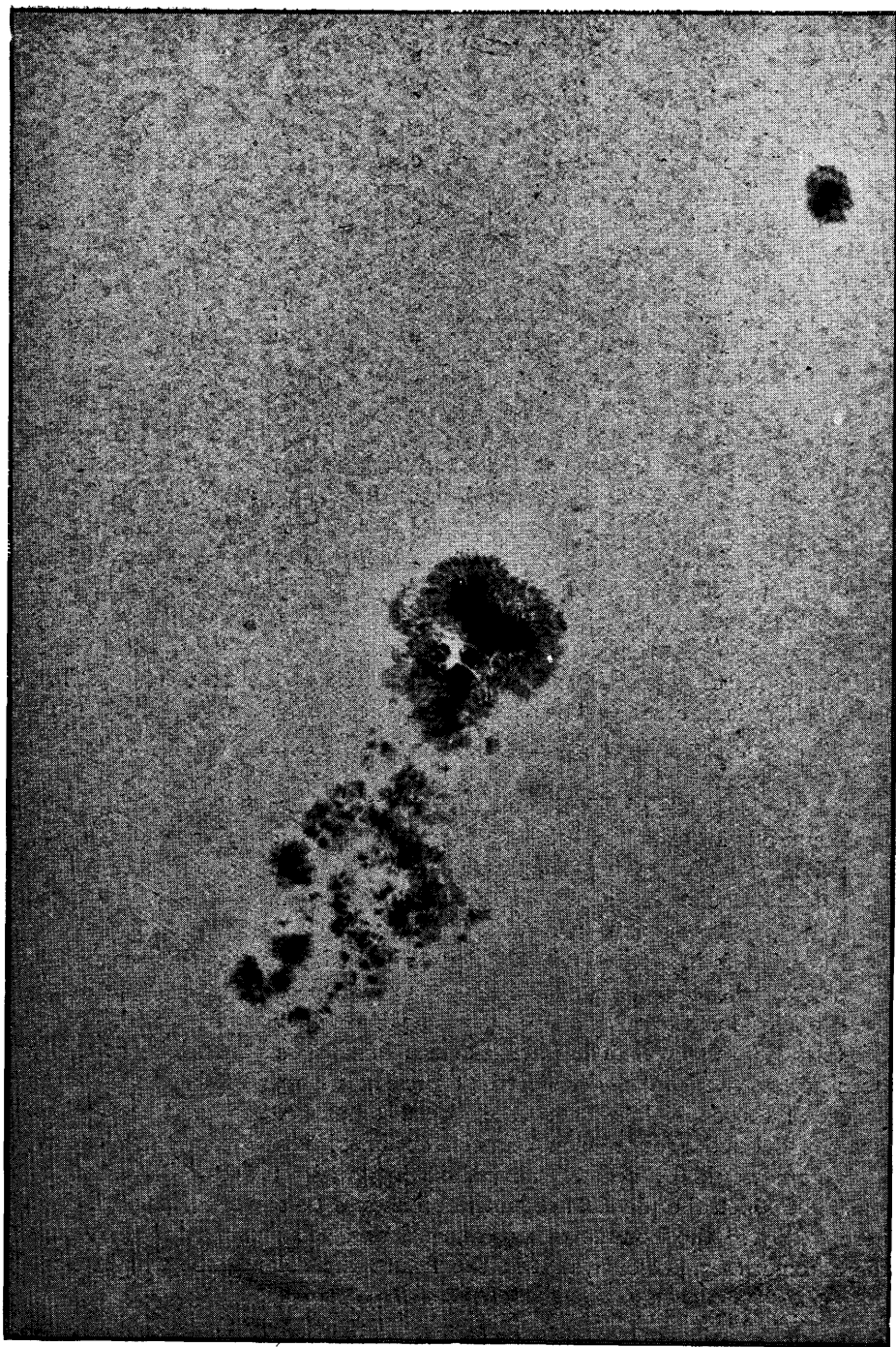
FIG. 133.—A REMARKABLE SUN-SPOT. (From a Photograph by Dr. Janssen)
