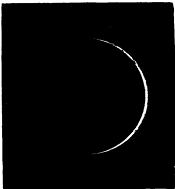
FIG. 162.—CRESCENT OF VENUS ONE DAY BEFORE INFERIOR CONJUNCTION WITH THE SUN
