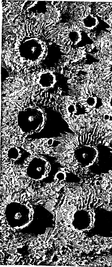
A Volcanic District—The Moon
