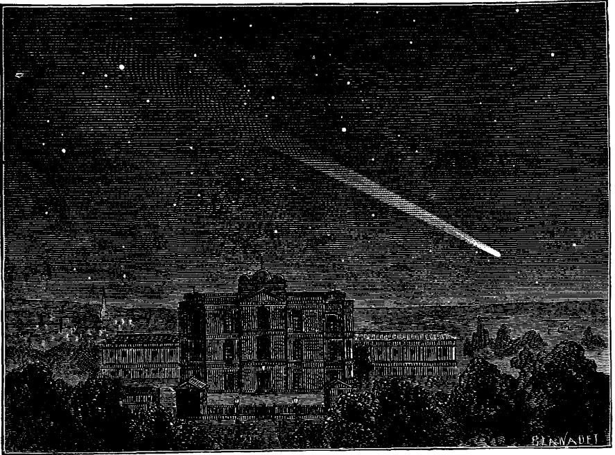
FIG. 215.—THE GREAT COMET OF 1843
