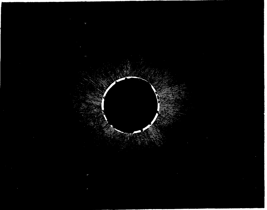
FIG. 74.—TOTAL ECLIPSE OF THE SUN, JULY 18, 1860
