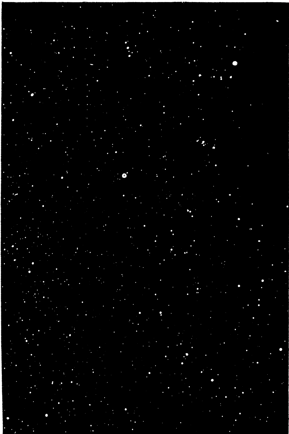
FIG. 265.—DIRECT PHOTOGRAPH OF A REGION IN THE CONSTELLATION GEMINI (Three exposures of an hour each. Untouched heliogravure reproduction)
