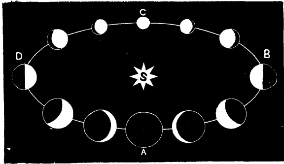
FIG. 160.—PHASES OF VENUS
