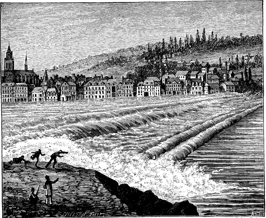
FIG. 65.—THE 'MASCARET' AT CAUDEBEC
