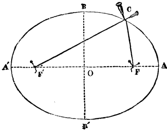
FIG. 8.—THE ELLIPSE
