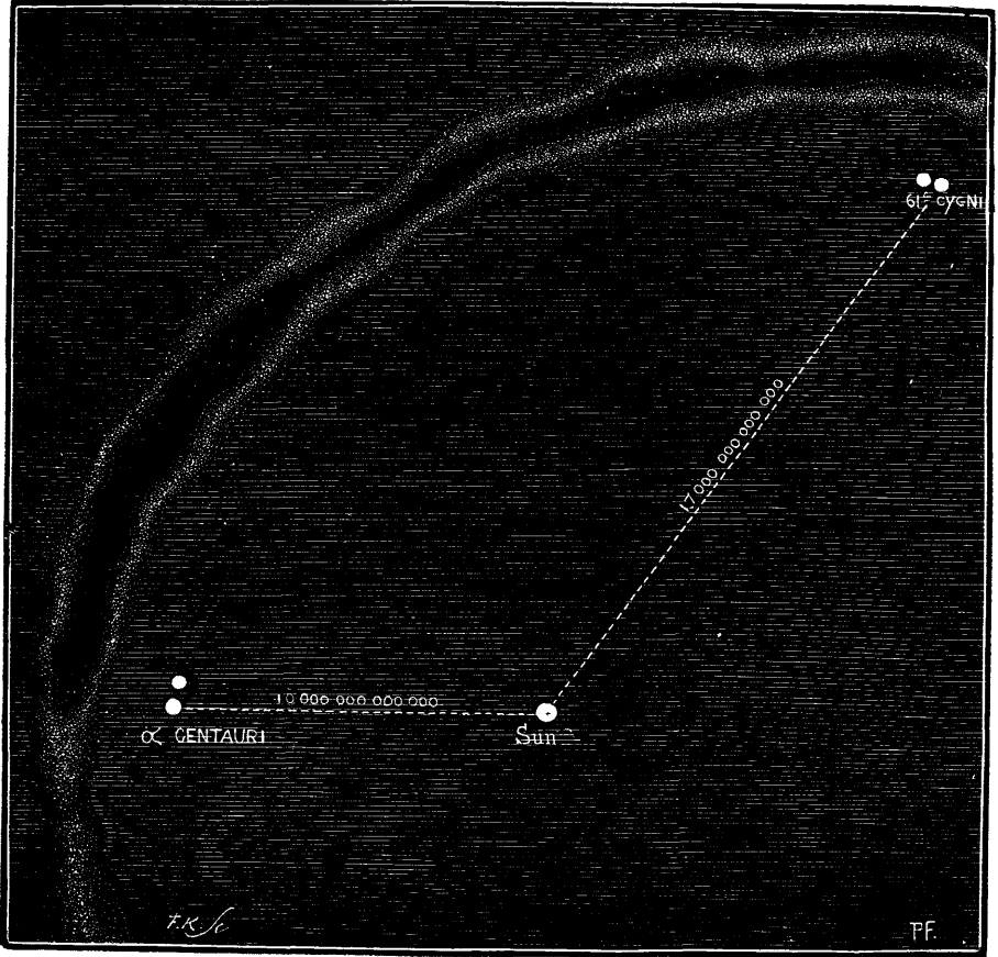
FIG. 262.—THE TWO SUNS THAT ARE NEAREST OURS
