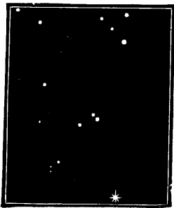
FIG. 258.—A REGION OF THE HEAVENS SEEN WITH THE NAKED EYE
