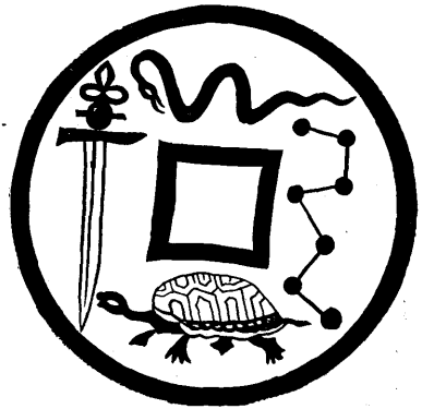
FIG. 254.—CHINESE MEDAL, SHOWING THE GREAT BEAR
