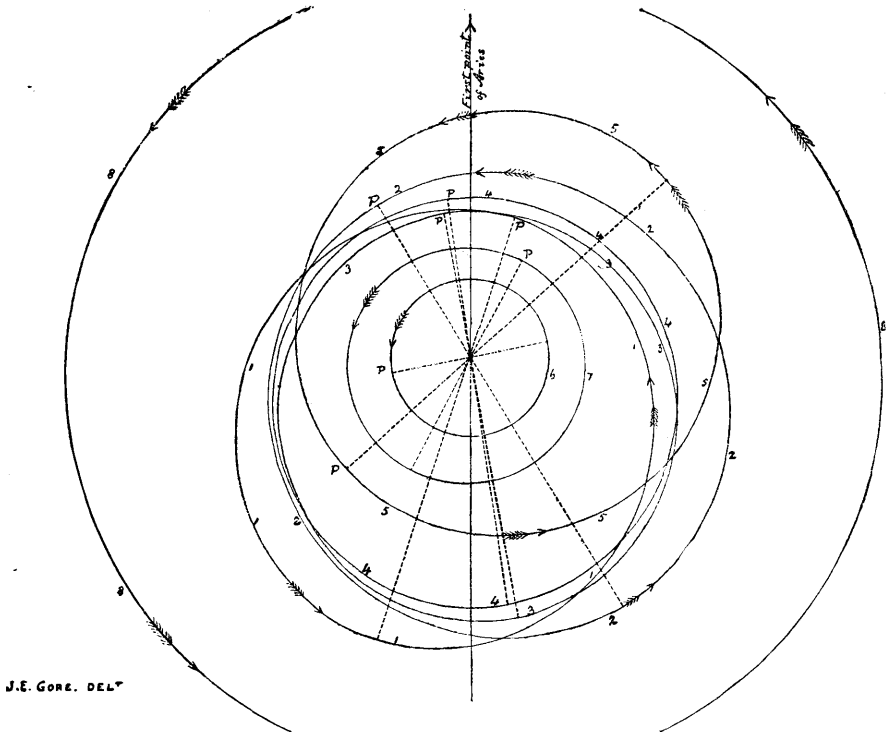
FIG. 174.—ORBITS OF SOME OF THE ASTEROIDS
