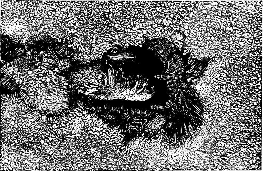
FIG. 132.—PHYSICAL CONSTITUTION OF THE SUN'S SURFACE—SPOT OF DECEMBER 1873 (From a Drawing by Langley)
