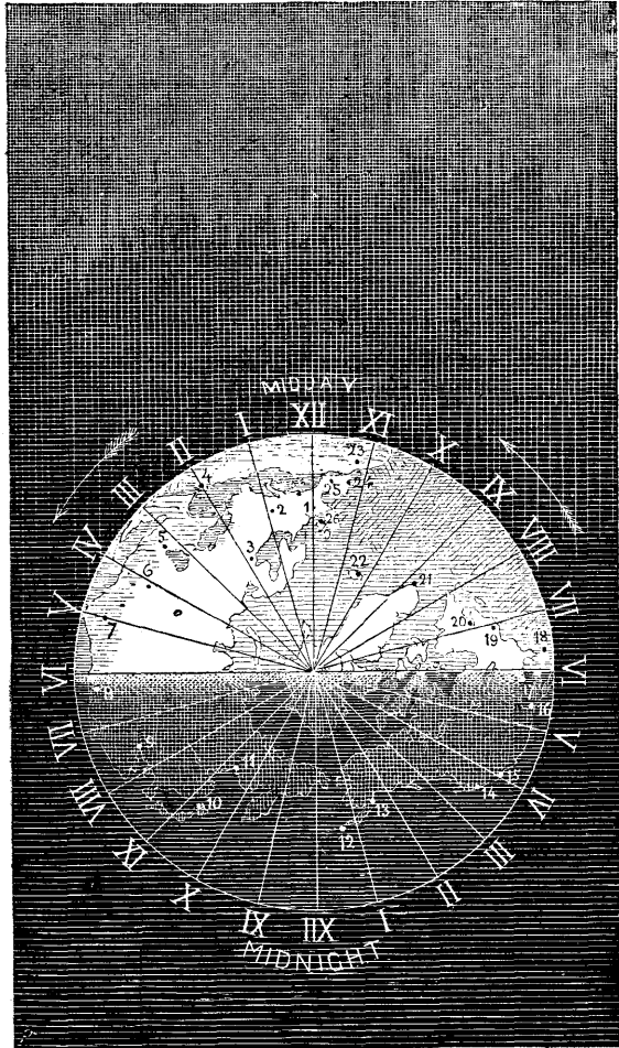
FIG. 4.—HOURS OF THE DAY AND NIGHT
