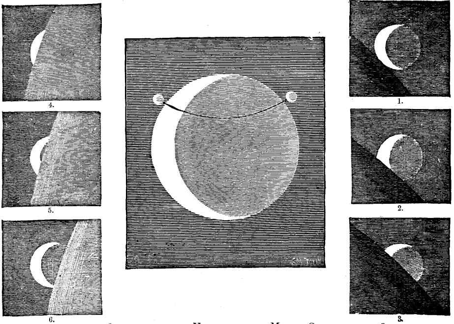
FIG. 55.—OCCULTATION OF VENUS BY THE MOON, OCTOBER 14, 1874 (As seen in an inverting telescope)
