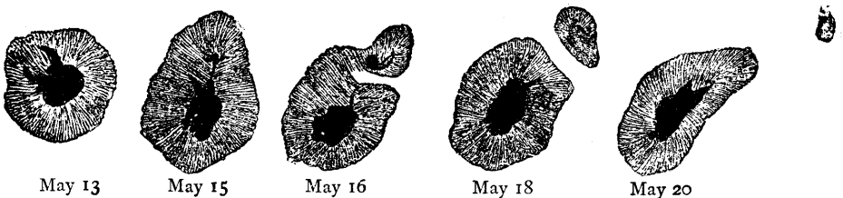
FIG. 107.—SEGMENTATION OF A SUN-SPOT
