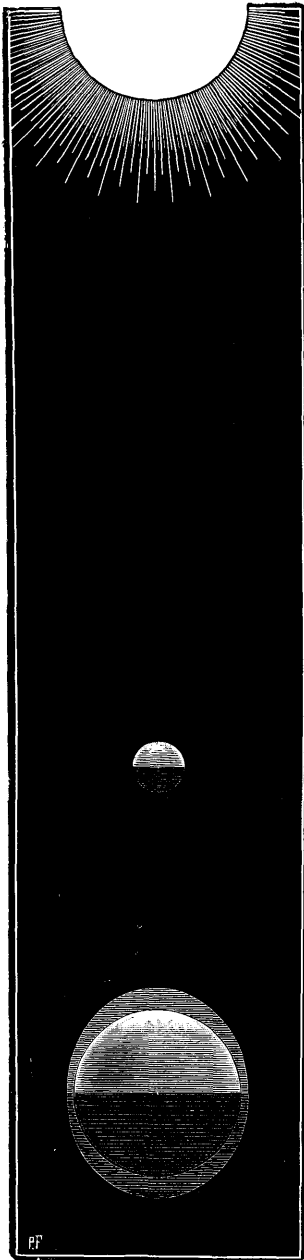
FIG. 63.—EXPLANATION OF THE TIDES
