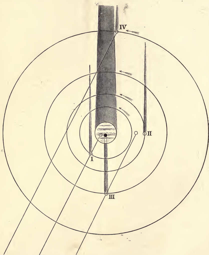
ECLIPSES AND TRANSITS OF JUPITER'S SATELLITES.
