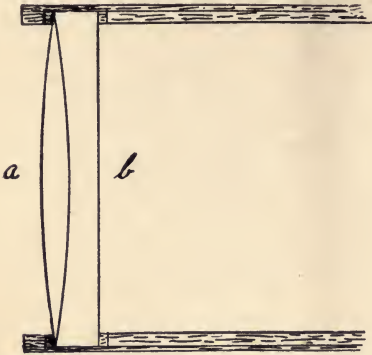
ACHROMATIC OBJECT GLASS. a, crown glass; b, flint glass.
