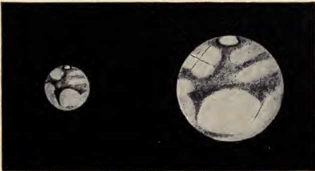
TWO VIEWS OF MARS IN 1892.
