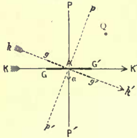
FIG. 148.—Shifting of a rotating body under the action of external forces.
