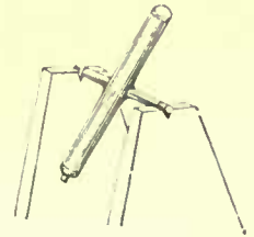
FIG. 23A.—Illustrating the principle of Transit Instruments.
