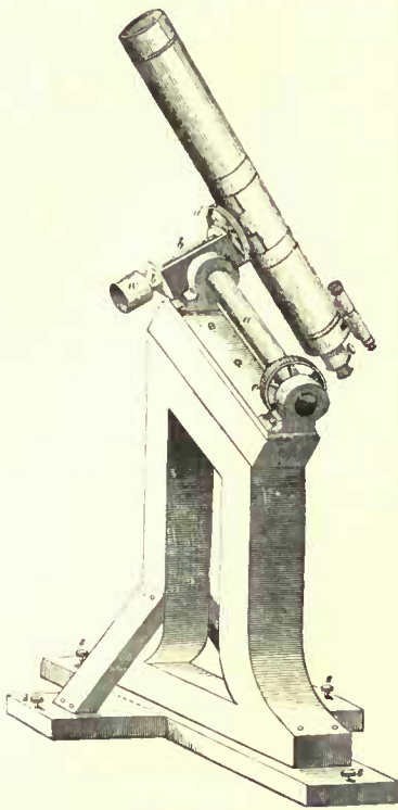
FIG. 27.—The Equatorial Telescope.
