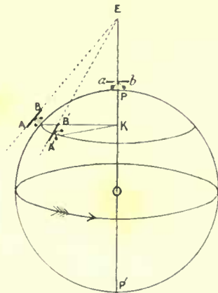
Fig. 157.—Illustrating Foucault's Pendulum experiment.
