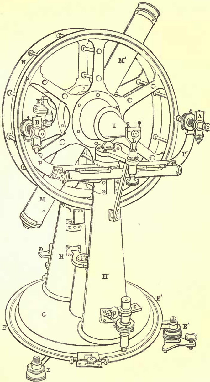
FIG. 31.—The Alt-azimuth as used in large observatories.
