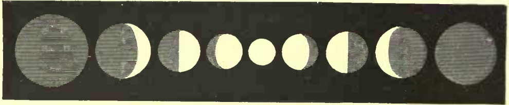
FIG. 301.—Varying phases of the planet Mercury.
