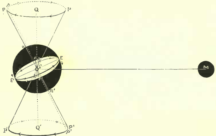
FIG. 150.—Illustrating the Precession of the Equinoxes.
