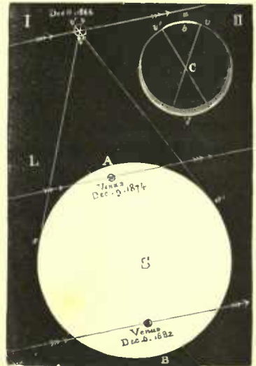
FIG. 316.—Illustrating the illumination round Venus when she is in inferior conjunction.
