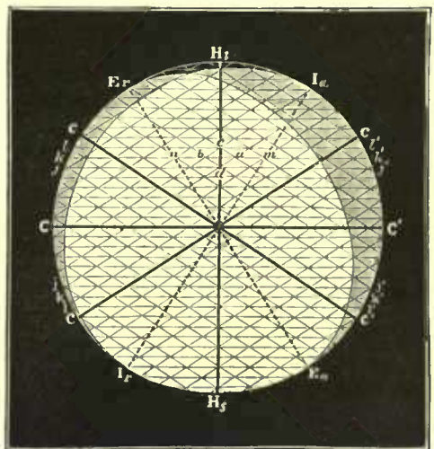
FIG. 185.—The Halleyan Poles and Circles of equal duration in the Transit of 1871.
