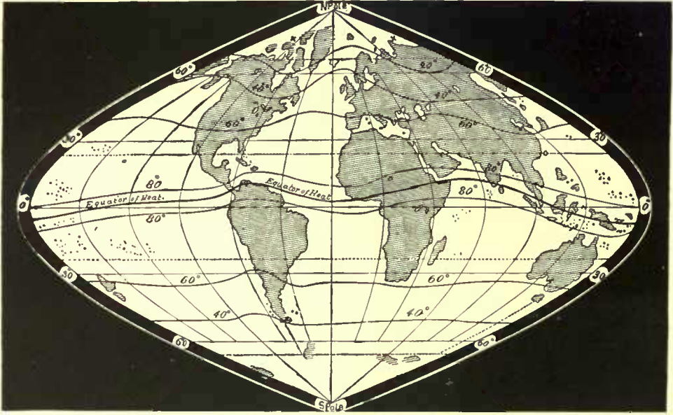
FIG. 71.—The World on an equal-surface projection, showing the Mean Annual Isotherms, or lines of equal mean temperature throughout the year.
