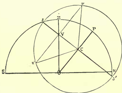
FIG. 64.—Illustrating use of Prime Vertical Instrument for determining latitudes.
