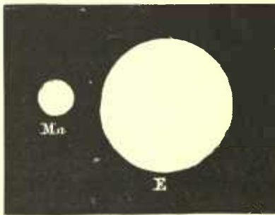
FIG. 333.—The globes of the Earth, E , and the moon, M_n , on the same scale.
