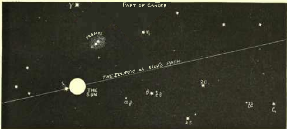
FIG. 299.—Professor Watson's observation of supposed intra-Mercurial Planets.
