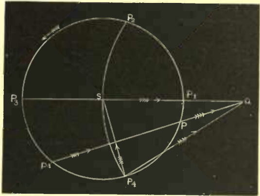
FIG. 425.—Diagram to illustrate the perturbing action of an outer planet on an inner one.
