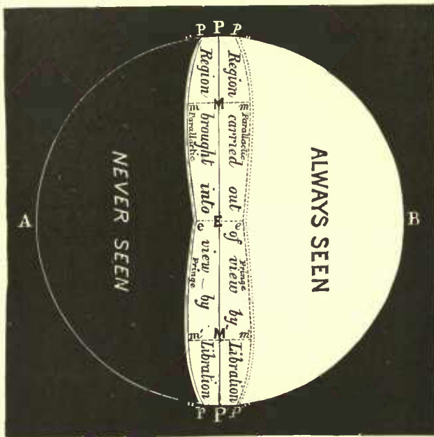
FIG. 341.—Imaginary side view of the Moon's Globe, showing the relative extent of the areas brought into view and carried out of view by libration.
