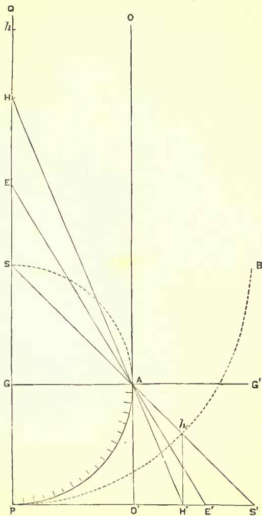
FIG. 66.—Illustrating the principal Projections of the Sphere.
