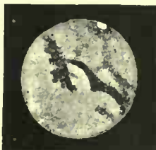
FIG. 367.—Sept. 16, 9h. 40m. G.M.T. (Trouvelot).
