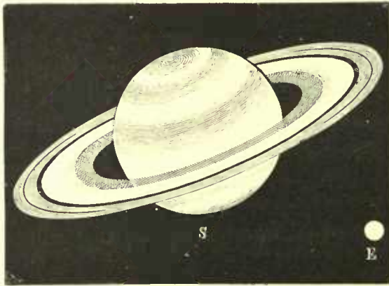
FIG. 408.—The globes of Saturn S, and the Earth E, on the same scale. 2
