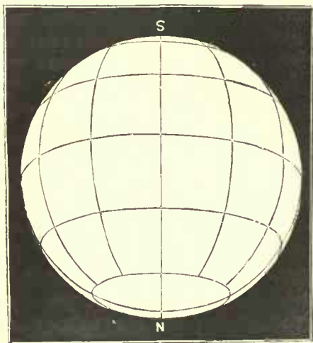
FIG. 357.—Aspect of Mars, February 1, 1884 (inverting telescope).
