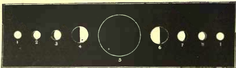
FIG. 313.—Corresponding phases of Venus.
