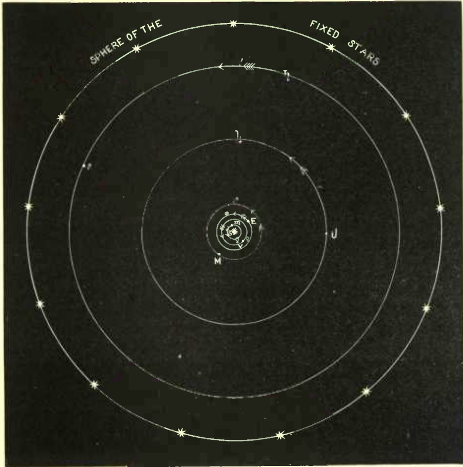
FIG. 117.—System of Copernicus.
