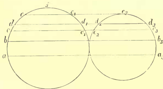
FIG. 461.—Diagram illustrating collision of two spherical bodies.
