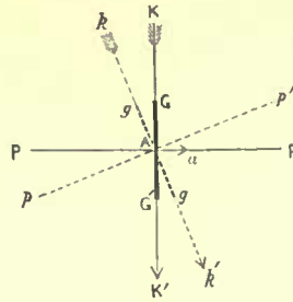
FIG. 149.—Another example of the same.
