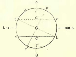
FIG. 318.—Illustrating the Earth's axial rotation.
