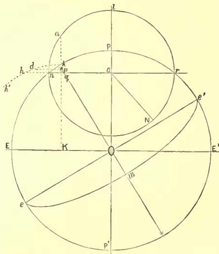
FIG. 358.—Construction for determining Mars's aspect, May 1, 1888.
