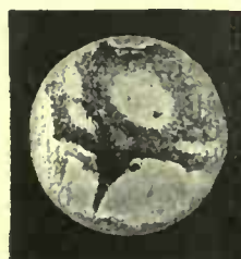
FIG. 370.—Sept. 18, 11h. 20m. G.M.T. (Green).
