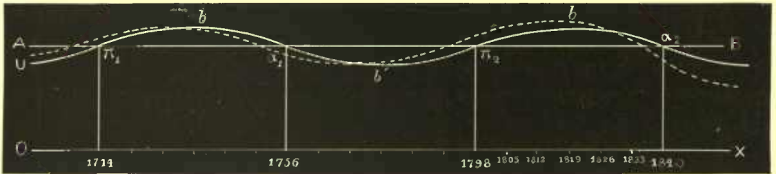
FIG. 429.—Diagram showing the displacement of Uranus relatively to a planet moving uniformly in a circular orbit.
