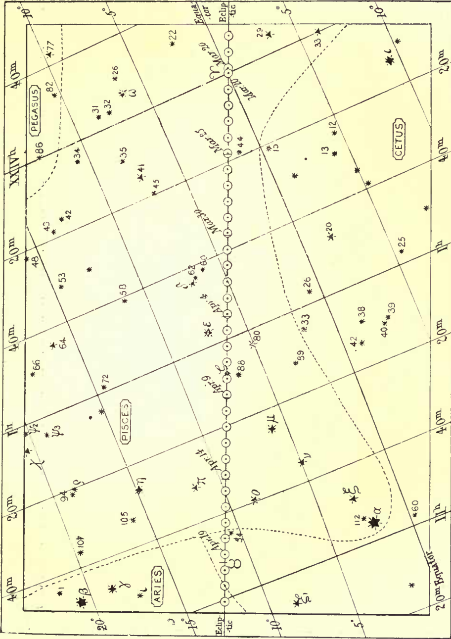
FIG. 89.--THE SUN'S COURSE THROUGH THE SIGN ARIES.
