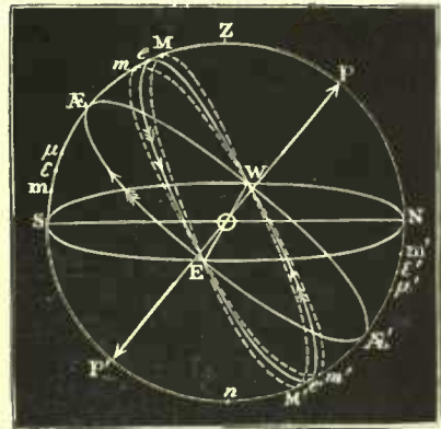
FIG. 103.—Showing the Moon's path round the Star-sphere when it has its mean inclination of the celestial equator.
