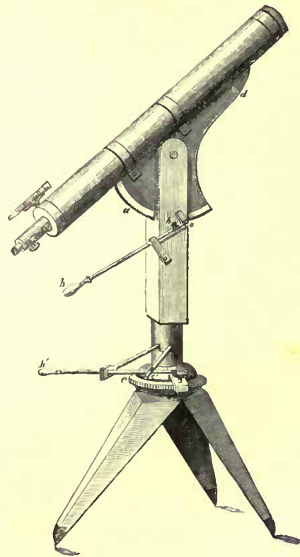
FIG. 29. — Proctor's Alt-azimuth Mounting.
