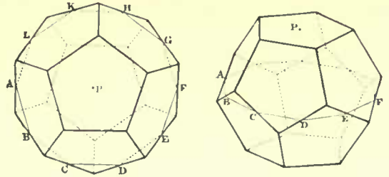
FIG. 81.—The Dodecahedron.
