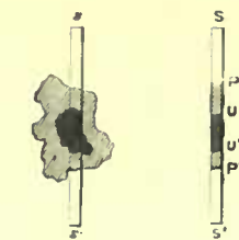
FIG. 253.—Illustrating the Spectroscopic study of a Sun-spot.
