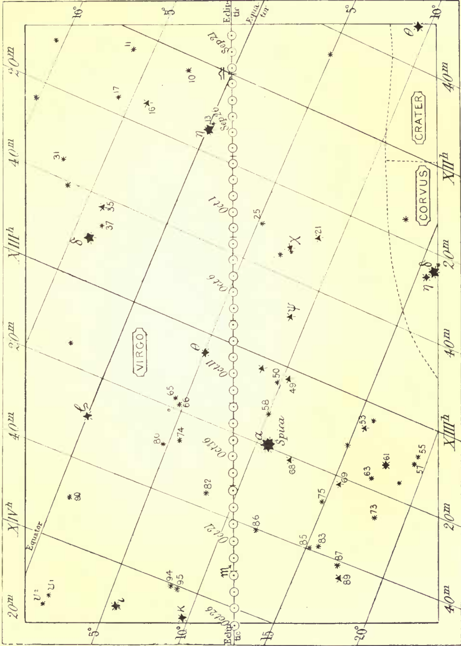
FIG. 95.—THE SUN'S COURSE THROUGH THE SIGN LIBRA.
