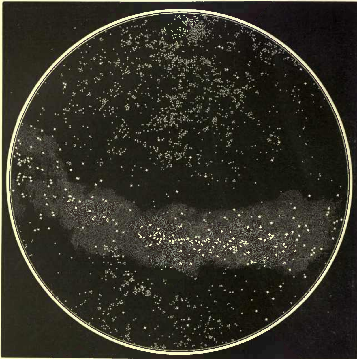
FIG. 446.—The Nebulae and Clusters in the Northern Hemisphere, plotted on an equal surface-projection by Mr. Sidney Waters, from Sir John Herschel's catalogue. The nebulae are represented by dots, the clusters by crosses.
