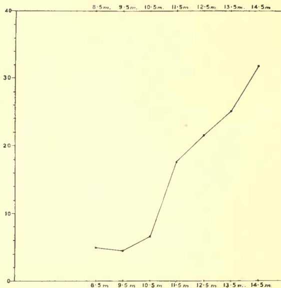
FIG. 444.—The ordinates of the curve represent the number of stars in the Pleiades cluster of various magnitudes from the 8th to the 15th comprised within a limited area about Aleyone.
