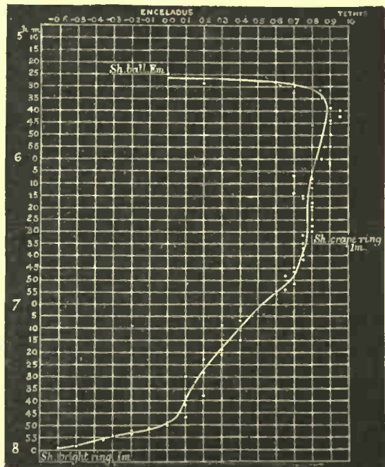
FIG. 422.—Light curve showing the brightness of Japetus in the shadows of the globe, crape ring and bright ring of Saturn, Nov. 1, 1889. The vertical scale corresponds to time, the horizontal to brightness.
