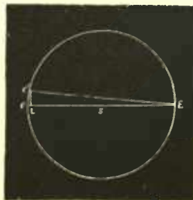
FIG. 204.—Illustrating the Sun's pull on the Earth.
