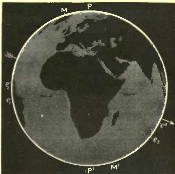
FIG. 349.—Earth's face turned moonwards at the time of central eclipse. October 1, 1884, 10.2 P.M. (Greenwich mean time).
