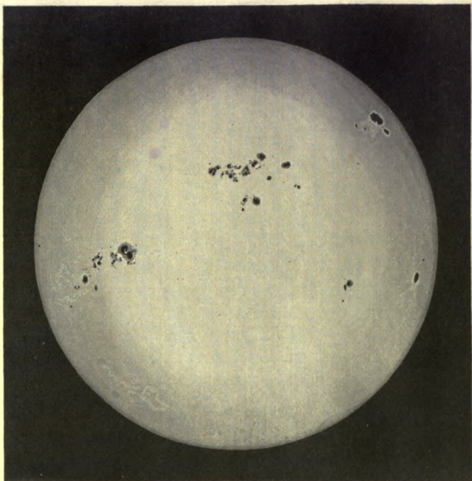
PHOTOGRAPH OF THE SUN, SEP. 22 ND 1870.
