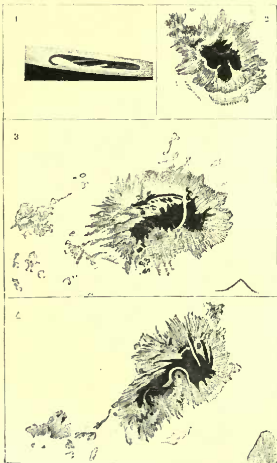
FIG. 228.—The great Sun-spot of 1865, from Oct. 7 to Oct. 16 (Howlett).
