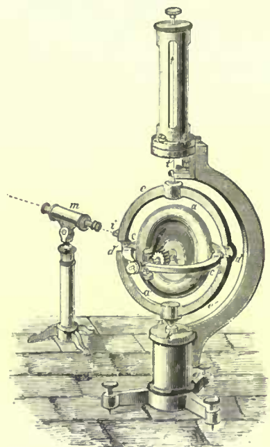
FIG. 161.—Foucault's original Gyroscope.
