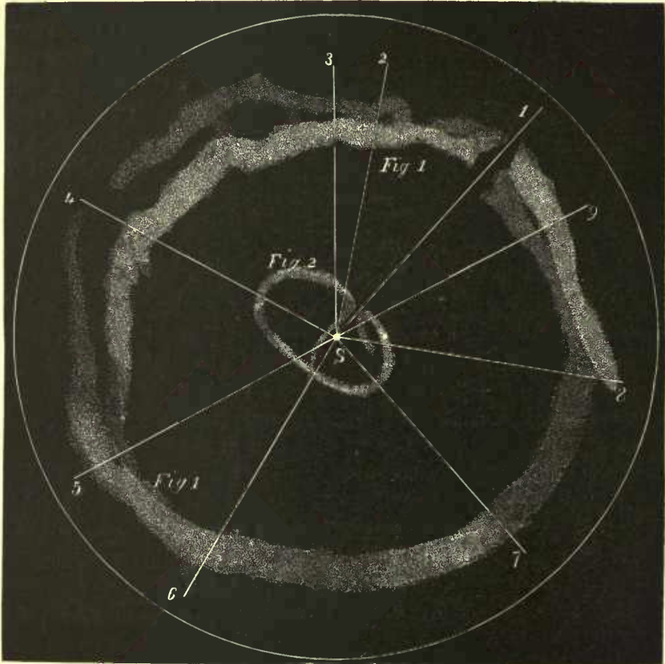
FIG. 44). - (Fig. 1) The Milky Way as seen in the heavens. (Fig. 2) The Spiral Stream which Mr. Proctor assumed represented the actual form of the Milky Way.
