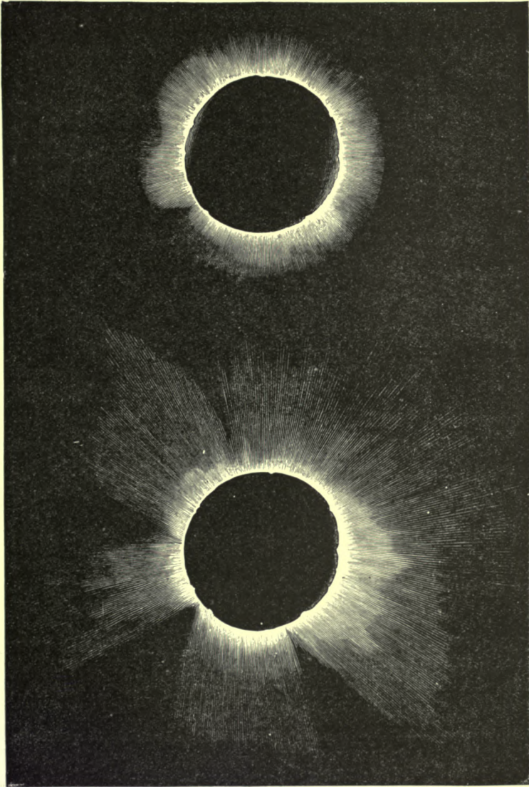
FIG. 293.—Mr. Brothers' photograph, taken at Syracuse.
