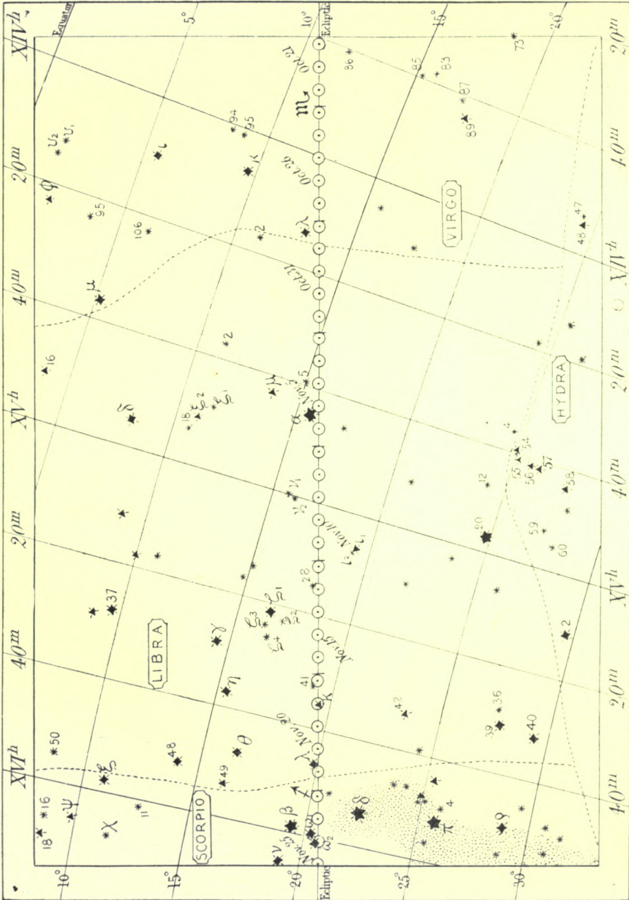
FIG. 96. — THE SUN'S COURSE THROUGH THE SIGN SCORPIO.
