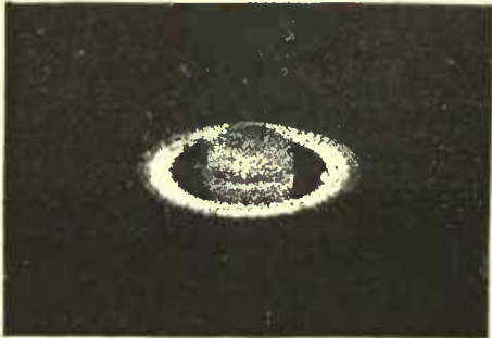
FIG. 421.—Photograph of Saturn. (Bros. Henry.) Process block untouched by engraver.
