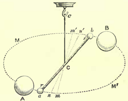
FIG. 201.—Illustrating the principle of the Cavendish experiment. (Baily.)
