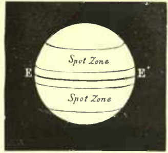
Fig. 212.—The Spot Zones on the surface of the Sun.
