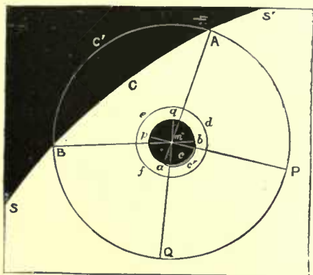
FIG. 309.—Illustrating the action of the Atmosphere of a Planet in transit.
