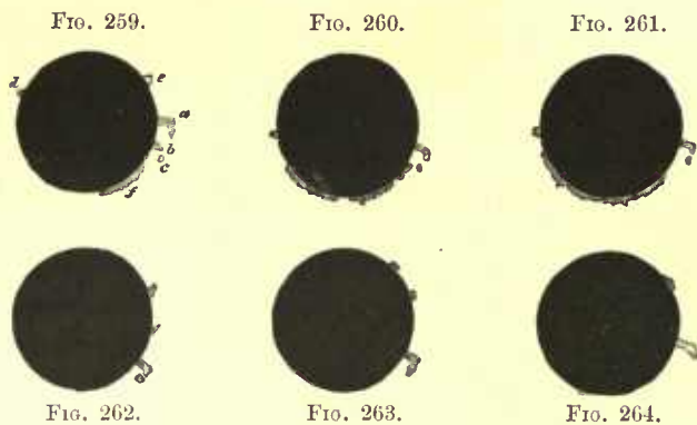
The Coloured Prominences seen during the Eclipse of 1851.
