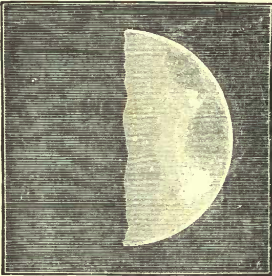
FIG. 315.—Venus when half-full ( Folache ).
