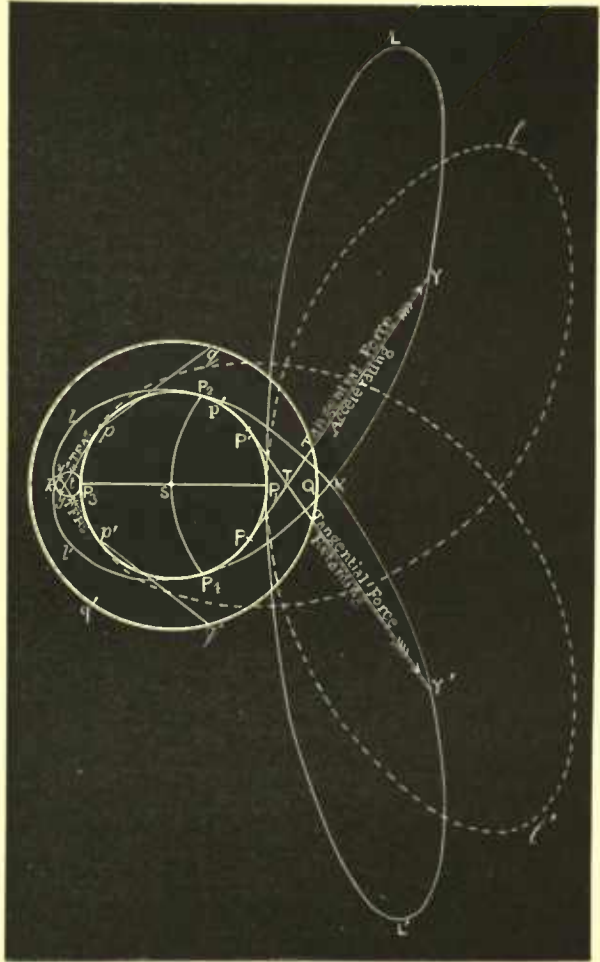
FIG. 427.—Diagram showing magnitude of tangential accelerating and retarding forces. Continuous curve when the outer body is stationary, dotted curve when the outer body moves like a planet.
