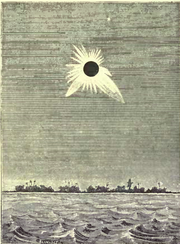
FIG. 297.—The Corona during the Eclipse of May 1883.
