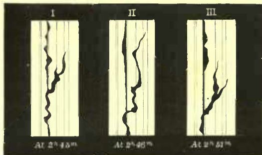
FIG. 256.—Changes in the C line of Hydrogen, September 22, 1870 (Young).
