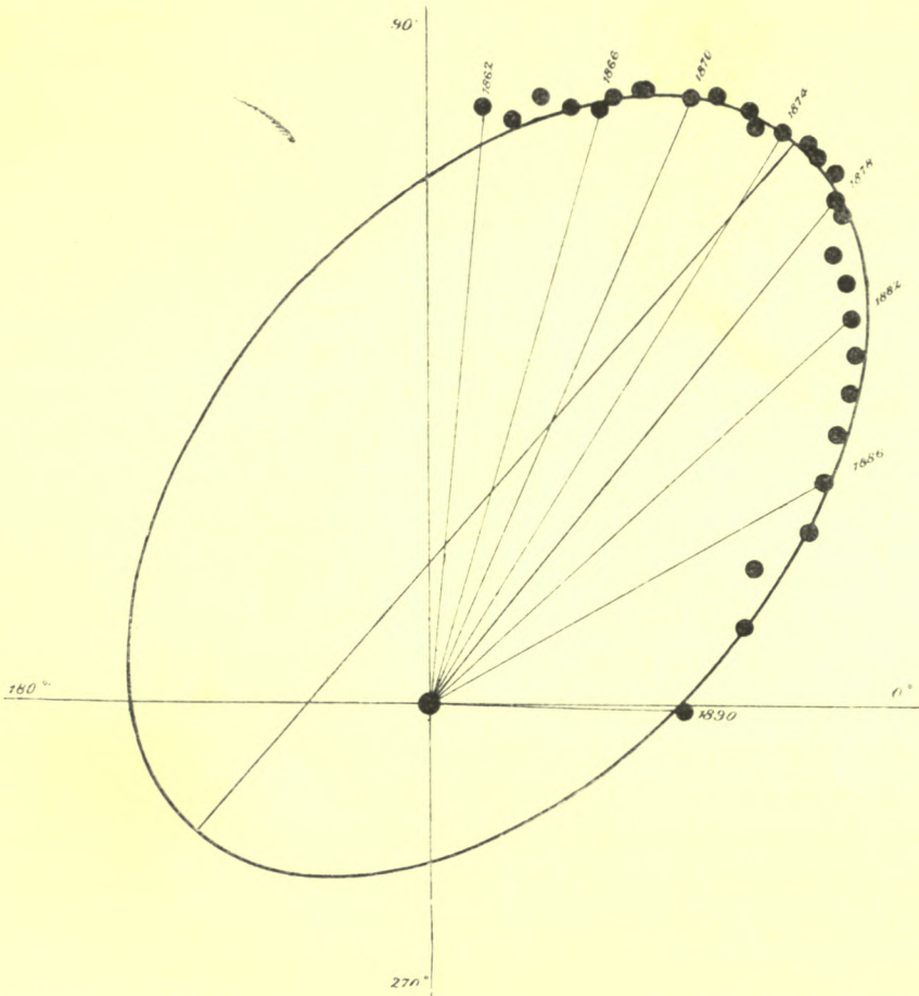
FIG. 465. Apparent orbit of the companion of Sirius, as plotted by Mr. Burnham from measures of its position angle and distance, from 1862 to 1890.
