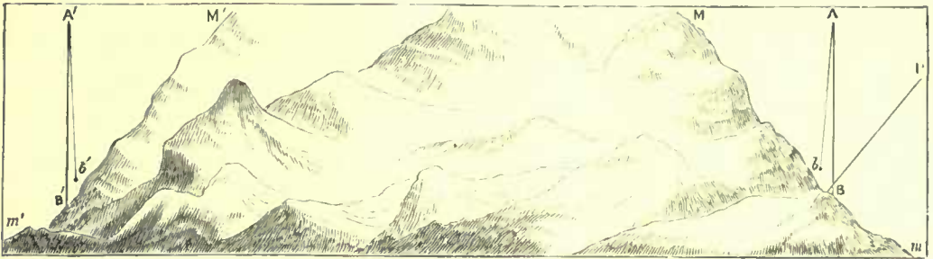
FIG. 198.—The Schhallien experiment for determining the Earth's mass.
