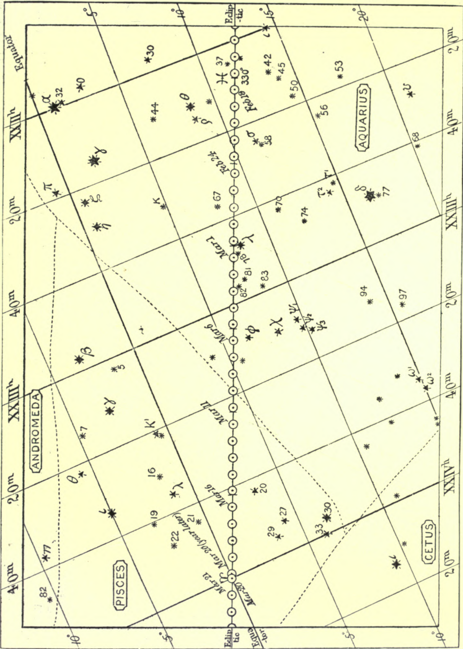
FIG. 88.—THE SUN'S COURSE THROUGH THE SIGN PISCES.
