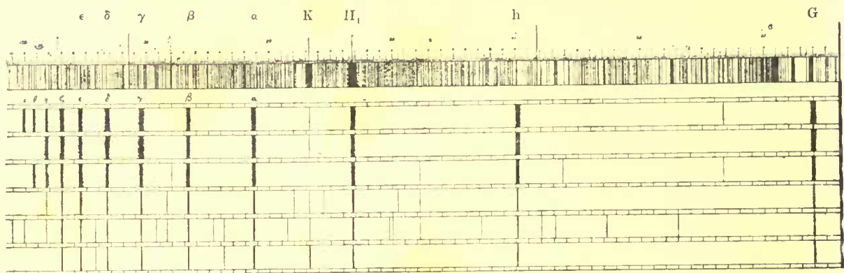
FIG. 472.—Diagram showing the relative intensity of the lines of the hydrogen spectrum in six stellar spectra. Photographed by Dr. Huggins. 1. Solar spectrum. 2. Spectrum of \alpha Lyrae. 3. Sirius. 4. \eta Ursae Majoris. 5. \alpha Virginis. 6. \alpha Aquilae. 7. \alpha Cygni. Copied from a paper on the Photographic Spectra of Stars in the 'Phil. Trans.' for 1880.
