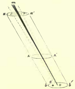
FIG. 290.—The cylindrical Shadow of the Moon in the Earth's atmosphere.
