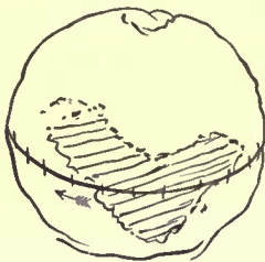
FIG. 361.—Drawing of Mars by Huyghens, August 13, 1672 (N.S.), 10.30 P.M., Paris mean time.
