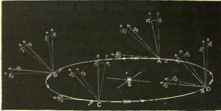
FIG. 164.—Illustrating the aberration of the Stars.
