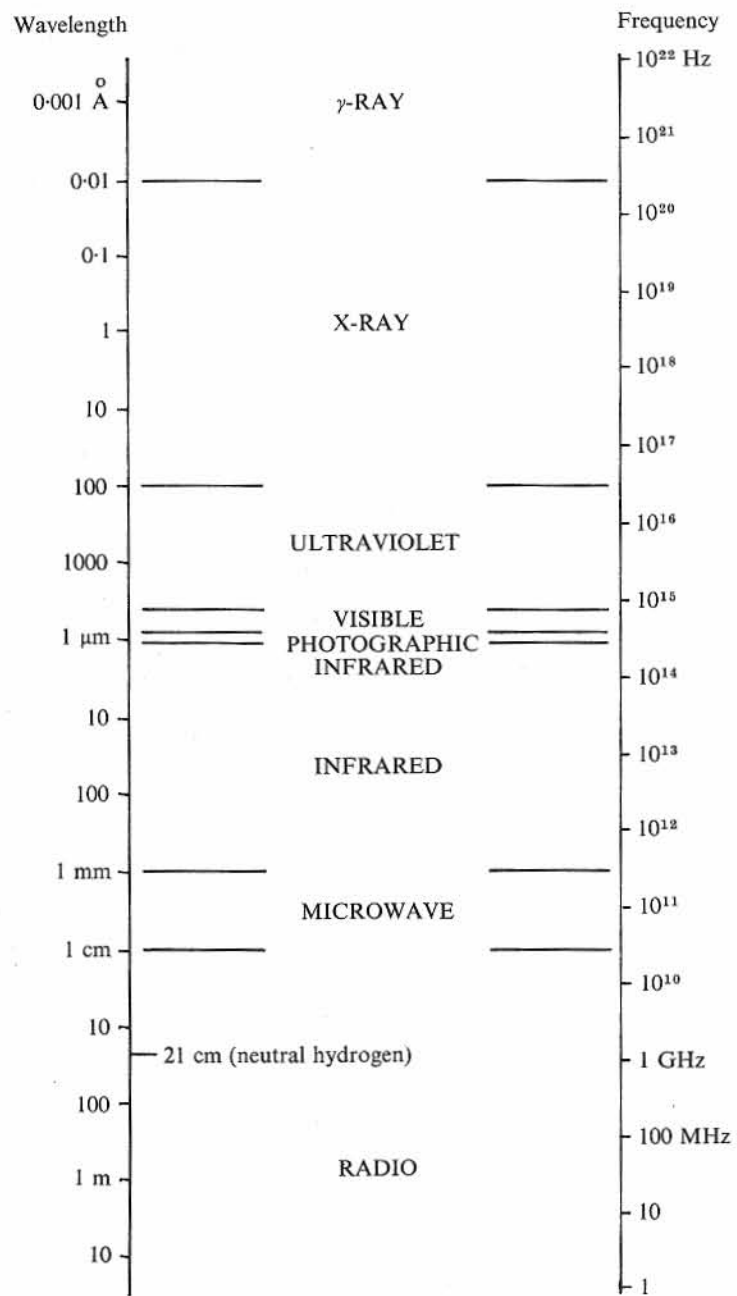
Fig. 2 The electromagnetic spectrum.
