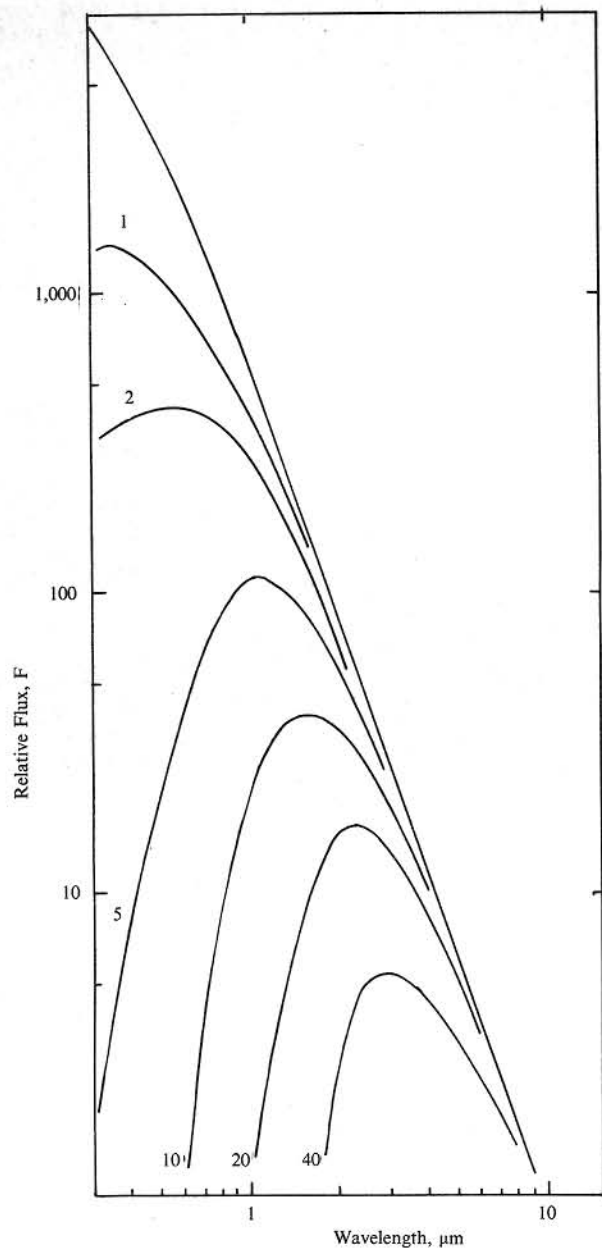
Fig. 34 The effects of reddening on the energy distribution of a hot stellar continuum. Numbers accompanying the curves are values of the visual extinction, A_v , in magnitudes.
