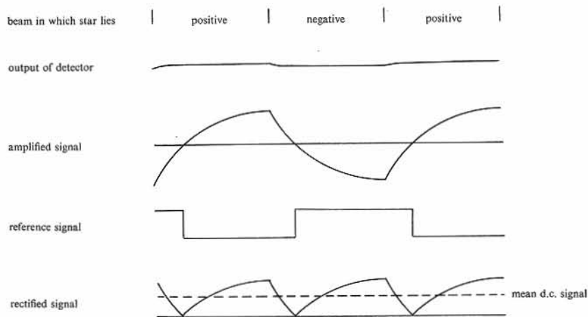
Fig. 10 Stages in the electronic processing of a signal
