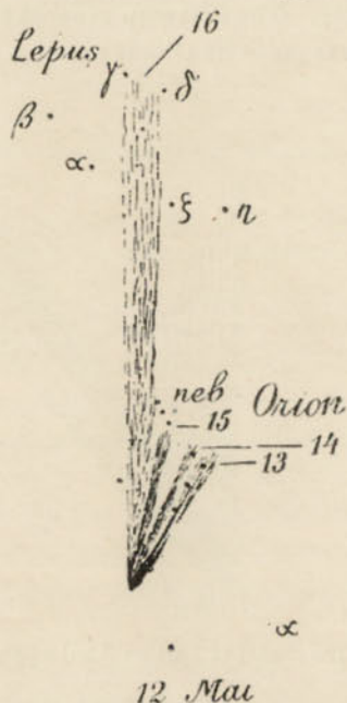
FIG. 41.—The Comet of 1901 on May 12.
