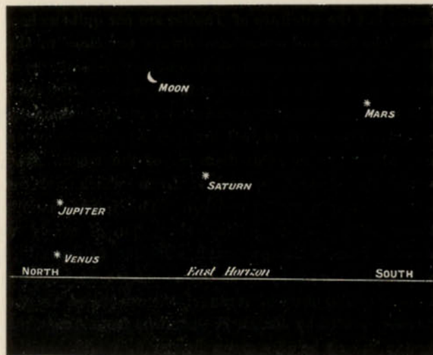
FIG. 28.—The East Horizon at 2 a.m. on the morning of 1881, June 22.
