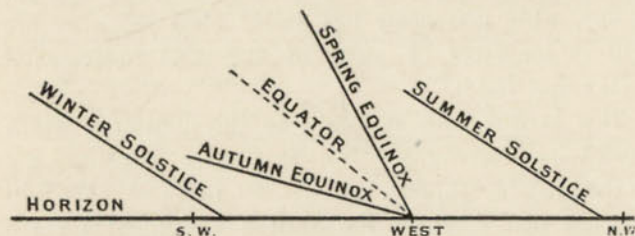
FIG. 34.—Inclination of the Ecliptic when the Equinoctial and Solstitial Points are on the West Horizon.
