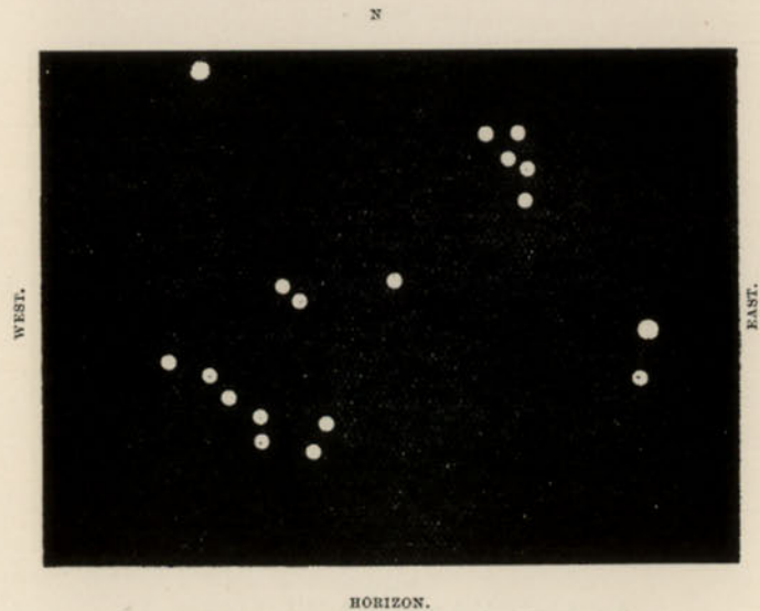
FIG. 8.—Looking north at Midnight on AUGUST 14.
