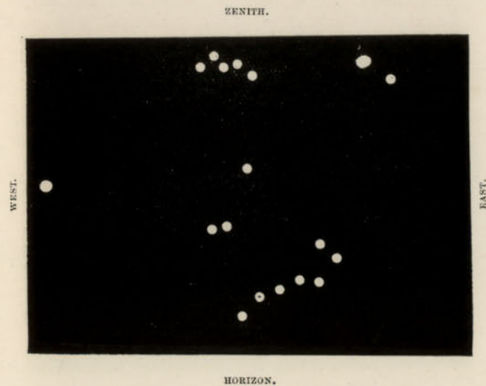
FIG. 10.—Looking north at Midnight on OCTOBER 14.
