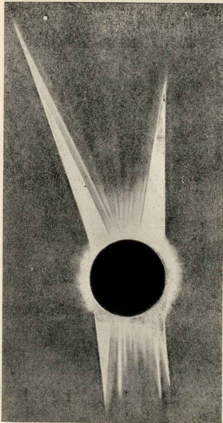
FIG. 43.—The Corona of 1900, May 28.
