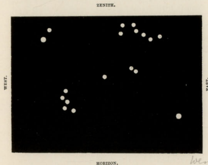
FIG. 2.—Looking north at Midnight on FEBRUARY 13.
