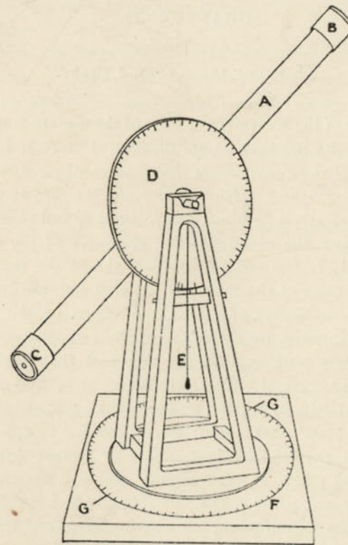
FIG. 24.—Pinhole Altazimuth for Observation of the Sun.
