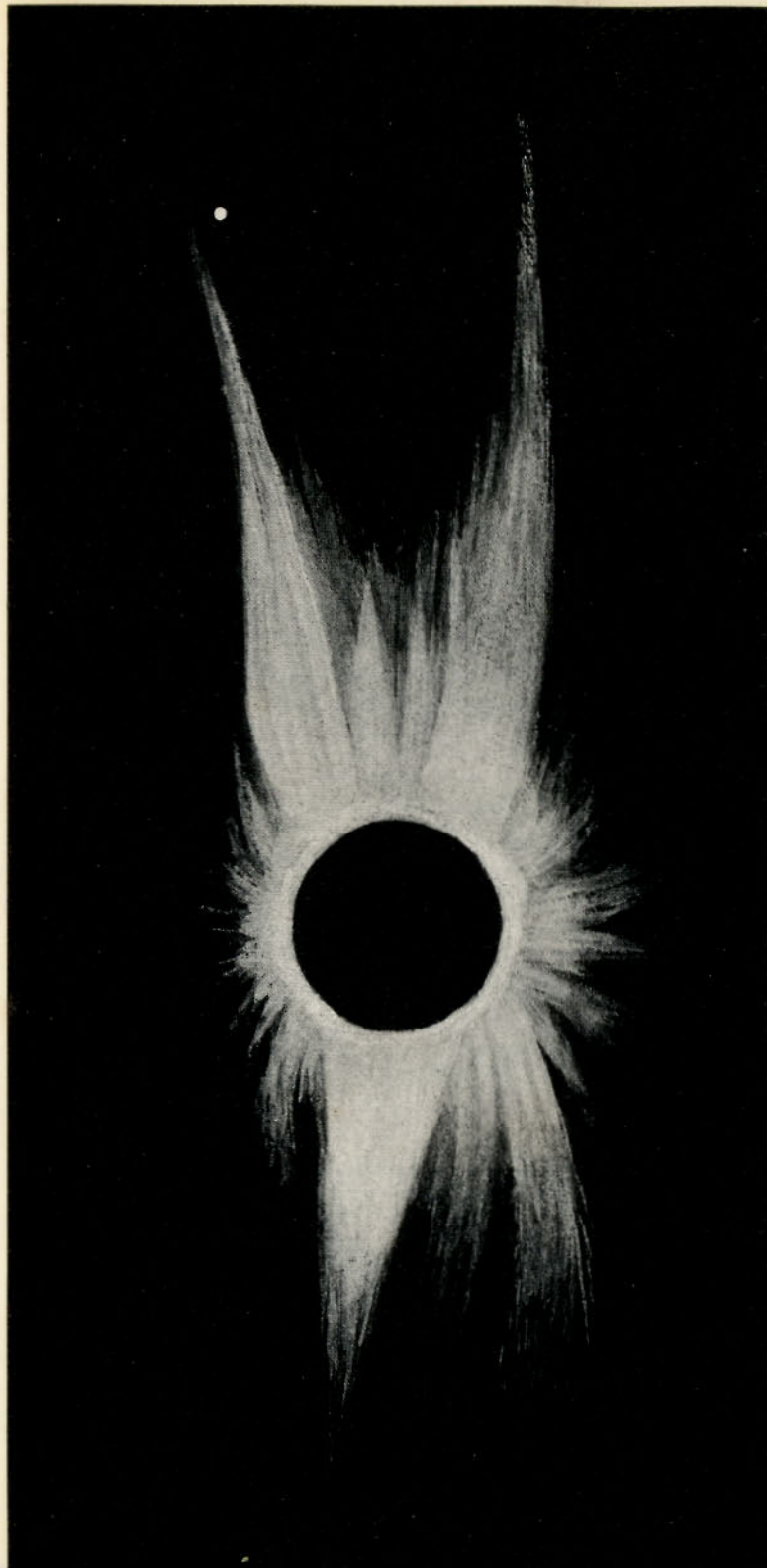
THE CORONA OF 1900, MAY 28.
