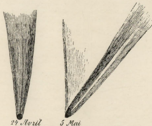
FIG. 40.—The Comet of 1901 on April 24 and May 5.
