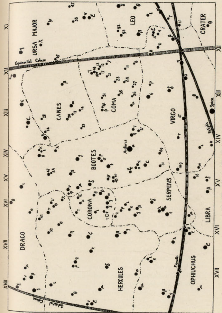
Star Map No. 4; The Region of Arcturus.
