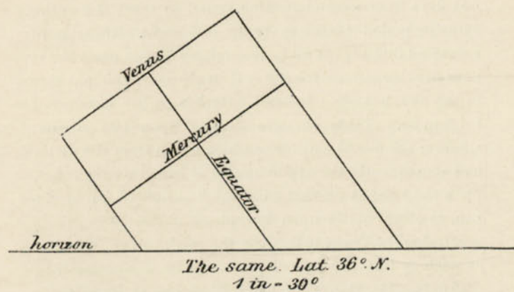
FIG. 27.—Positions of the Equator and Tropics, relative to the West horizon, for Latitudes 52^\circ and 36^\circ N.
