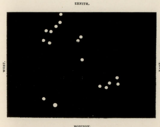
FIG. 5.—Looking north at Midnight on MAY 15.
