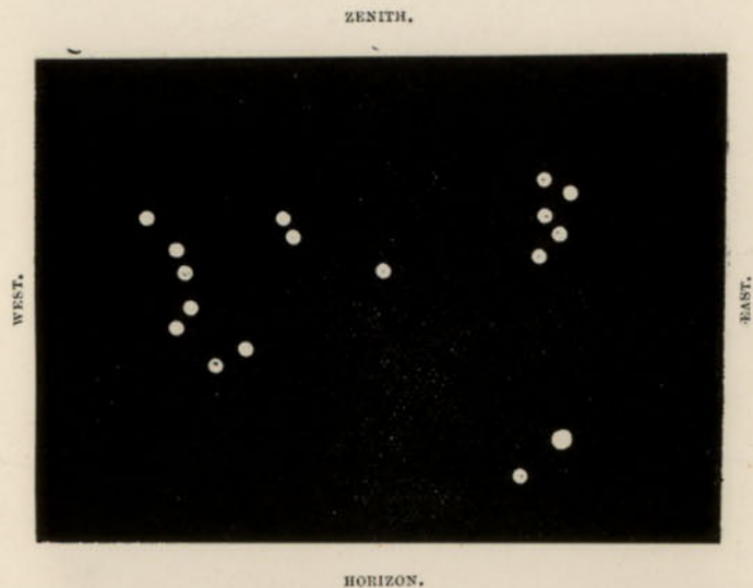
FIG. 7.—Looking north at Midnight on JULY 15.
