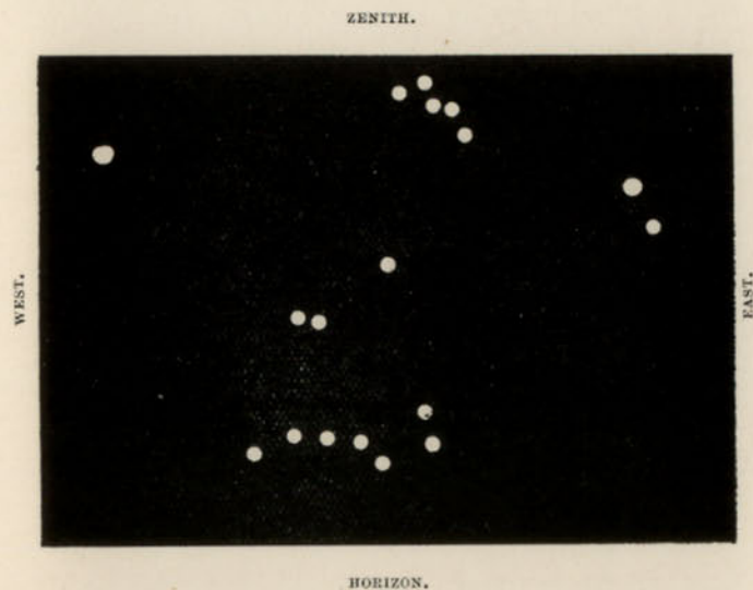
FIG. 9.—Looking north at Midnight on SEPTEMBER 14.
