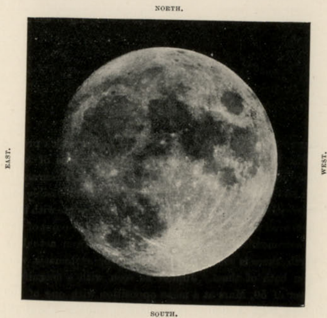
FIG. 29.—Photograph of Moon, taken 1902, March 22, 10h. 37m. 24s. G.M.T.
