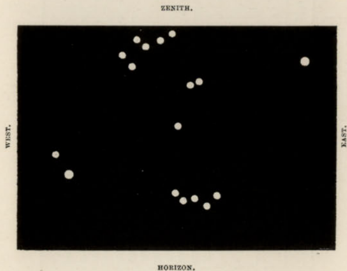
FIG. 4.—Looking north at Midnight on APRIL 15.
