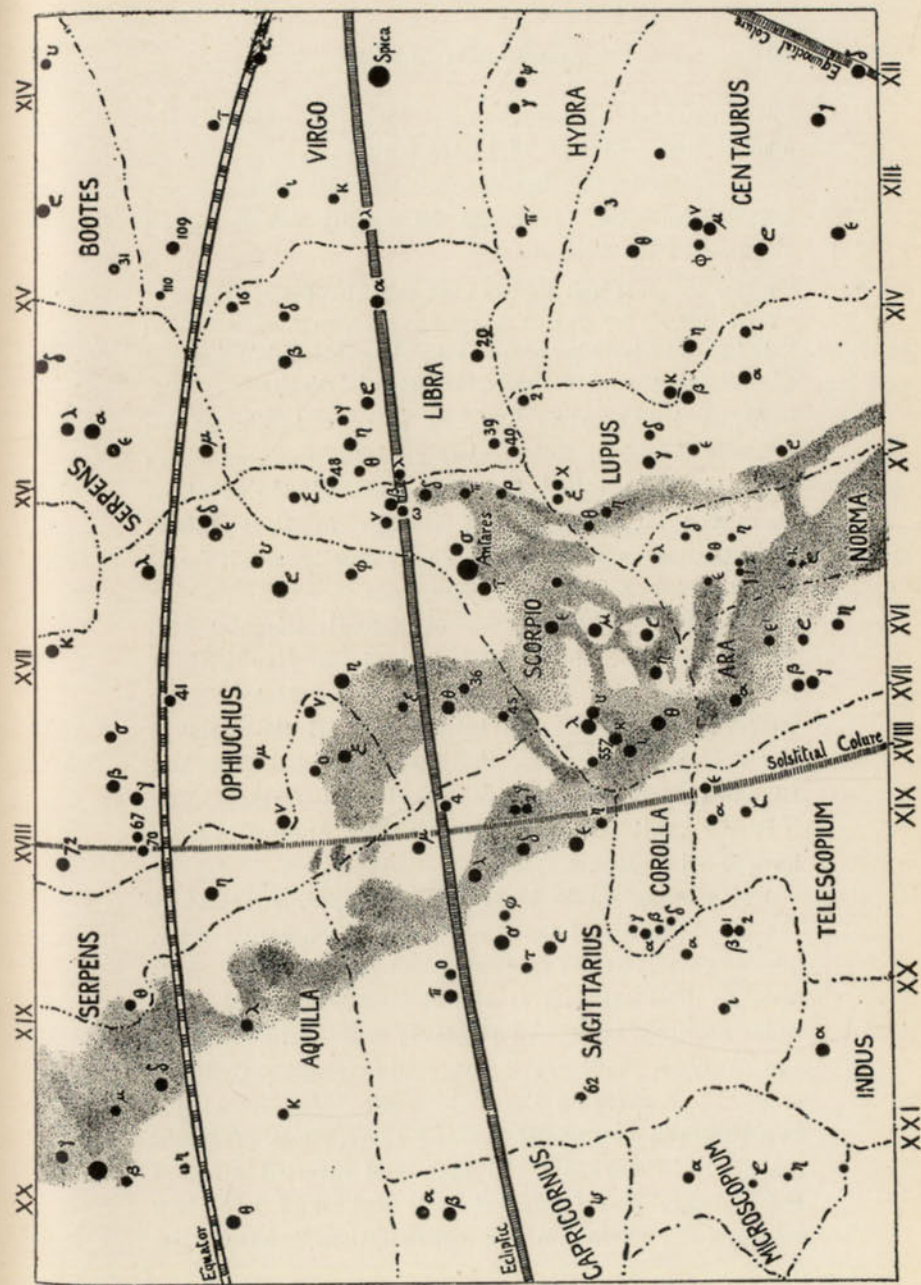
Star Map No. 5; The Region of the Scorpion.
