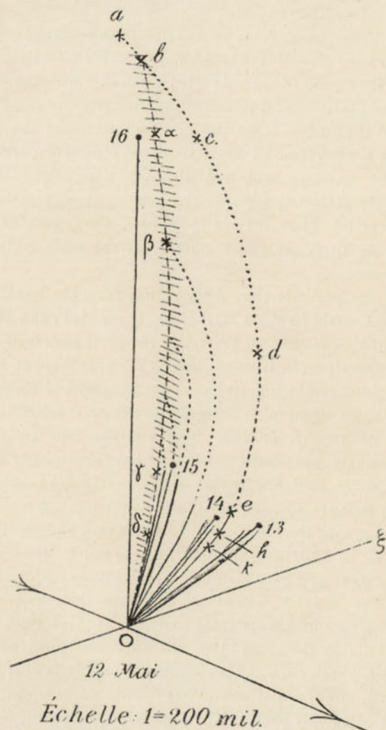
FIG. 42.—Prof. Brédikhine's analysis of the tail of the Comet on 1901, May 12.
