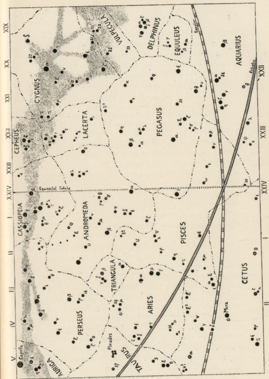
Star Map No. 7; The Region of the Royal Family.
