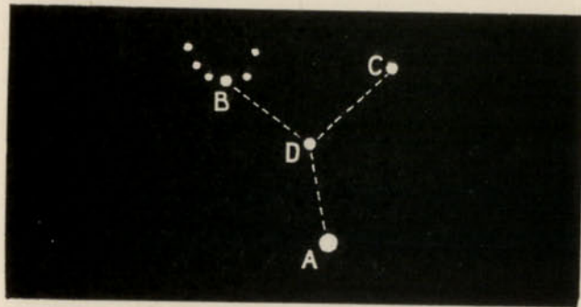
A, Arcturus. B, Alphecca. C, Gamma Bootis. D, Epsilon Bootis
