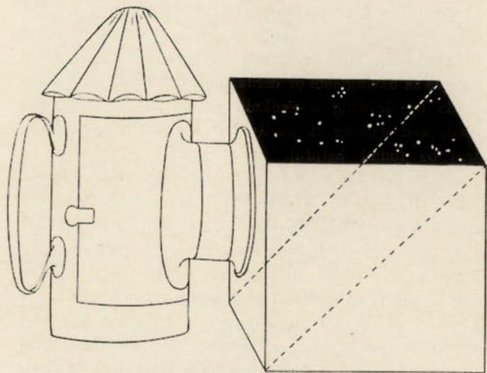
FIG. 35.—Illuminated Star Chart.
