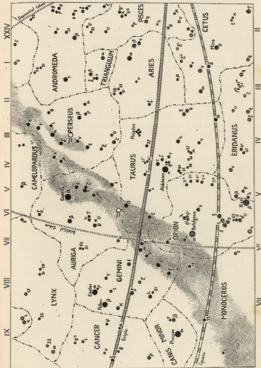
Star Map No. 10; The Region of Orion and the Bull.
