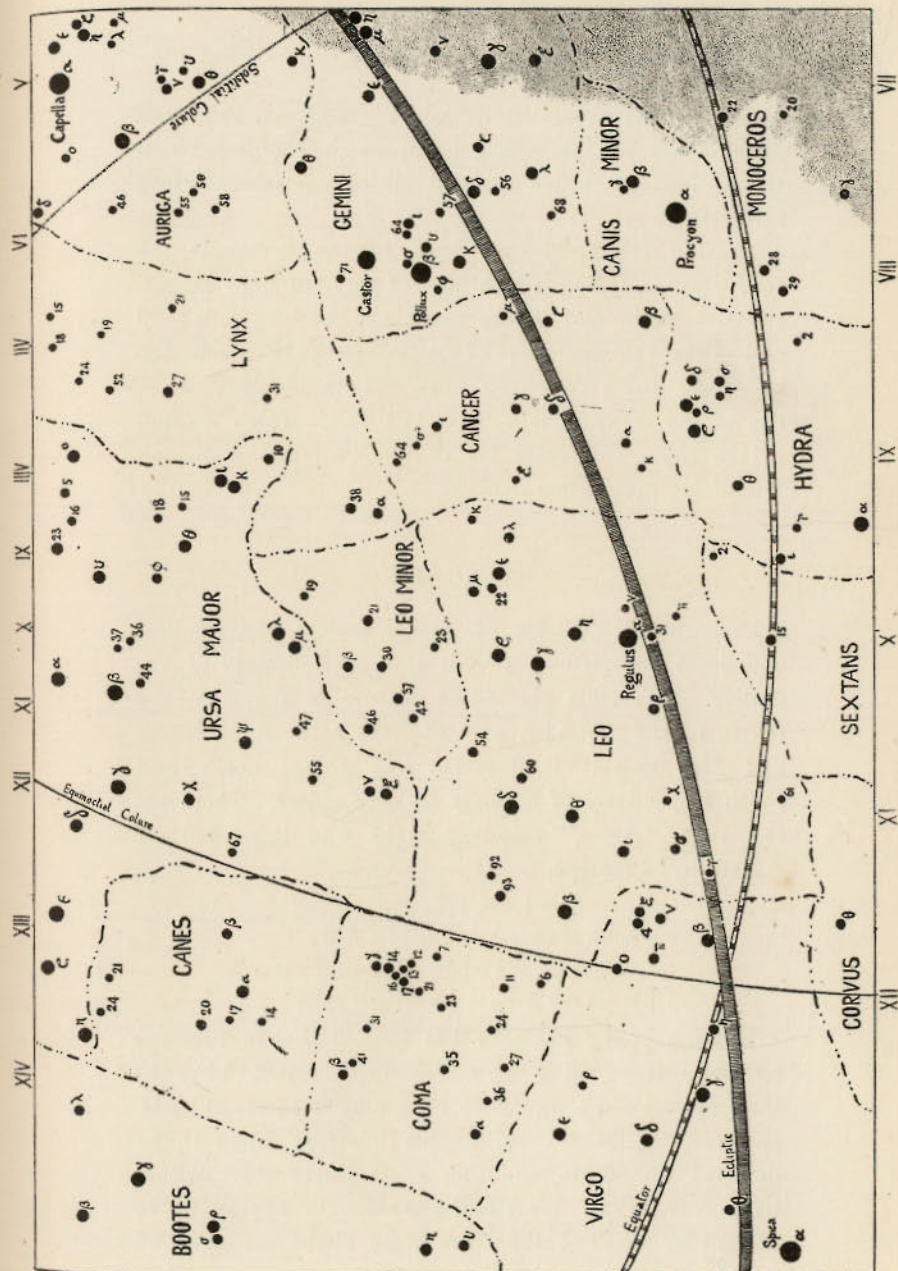
Star Map No. 2; The Region of the Lion.
