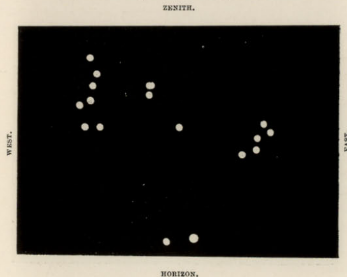
FIG. 6.—Looking north at Midnight on JUNE 14,
