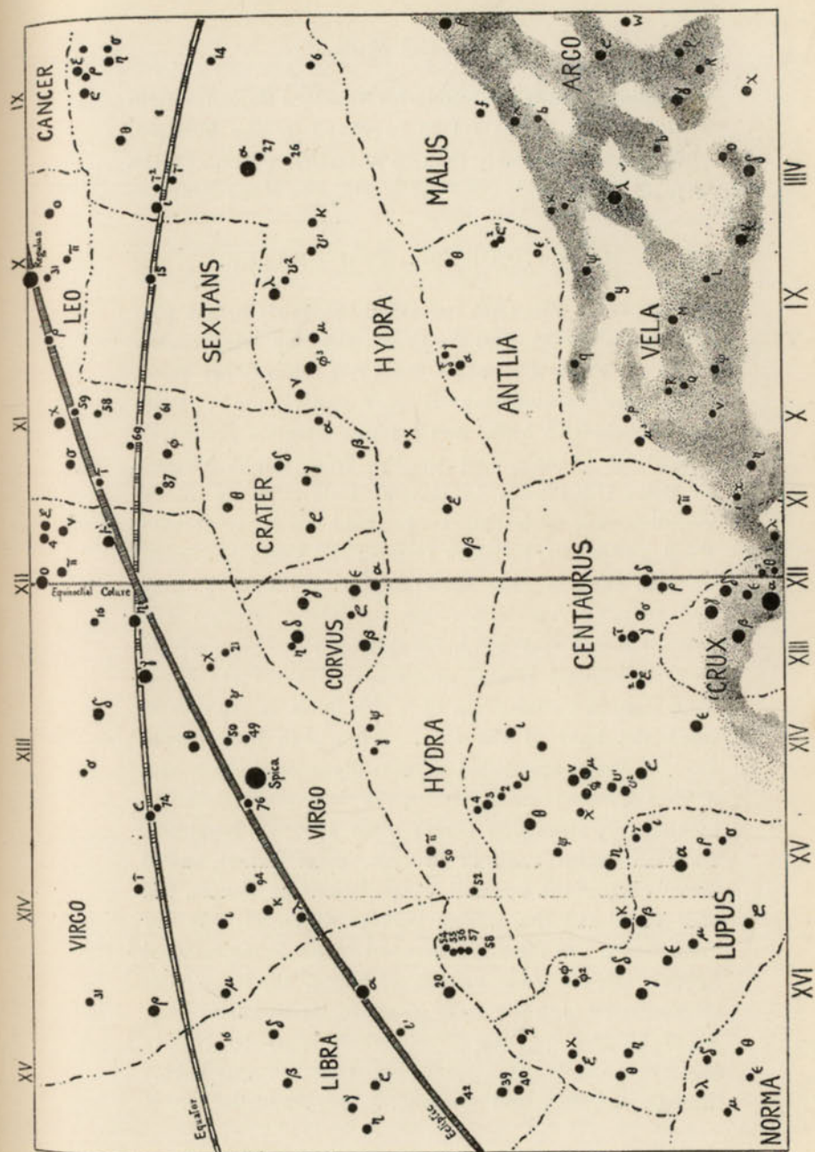
Star Map No. 3; The Region of the Water-Snake.
