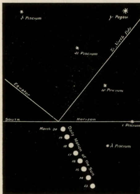
FIG. 26.—Positions of the Sun below the West horizon, near the Spring Equinox, at the setting of \epsilon Piscium.
