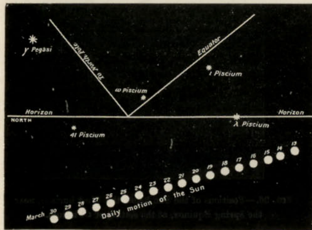
FIG. 25.—Positions of the Sun below the East horizon, near the Spring Equinox, at the rising of \lambda Piscium.
