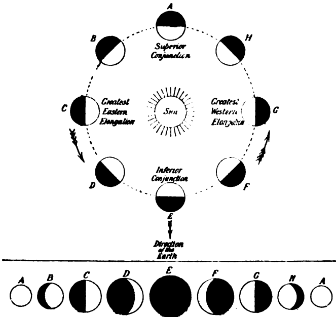
Corresponding views of the same situations of an Inferior Planet as seen from the Earth, showing consequent phases and alterations in apparent size.
