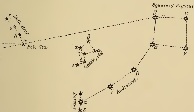
FIG. 6.—To find Pegasus and Andromeda.
