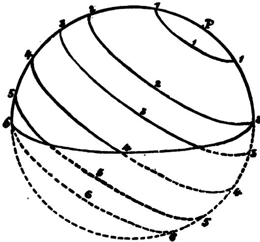
Diagram of Circles (VI).
