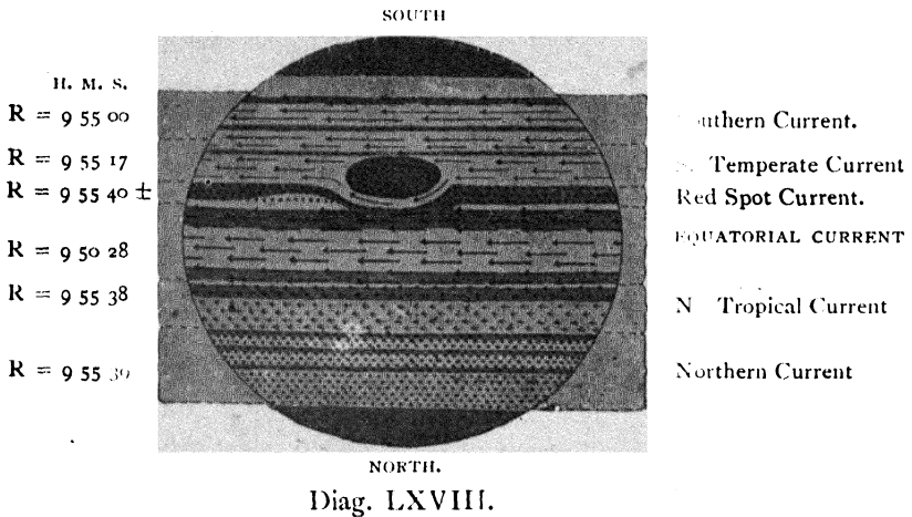
SURFACE CURRENTS OF JUPITER IN 1887-8.
