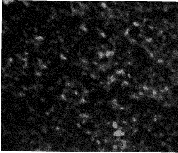
Diag. LVII.--Granules on Sun.
