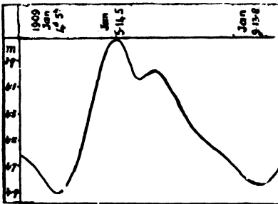
Diag. XCII. Light changes of \delta Cephei.
