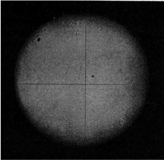
Diag. LVI.—Photograph of Sun.
