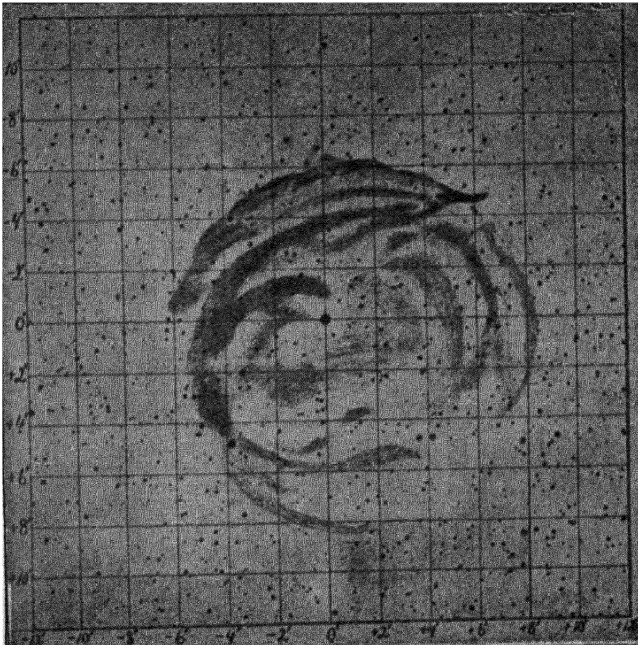
Diag. XCIV. Nebula surrounding Nova Persei ( Ritchey ).
