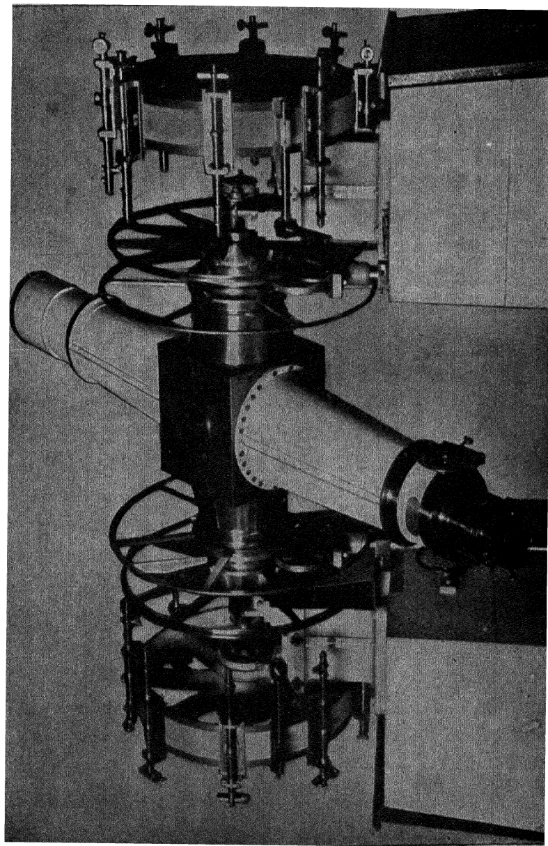
Diag. XL.—Transit-Circle.
