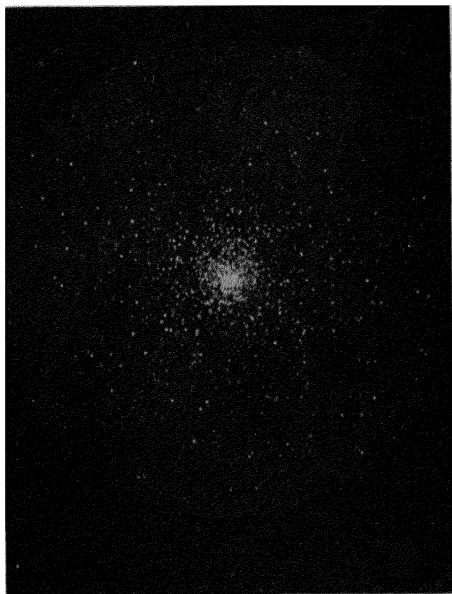
Diag. LXXXVI.—Cluster of Stars.
