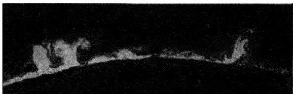
Diag. LVIII.—Solar Prominences.
