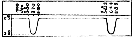
Diag. LXXXVIII. Light changes of Algor.
