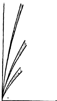
Diag. LXXII.— Types of Comets' Tails.
