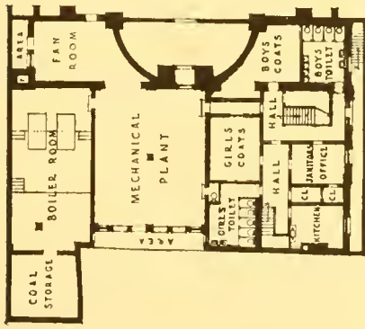
BASEMENT PLAN
