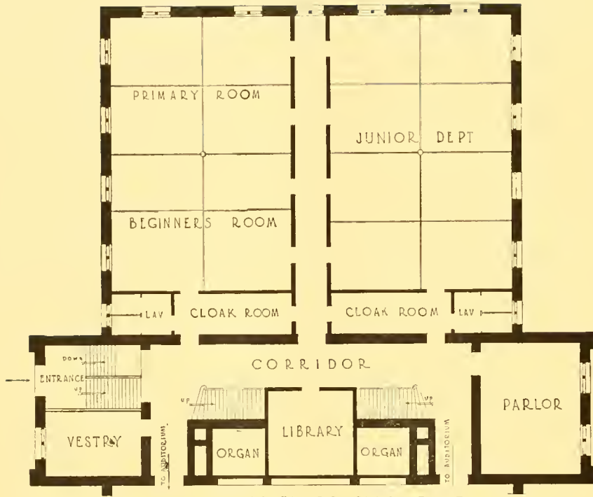
MAIN FLOOR PLAN • REAR PART
