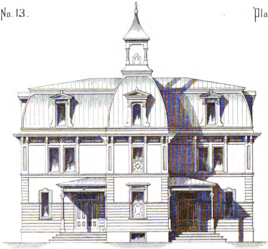
FRONT ELEVATION AND FIRST FLOOR PLAN 1/16 inch to the foot
