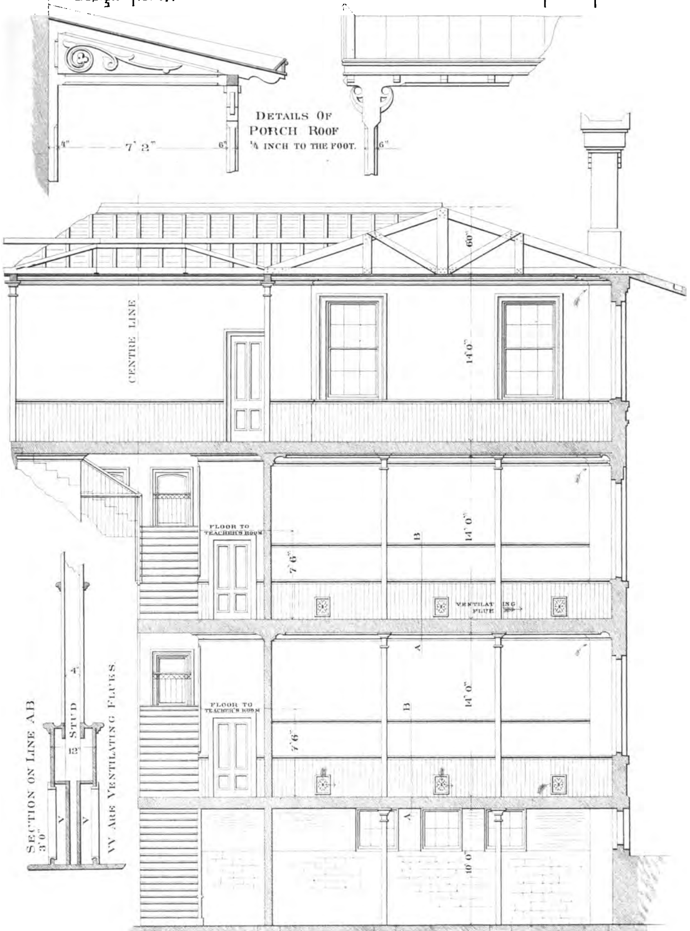
HALF LONGITUDINAL SECTION 1/8 INCH TO THE FOOT.
