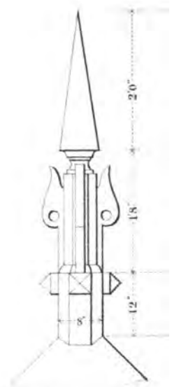
FINIAL
