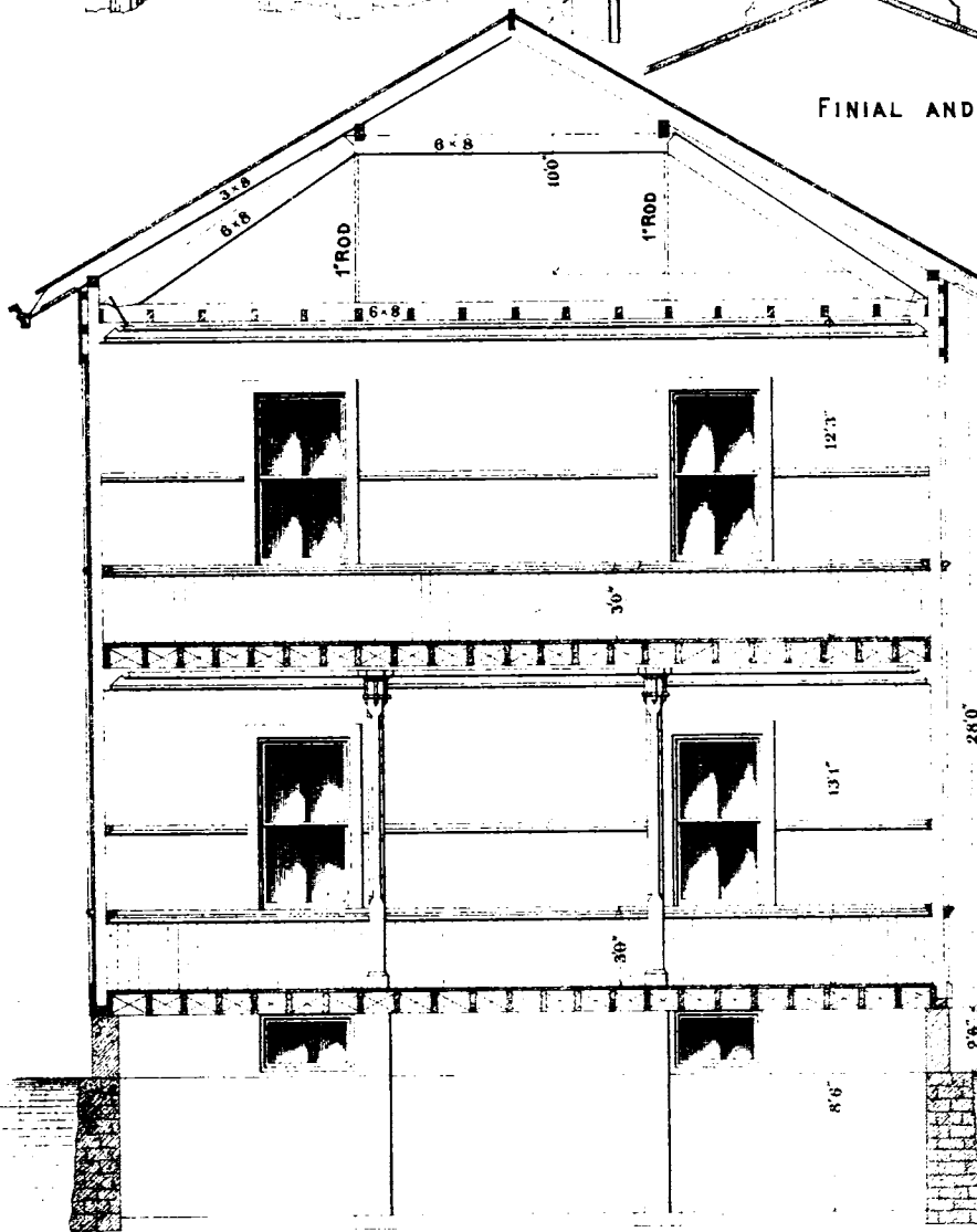
CROSS SECTION 1/8 inch to the foot
