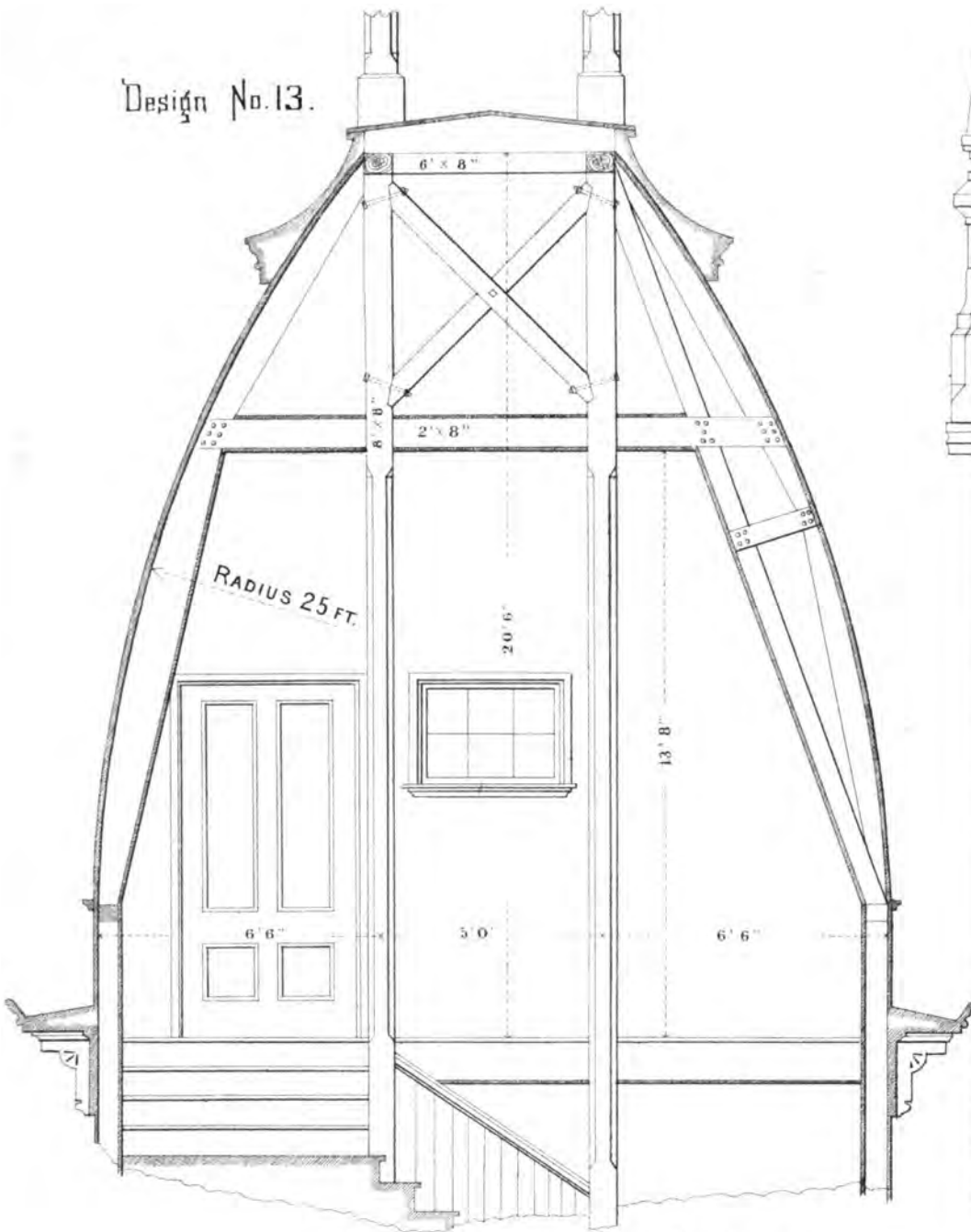
SECTION OF TOWER ROOF. SHOWING FRAMING 1/4 inch to the foot.
