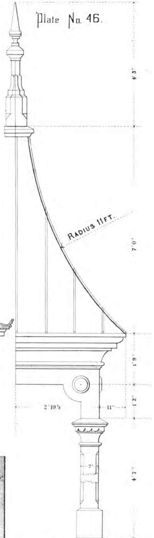
BELFRY FINISH.
