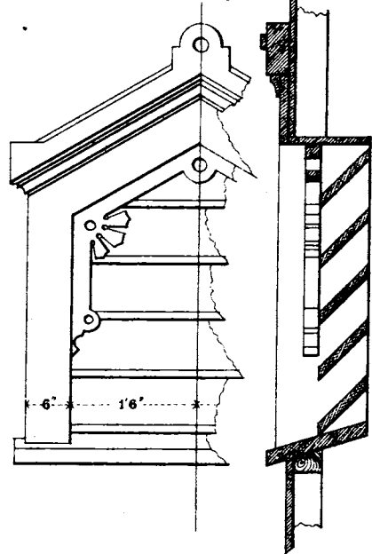
GABLE WINDOWS
