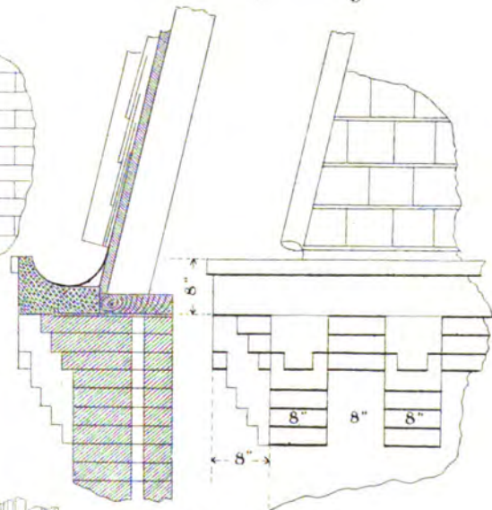
MAIN CORNICE
