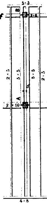
METHOD OF FRAMING GIRDERS TO POSTS. GIRDER AT A 6" x 10", AT B 8" x 8", 3/4 INCH BOLT AT END OF EACH
