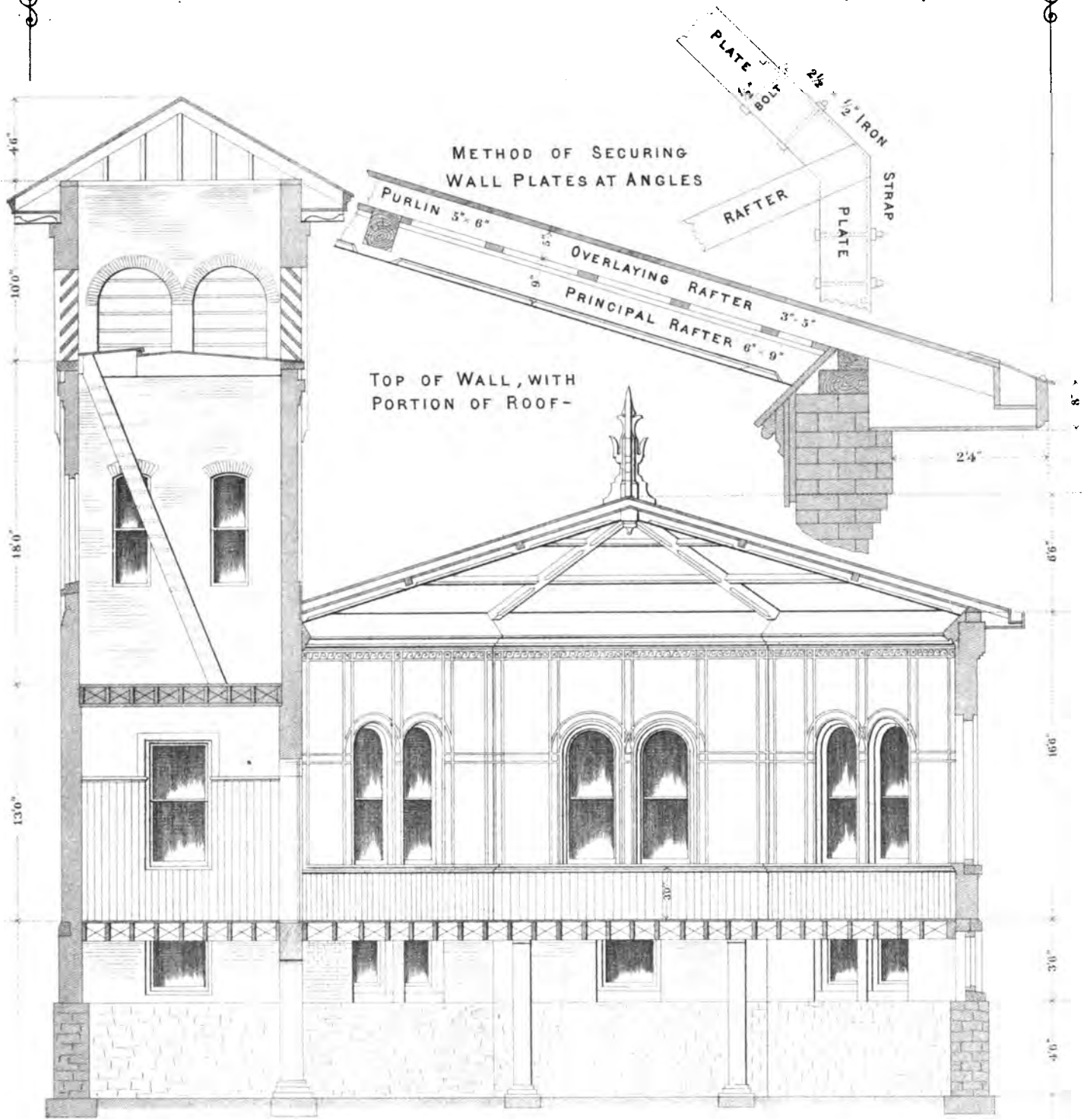
SECTION ON LINE A B 1/2 inch to the foot
