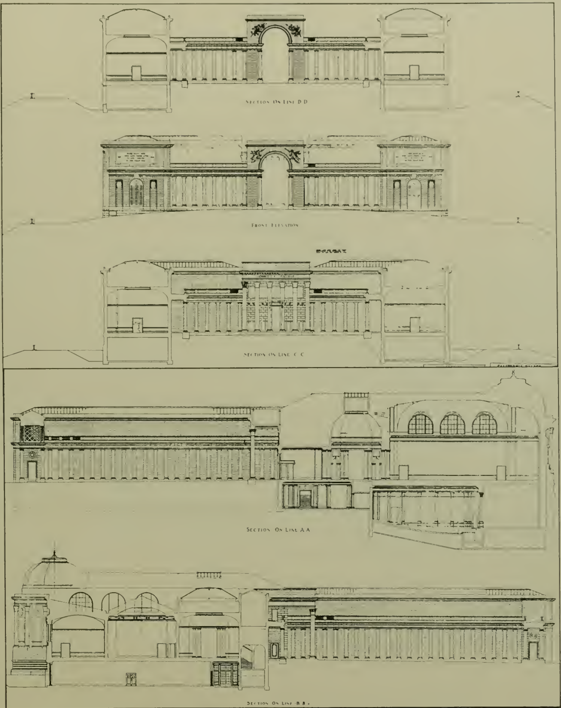
DETAIL DRAWINGS—CALIFORNIA PALACE OF THE LEGION OF HONOR. GEORGE A. APPLGARH, ARCHITECT
