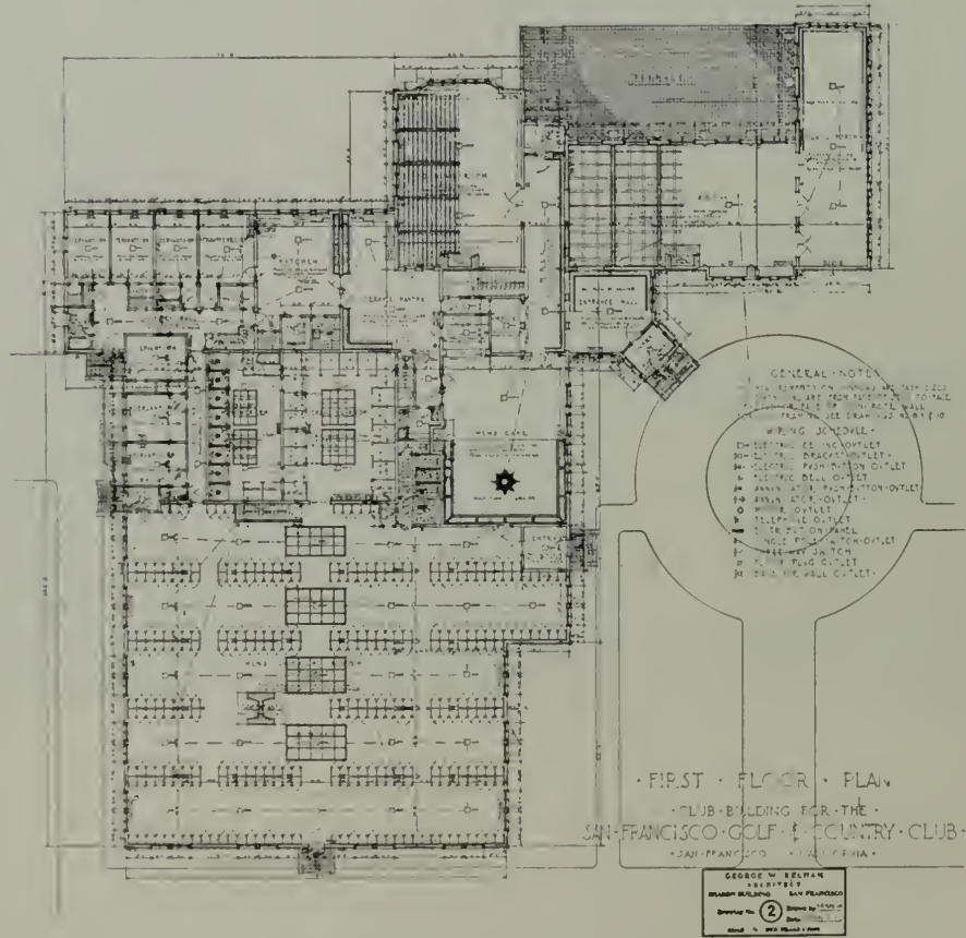
UPPER: SECOND FLOOR PLAN, SAN FRANCISCO GOLF AND COUNTRY CLUB, SAN FRANCISCO. LOWER: FIRST FLOOR PLAN, SAN FRANCISCO GOLF AND COUNTRY CLUB, SAN FRANCISCO, GEO. W. KELHAM, ARCHITECT
