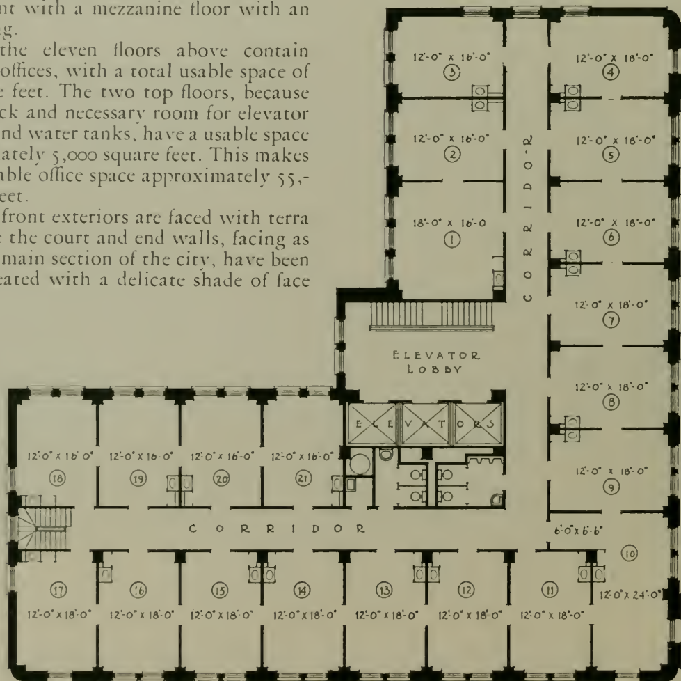
TYPICAL FLOOR PLAN, CALIFORNIA STATE LIFE BUILDING, SACRAMENTO, CALIFORNIA GEORGE C. SELTON AND COMPANY, ARCHITECTS
