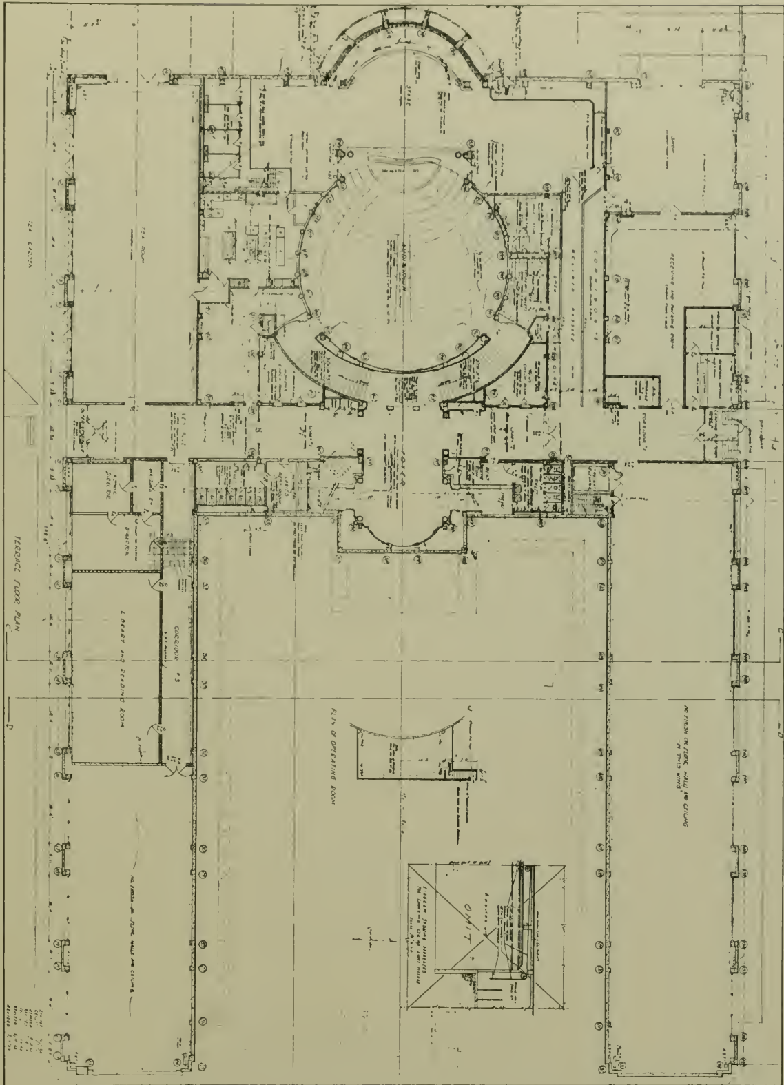
BASEMENT PLAN—CALIFORNIA PALACE OF THE LEGION OF HONOR. GEORGE A. APPELGARTH, ARCHITECT
