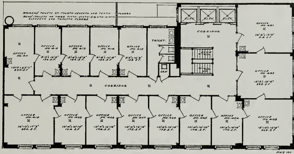
TYPICAL FLOOR PLAN (4th to 12th floors)
