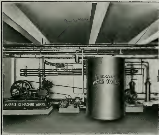
Water Cooling Plant Installed in the Yeon Building By the Harris Ice Machine Works
