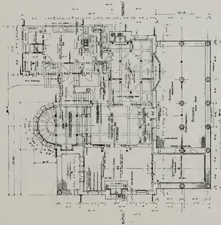
FIRST FLOOR PLAN 1/8" = 1'-0"
