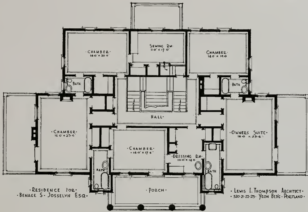
• SECOND FLOOR PLAN • • SCALE 1/8" = 1'-0" •
