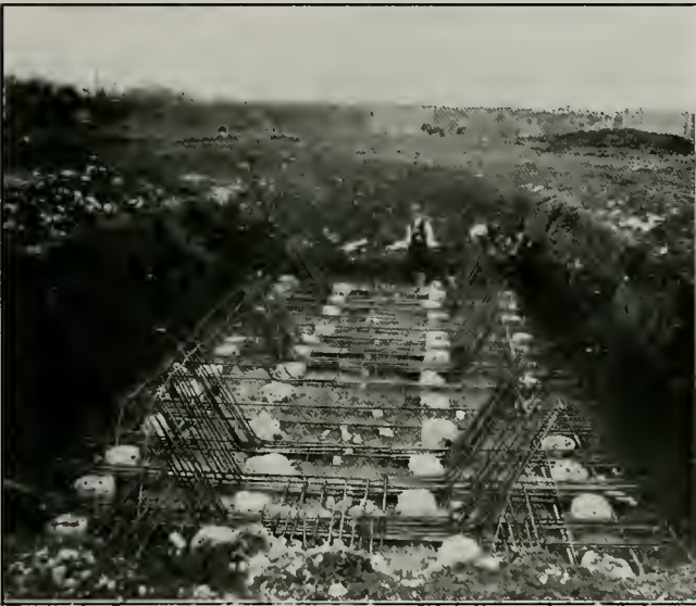
Bed of "Portland Concrete Piles," showing reinforcement: ready for cap.
