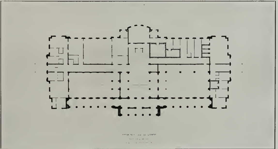
First Honorable Mention, Temple of Justice and First Floor Plan Washington State Capitol Competition Mr. G. Albert Lansburgh, Architect, San Francisco, Calif
