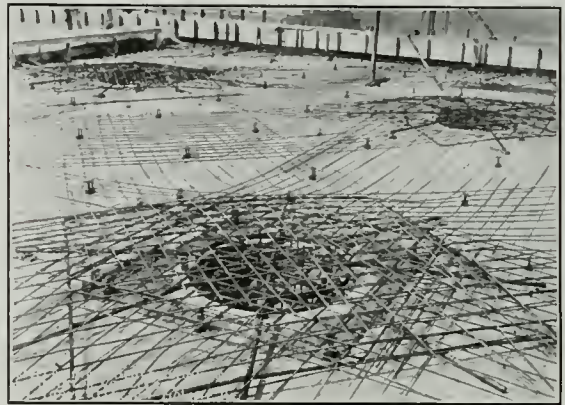
CORRECT ARRANGEMENT OF SLAB STEEL. THIS PREVENTS CRACKS AROUND THE COLUMN HEAD
