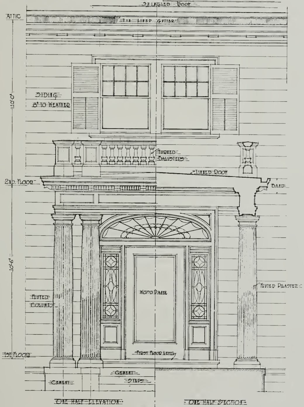
Front Porch Detail, Residence for Judge W. B. Gilbert Smith & Hall, Architects, Portland
