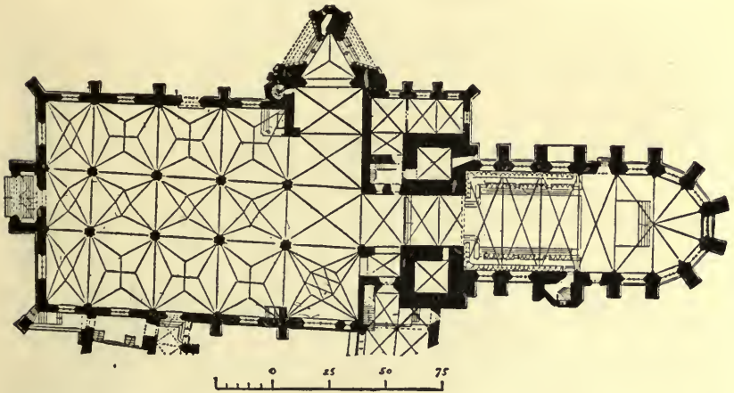
FIG. 160. Erfurt, Germany: Cathedral. Plan. Choir 1350 to 1355 A.D. Nave much later. Choir and nave have different axes.
