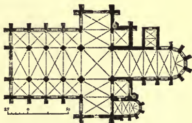
FIG. 155. Vilvorde, Belgium: Church. Fourteenth century. Plan.
