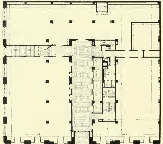
FIRST FLOOR PLAN, NORTHERN LIFE TOWER
