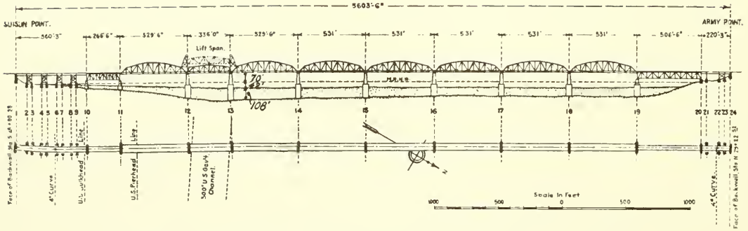
FIG. 2—SUPERSTRUCTURE, SUISUN BAY BRIDGE, NEAR BENICIA, CALIFORNIA
