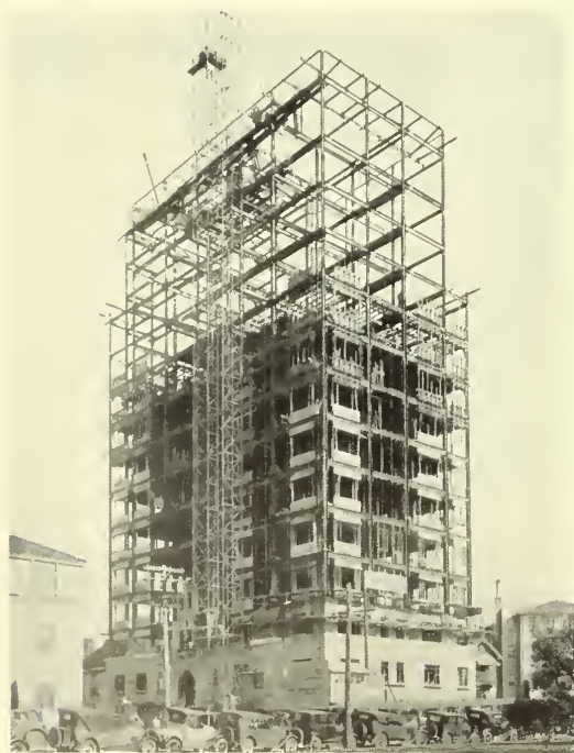
STEEL FRAME OF BELLEVUE-STATEN APARTMENTS, OAKLAND
