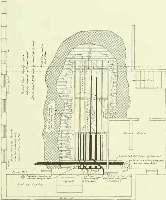
FIG. 1—PLAN OF BUILDING ATTACKED BY TERMITES
