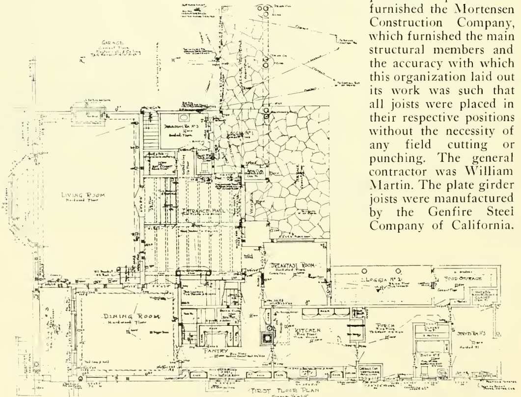
PLAN, RESIDENCE FOR N. F. BALDOCCHI, SEA CLIFF, SAN FRANCISCO Bertz, Winter & Maury, Architects
