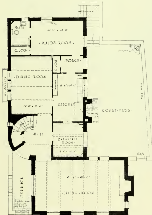
PLANS, STEEL FRAME, HOLLOW TILE RESIDENCE, PIEDMONT Miller & Warnecke, Architects
