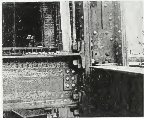
TYPICAL VIEW OF BEAM WIND CONNECTIONS TO COLUMN, FOX THEATER
