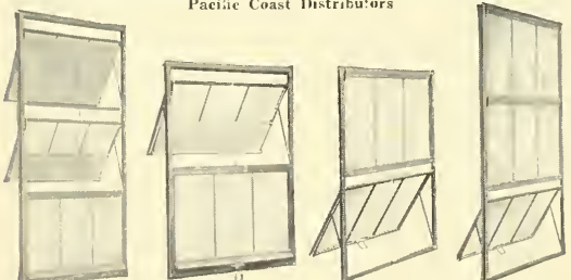
Upper two sash open — bottom sash closed. Upper sash open — lower sash closed. Upper sash closed — lower sash open. Bottom sash open — upper two sash closed.
