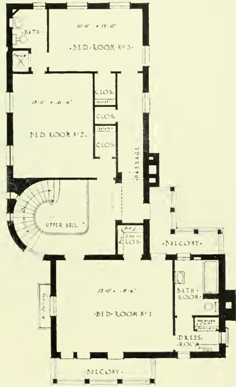
PLANS, STEEL FRAME, HOLLOW TILE RESIDENCE, PIEDMONT Miller & Warnecke, Architects
