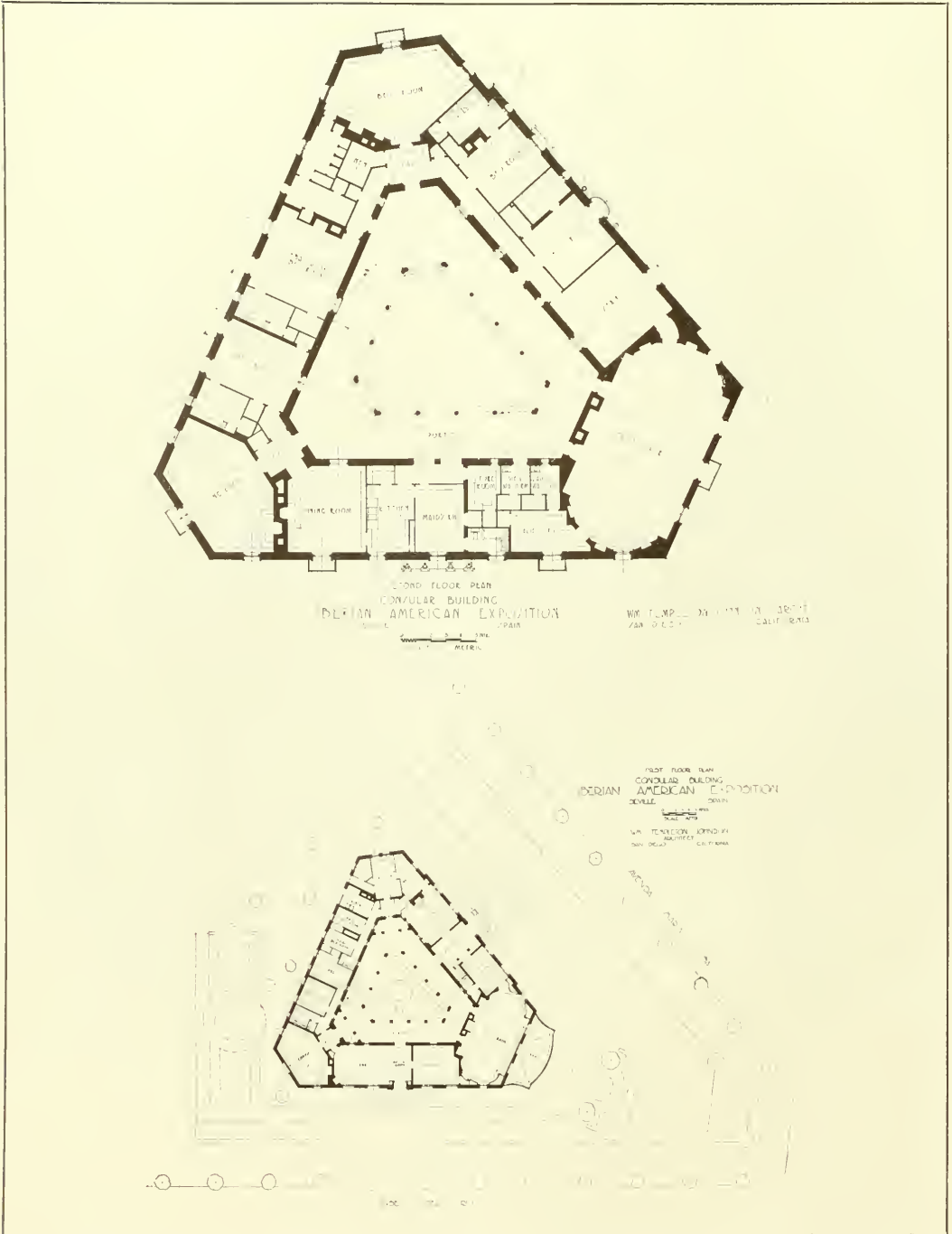
PLANS, FUTURE CONSULATE, U. S. EXPOSITION BUILDING, SEVILLE, SPAIN WM. TEMPLETON JOHNSON, ARCHITECT
