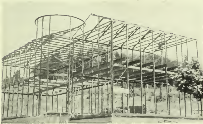
STEEL FRAME FOR RESIDENCE IN PIEDMONT, CALIFORNIA Roper and Gill, Structural Engineers
