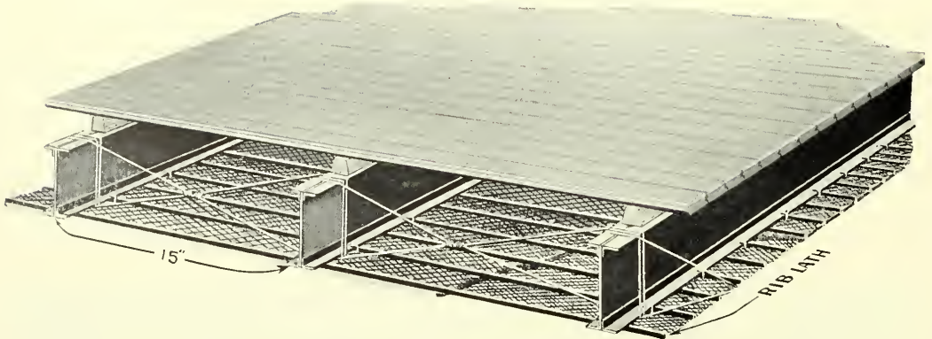
TYPICAL FLOOR CONSTRUCTION USED THROUGHOUT RESIDENCE OF N. F. BALDOCCHI
