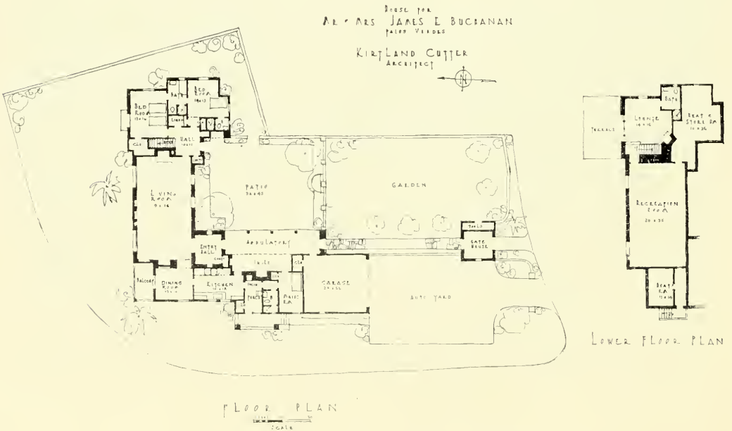
PLAN RESIDENCE OF JAMES E. BUCHANAN, PALOS VERDES ESTATES Kirtland Cutter, Architect
