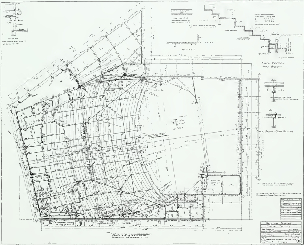
BALCONY FRAMING, FOX THEATER, SAN FRANCISCO
