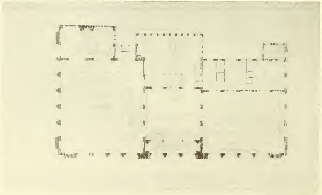
GROUND FLOOR PLAN, PUBLIC LIBRARY BUILDING, BERKELEY James W. Plachek, Architect
