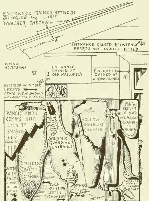
FIG. 2—HOW DRY-WOOD TERMITES MAY ATTACK THE FRAMEWORK OF A BUILDING
