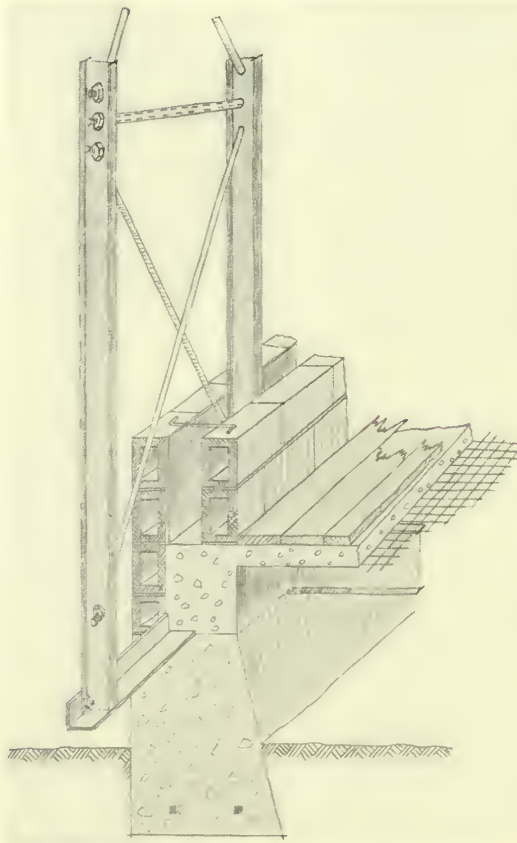
SECTIONAL VIEW OF WALL CONSTRUCTION, STEEL FRAME AND HOLLOW TILE RESIDENCE, PIEDMONT
